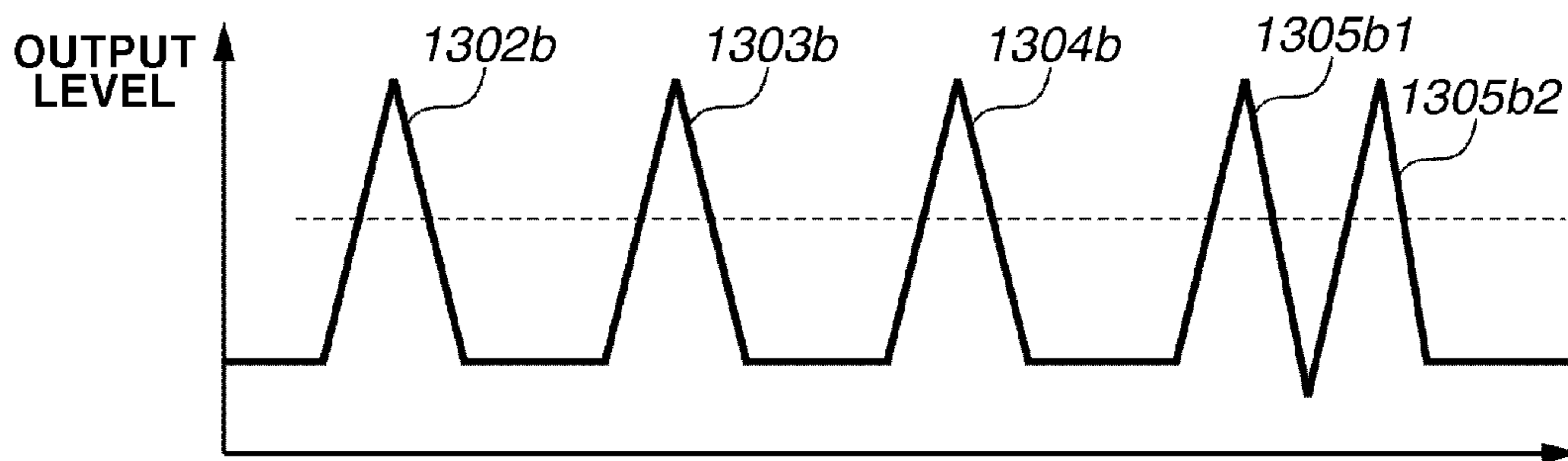
FIG.13C PRIOR ART
