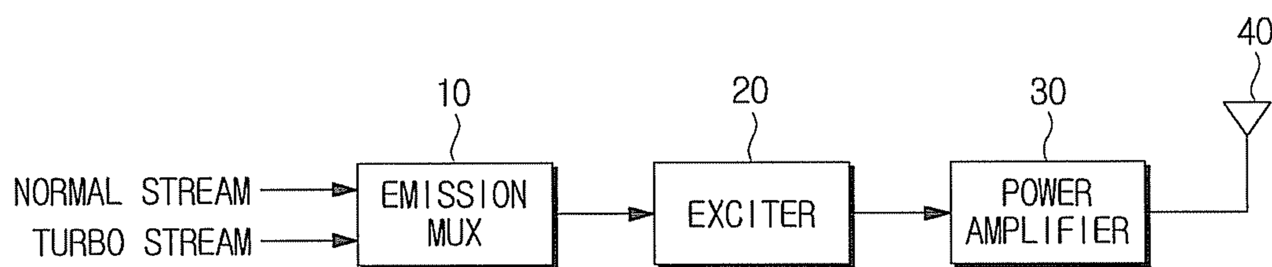
FIG. 1 (RELATED ART)
