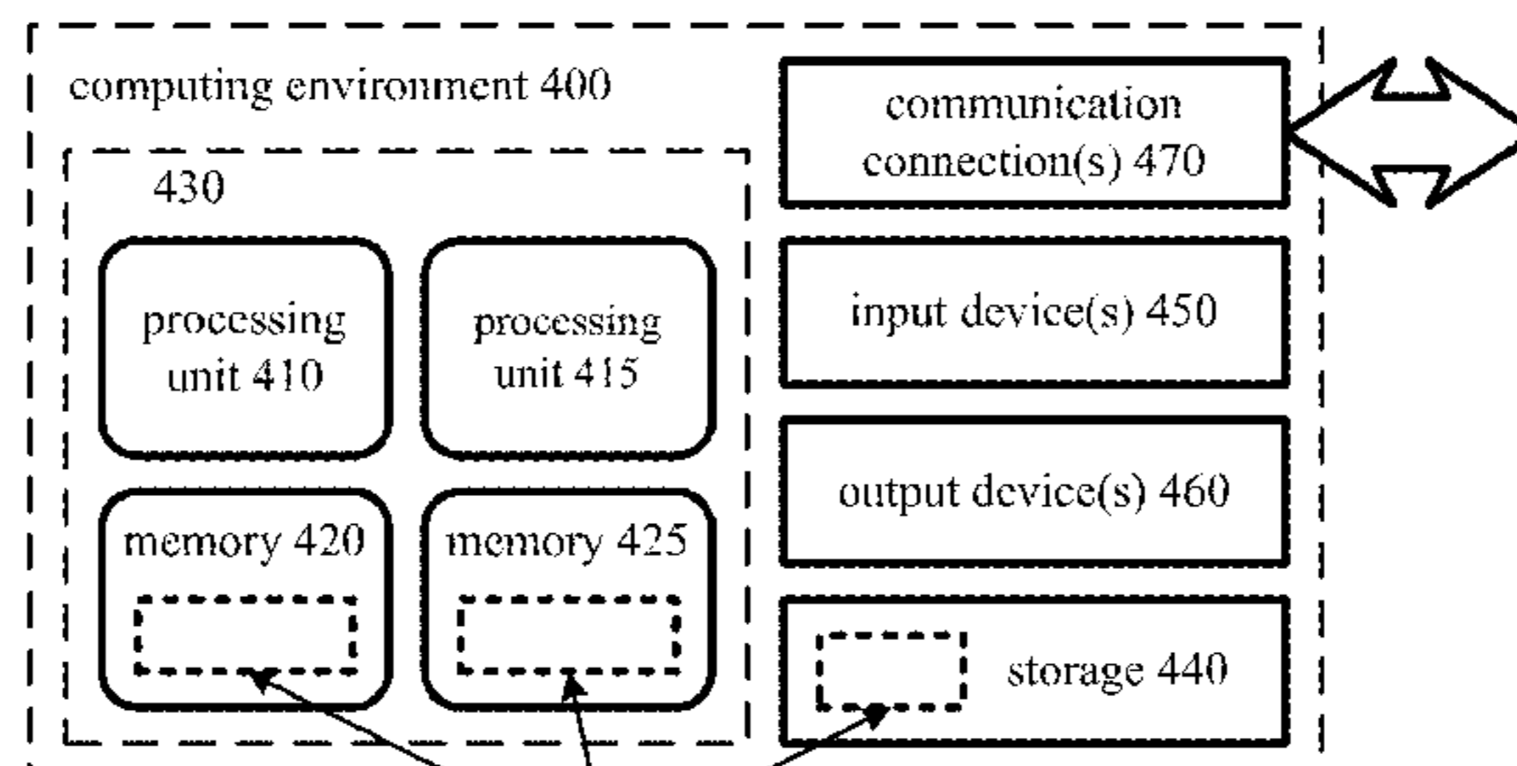
software 480 implementing described multi-threading techniques and tools for video decoding
