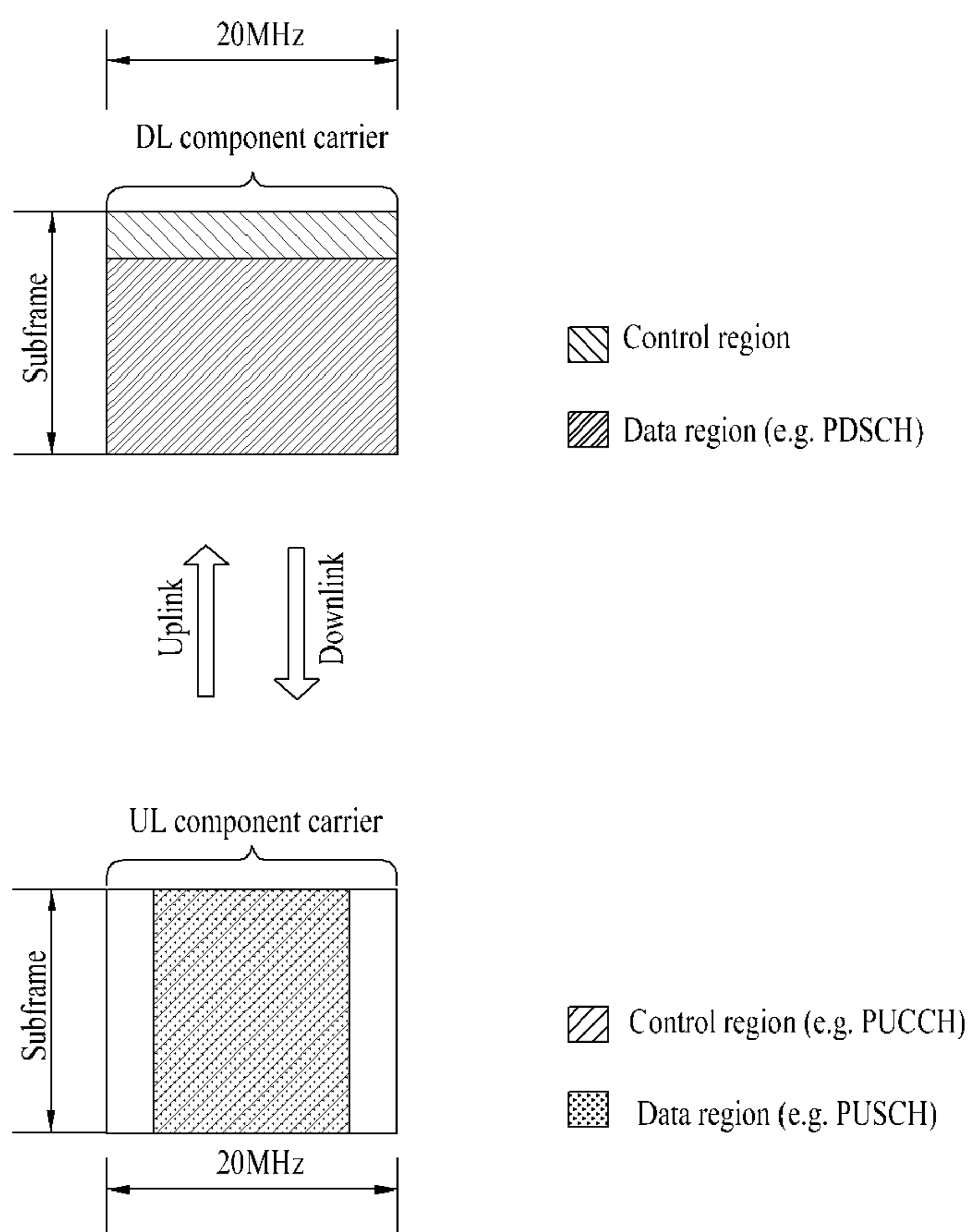
Single component carrier (e.g. LTE system)
