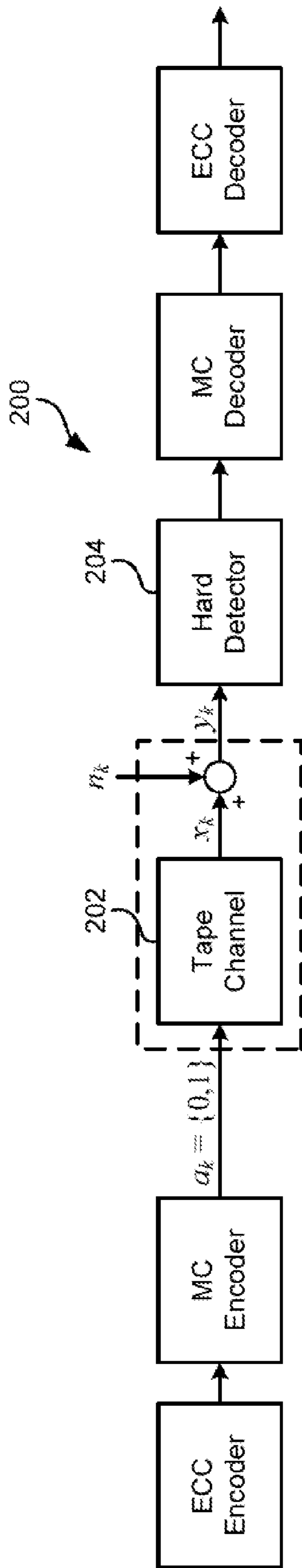
FIG. 2 (prior art)
