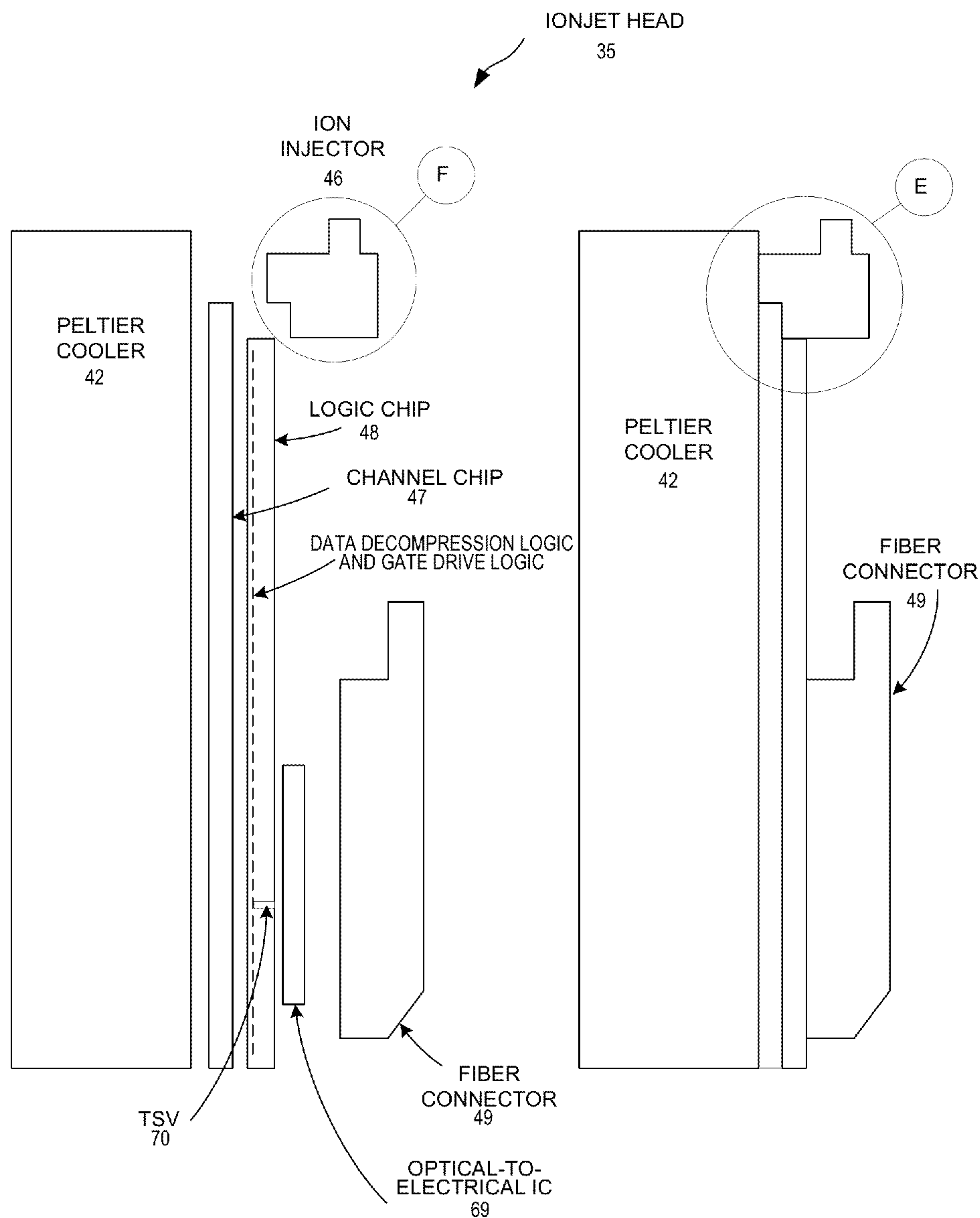
SECTION A-A IONJET HEAD SIDE VIEW SHOWN COMPRESSED FIG. 17
