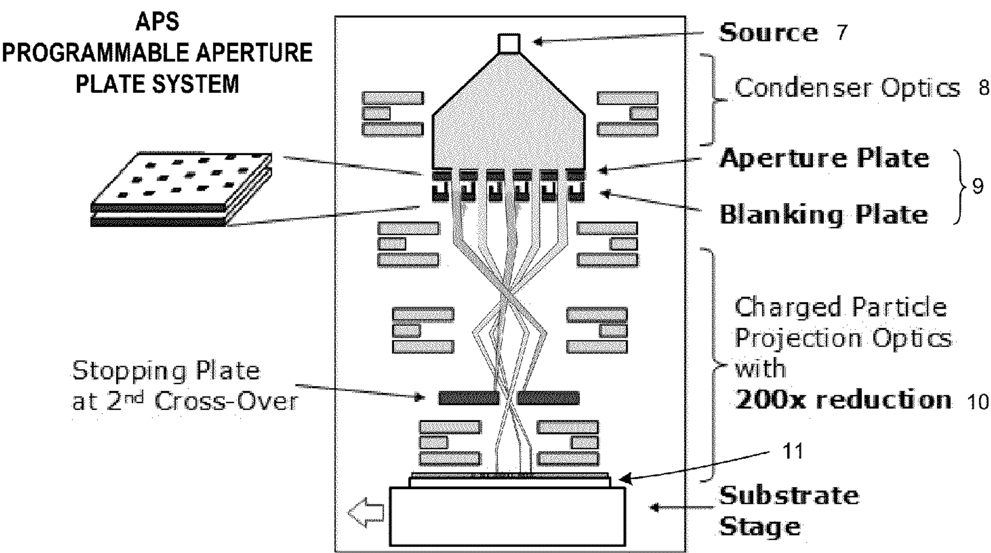
PROTON BEAM STEPPER
