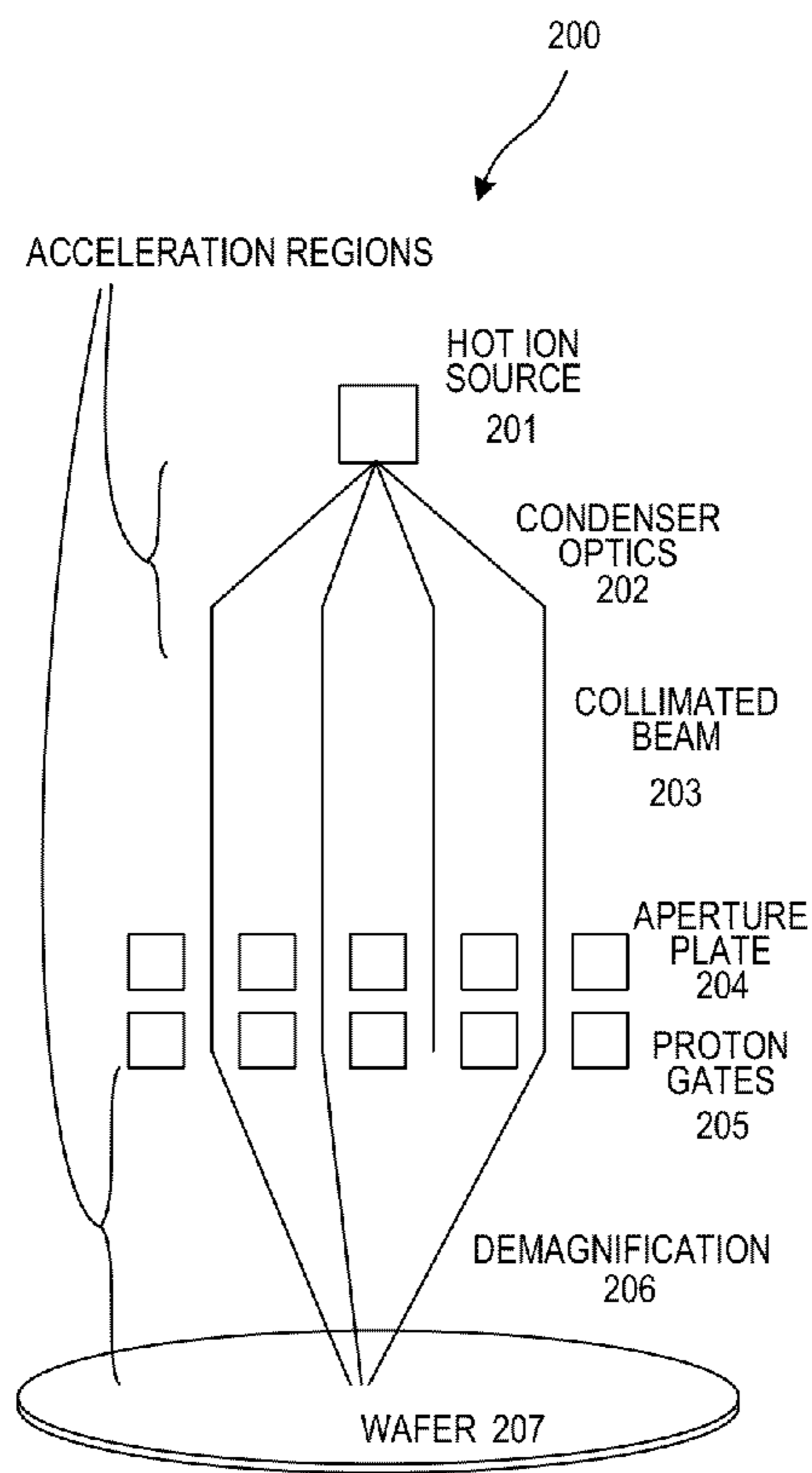
ION SOURCE AND COLLIMATOR (PRIOR ART) FIG. 36
