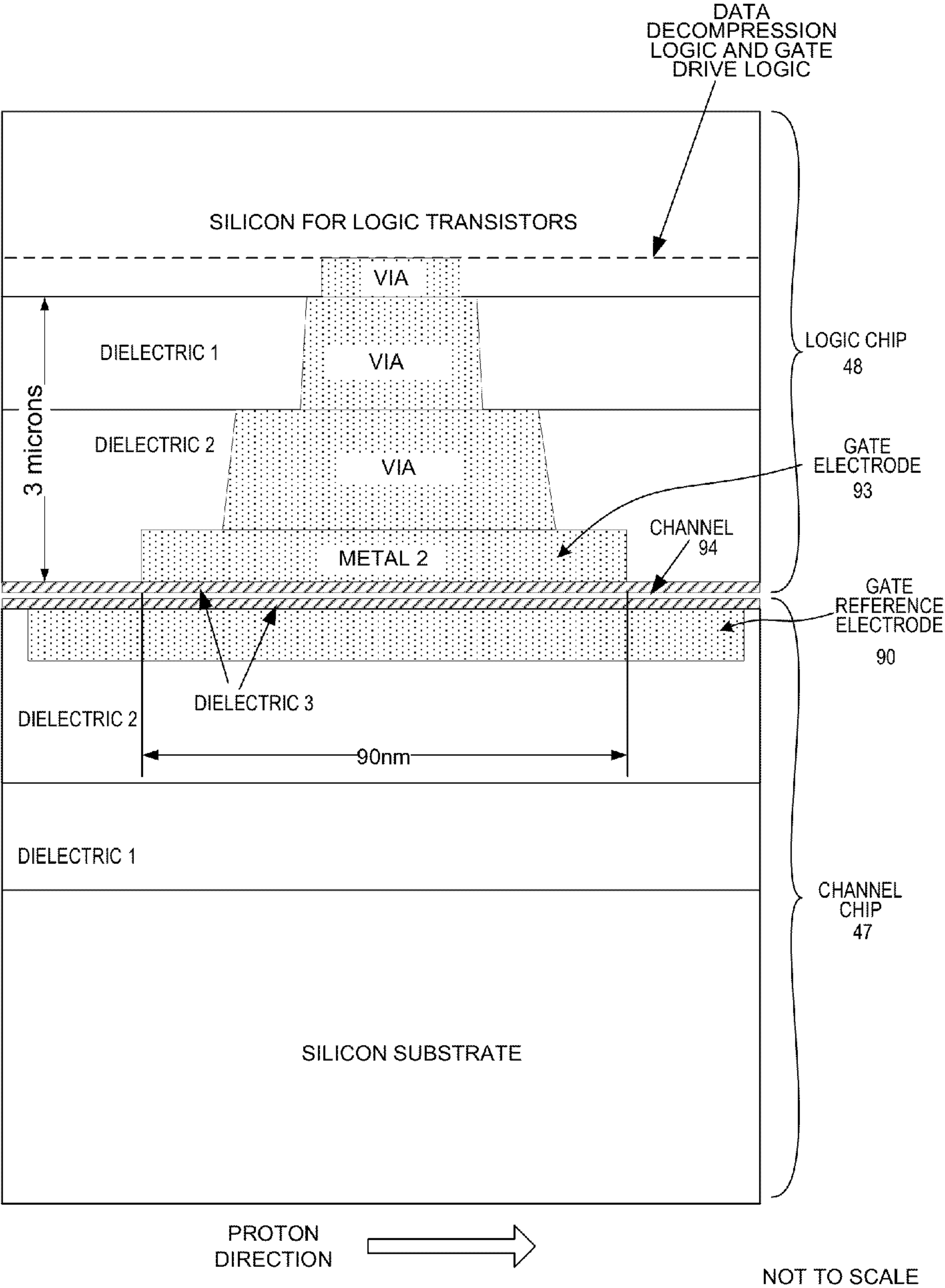
SECTION C-C – GATE CELL SIDE VIEW
