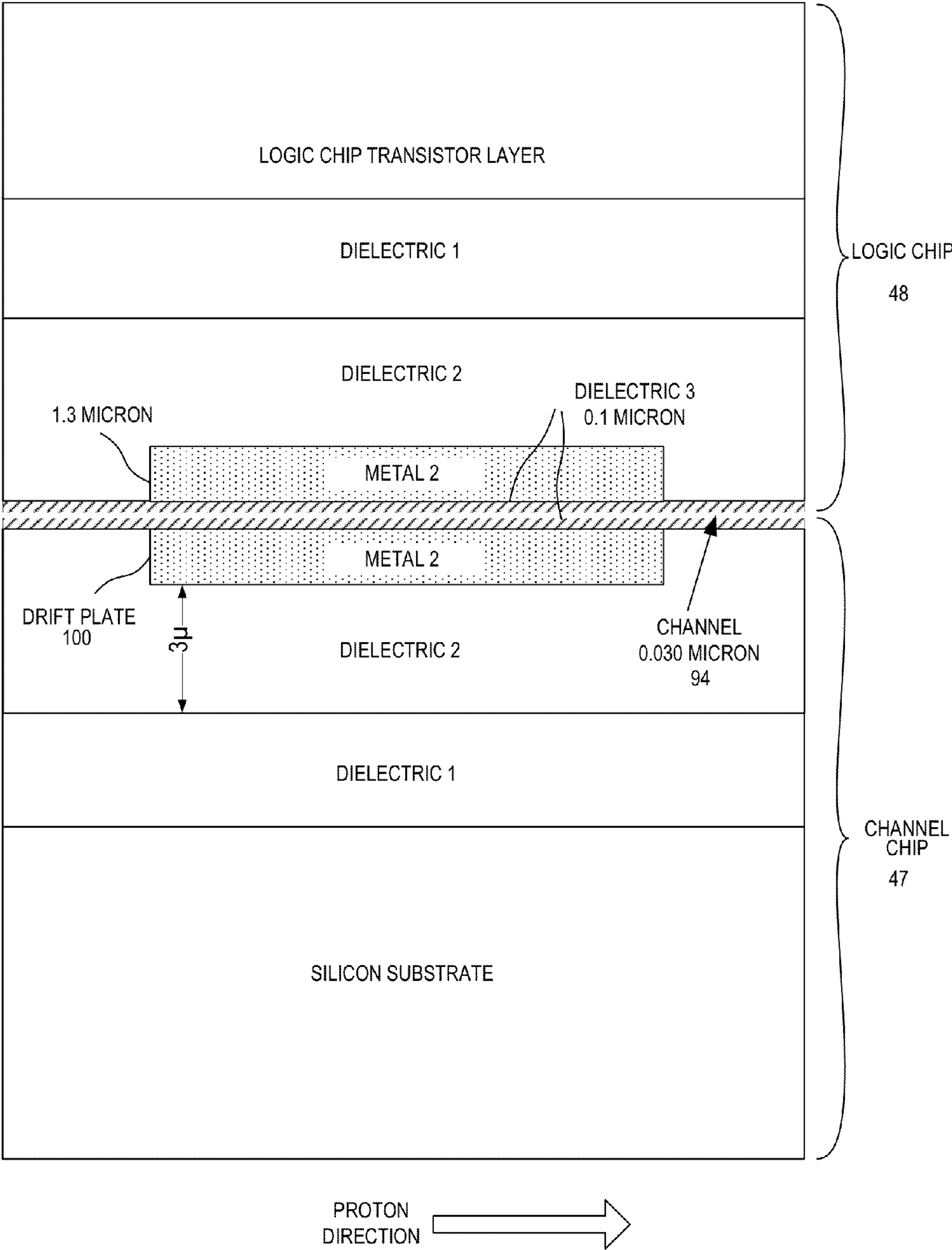
SECTION E-E – DRIFT CELL 2 SIDE VIEW FIG. 30
