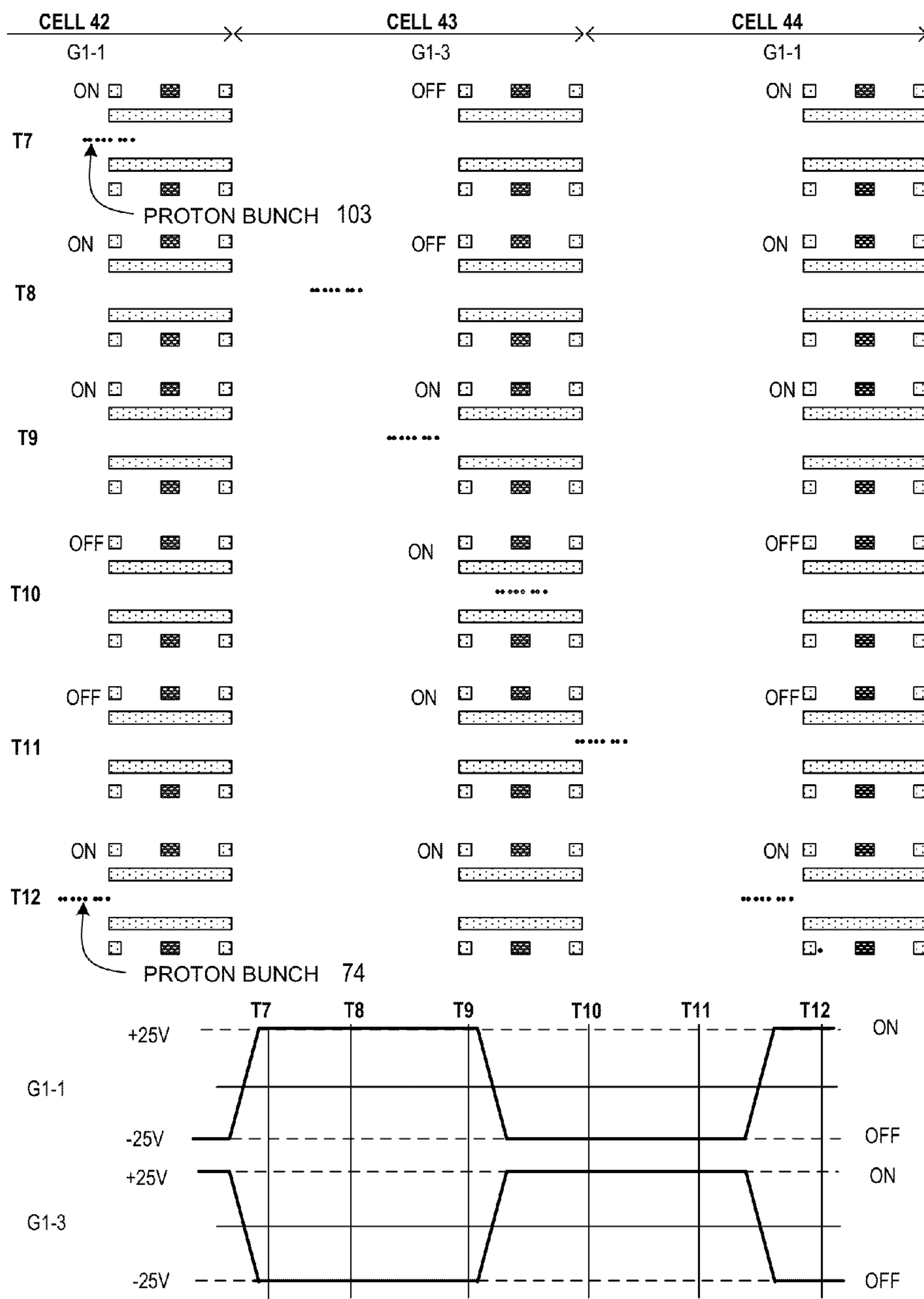
GATE PROTON TIMING SCHEME
