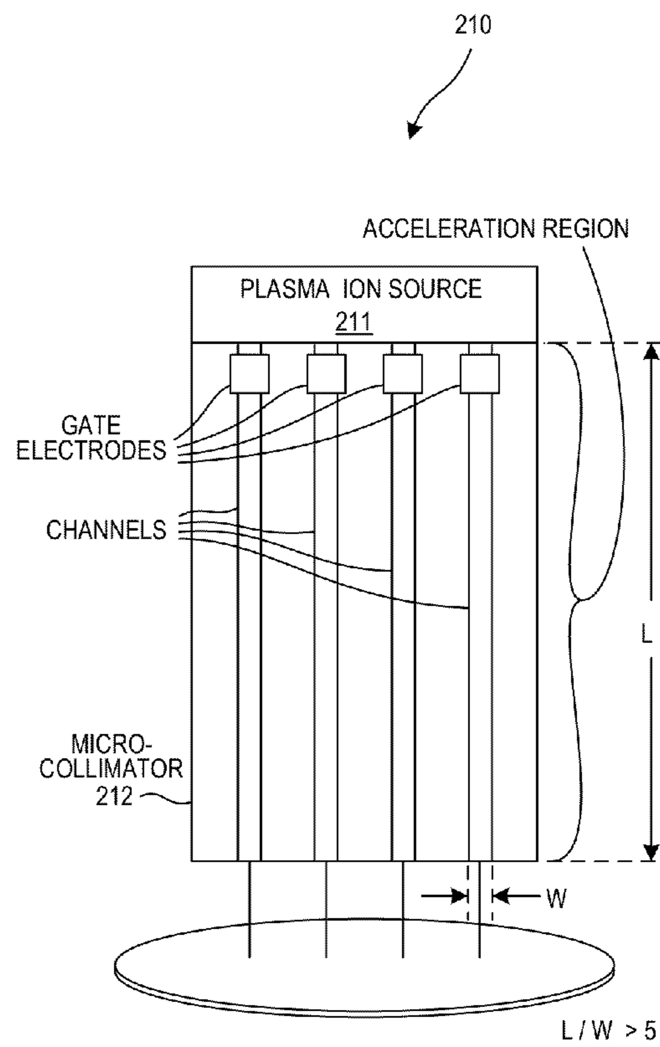
ACCELERATOR HAVING A MULTI-CHANNEL MICRO-COLLIMATOR FIG. 37
