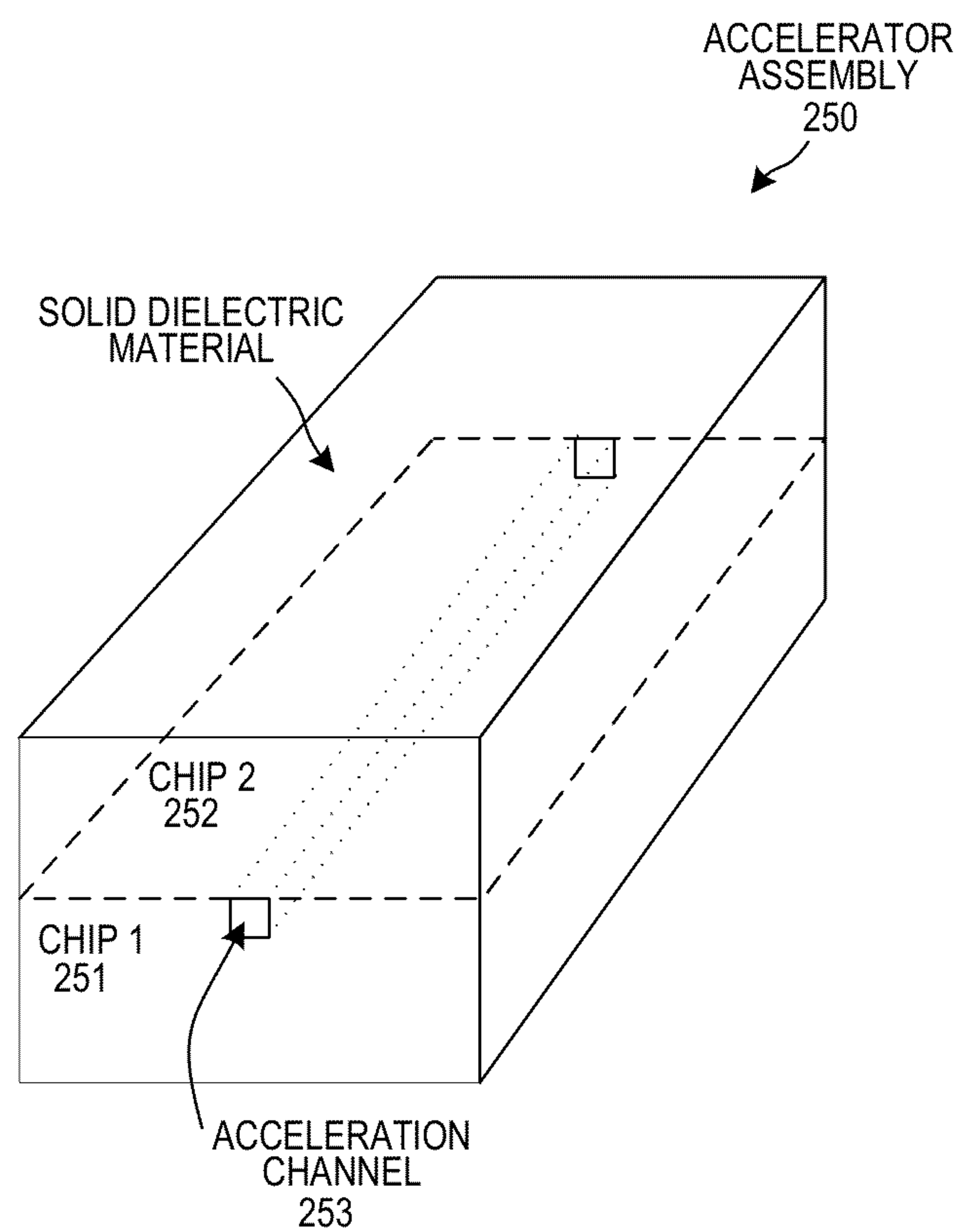
ACCELERTOR HAVING ACCELERATION CHANNELS FORMED BETWEEN COVALENTLY BONDED CHIPS
