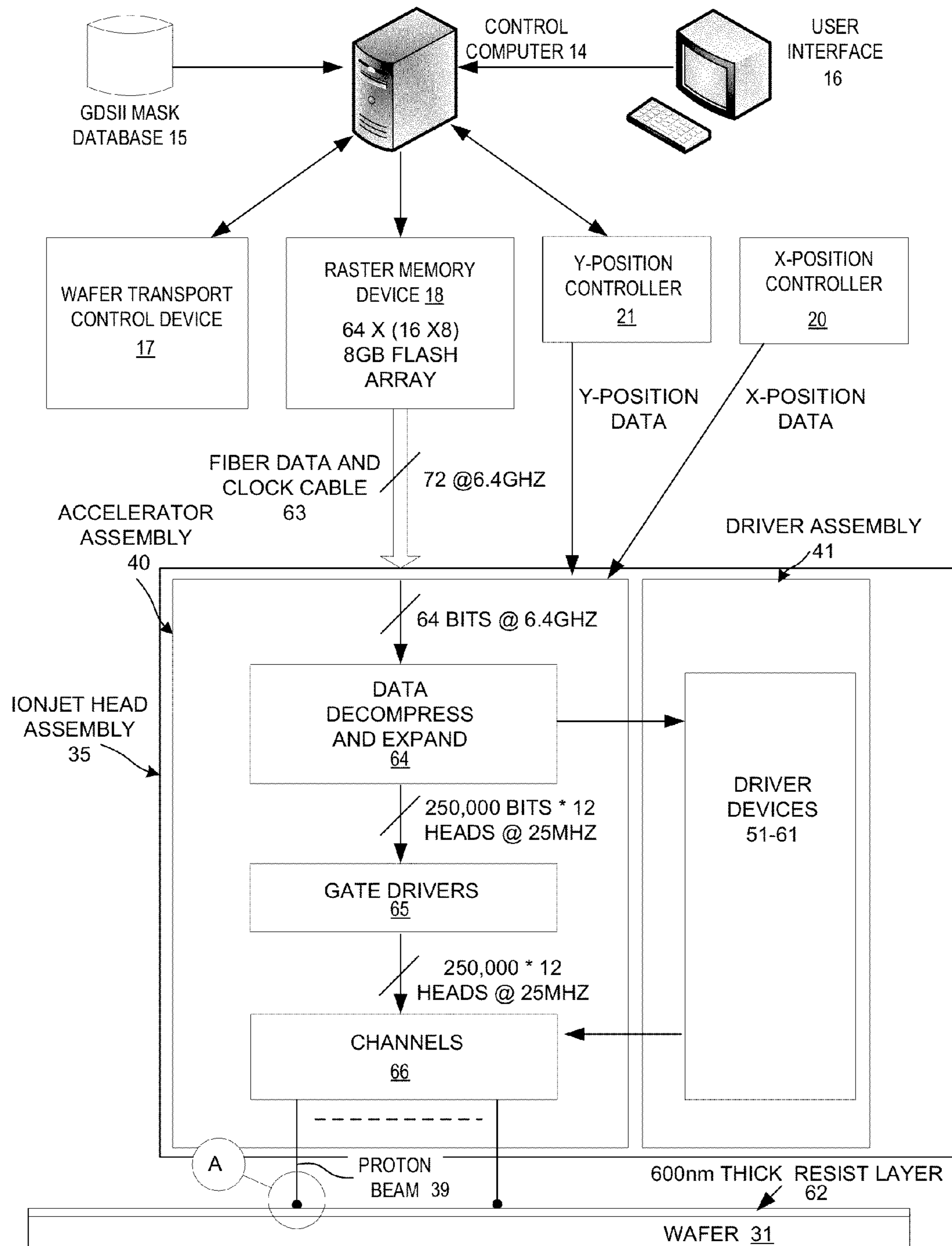
SYSTEM DATA PATH
