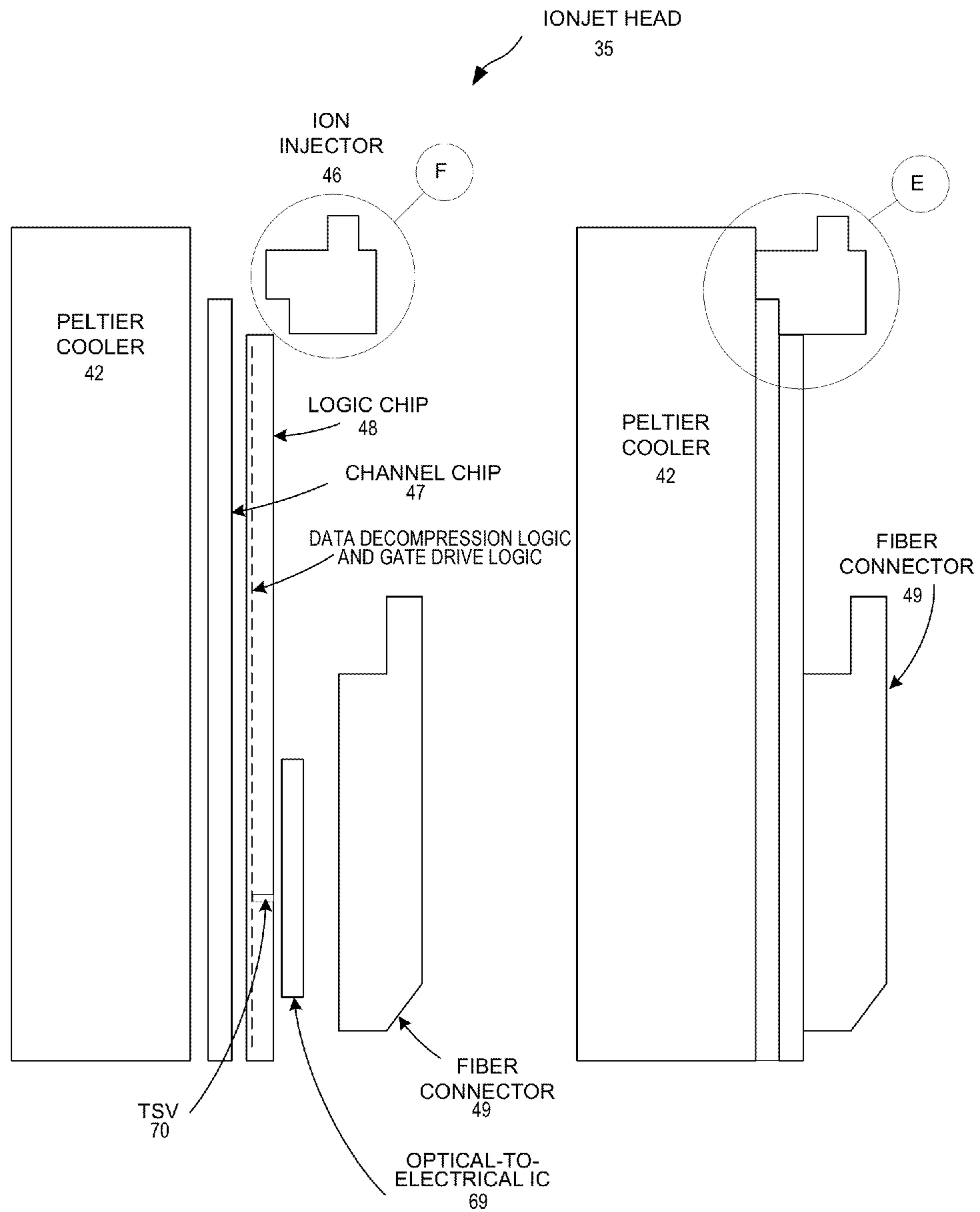
SECTION A-A IONJET HEAD SIDE VIEW
