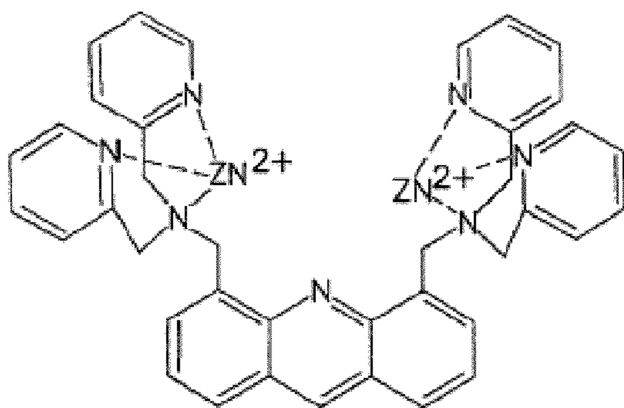
Compound 3
