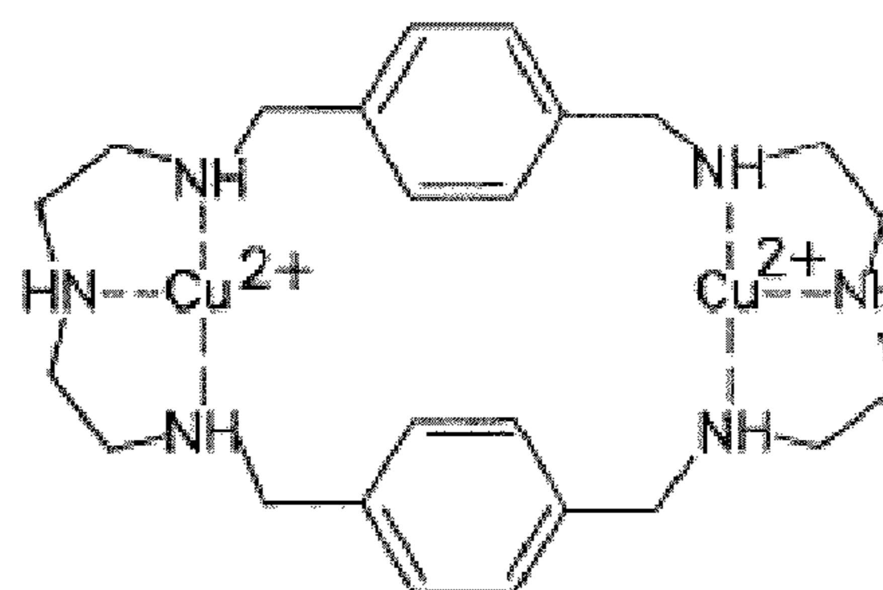
Compound 4
