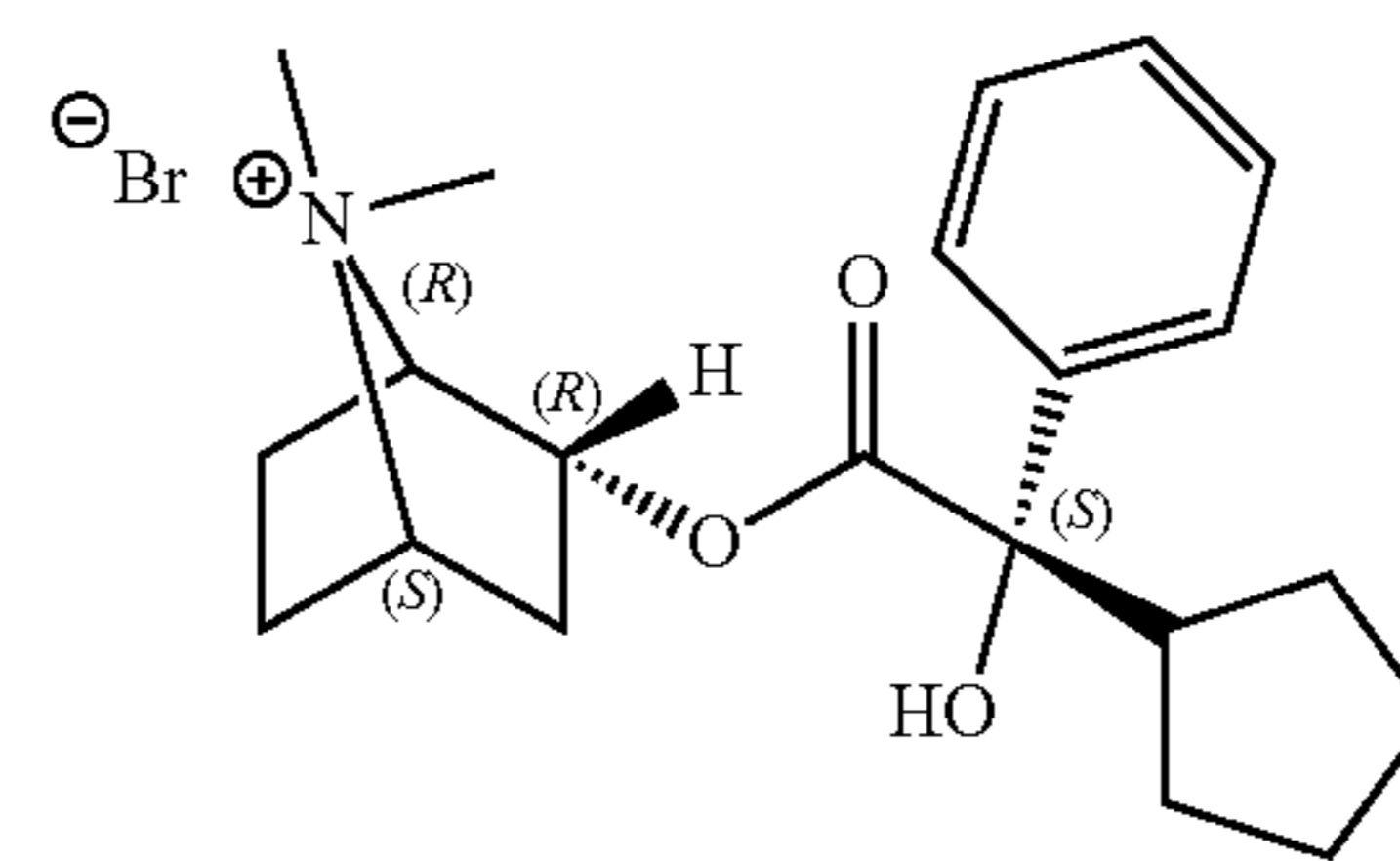
(1R,2R)-2-((S)-2'-cyclopentyl-2'-hydroxy-2'-phenylacetoxy)-7,7-dimethyl-7-azoniabicyclo[2.2.1]heptane bromide;
