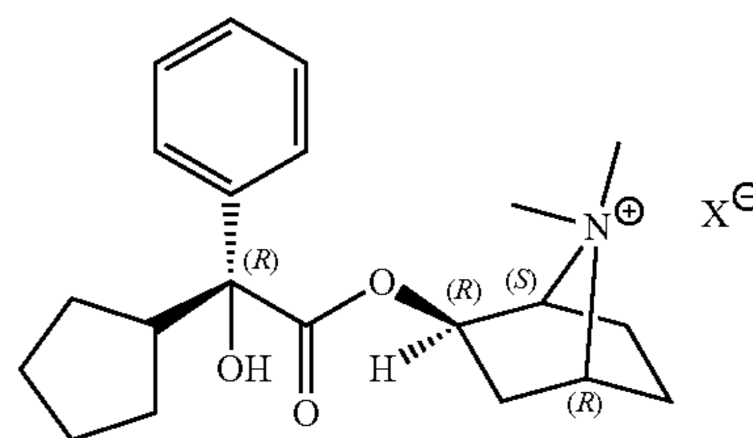
(1S,2R)-2-((R)-2'-cyclopentyl-2'-hydroxy 2'-phenylacetoxy)-7,7-dimethyl-7-azoniabicyclo[2.2.1]heptane with anion X^{\ominus} ;
