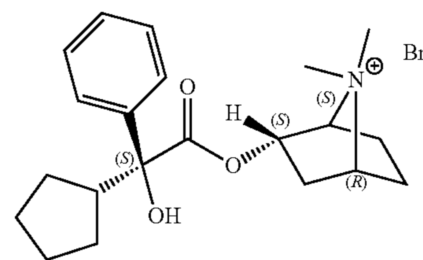
(1S,2S)-2-((S)-2'-cyclopentyl-2'-hydroxy-2'-phenylacetoxy)-7,7-dimethyl-7-azoniabicyclo[2.2.1]heptane bromide;
