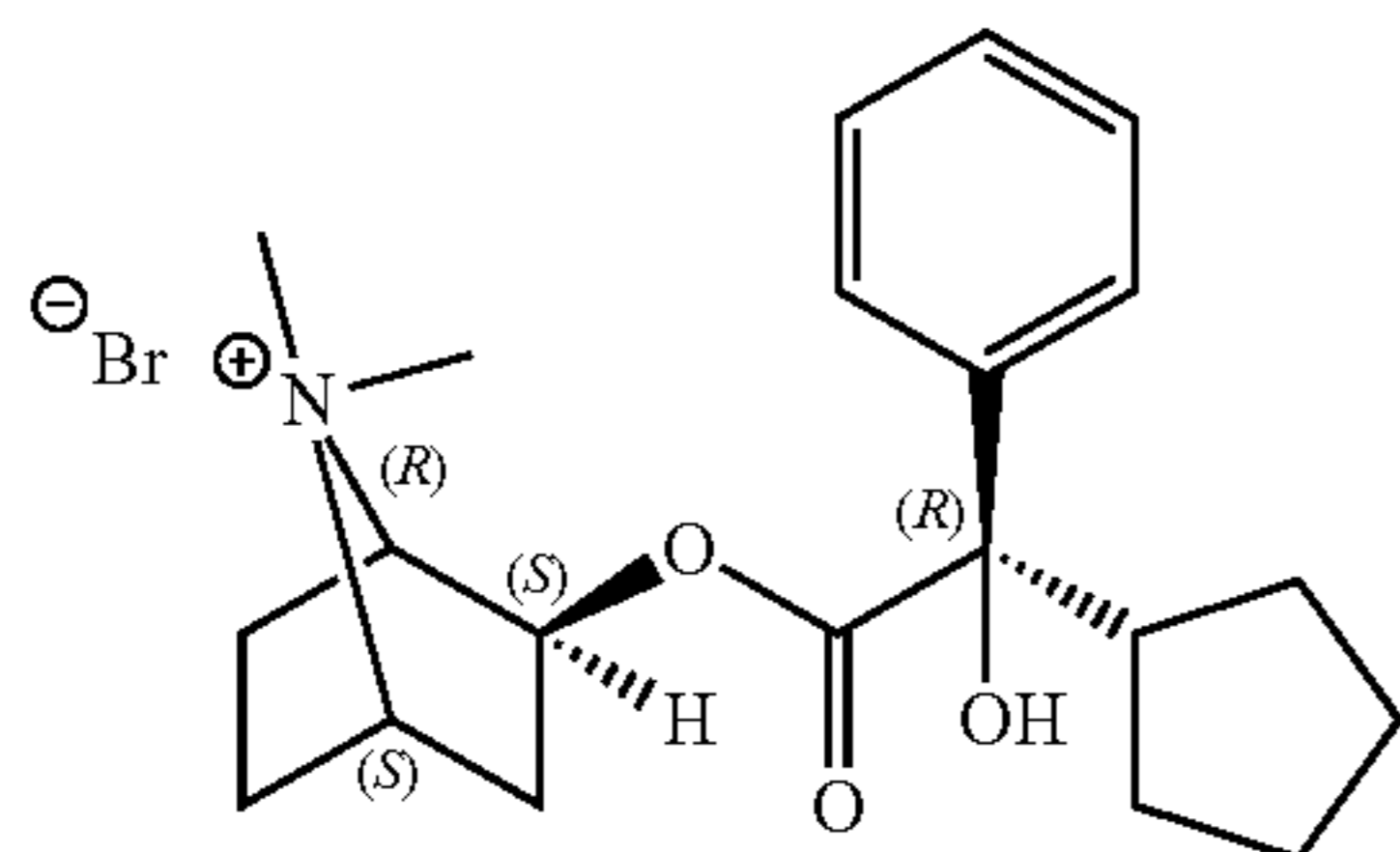
(1R,2S)-2-((R)-2'-cyclopentyl-2'-hydroxy-2'-phenylacetoxy)-7,7-dimethyl-7-azoniabicyclo[2.2.1]heptane bromide;
