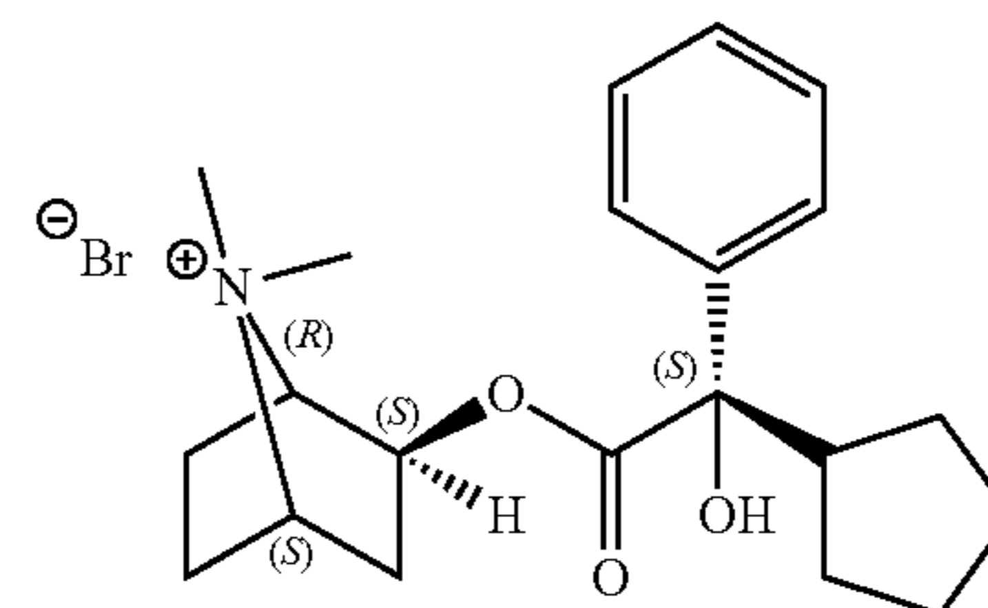
(1R,2S)-2-((S)-2'-cyclopentyl-2'-hydroxy-2'-phenylacetoxy)-7,7-dimethyl-7-azoniabicyclo[2.2.1]heptane bromide;
