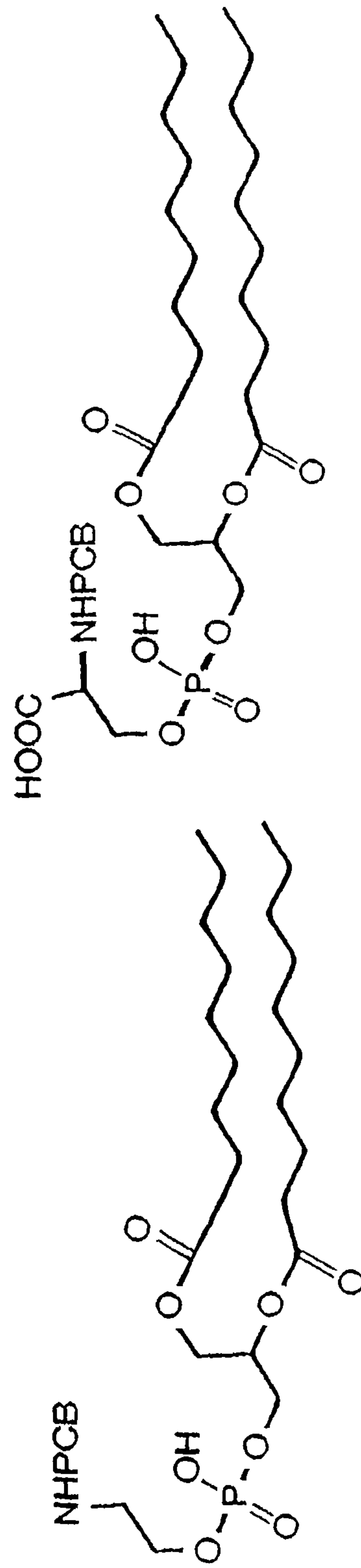
PCB-Phosphatidylethanoamine (PCB-PE)
