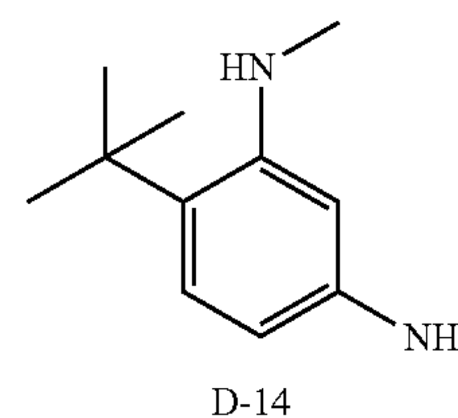
(3-Amino-4-tert-butyl-phenyl)-carbamic acid benzyl ester
