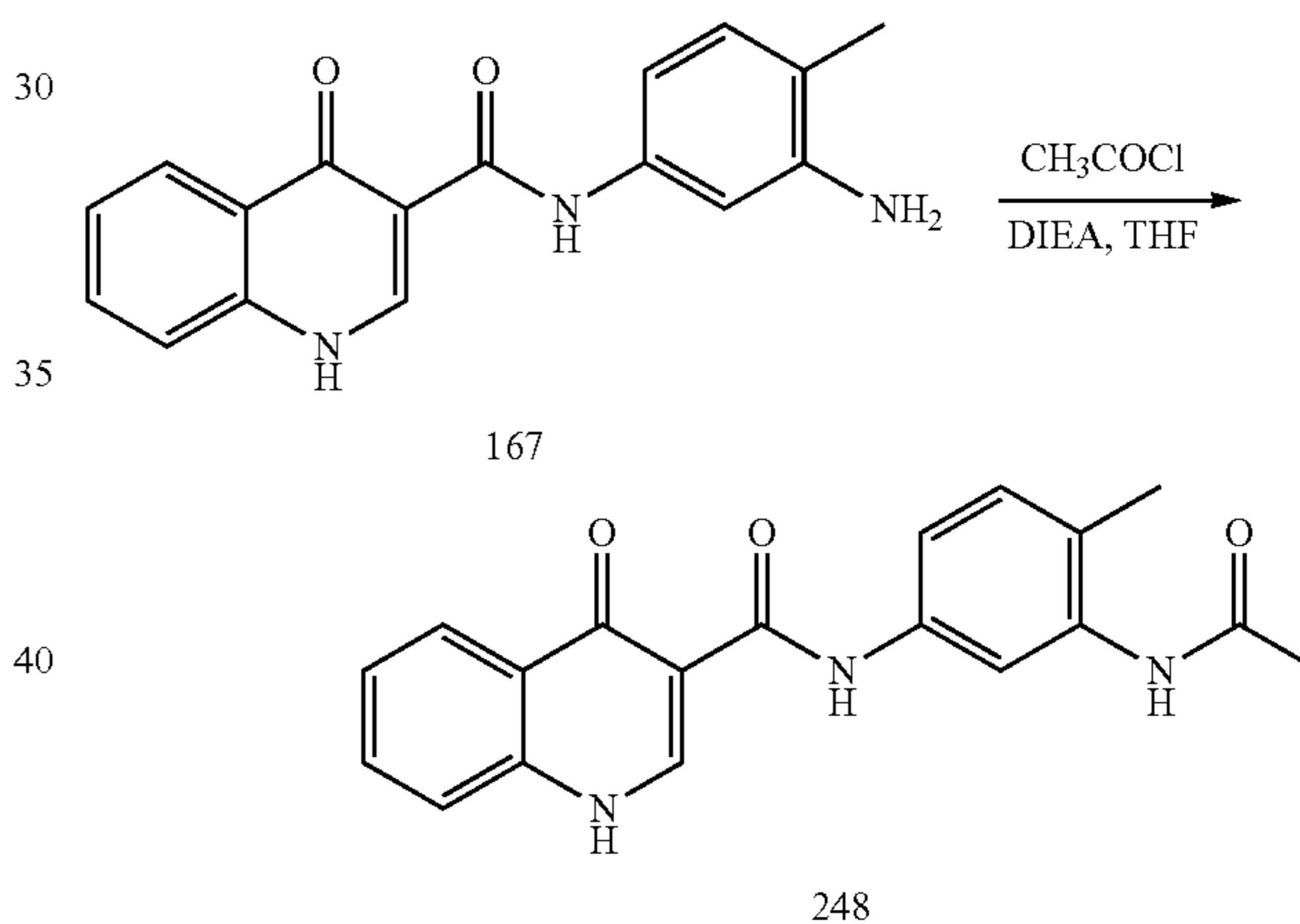
248; N-(3-Acetylamino-4-methyl-phenyl)-4-oxo-1H-quinoline-3-carboxamide
