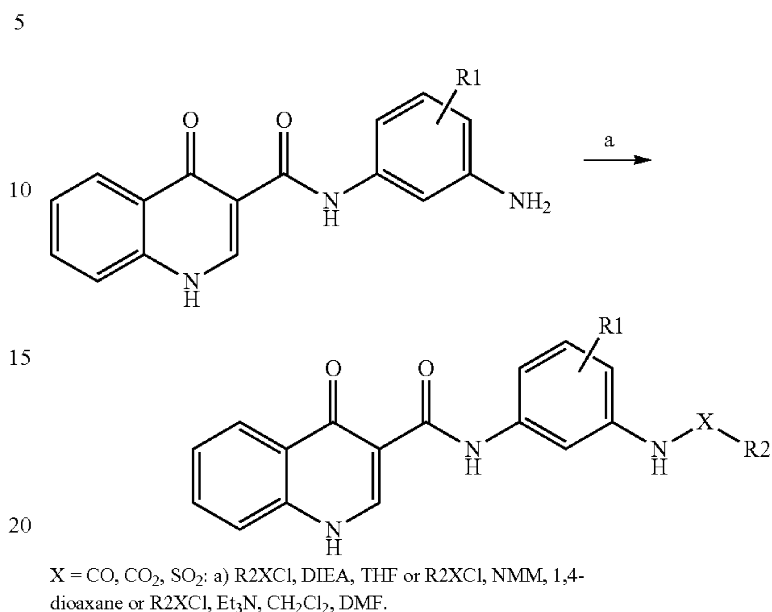
94; N-(5-Amino-2-methyl-phenyl)-4-oxo-1H-quinoline-3-carboxamide
