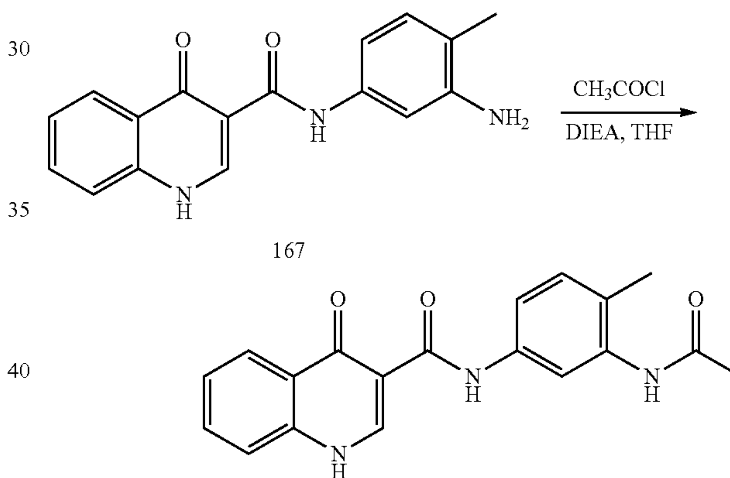
248; N-(3-Acetylamino-4-methyl-phenyl)-4-oxo-1H-quinoline-3-carboxamide
