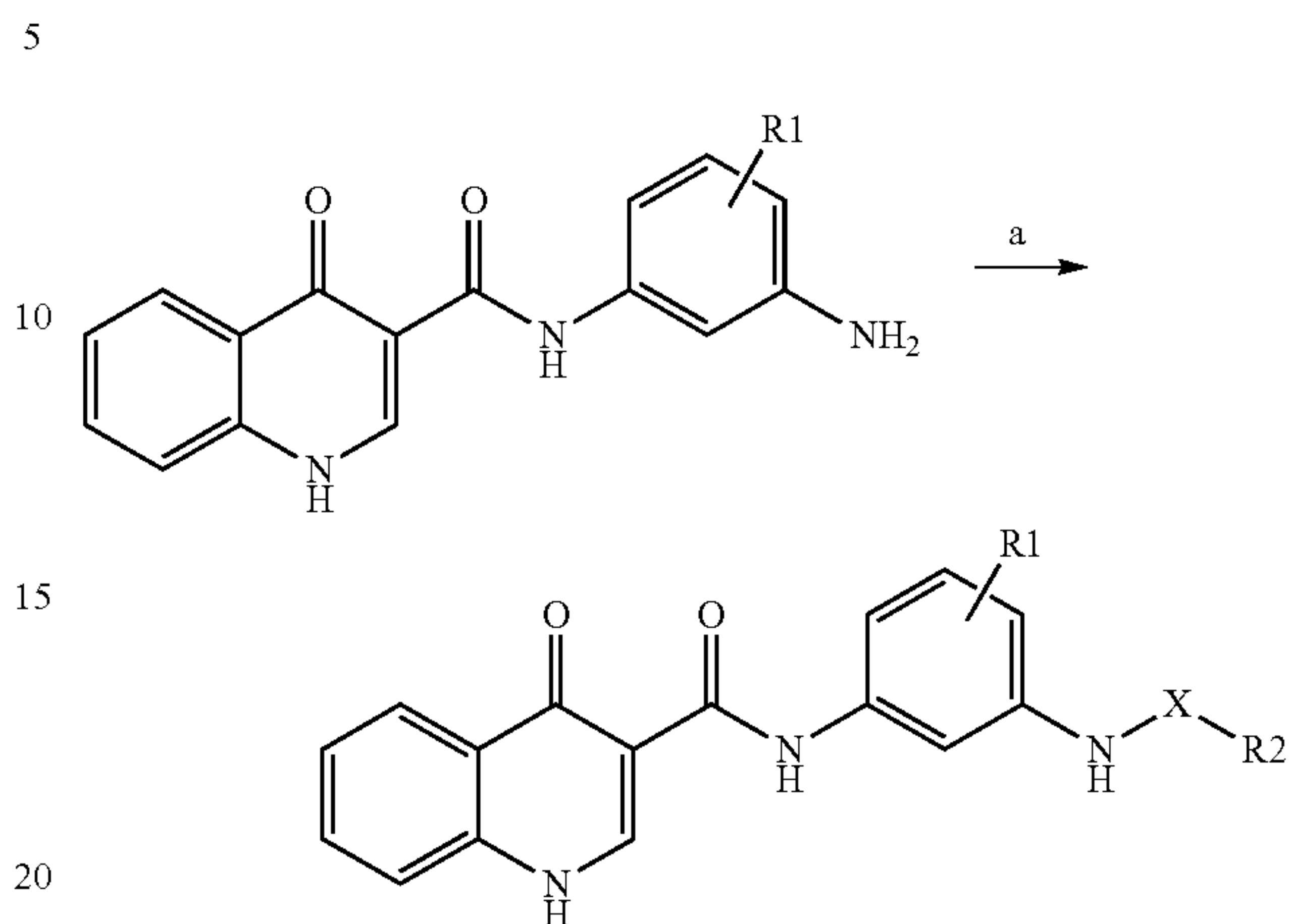
94; N-(5-Amino-2-methyl-phenyl)-4-oxo-1H-quinoline-3-carboxamide
