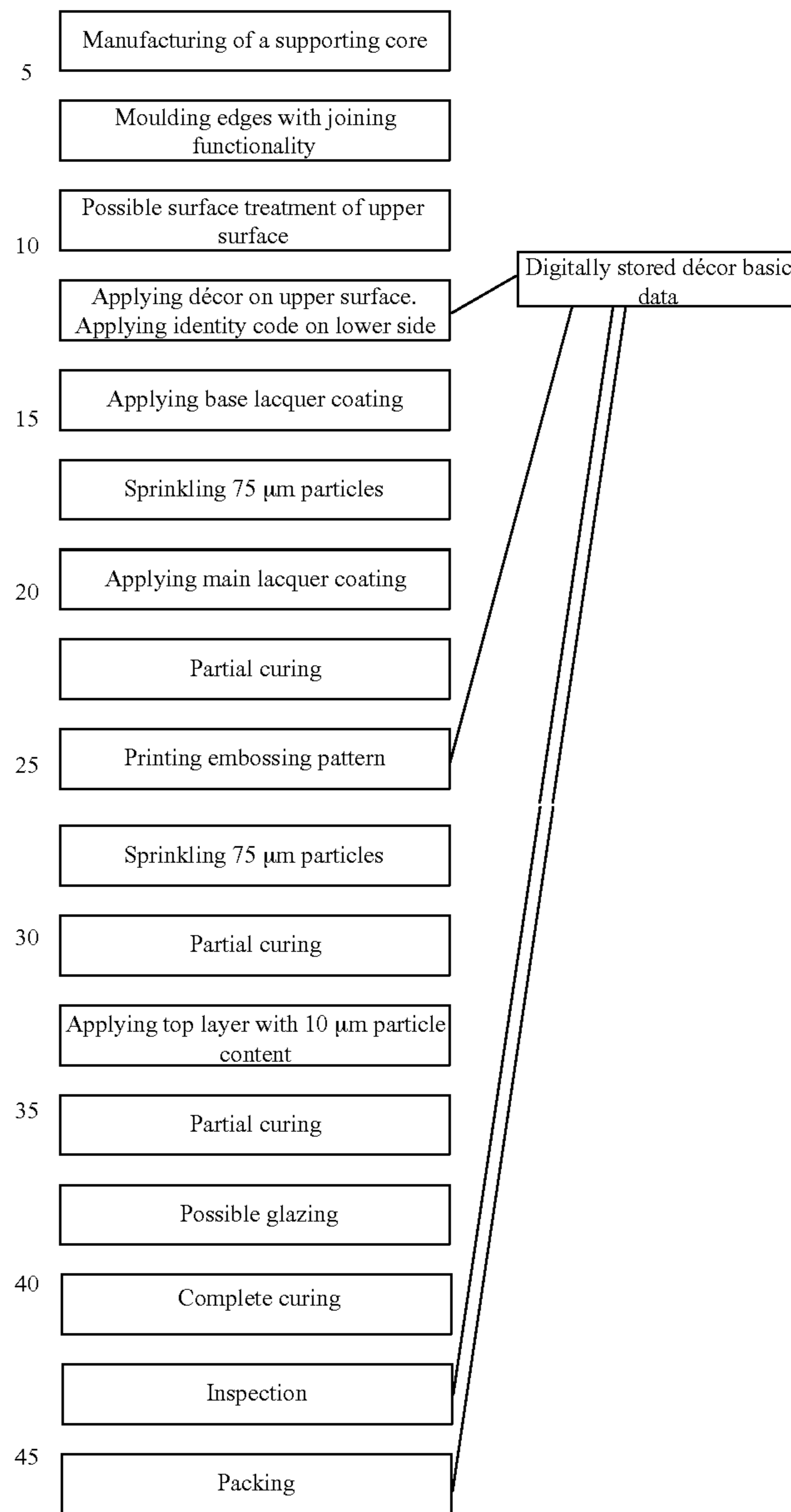
Process scheme 1.
