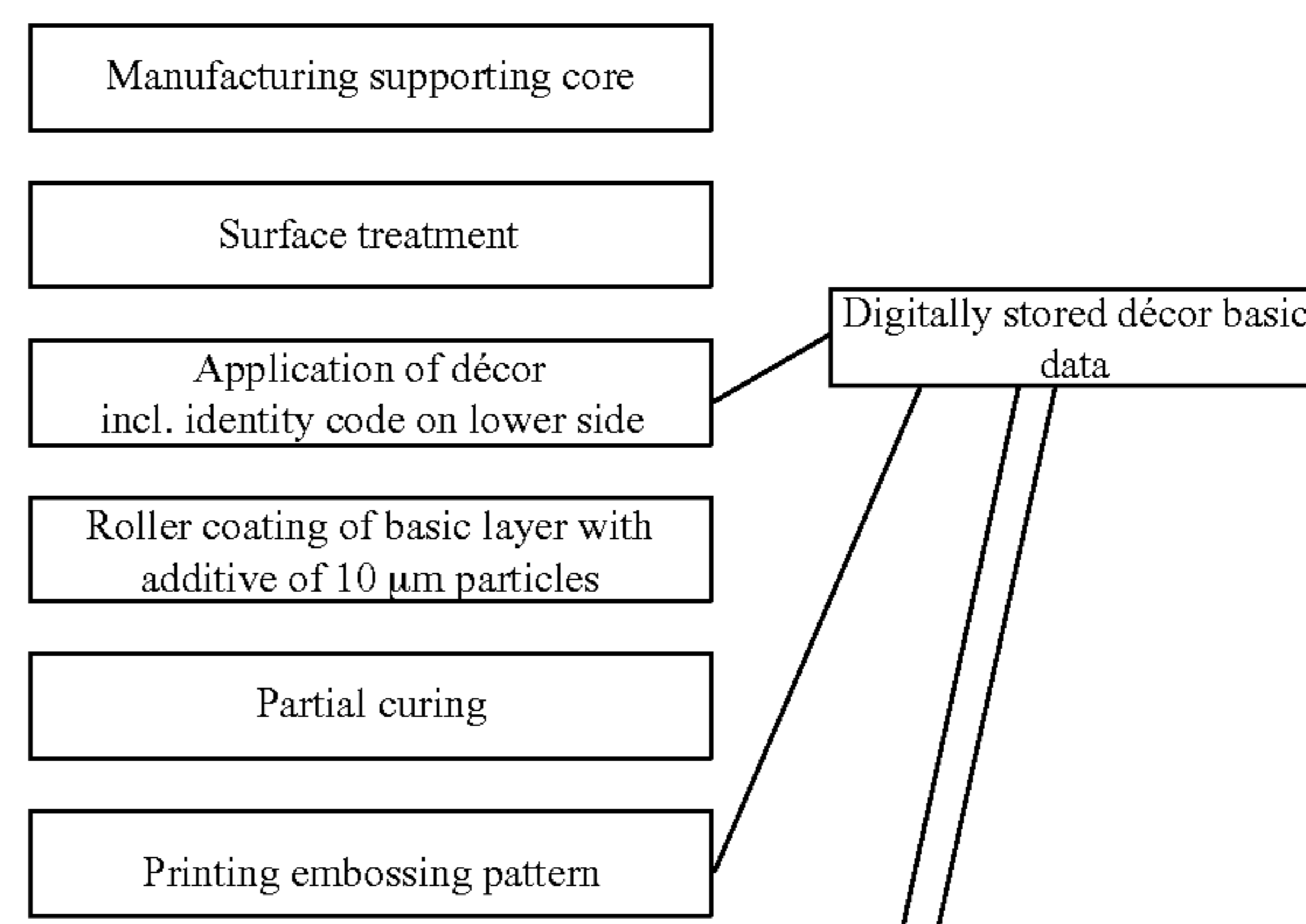
Process scheme 2
