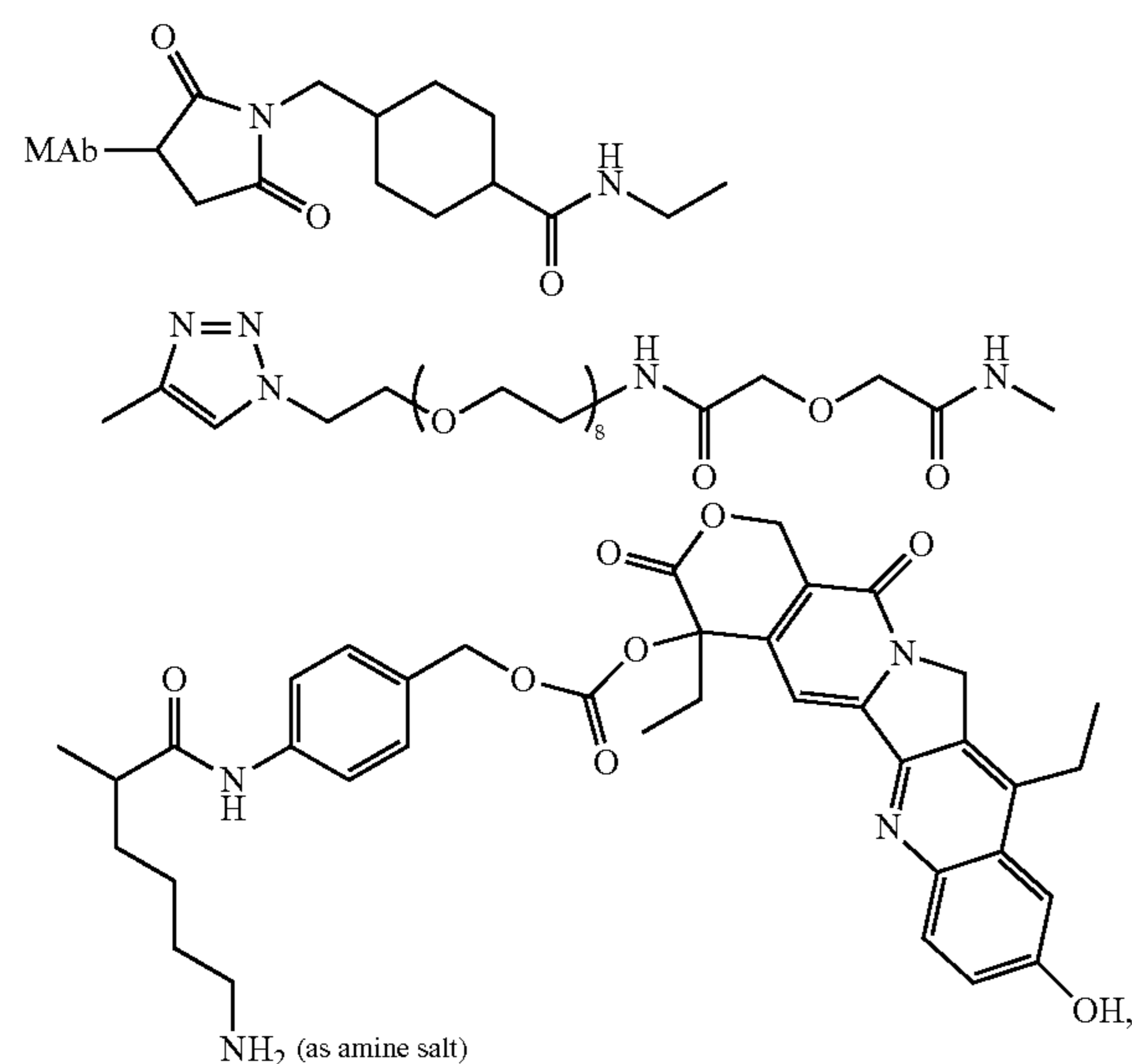
MAb-CL2A-SN-38
