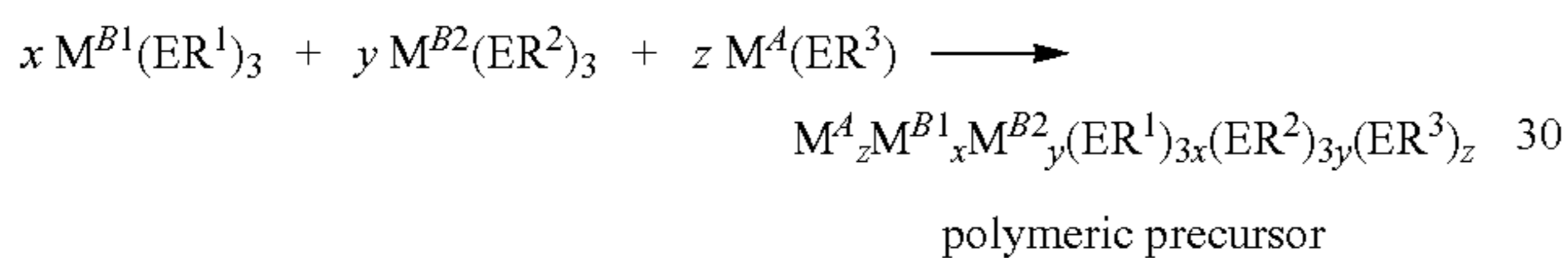
REACTION SCHEME 12:
