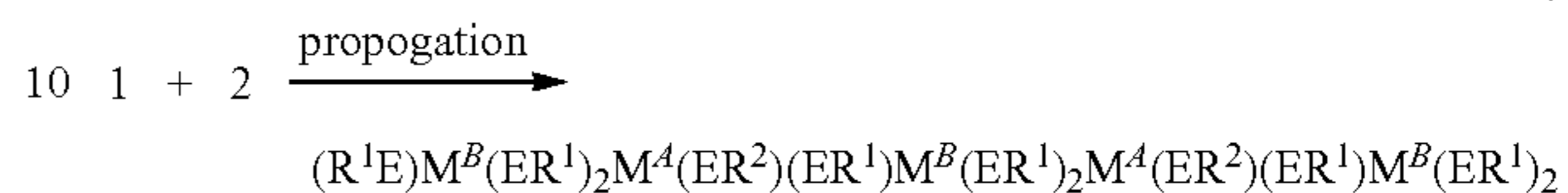
REACTION SCHEME 4:
