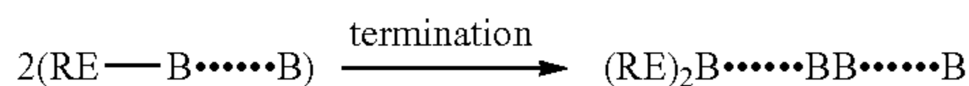
REACTION SCHEME 6:
