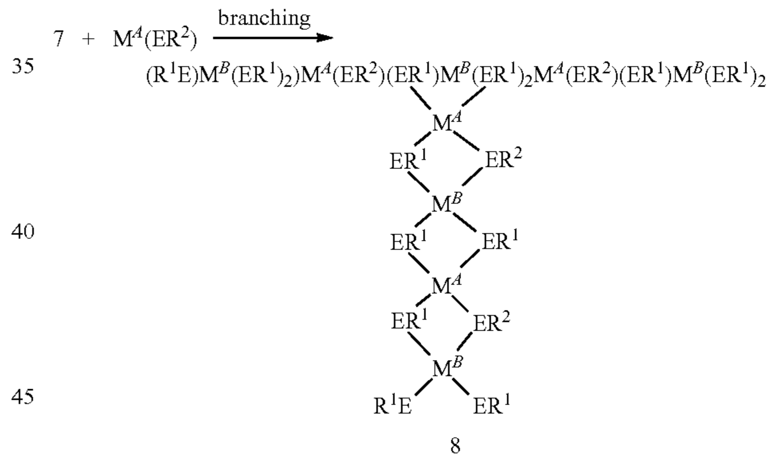
REACTION SCHEME 5:
