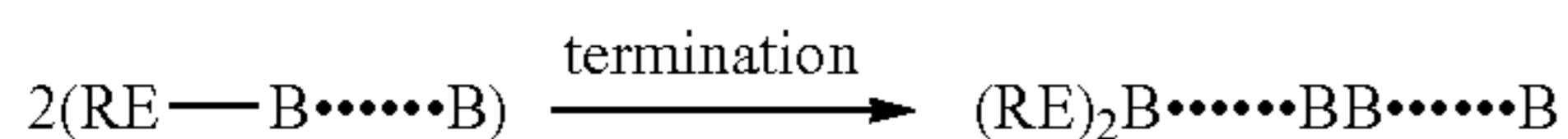
REACTION SCHEME 6:
