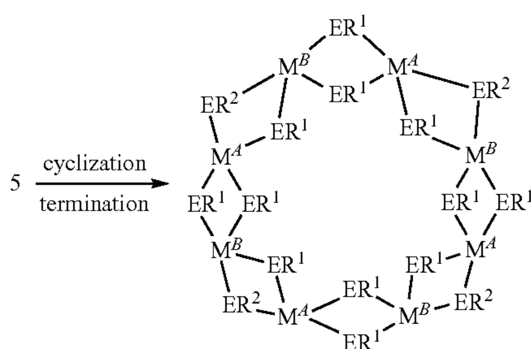
REACTION 7:
