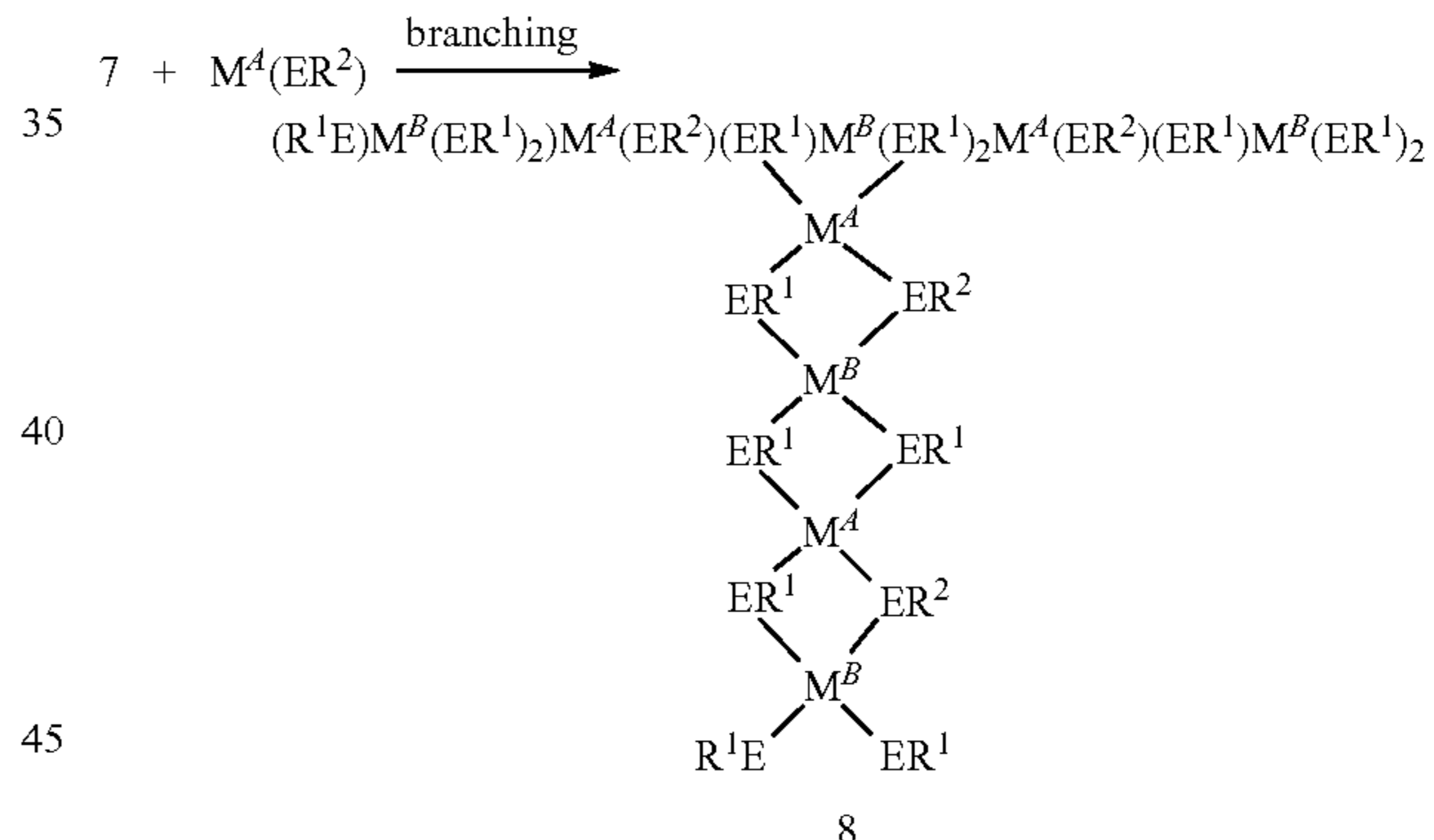
REACTION SCHEME 5:
