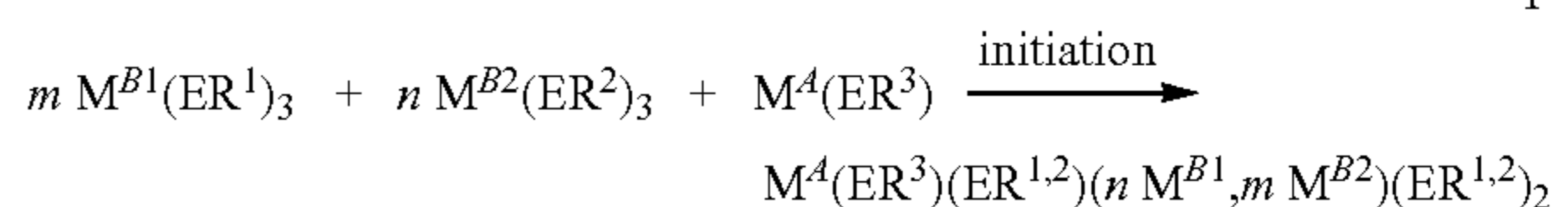
REACTION SCHEME 8:
