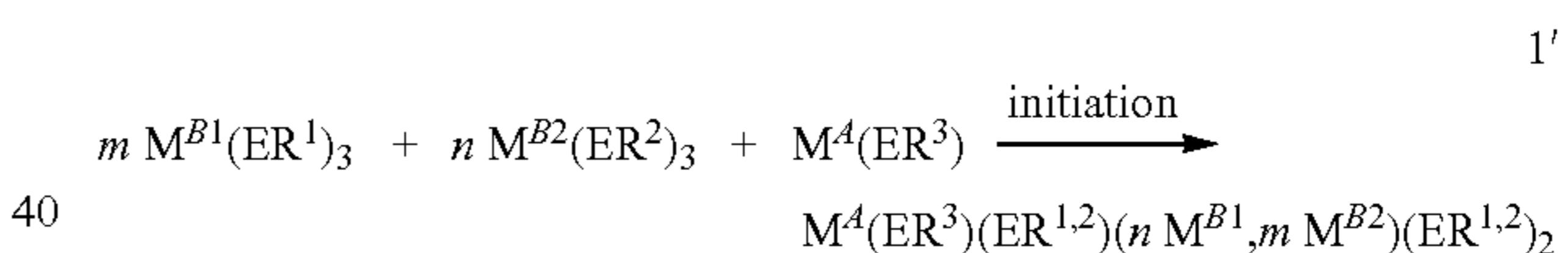
REACTION SCHEME 8:
