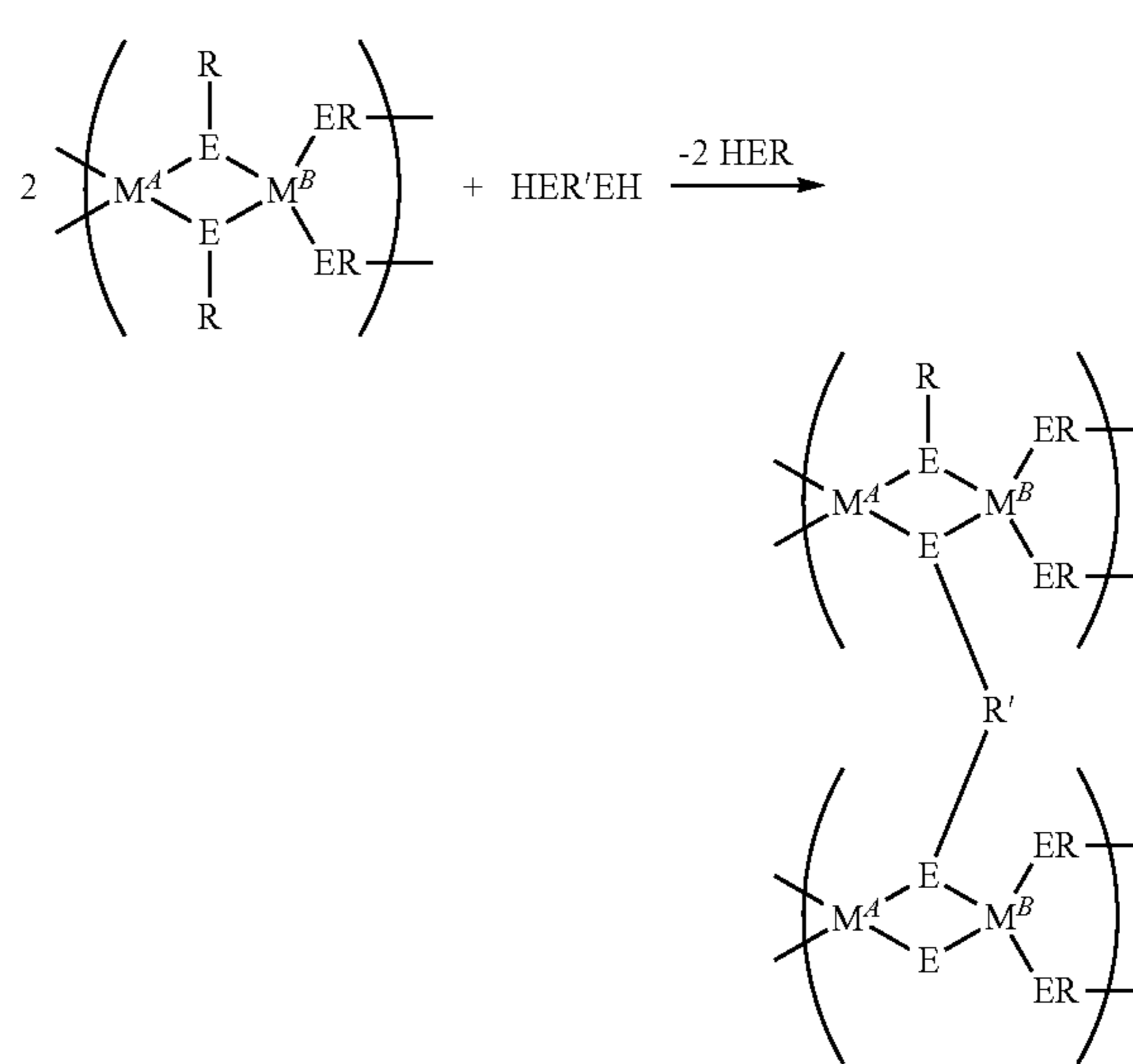
REACTION SCHEME 14
