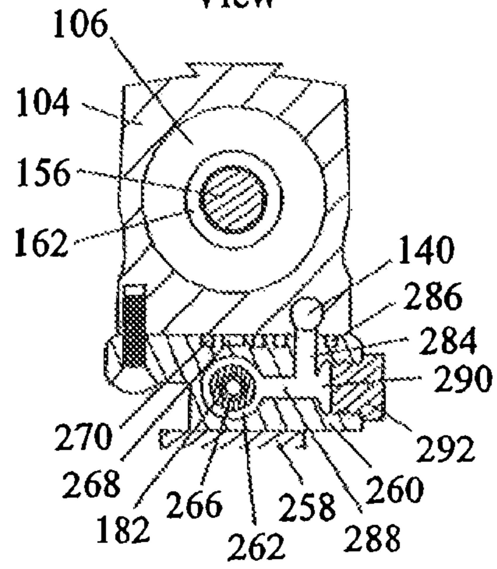
Rear Sectional View
