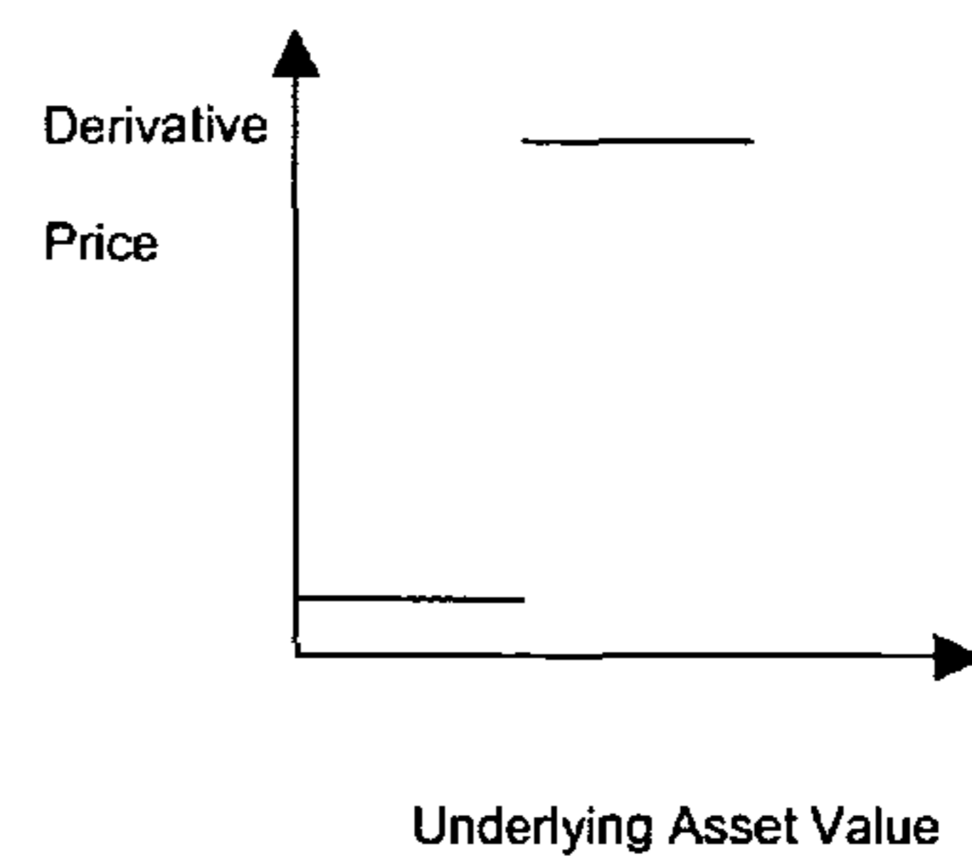
Figure 3. European Style Binary Option
