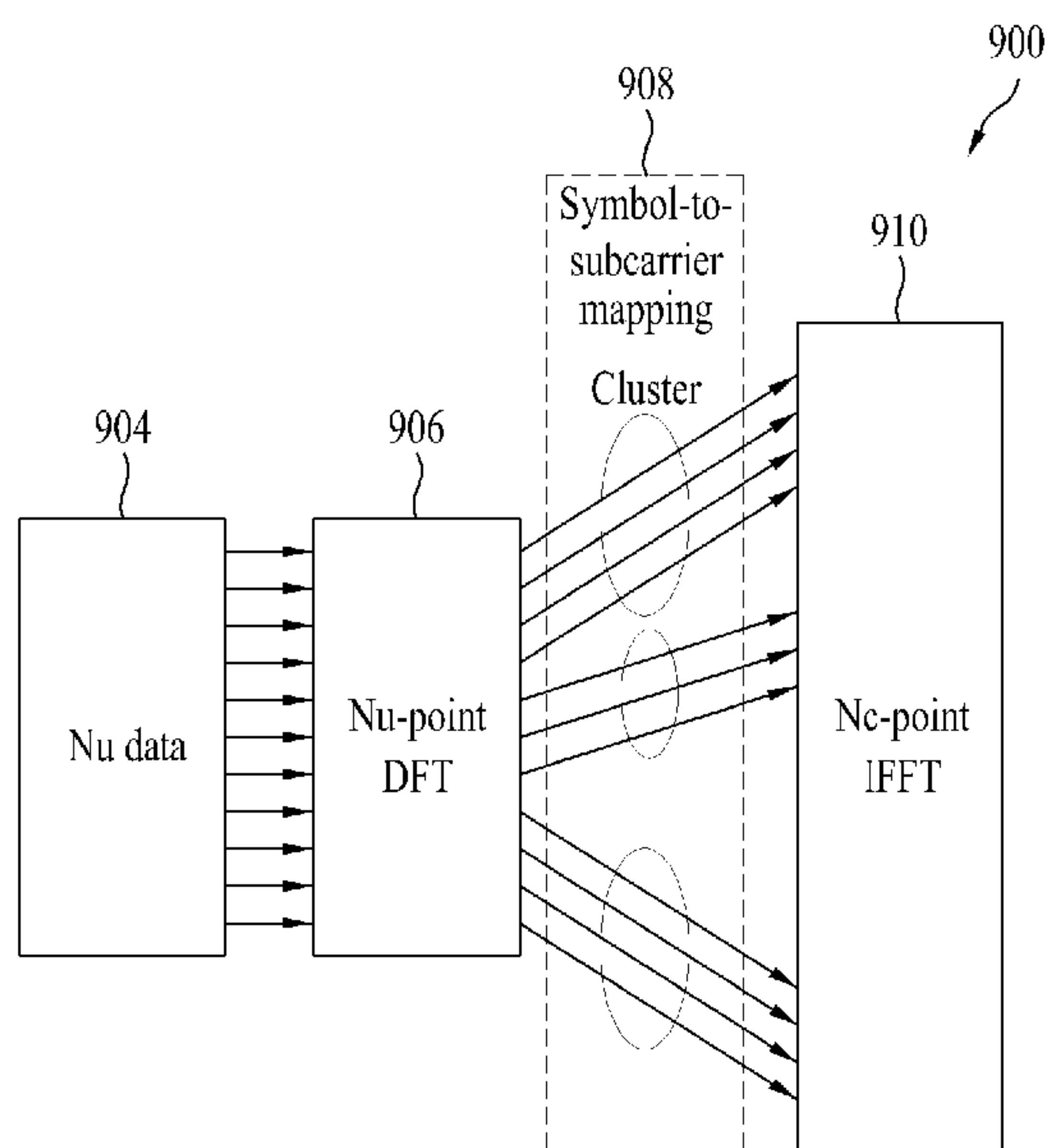
Clustered DFT-s-OFDMA
