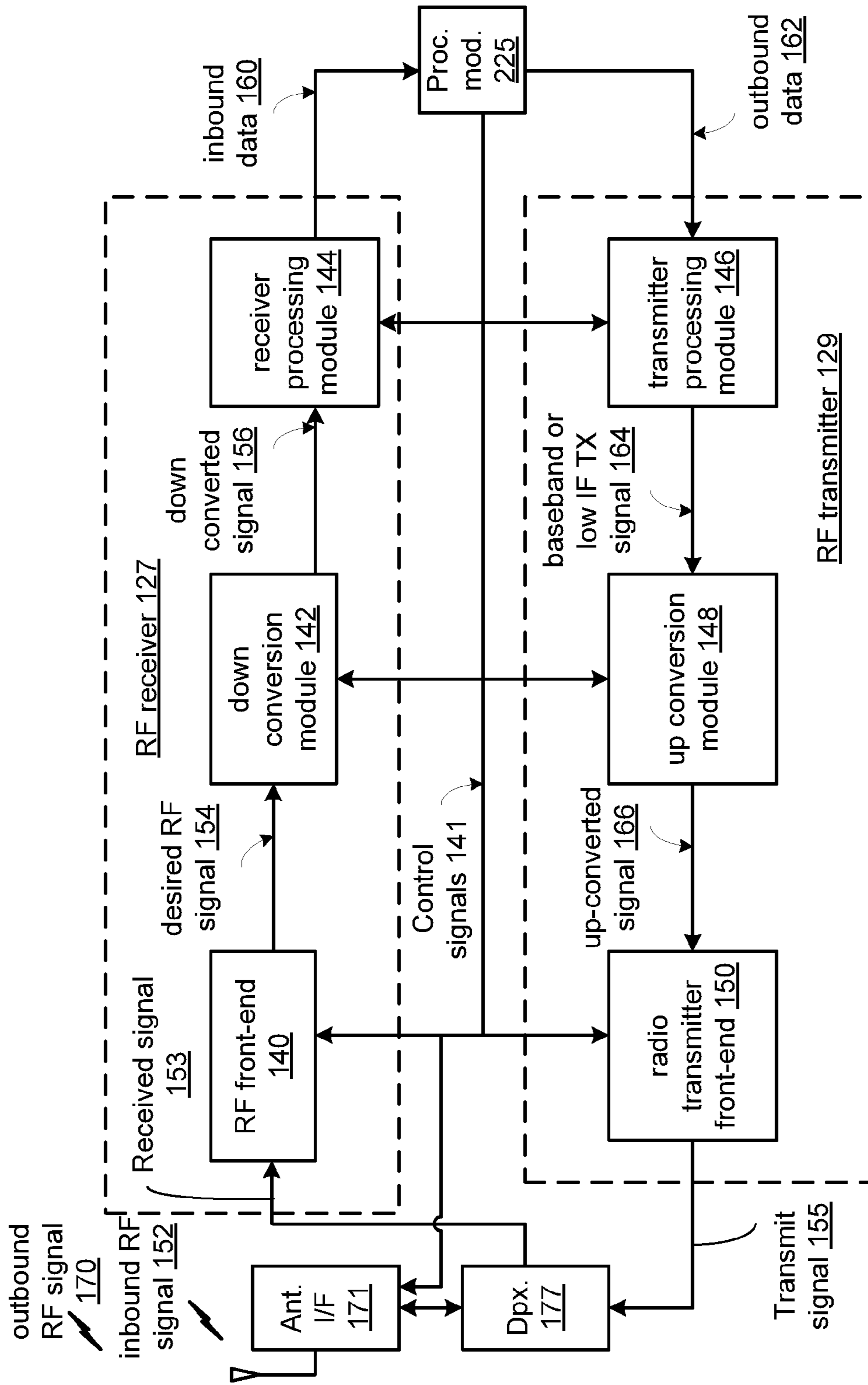
RF transceiver 123
