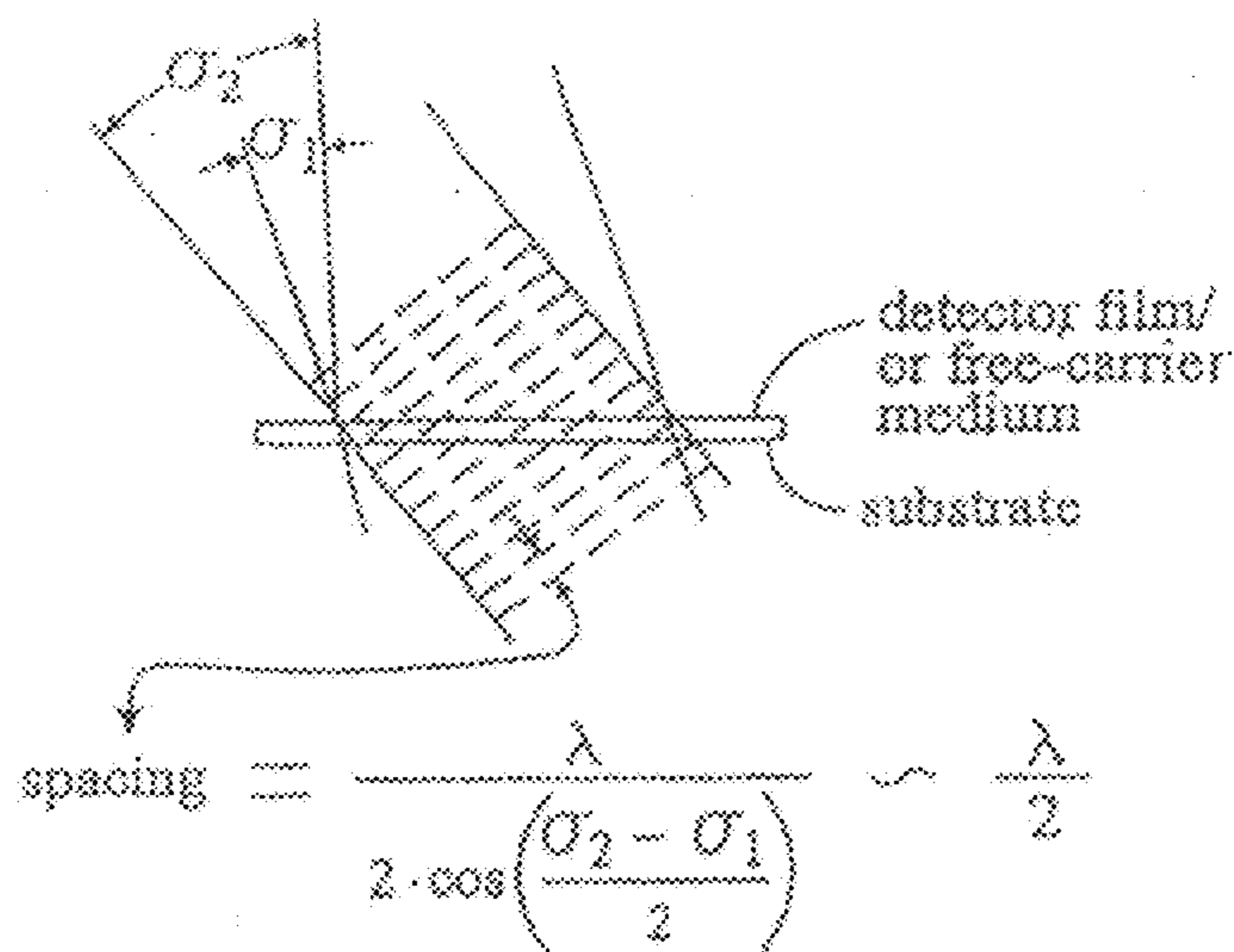
Double Sided Method (Holography/Interferogram)
