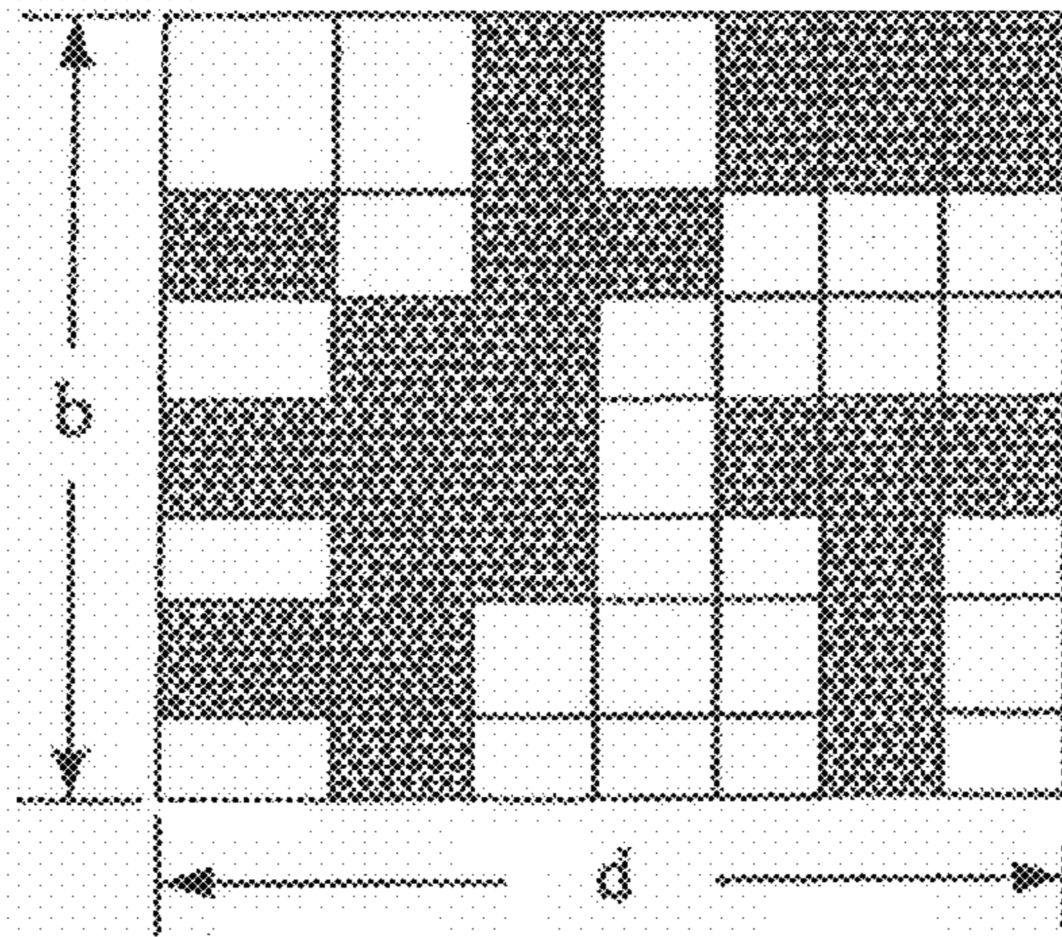
Illustration showing arrangement of generalized binary detour-phase IR Hologram
