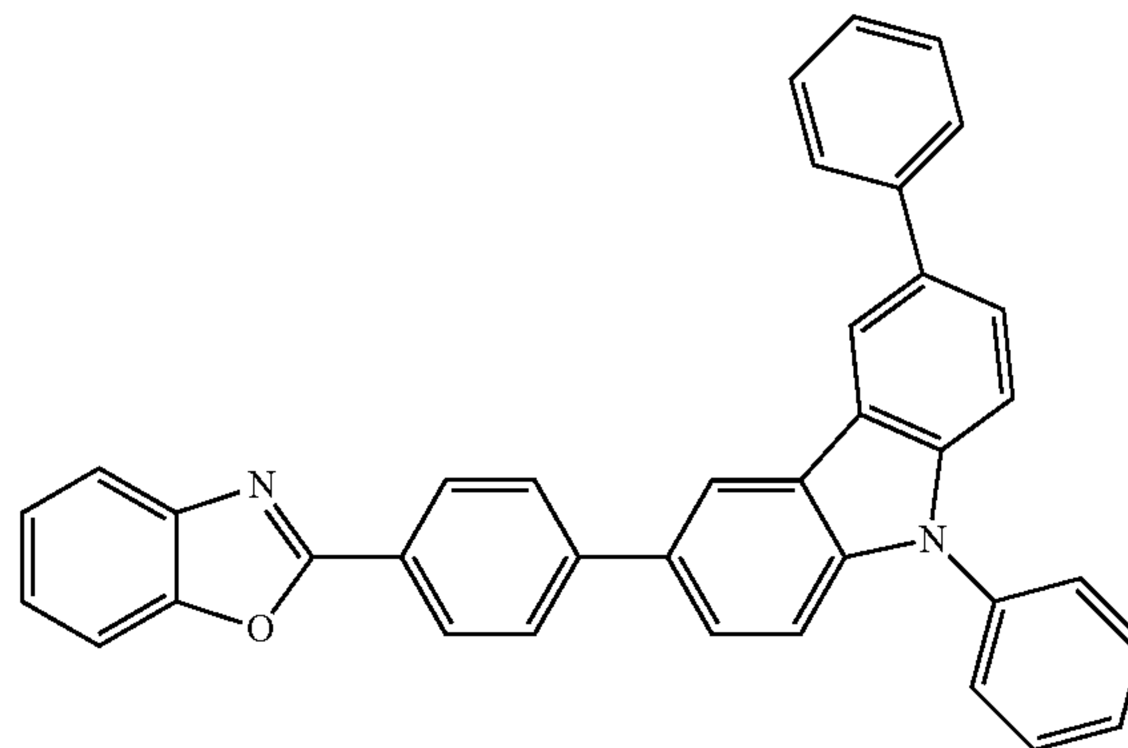
Synthesis of 3-[4-(Benzoxazol-2-yl)phenyl]-6,9-diphenyl-9H-carbazole
