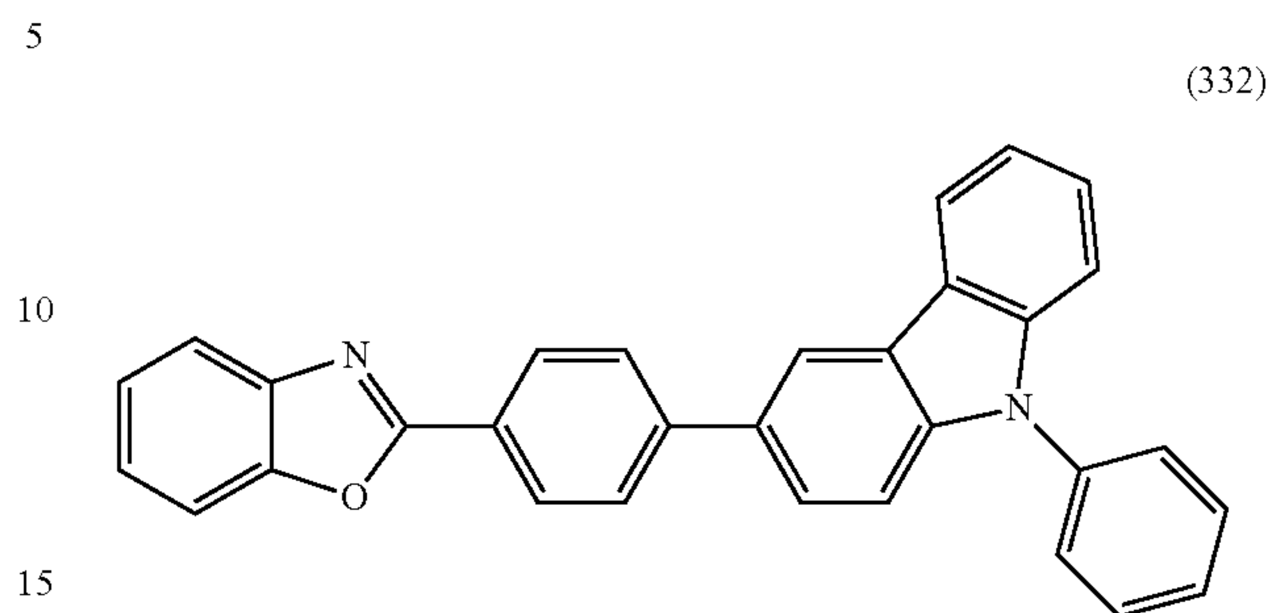
Synthesis of 3-[4-(Benzoxazol-2-yl)phenyl]-9-phenyl-9H-carbazole
