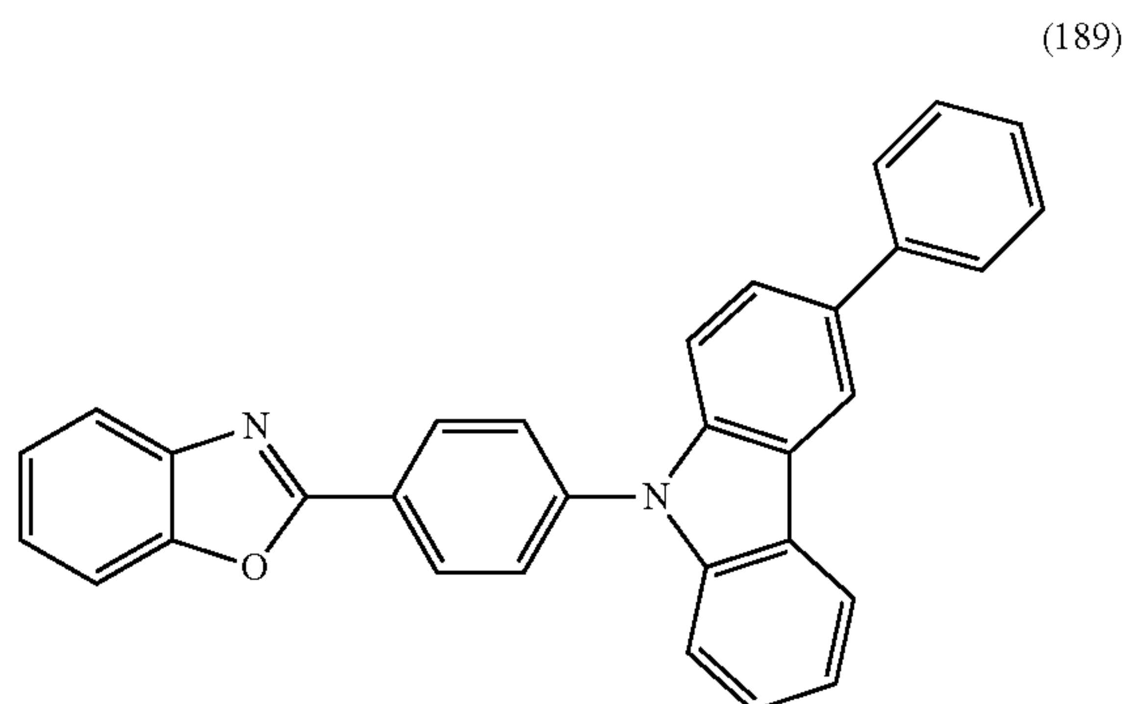
Synthesis of 9-(4-[Benzoxazol-2-yl]phenyl)-3-phenyl-9H-carbazole
