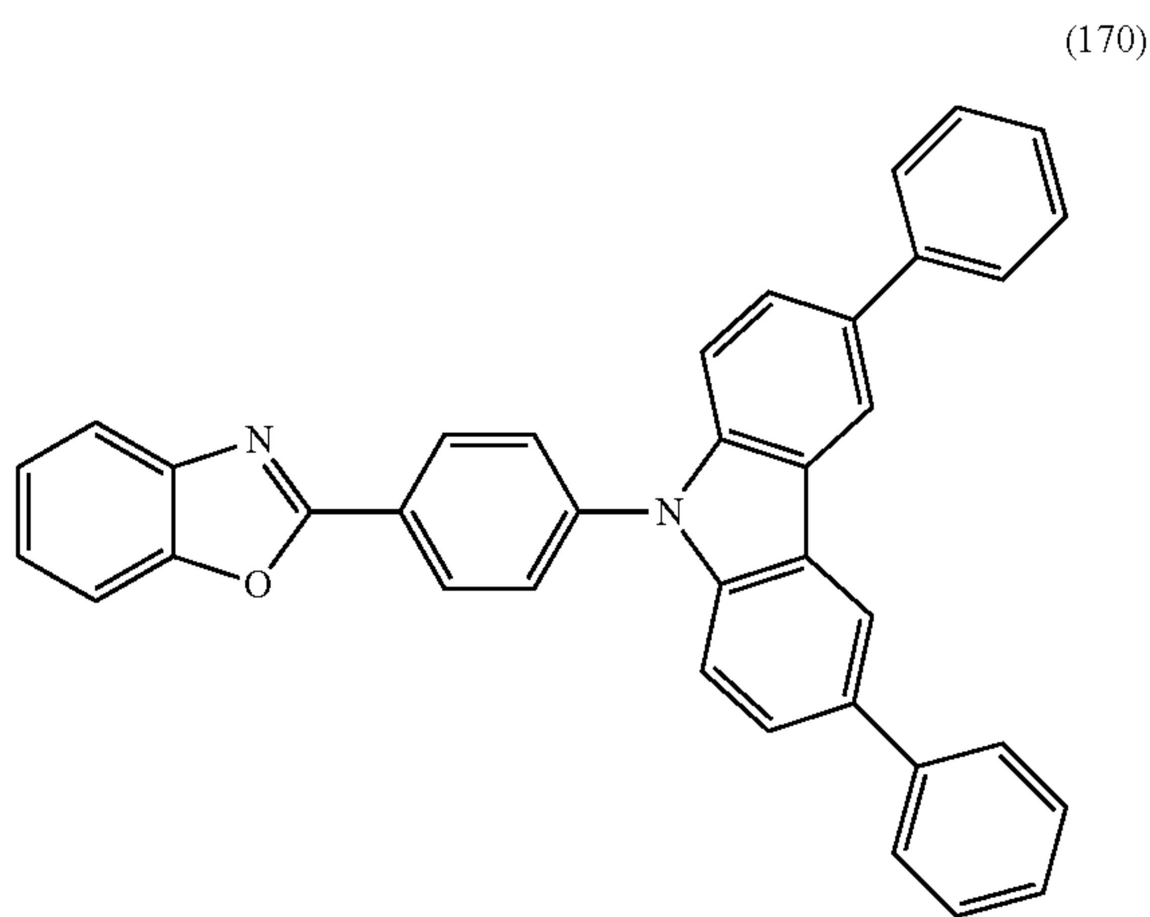
Synthesis of 9-(4-[Benzoxazol-2-yl]phenyl)-3,6-diphenyl-9H-carbazole
