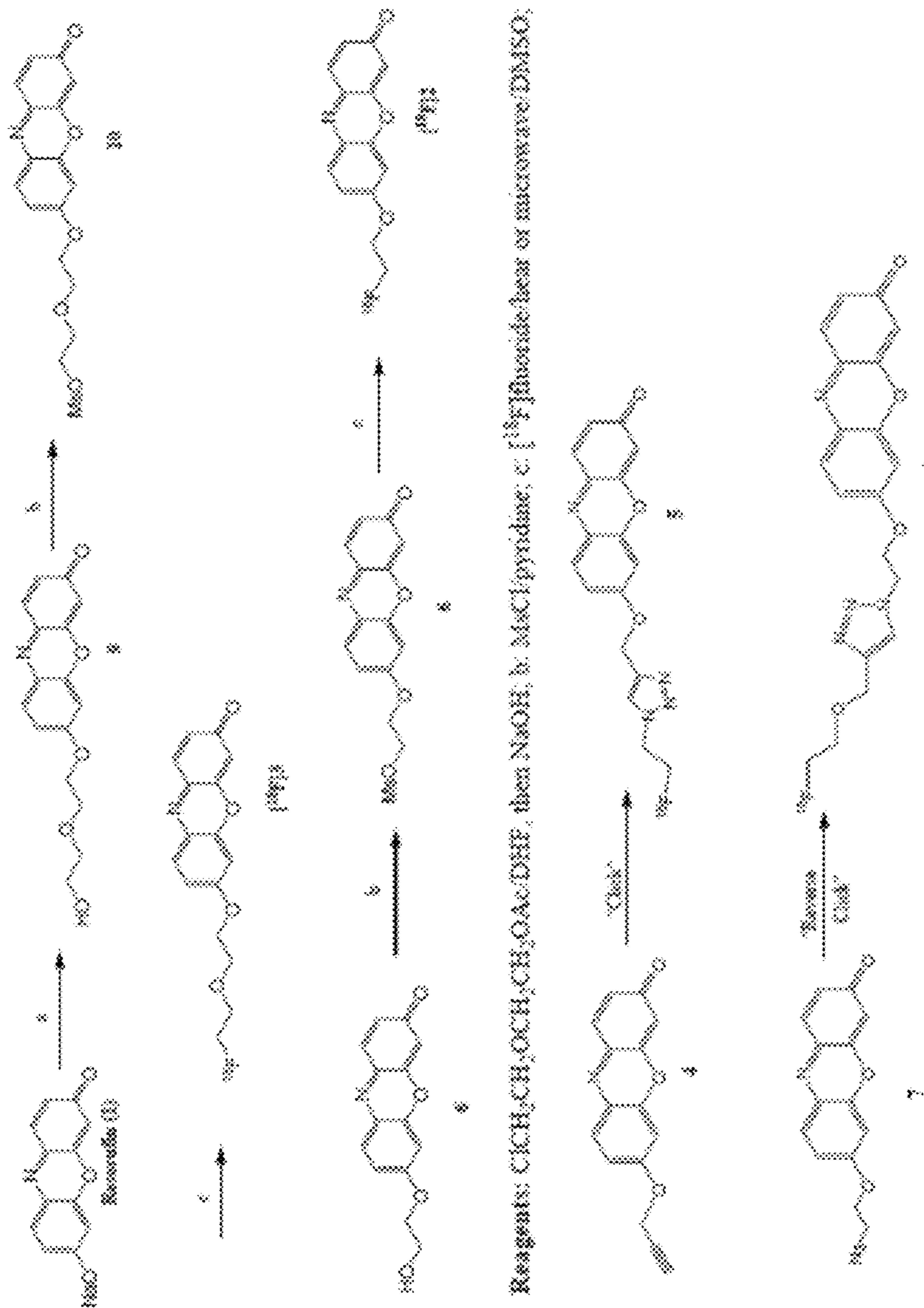
Synthesis of ^{18}\text{F} -resorufin analogs.
