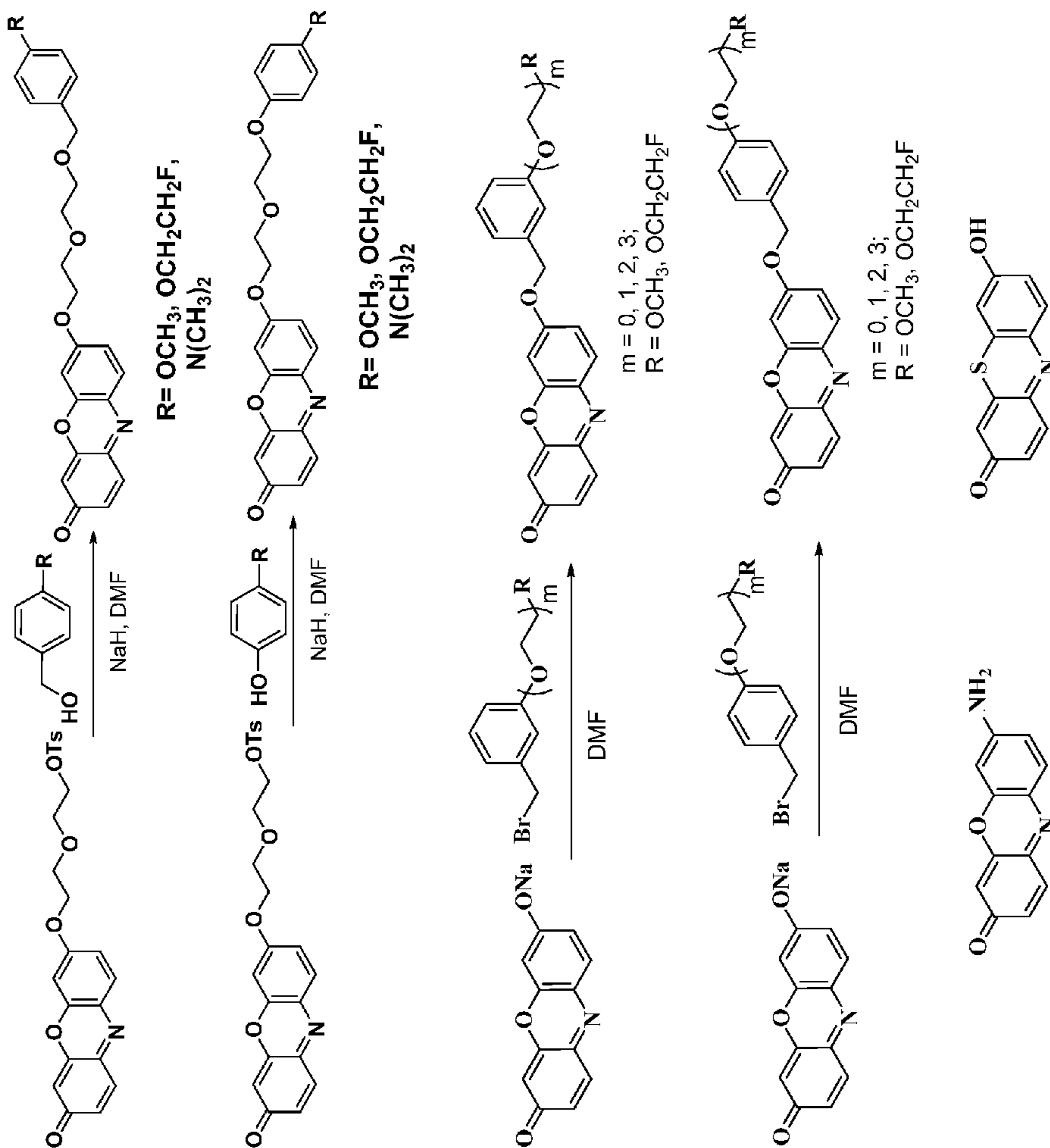
7-Amino-3H-Phenoxazin-3-one
