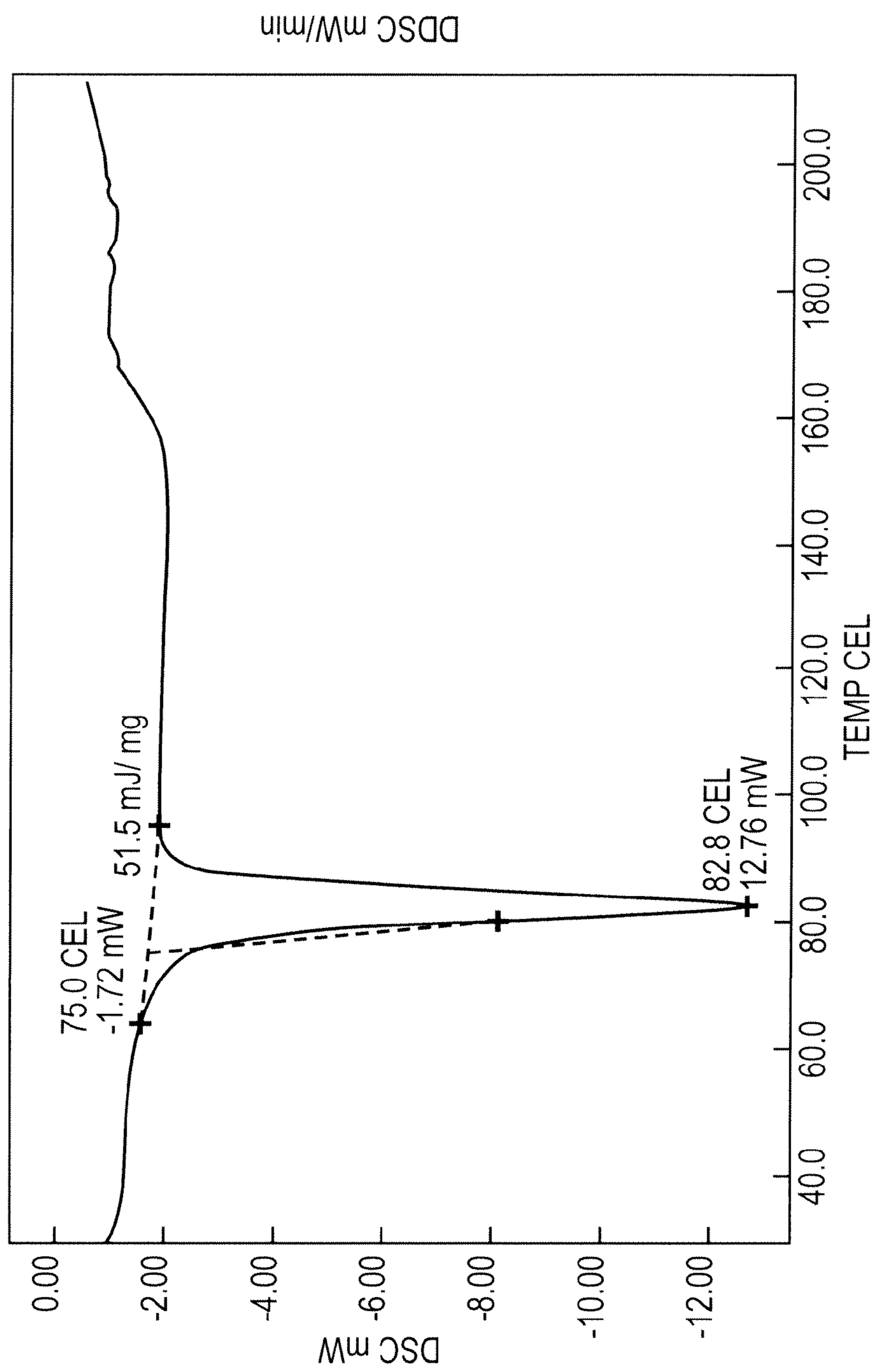
DSC OF FORMA
