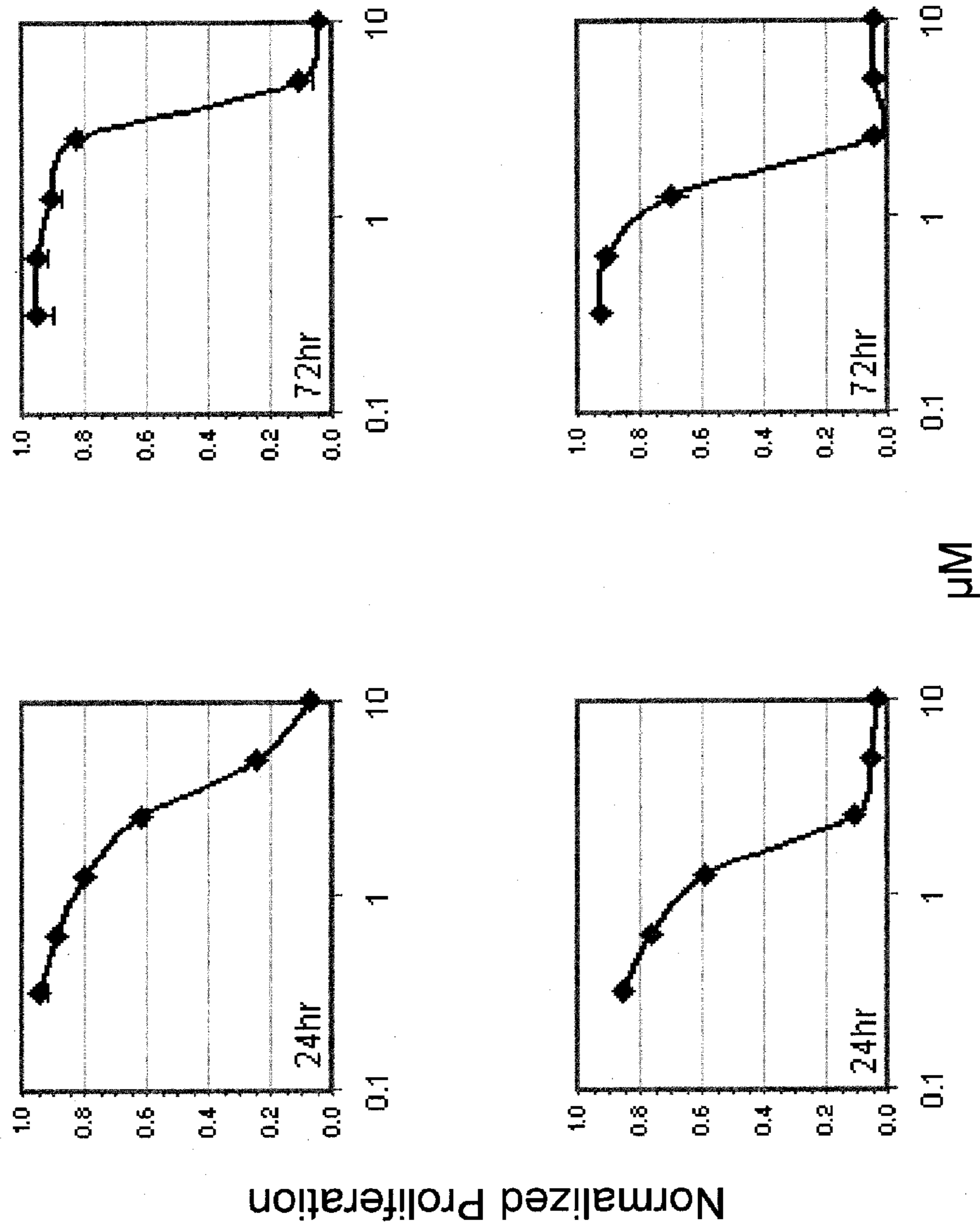
Compound 15
