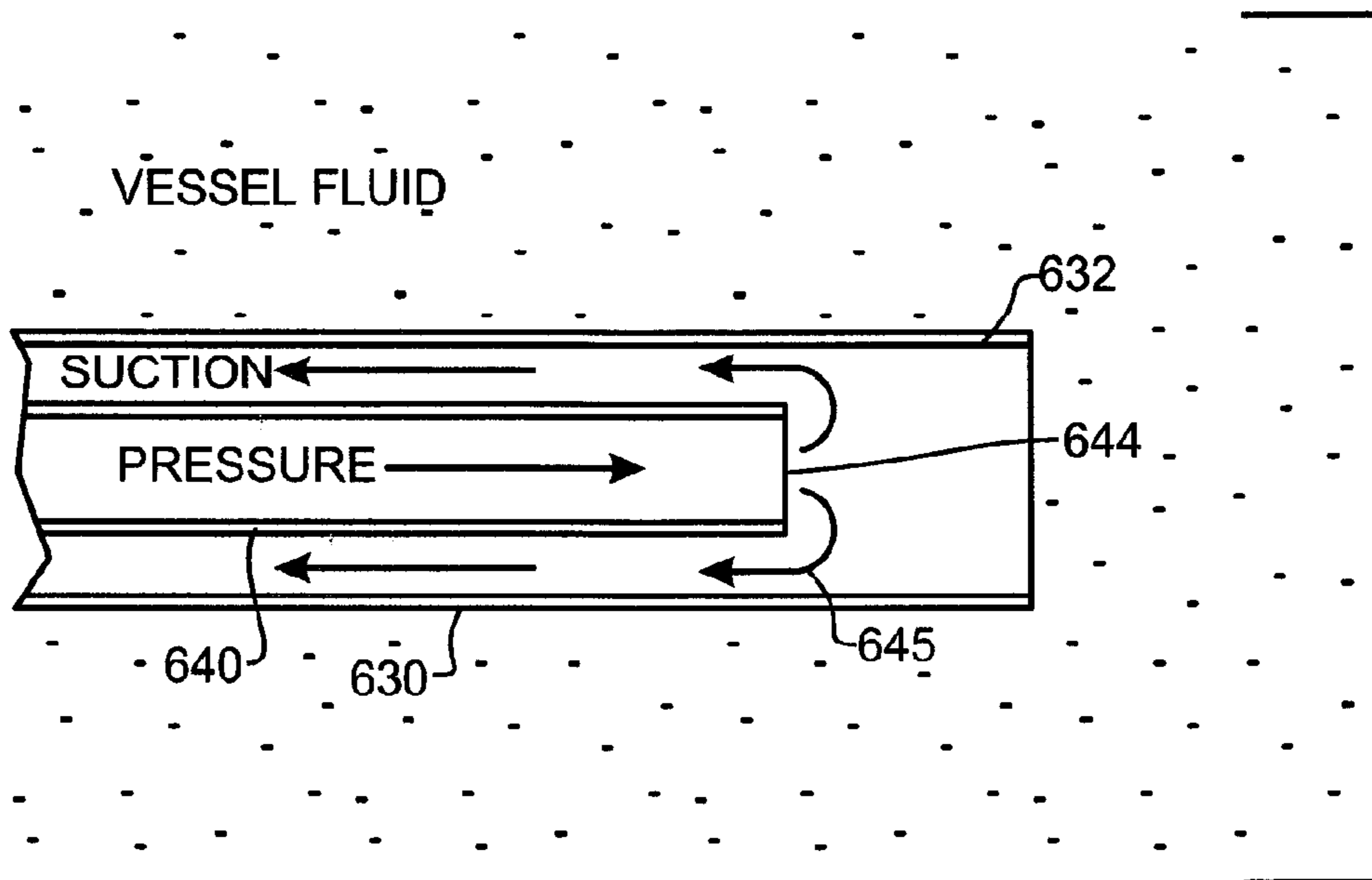
FIG. 11 (PRIOR ART)
