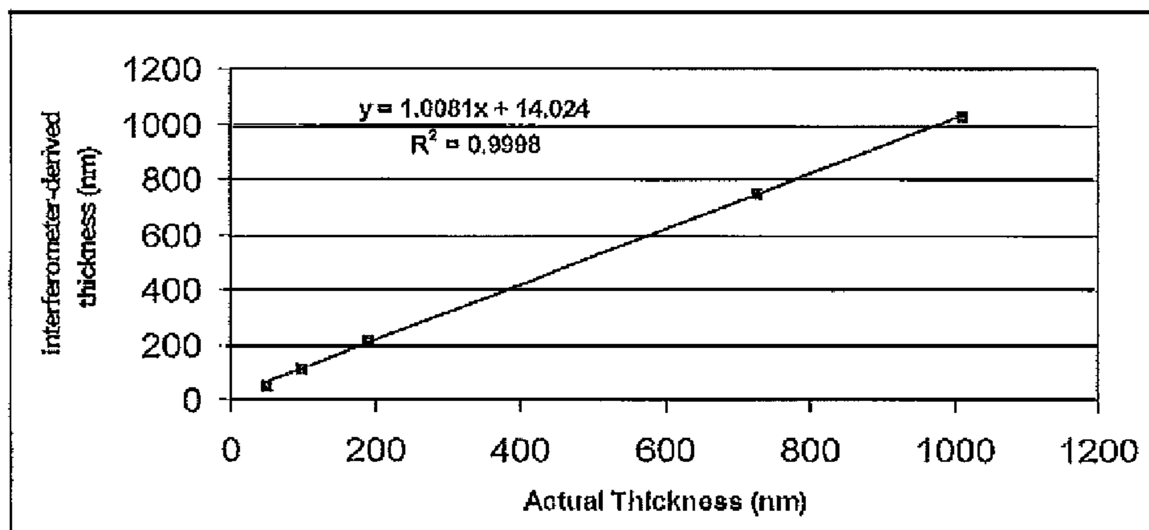
Figure 2. Standard curve from SiO 2 thin film thickness standards.
