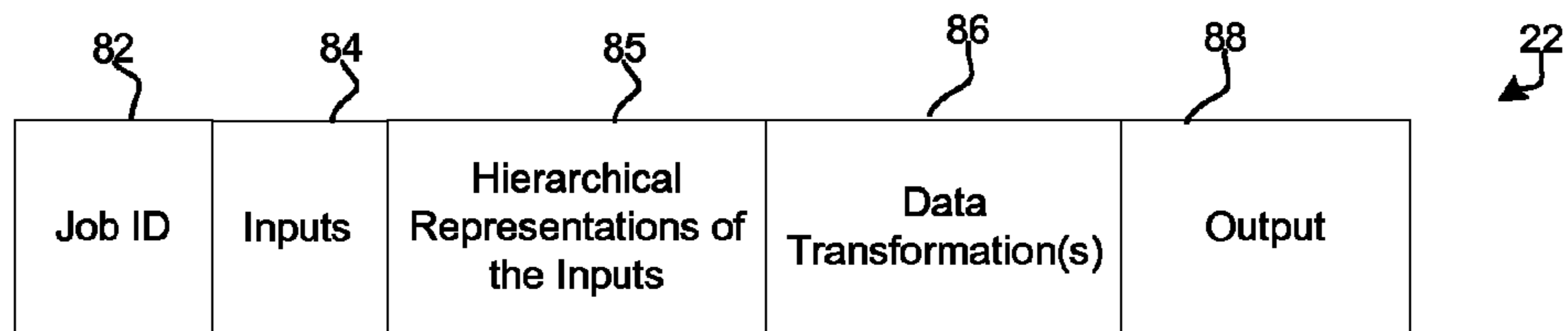
Data Transformation Job
