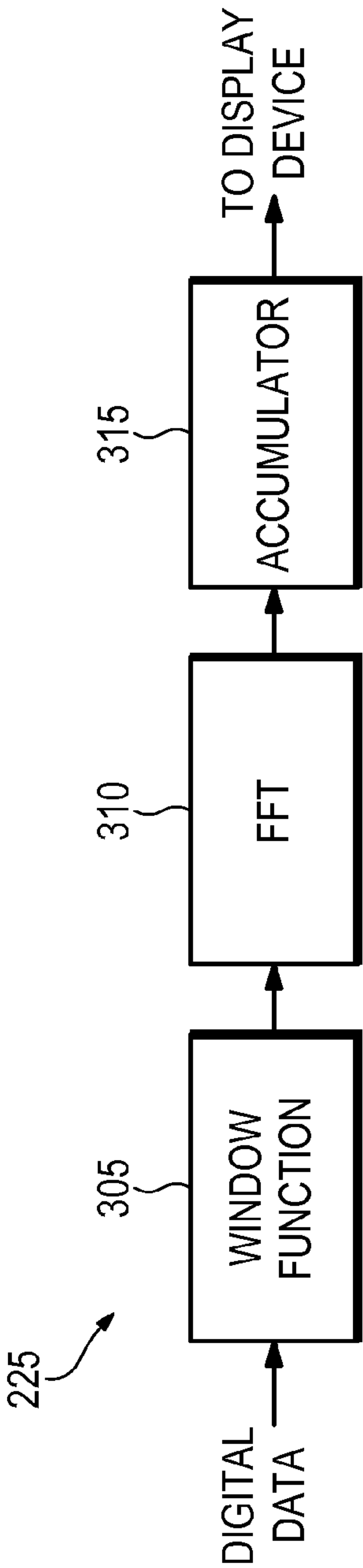
Figure 3 (PRIOR ART)
