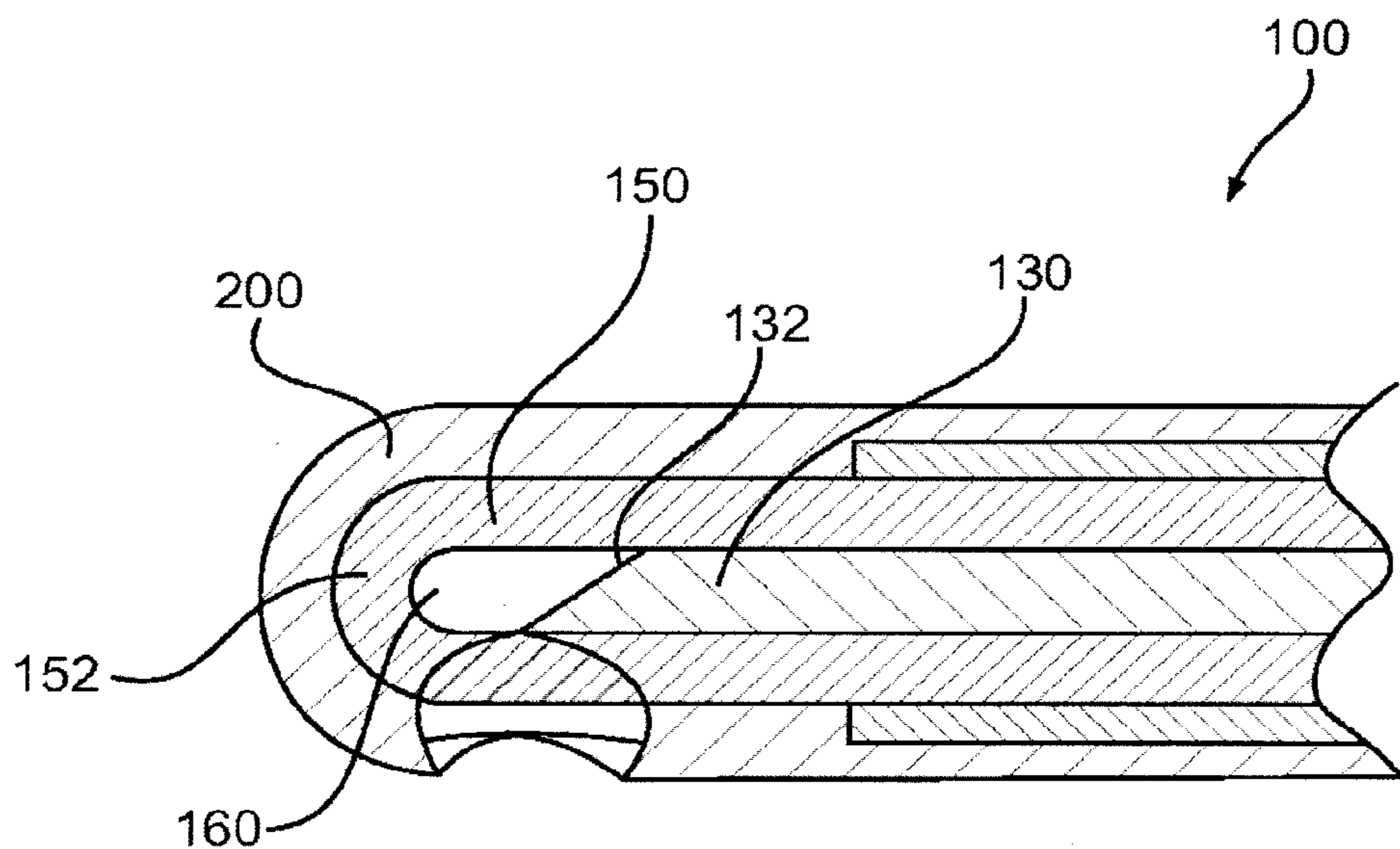
FIG. 2 (PRIOR ART)
