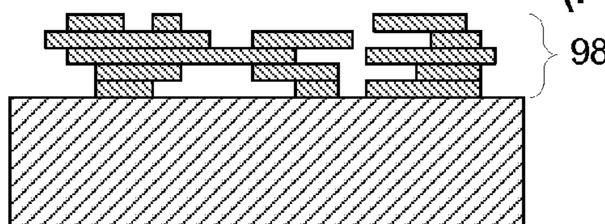
FIG. 4I (PRIOR ART)
