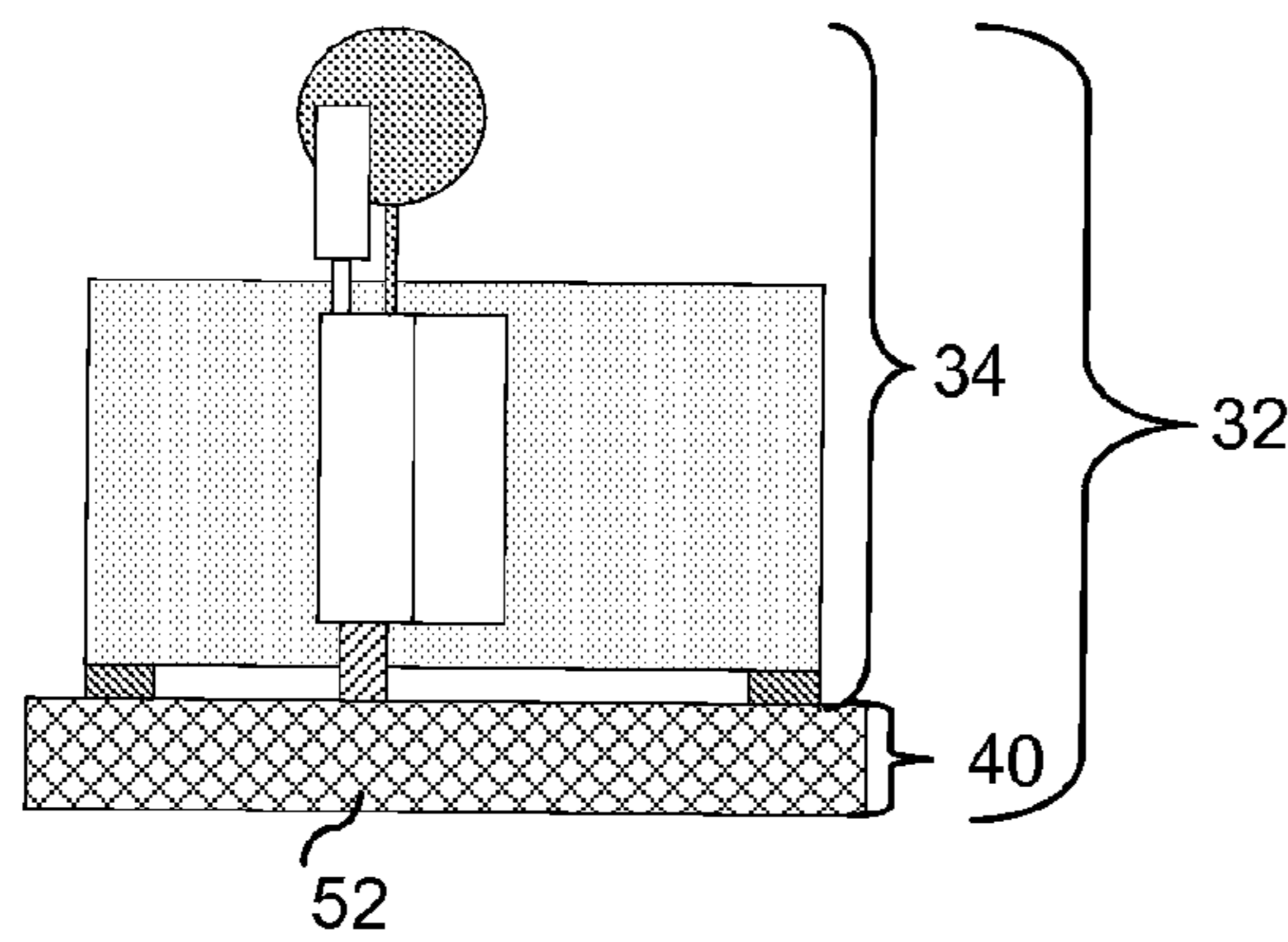
FIG. 3C (PRIOR ART)
