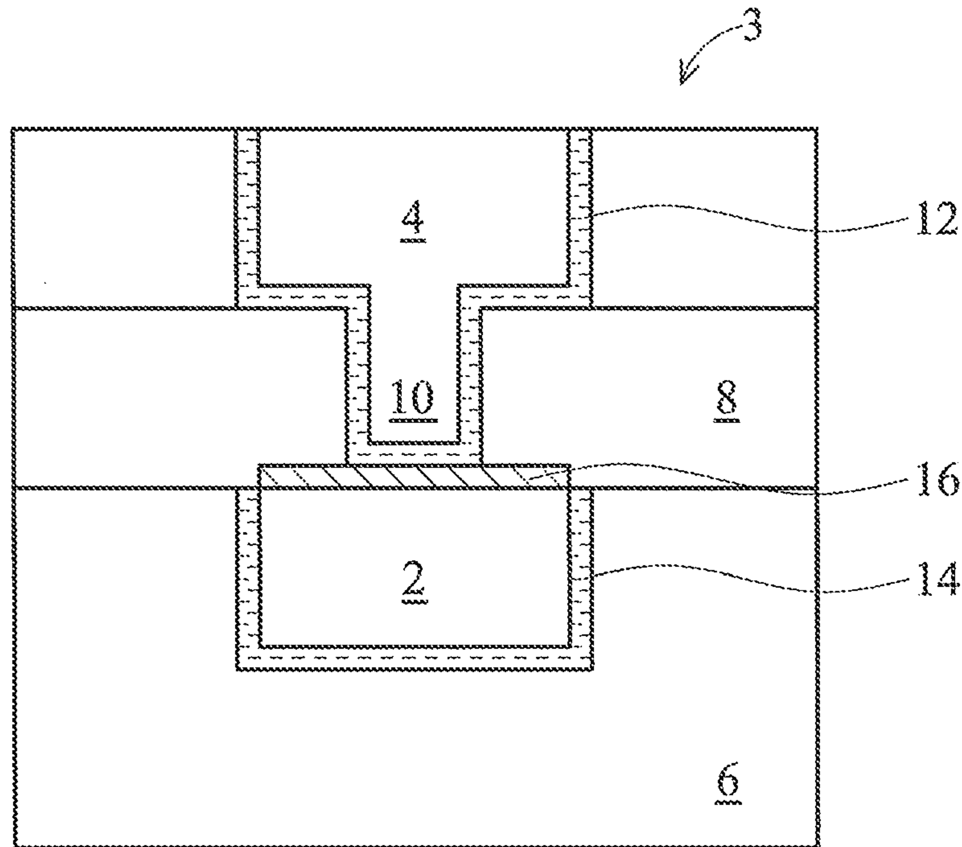
FIG. 2 (PRIOR ART)
