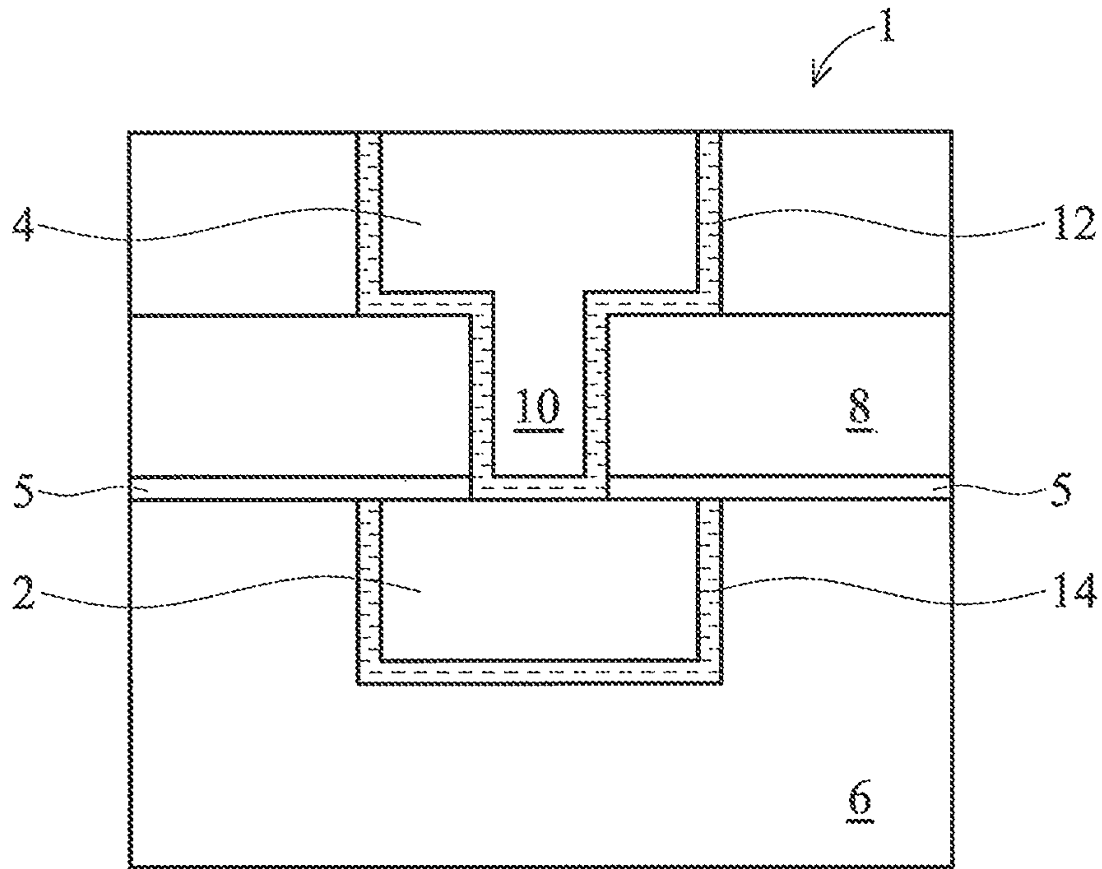
FIG. 1 (PRIOR ART)
