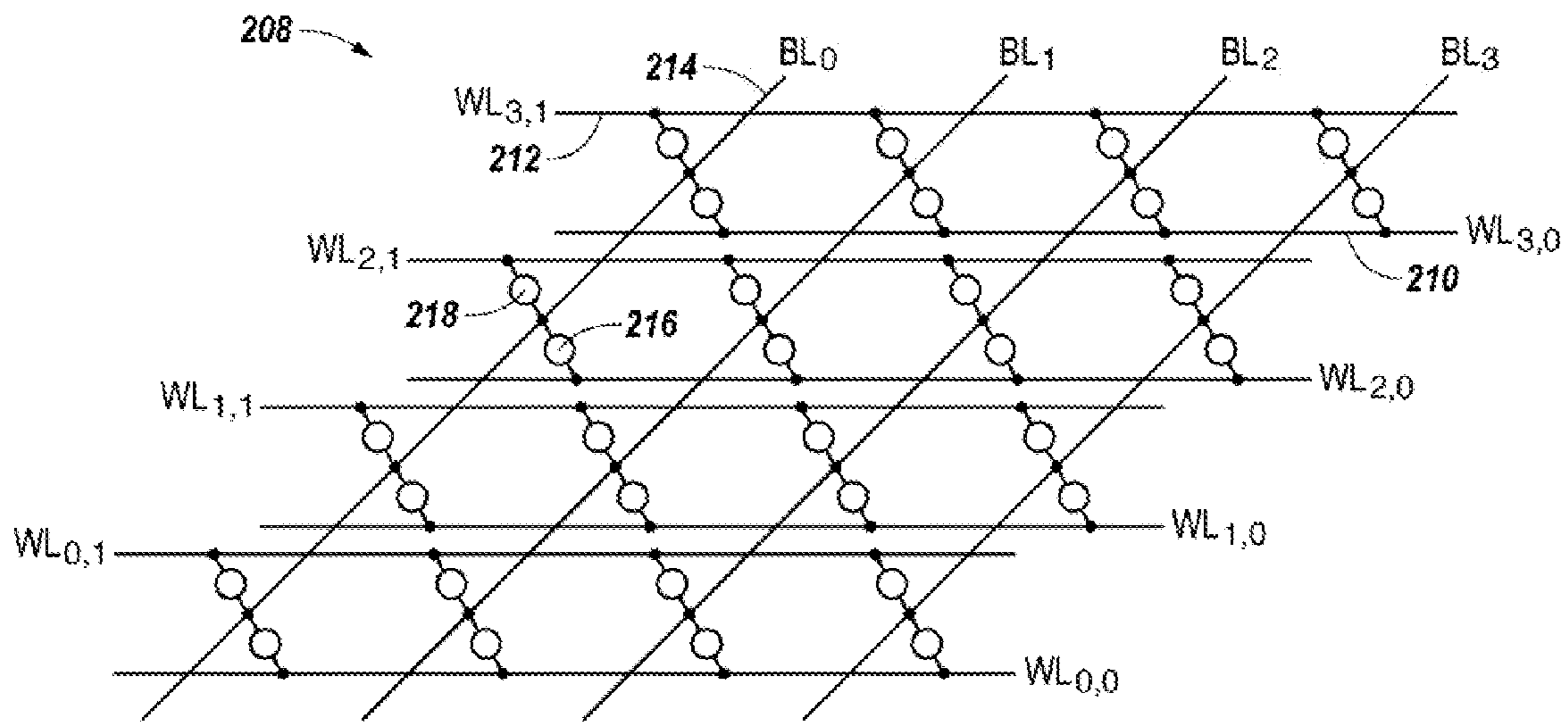
Fig. 2 (PRIOR ART)
