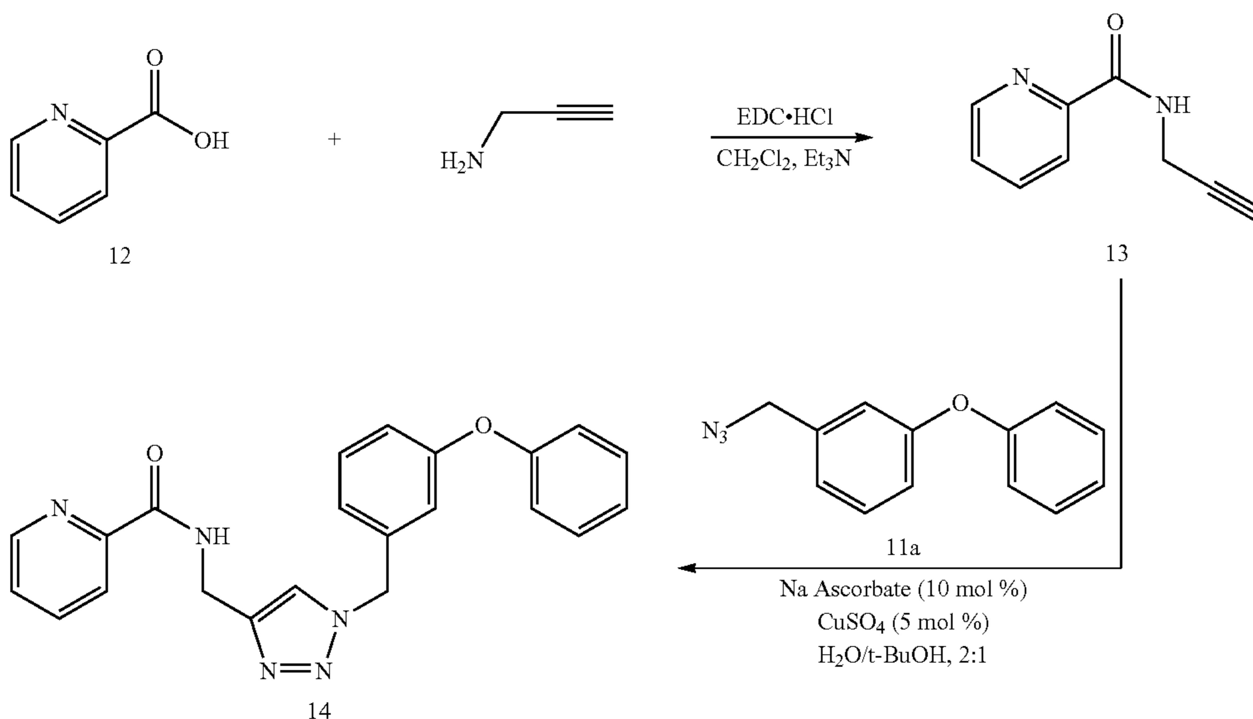
Scheme 3. Simplified synthesis of antimitotic 1,2,3-triazole from commercially available aryl acid
