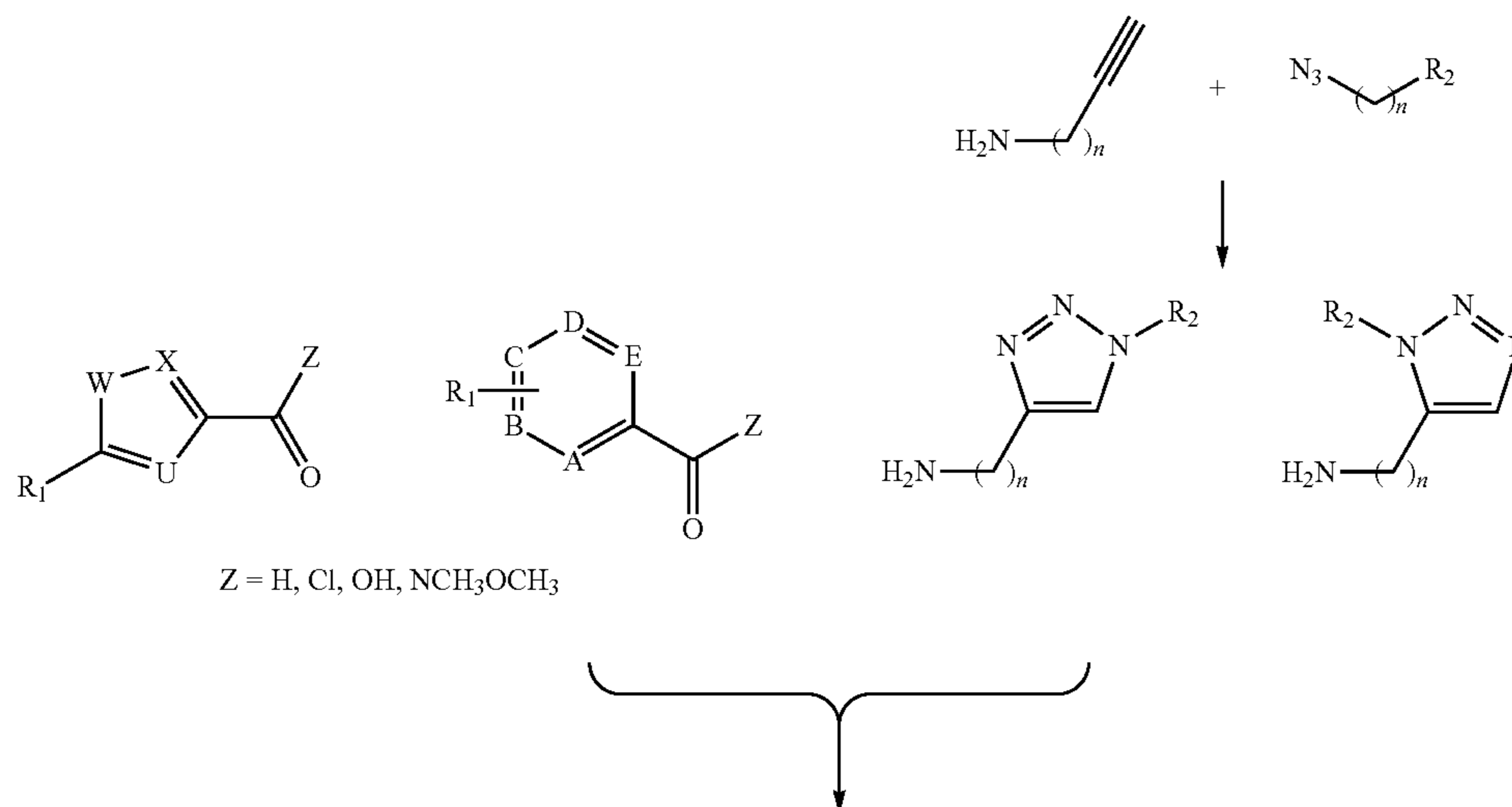
Scheme 4. Synthesis of various triazoles
