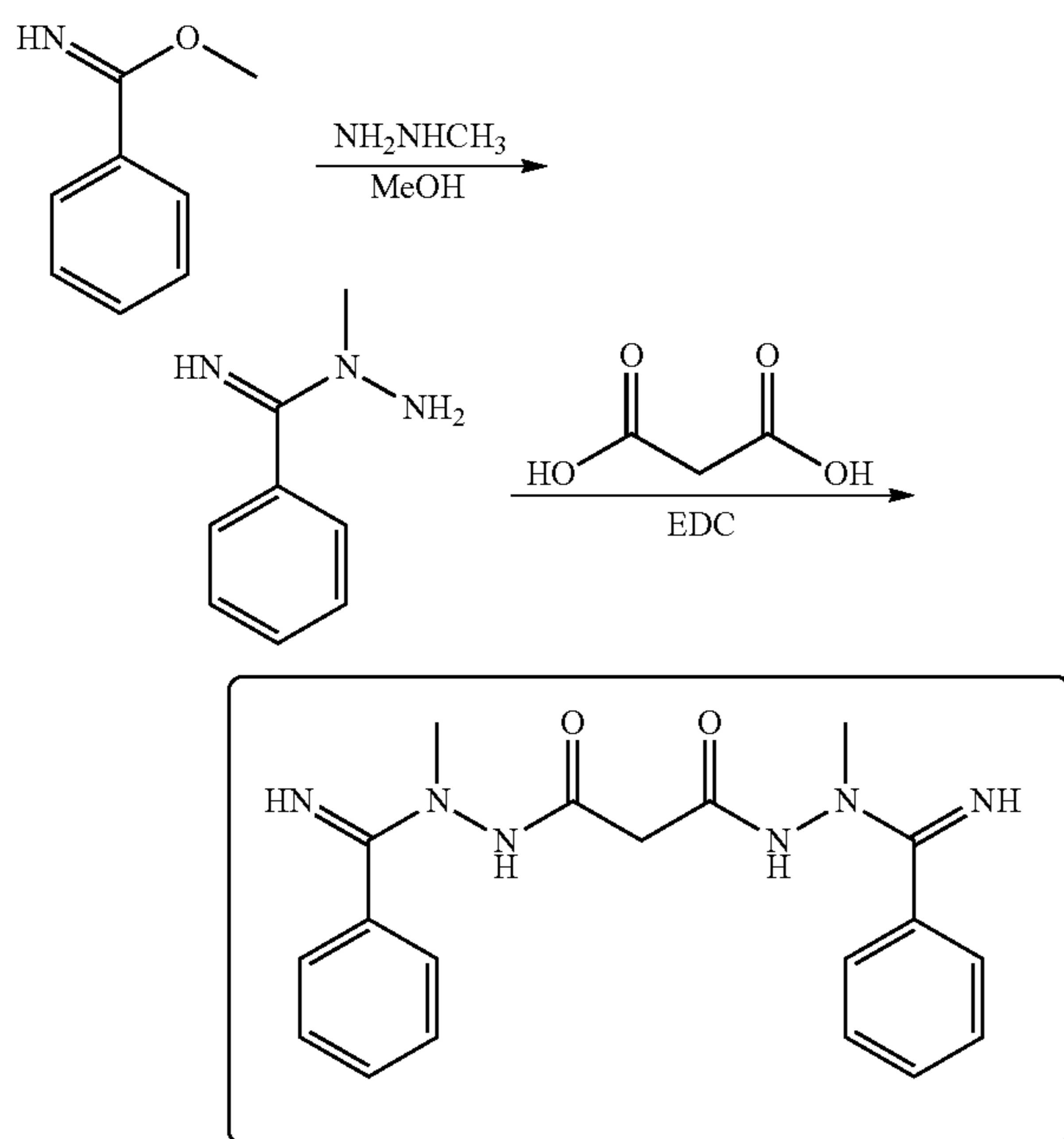
Scheme V:
