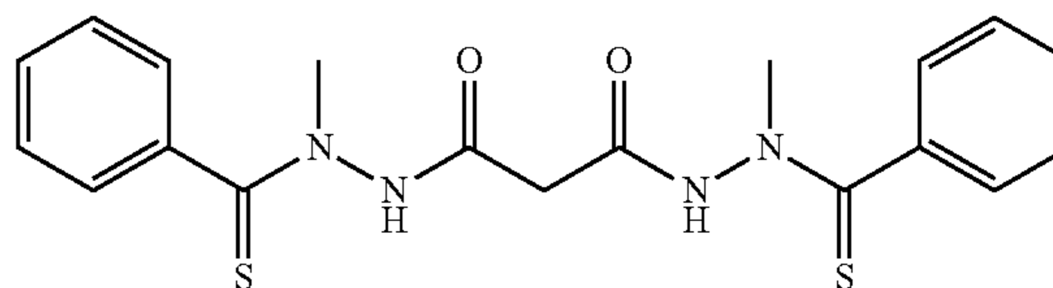
Compound A:
