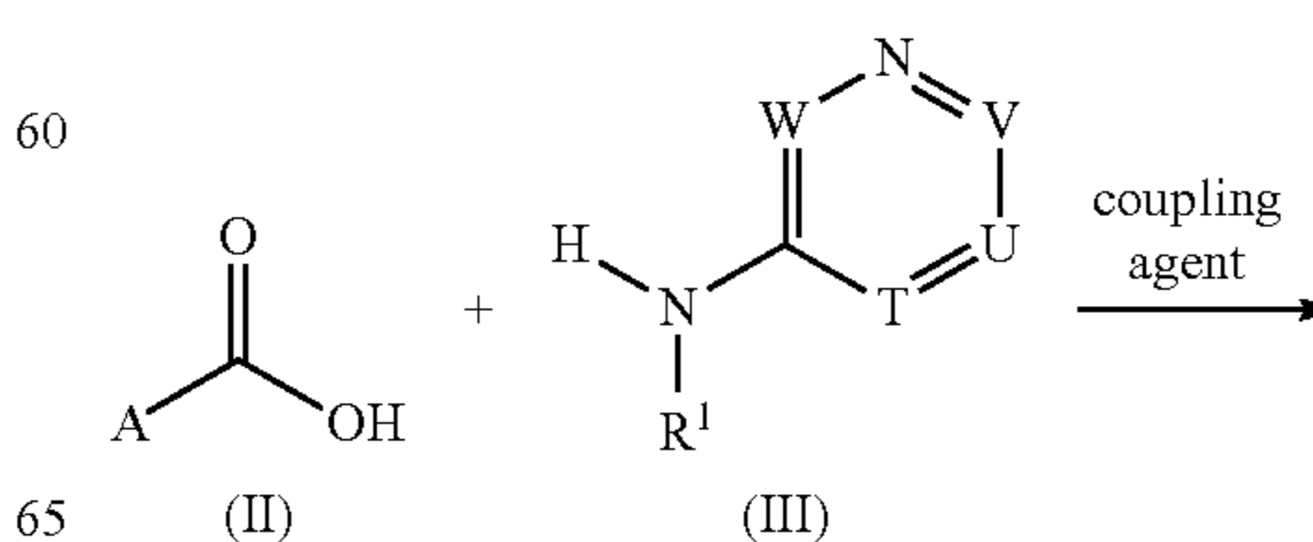
Scheme 2:
