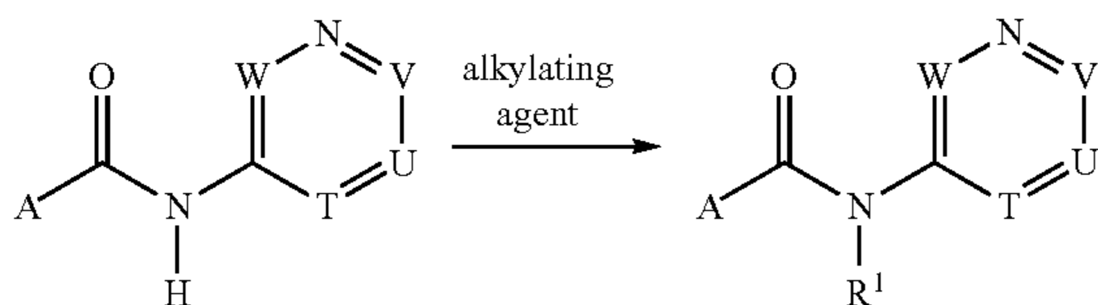
Scheme 3:
