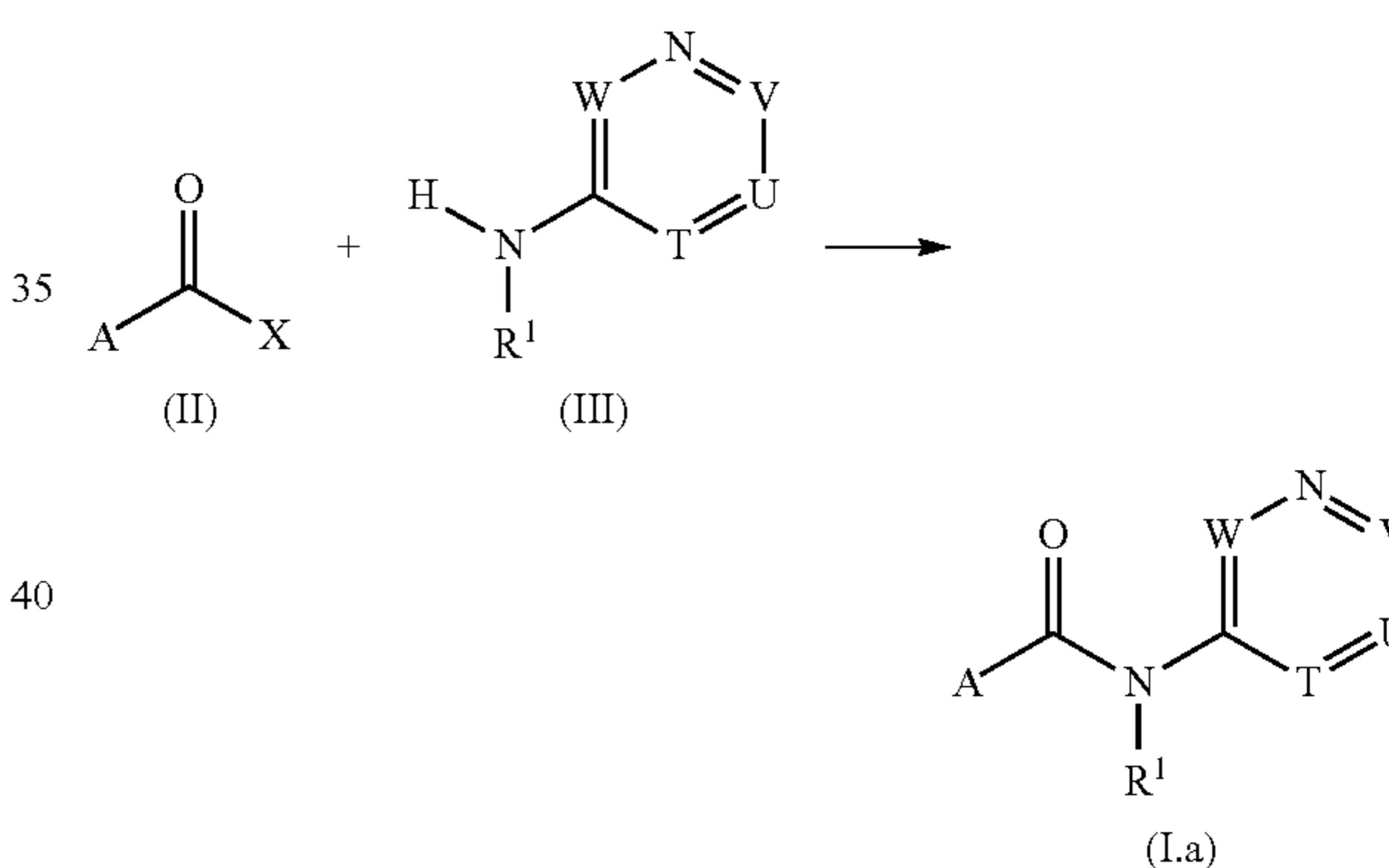
Scheme 1:
