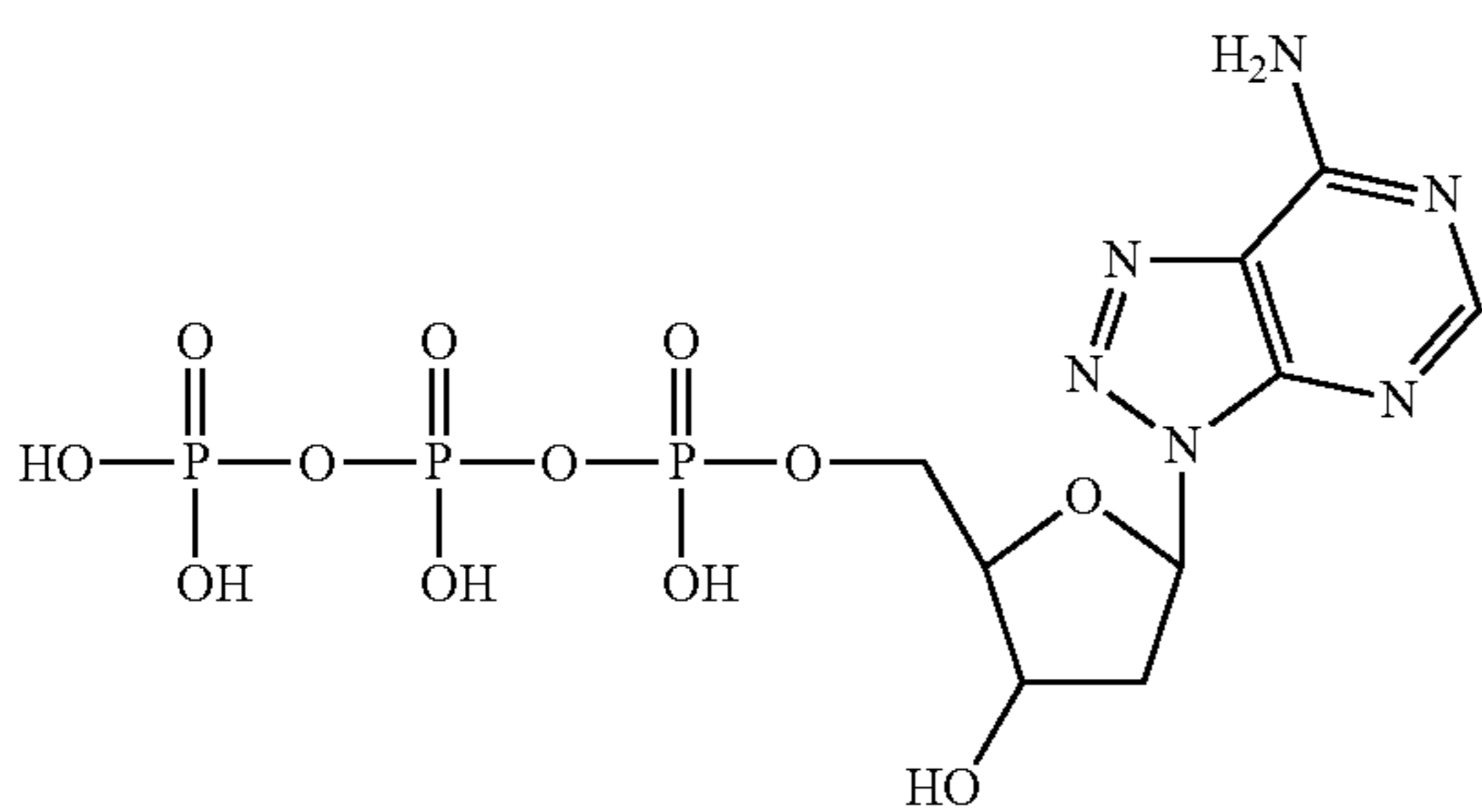
8-aza-2'-deoxy-adenosine-5'-triphosphate
