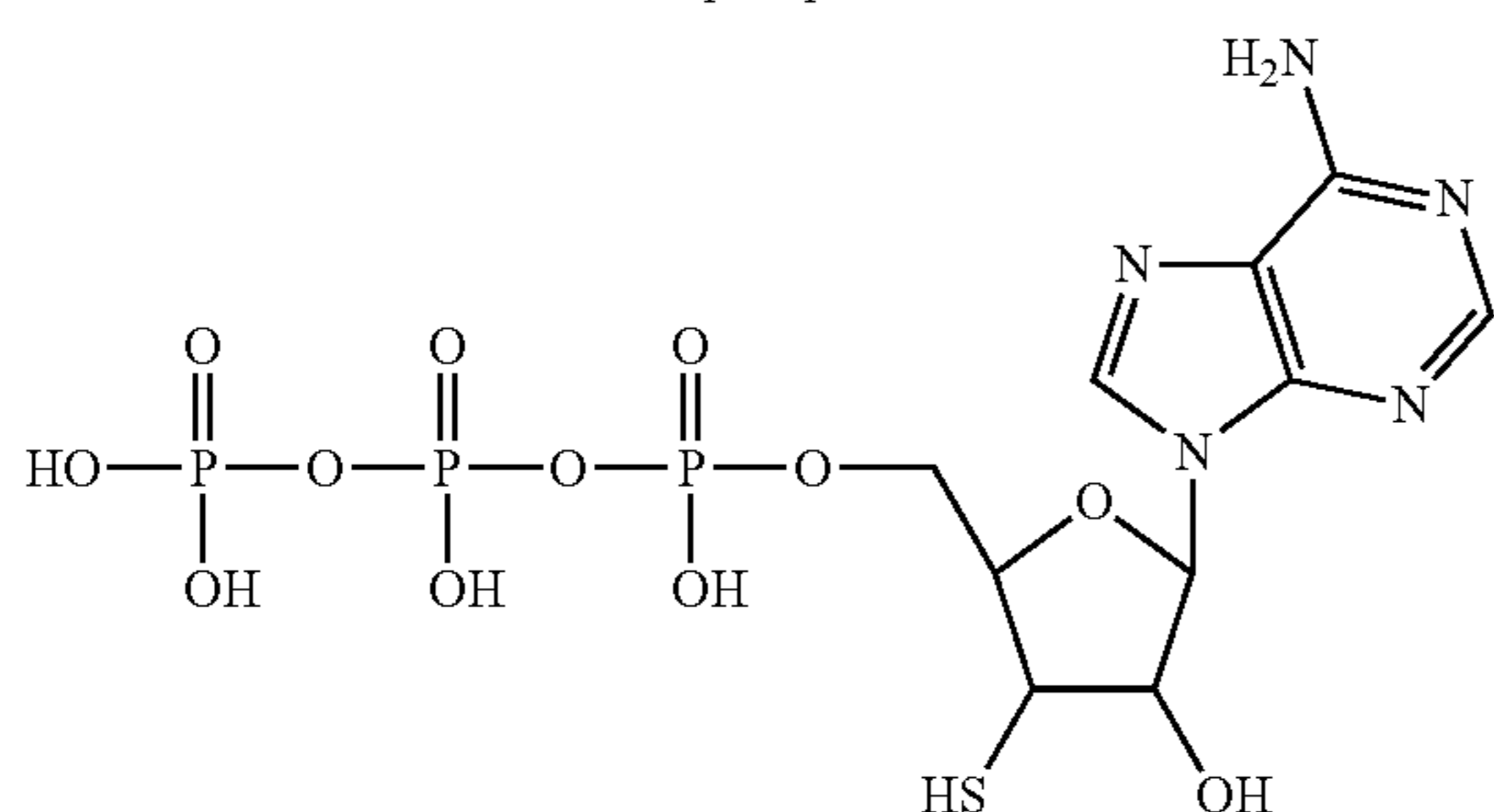
3'-thio-3'-deoxyadenosine-5'-triphosphate
