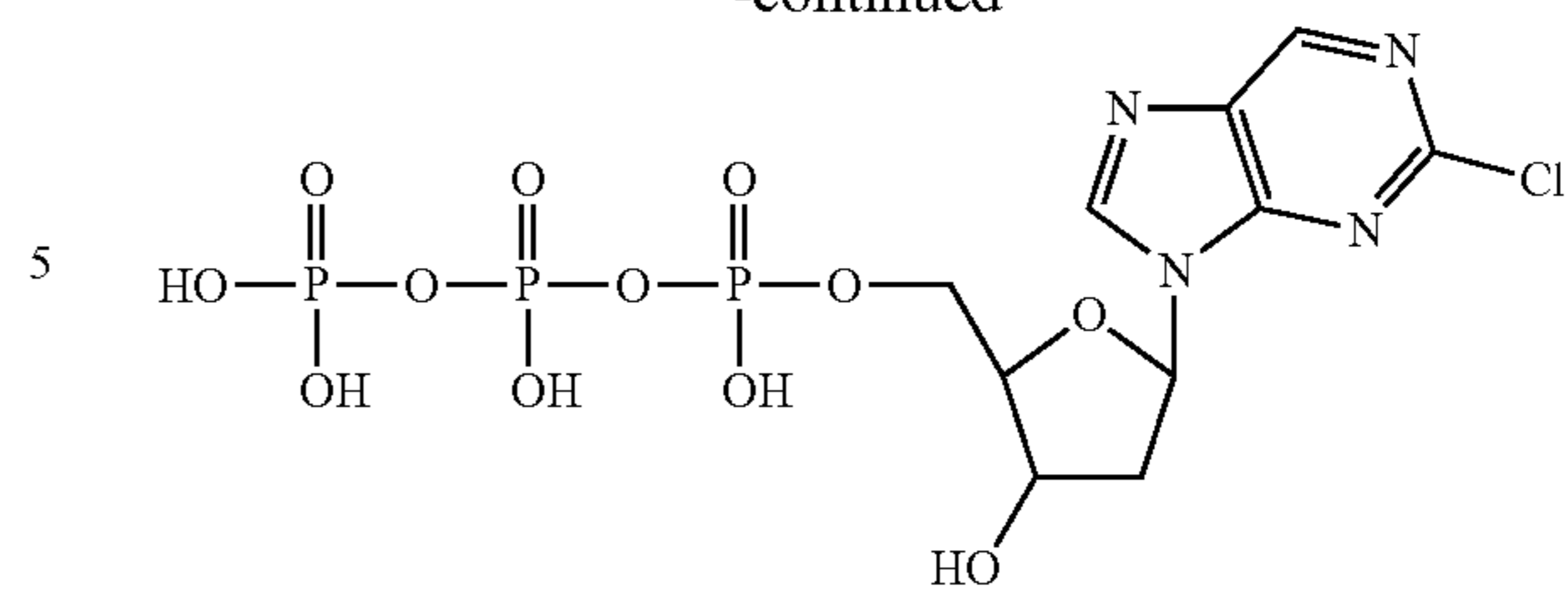
2-Chloropurine-2'-deoxyriboside-5'-triphosphate
