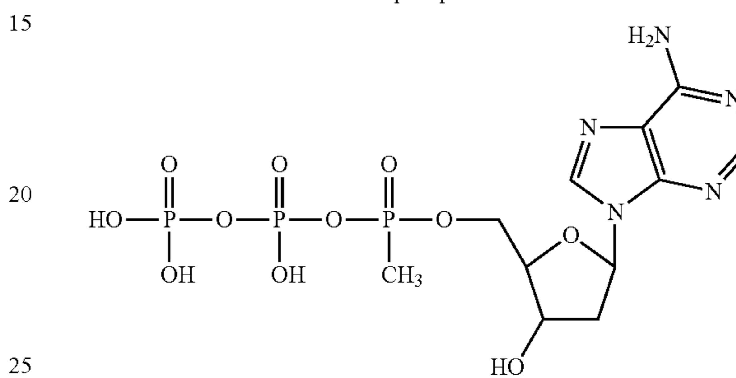
5'-alpha-methylphosphonate-2'-deoxyadenosine-5'-triphosphate
