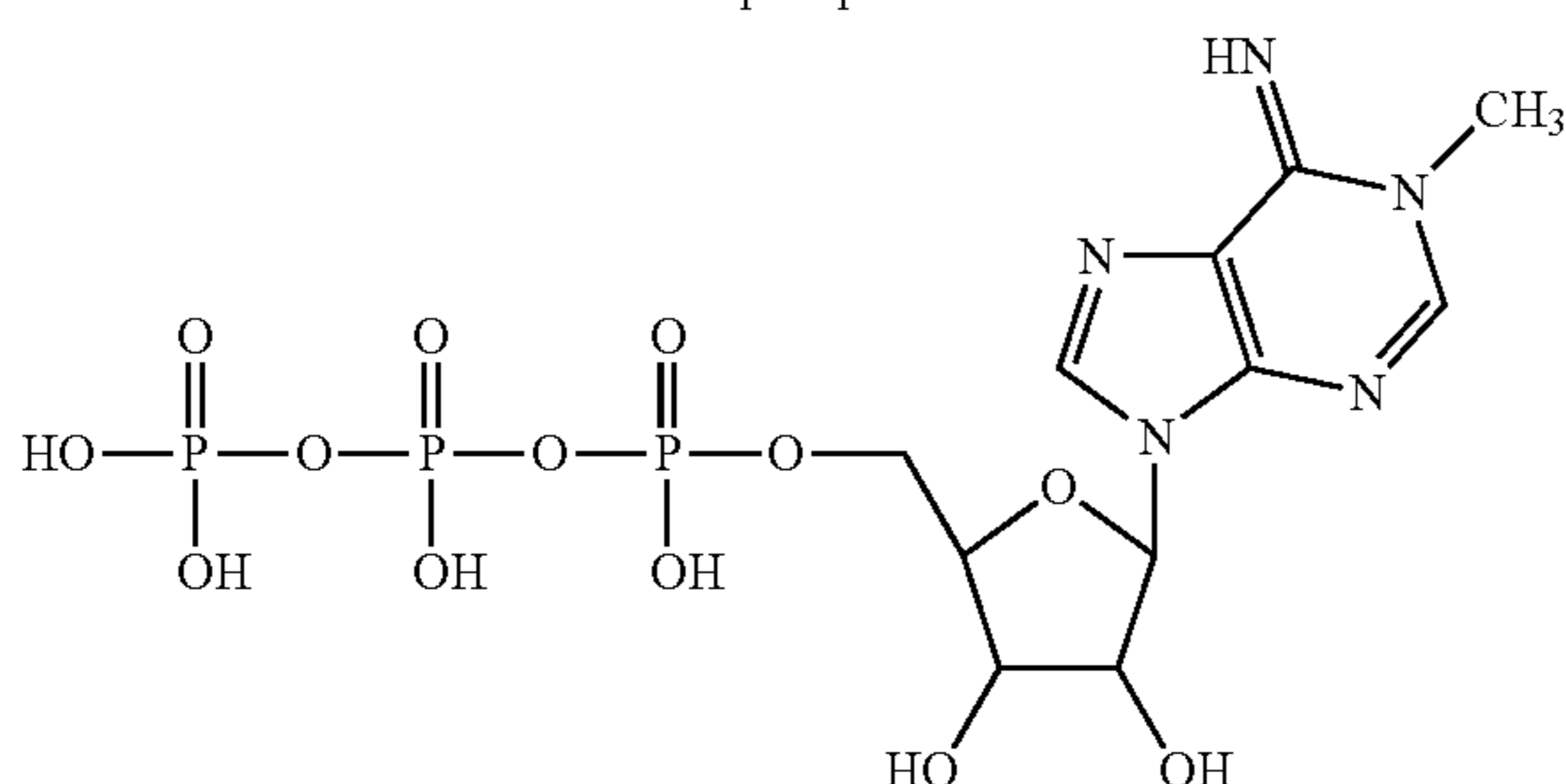
N1-methyl-adenosine-5'-triphosphate
