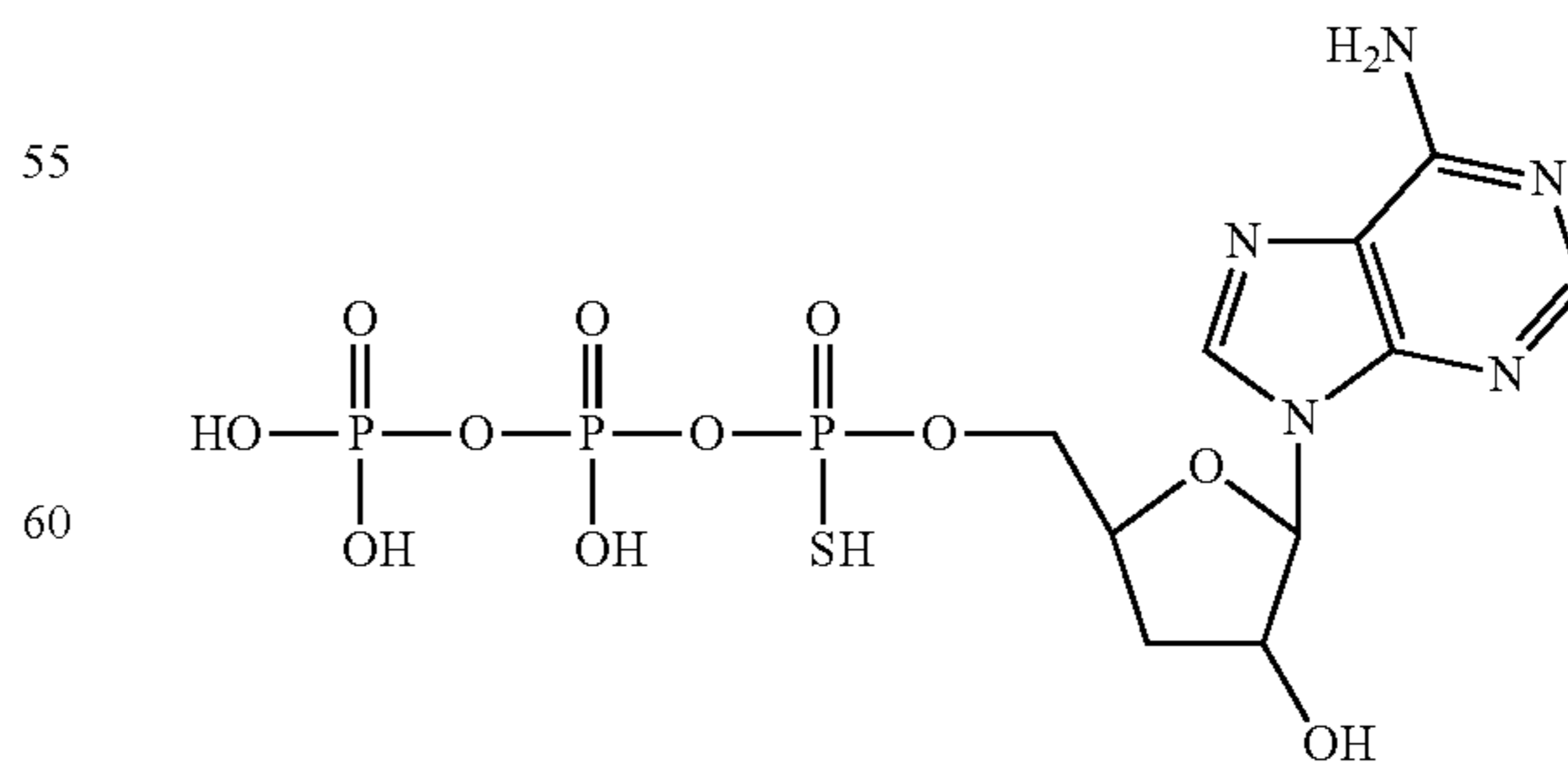
5'-alpha-thio-3'-deoxyadenosine-5'-triphosphate
