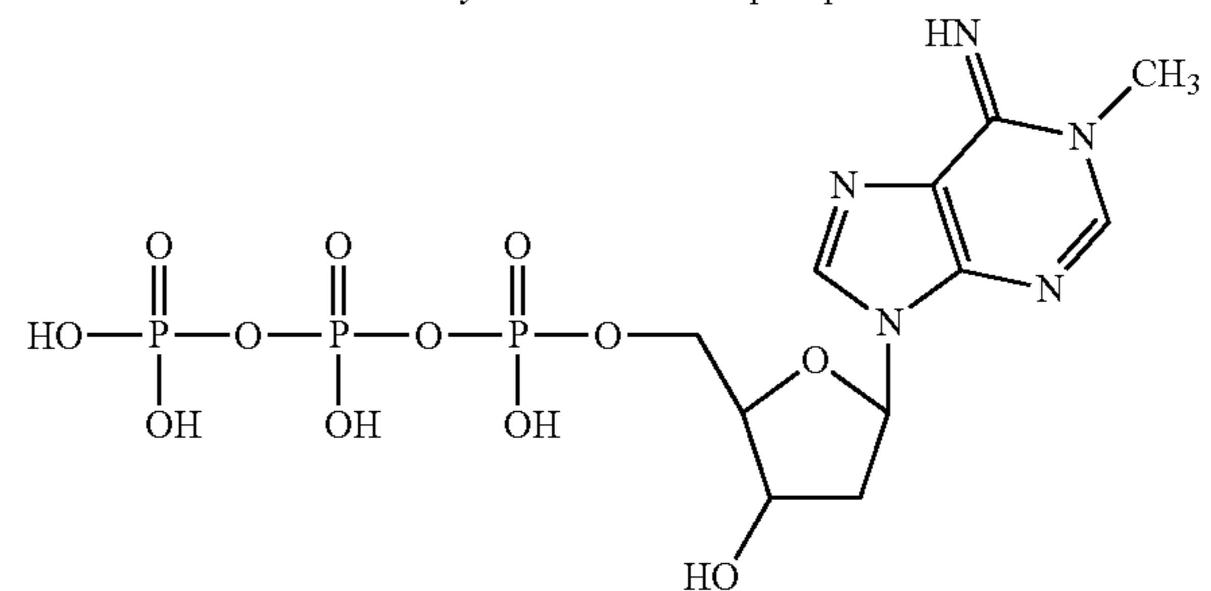
N1-methyl-2'-deoxyadenosine-5'-triphosphate
