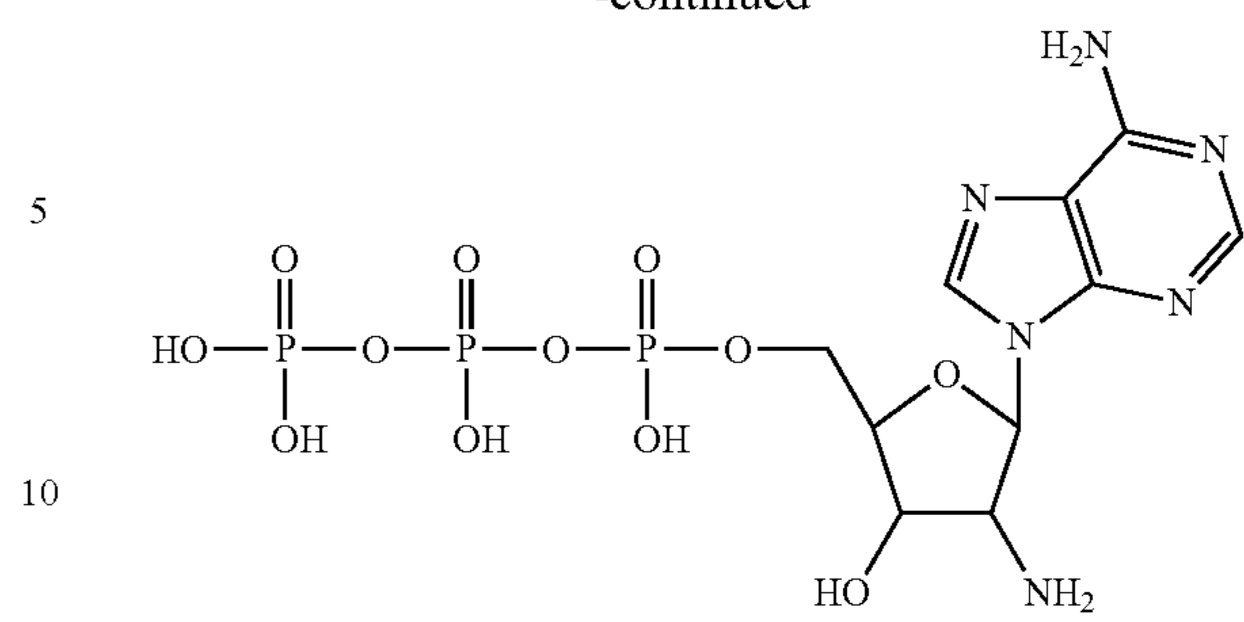
2'-amino-2'-deoxy-adenosine-5'-triphosphate
