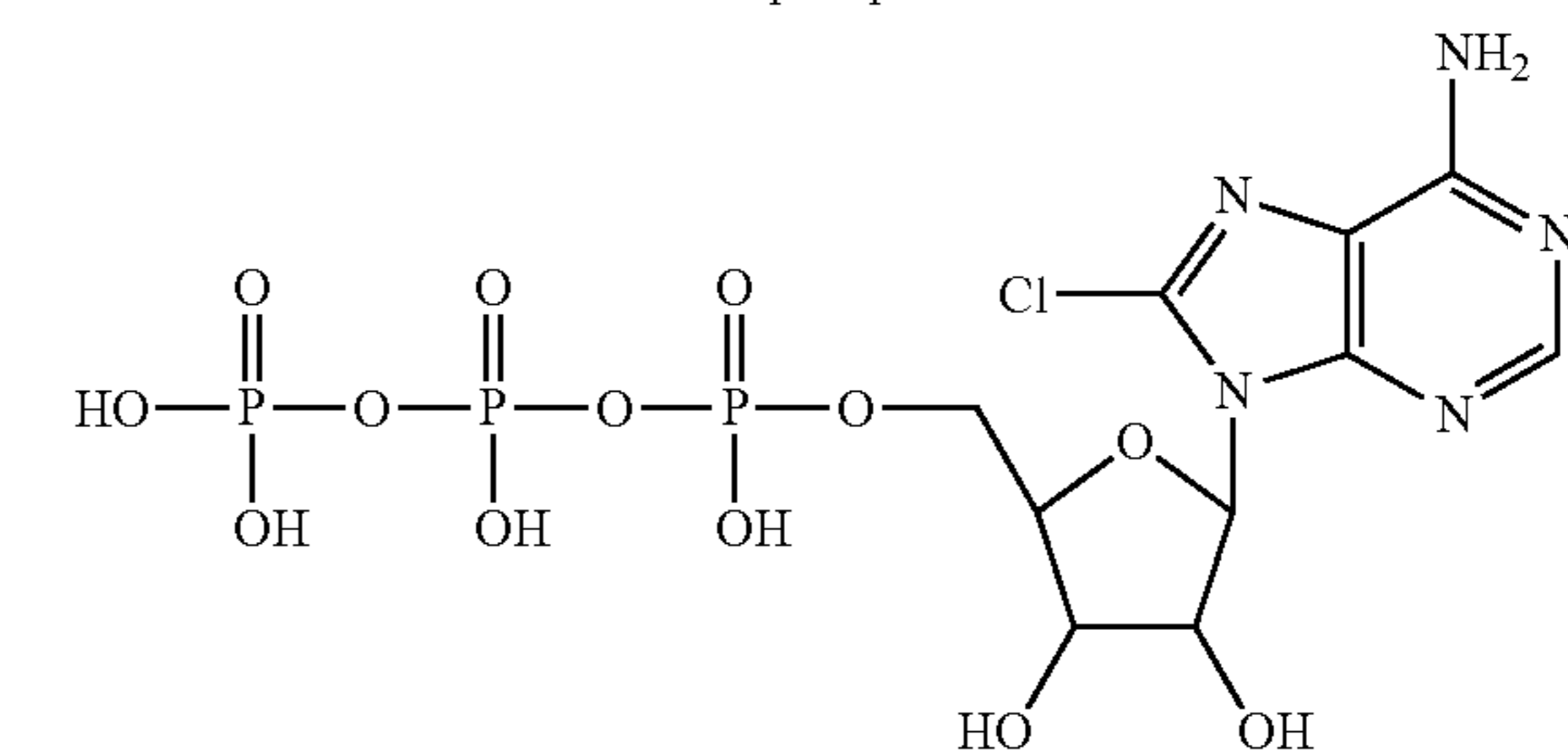
8-chloro-adenosine-5'-triphosphate
