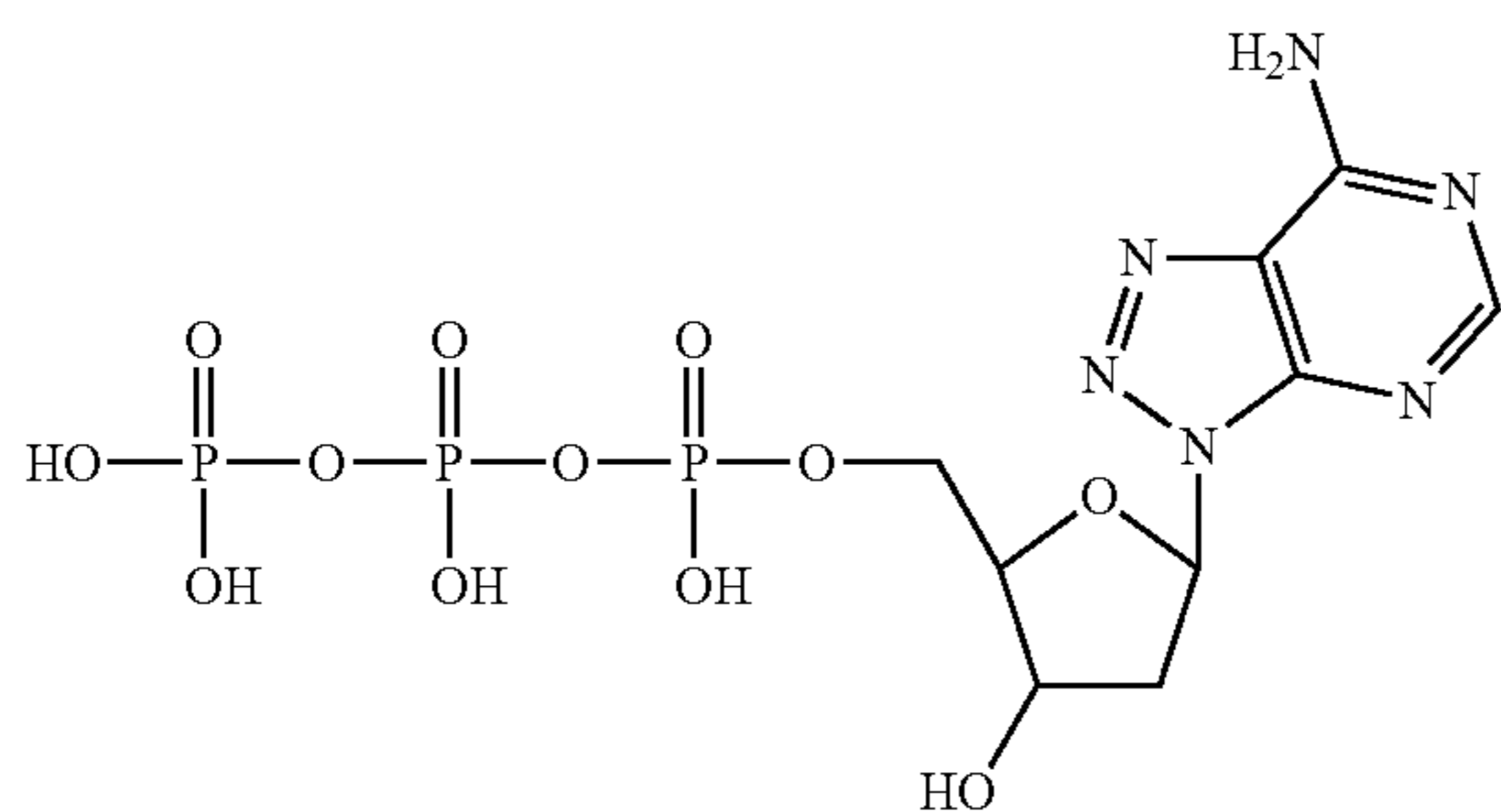
8-aza-2'-deoxy-adenosine-5'-triphosphate
