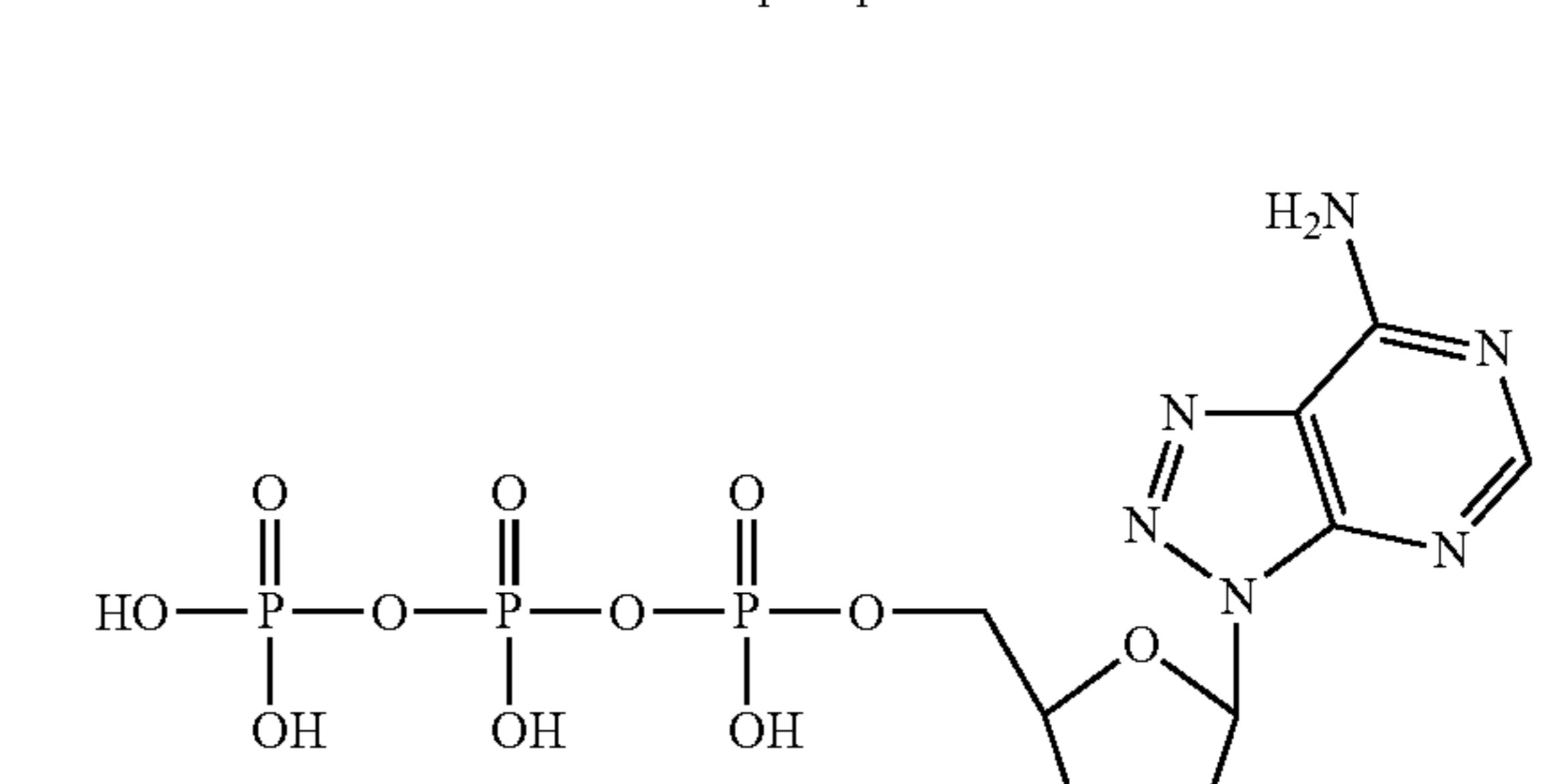
8-chloro-2'-deoxy-adenosine-5'-triphosphate
