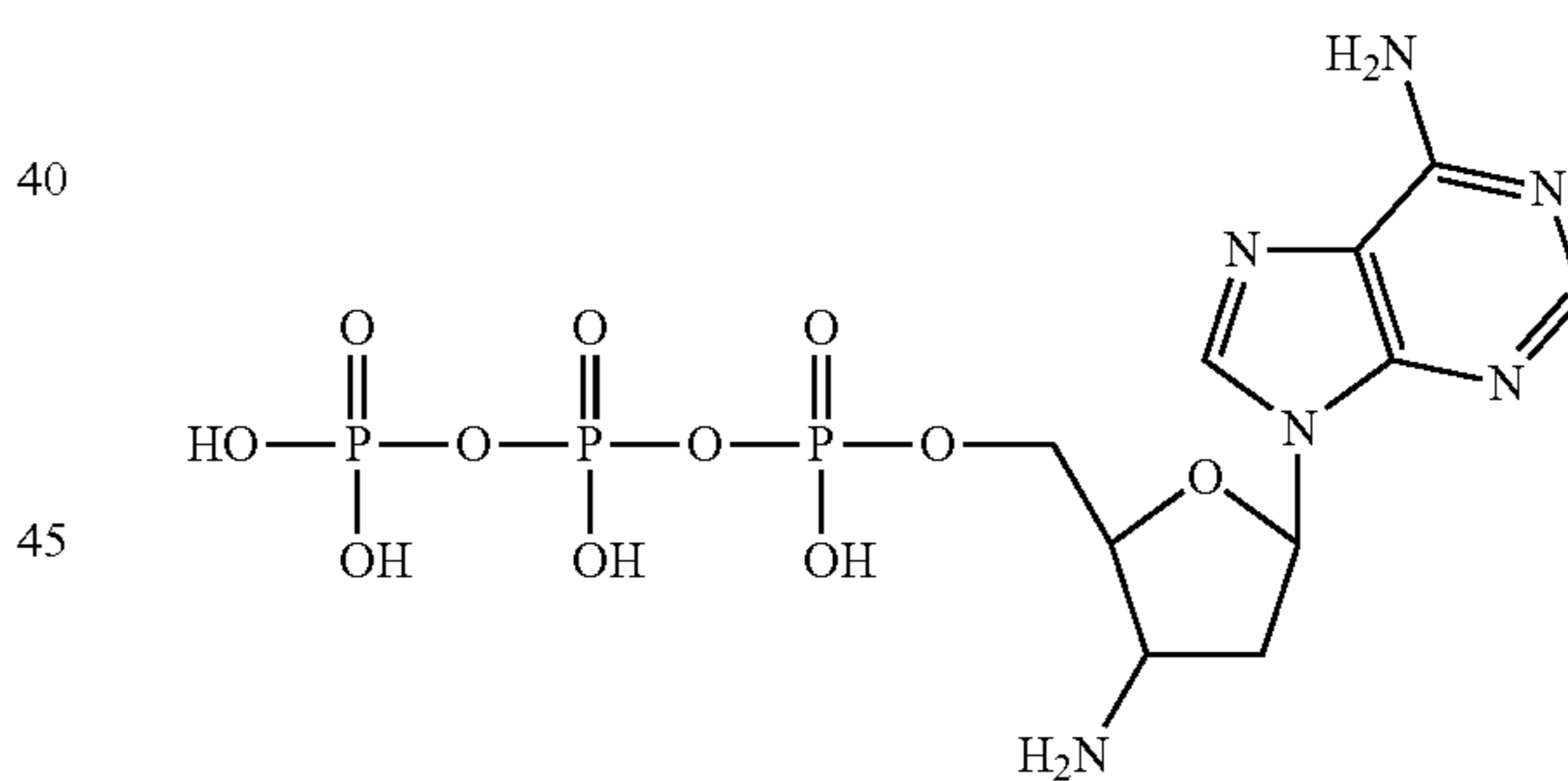
3'-amino-2',3'-dideoxy-adenosine-5'-triphosphate
