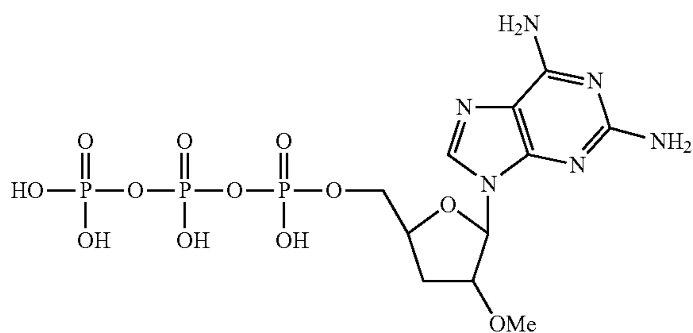
2'-methoxy-2',3'-dideoxy-2-amino-adenosine-5'-triphosphate
