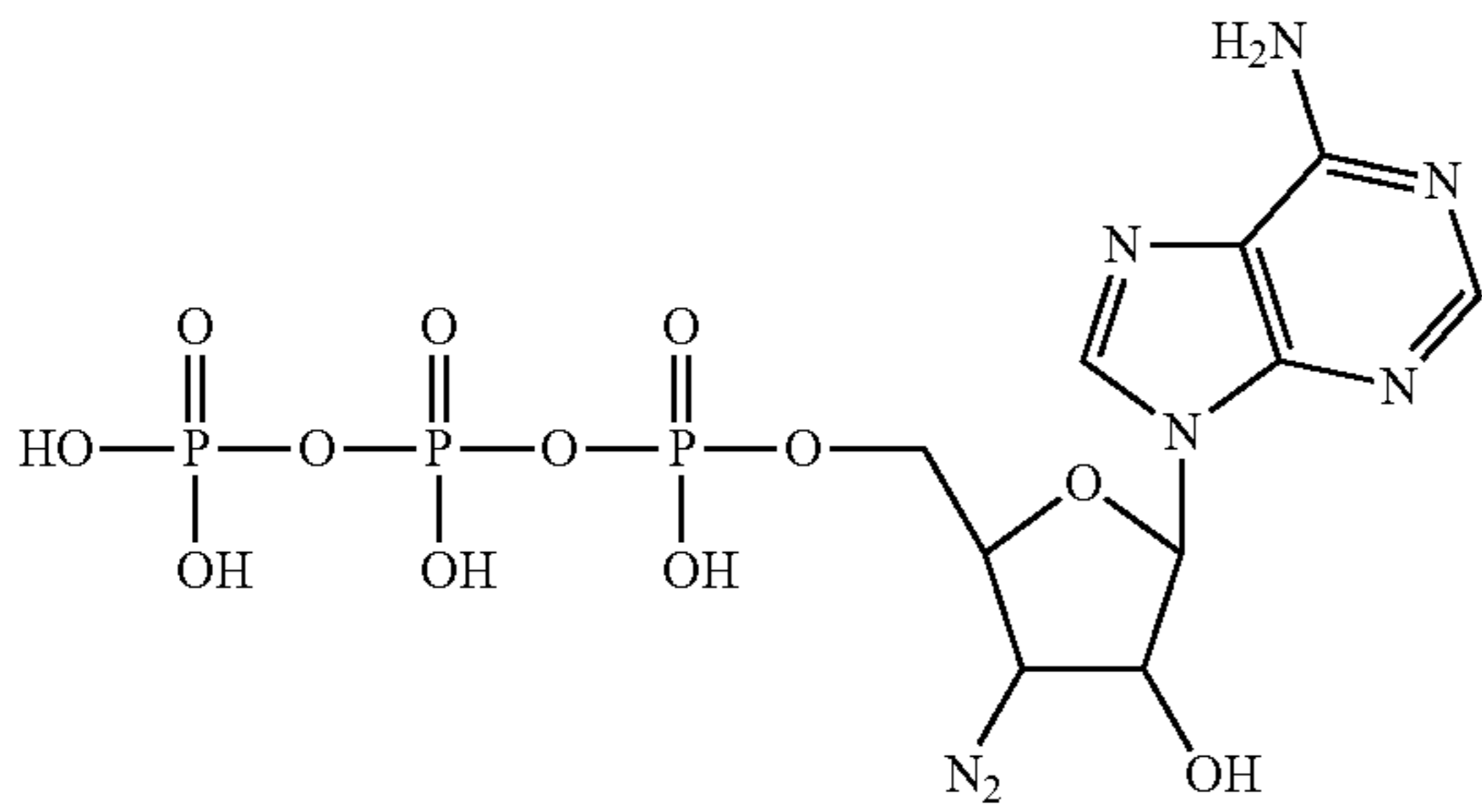
3'-azido-3'-deoxy-adenosine-5'-triphosphate
