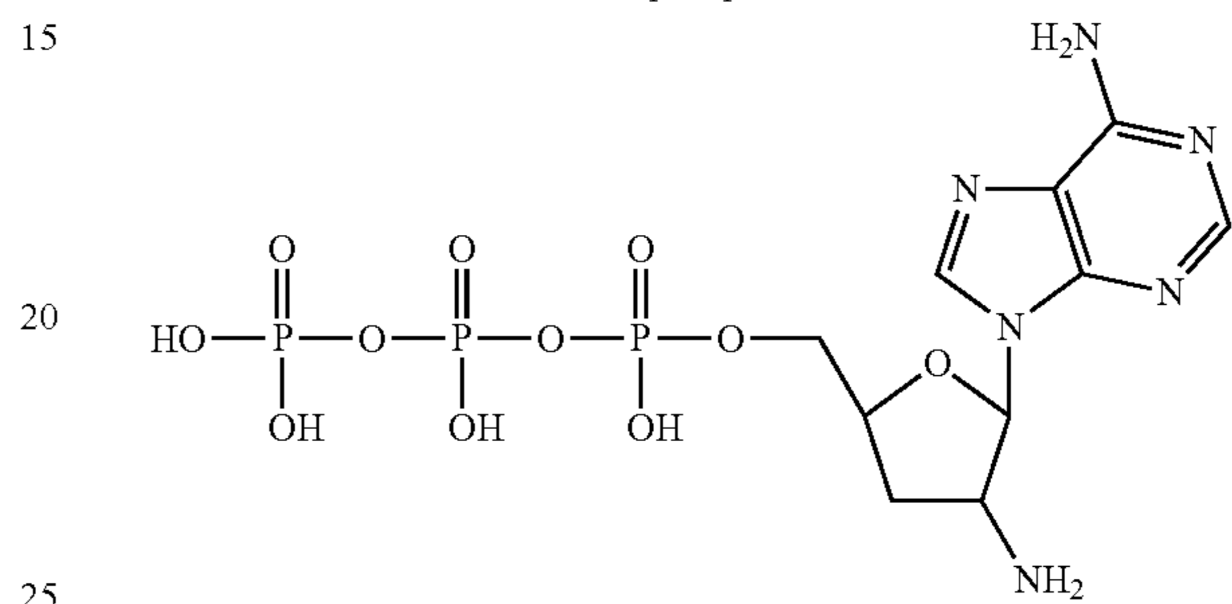
2'-amino-2',3'-dideoxy-adenosine-5'-triphosphate
