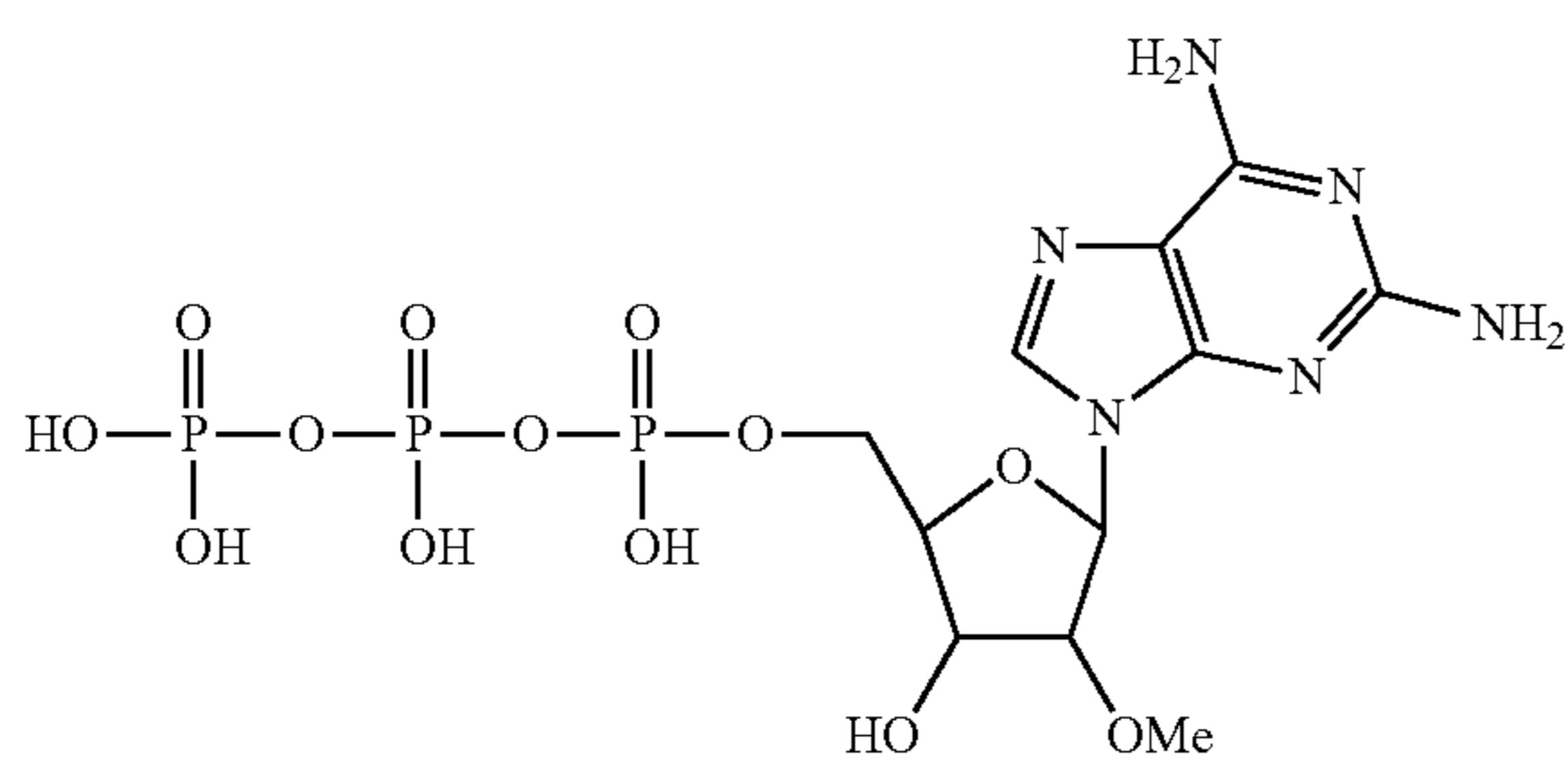
2'-methoxy-2'-deoxy-2-amino-adenosine-5'-triphosphate
