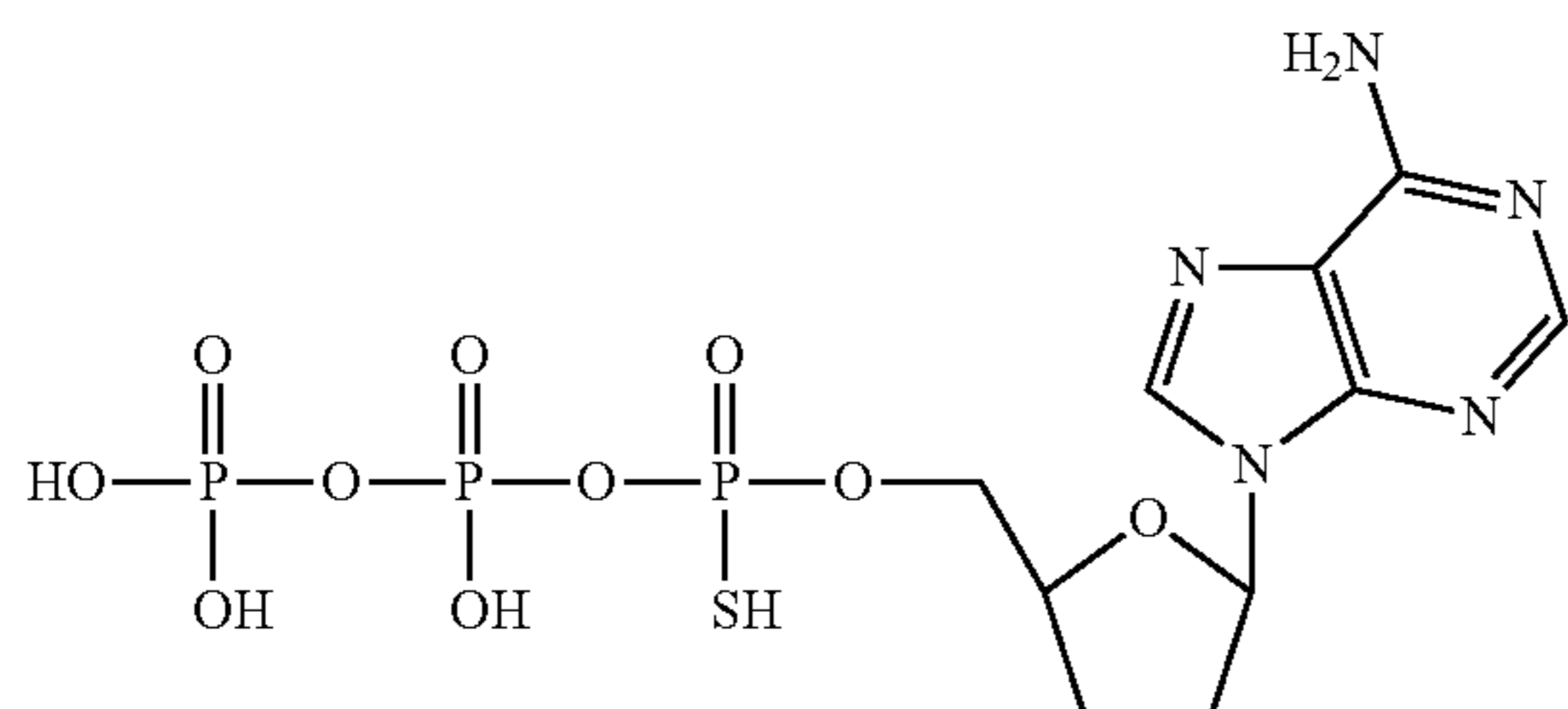
5'-alpha-thio-2',3'-dideoxyadenosine-5'-triphosphate
