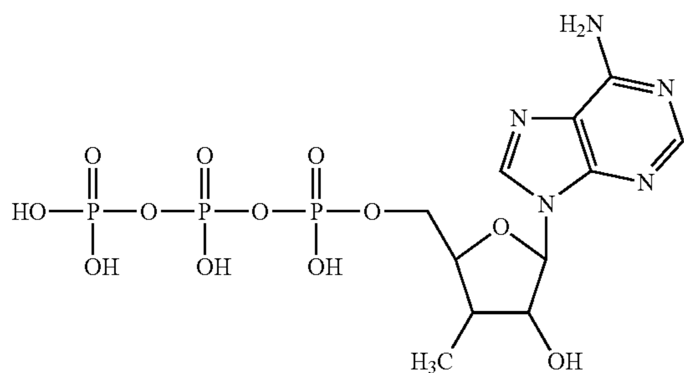
3'-methyl-3'-deoxyadenosine-5'-triphosphate
