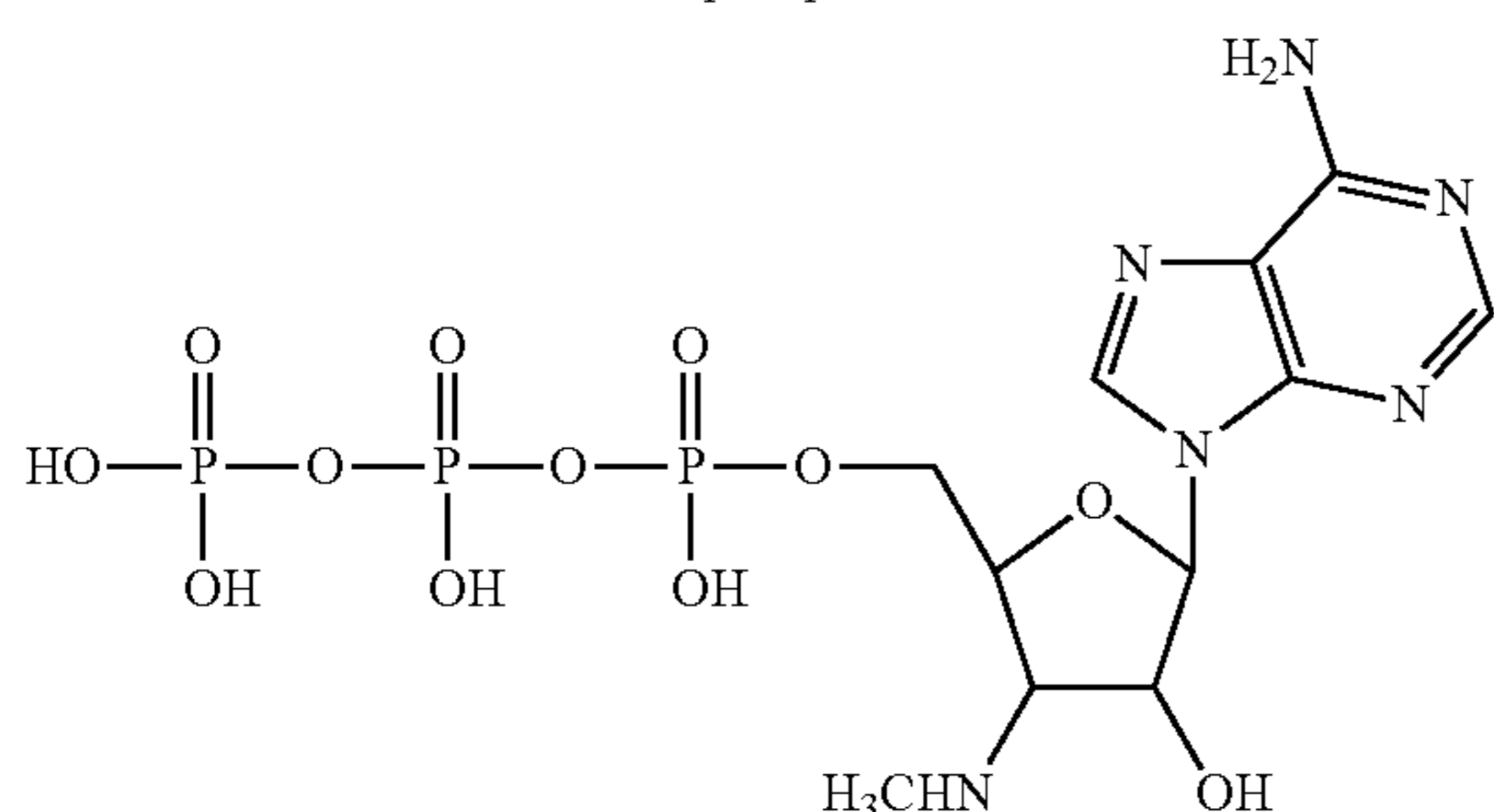
3'-methylamino-3'-deoxyadenosine-5'-triphosphate
