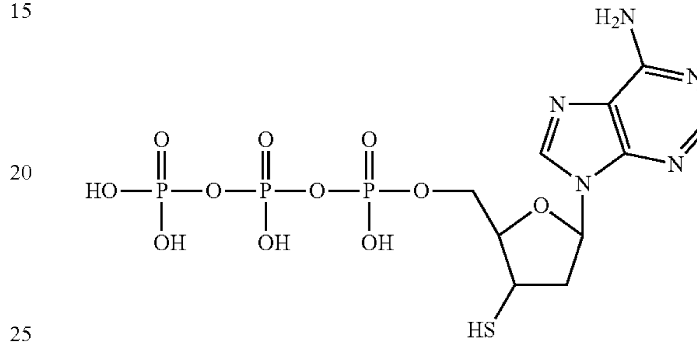
3'-thio-2',3'-dideoxyadenosine-5'-triphosphate
