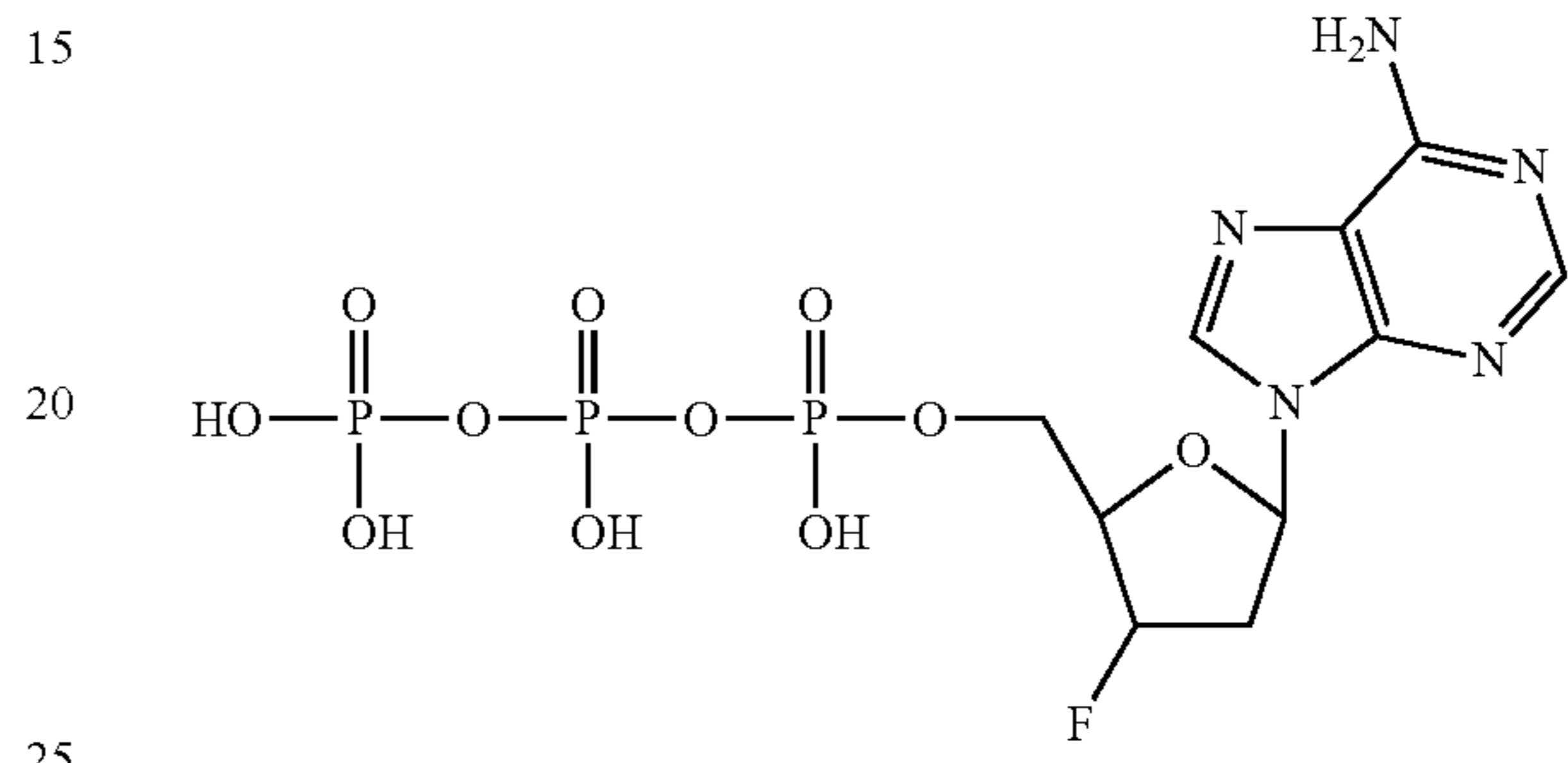
3'-fluoro-2',3'-dideoxy-adenosine-5'-triphosphate
