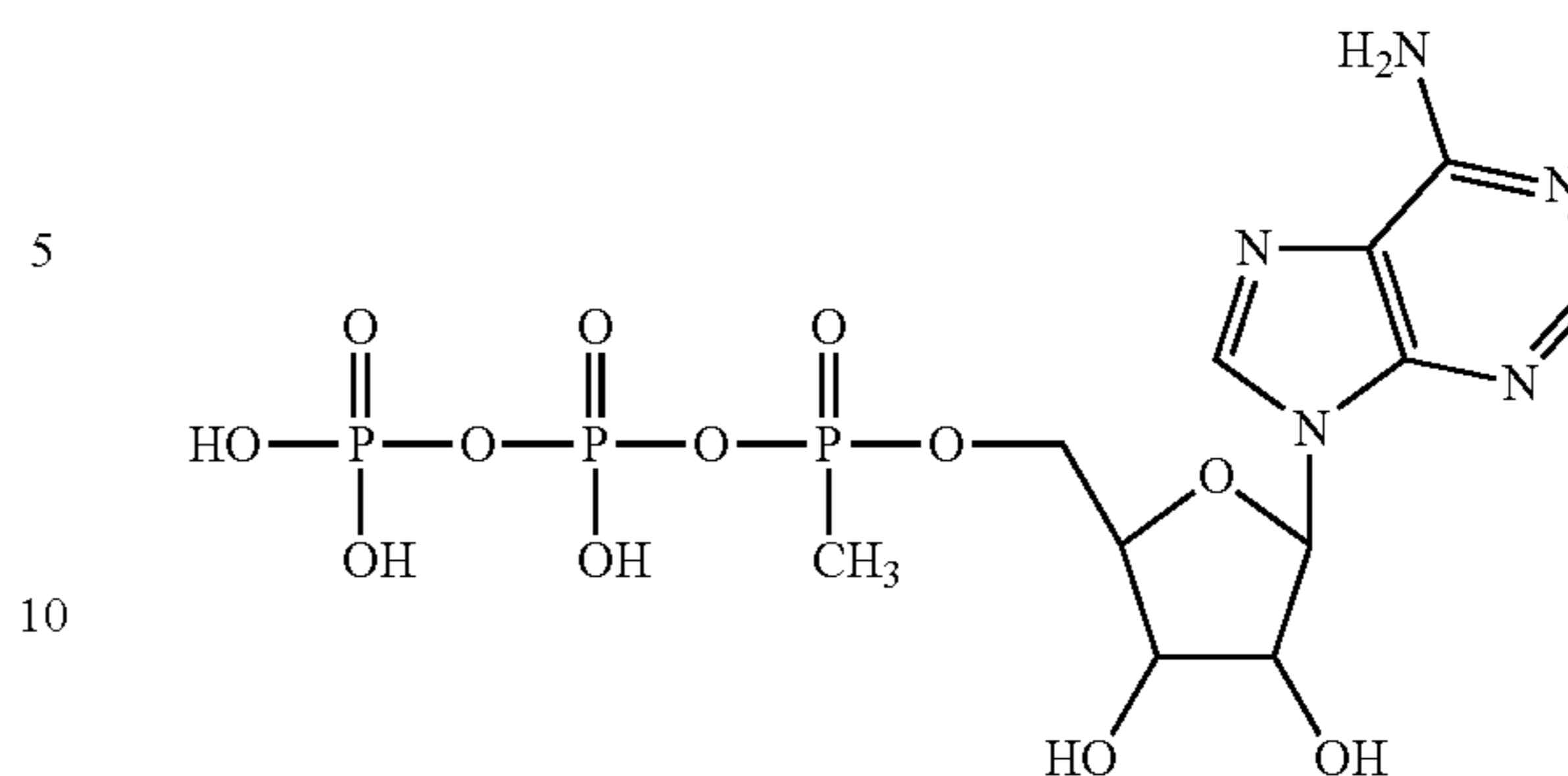
5'-alpha-methylphosphonate-adenosine-5'-triphosphate
