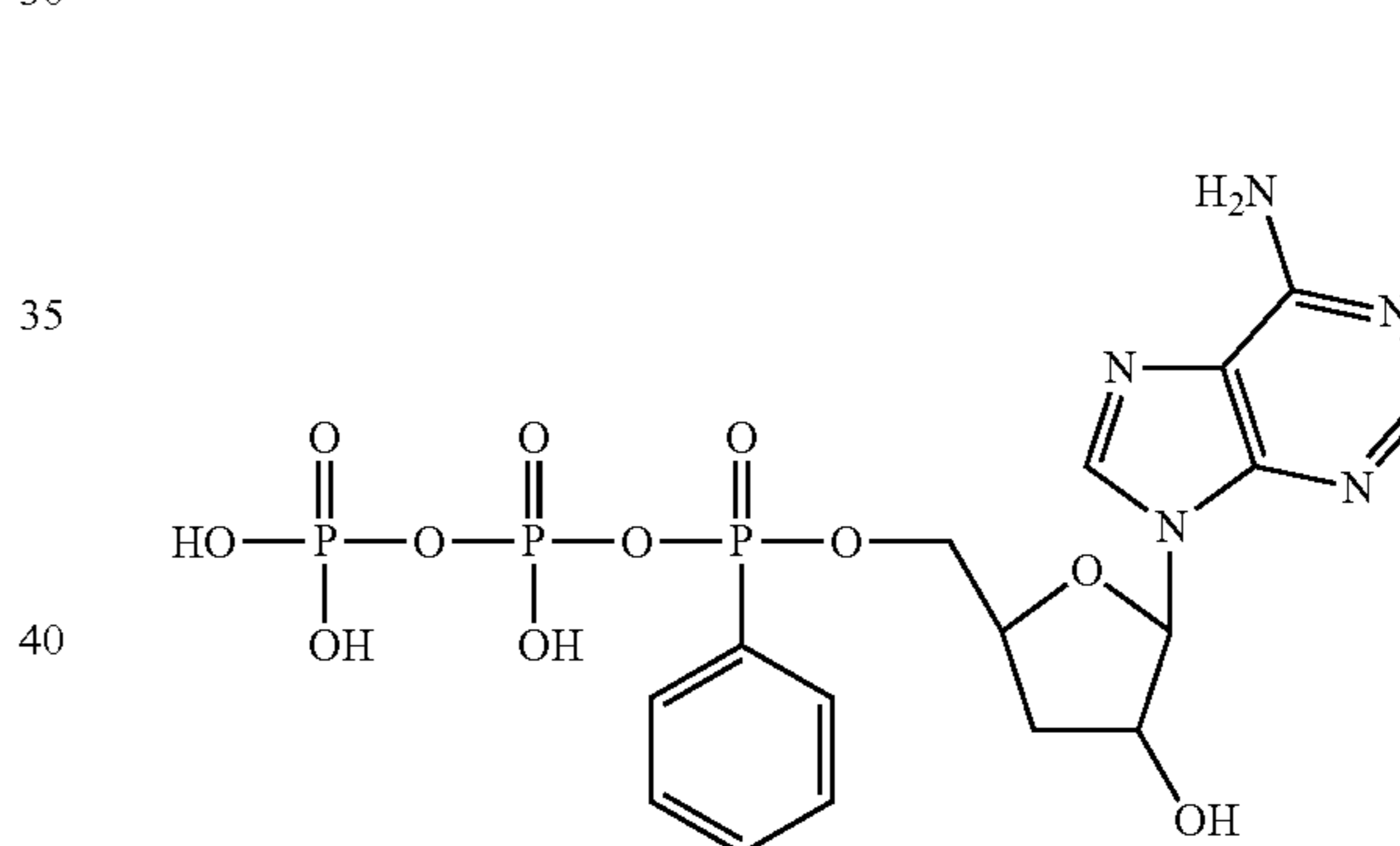
5'-alpha-phenylphosphonate-3'-deoxyadenosine-5'-triphosphate
