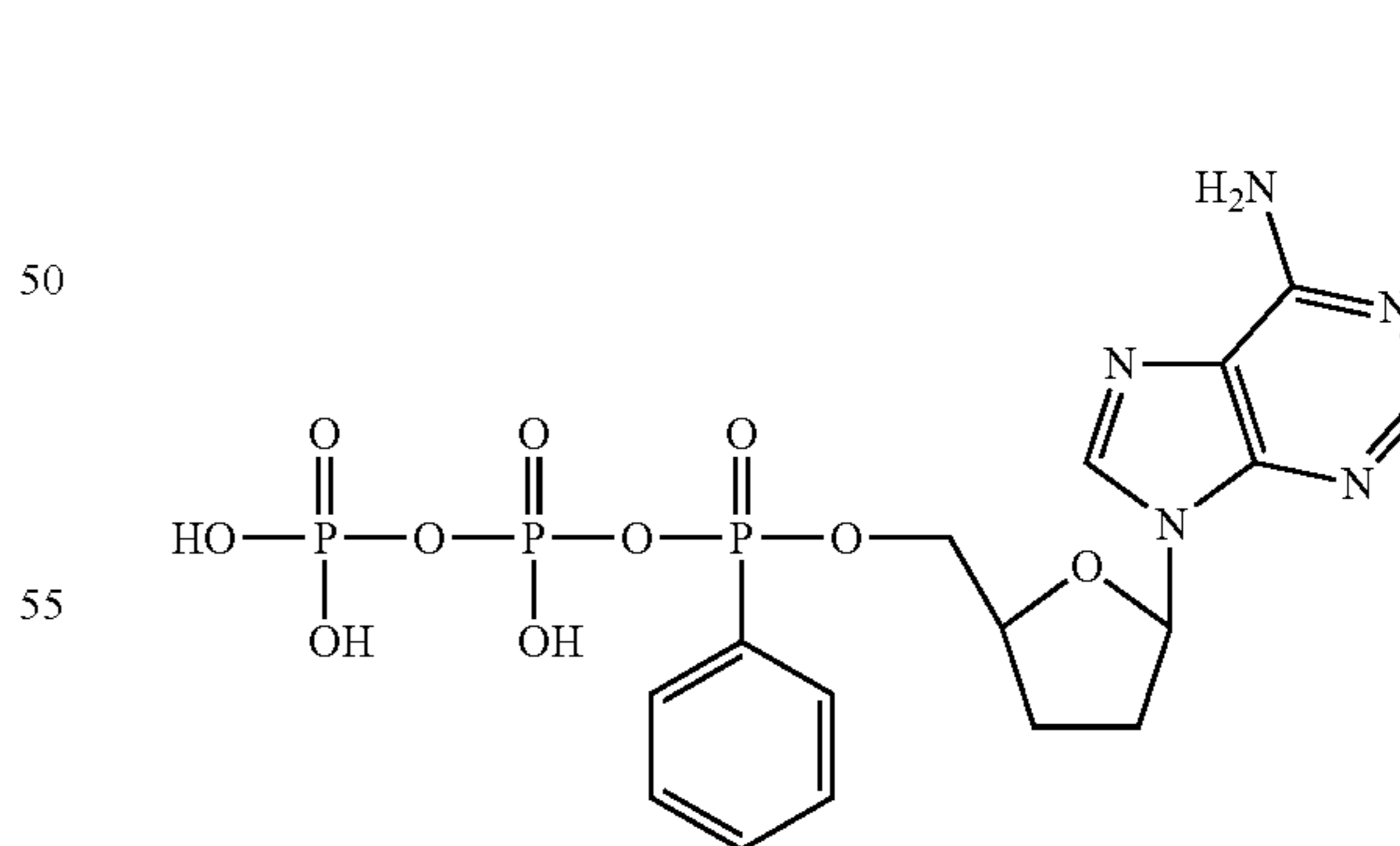
5'-alpha-phenylphosphonate-2',3'-dideoxyadenosine-5'-triphosphate
