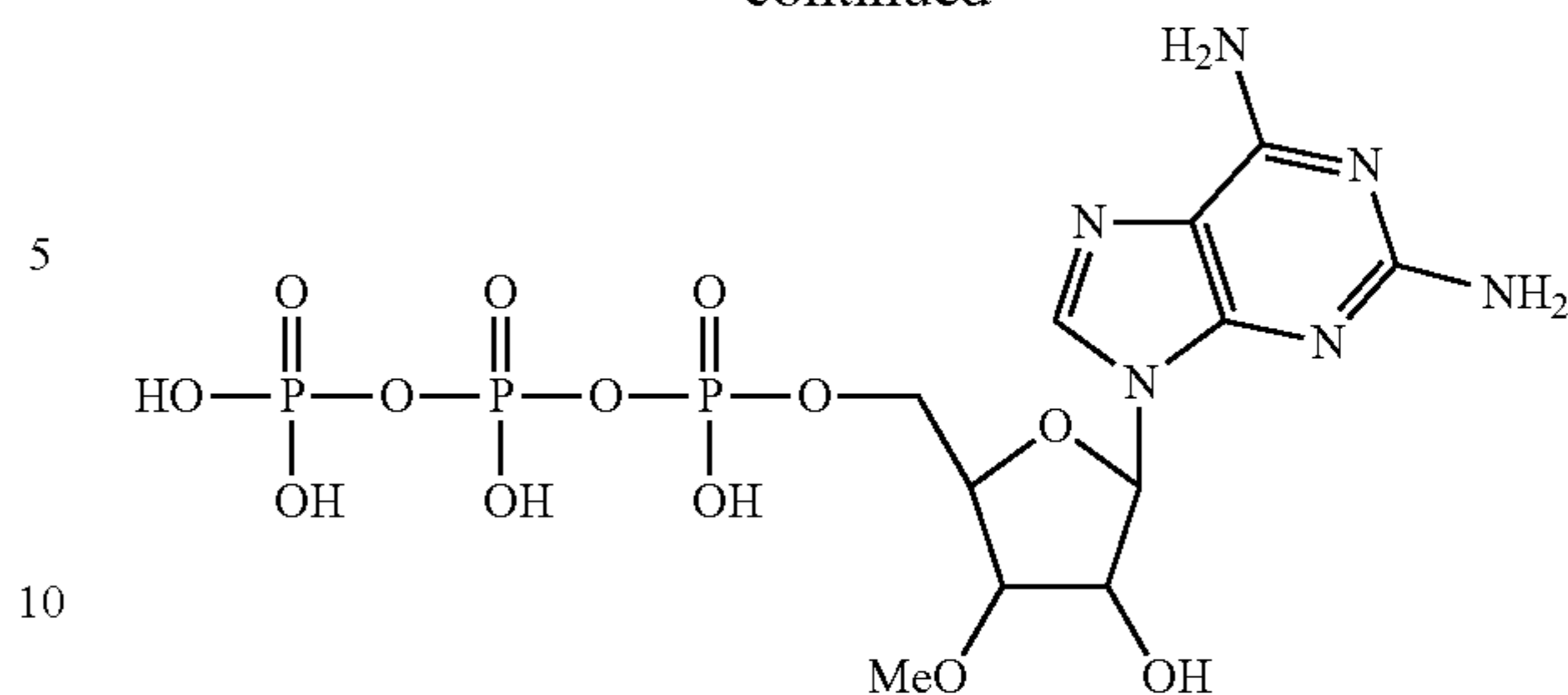
3'-methoxy-3'-deoxy-2-aminoadenosine-5'-triphosphate
