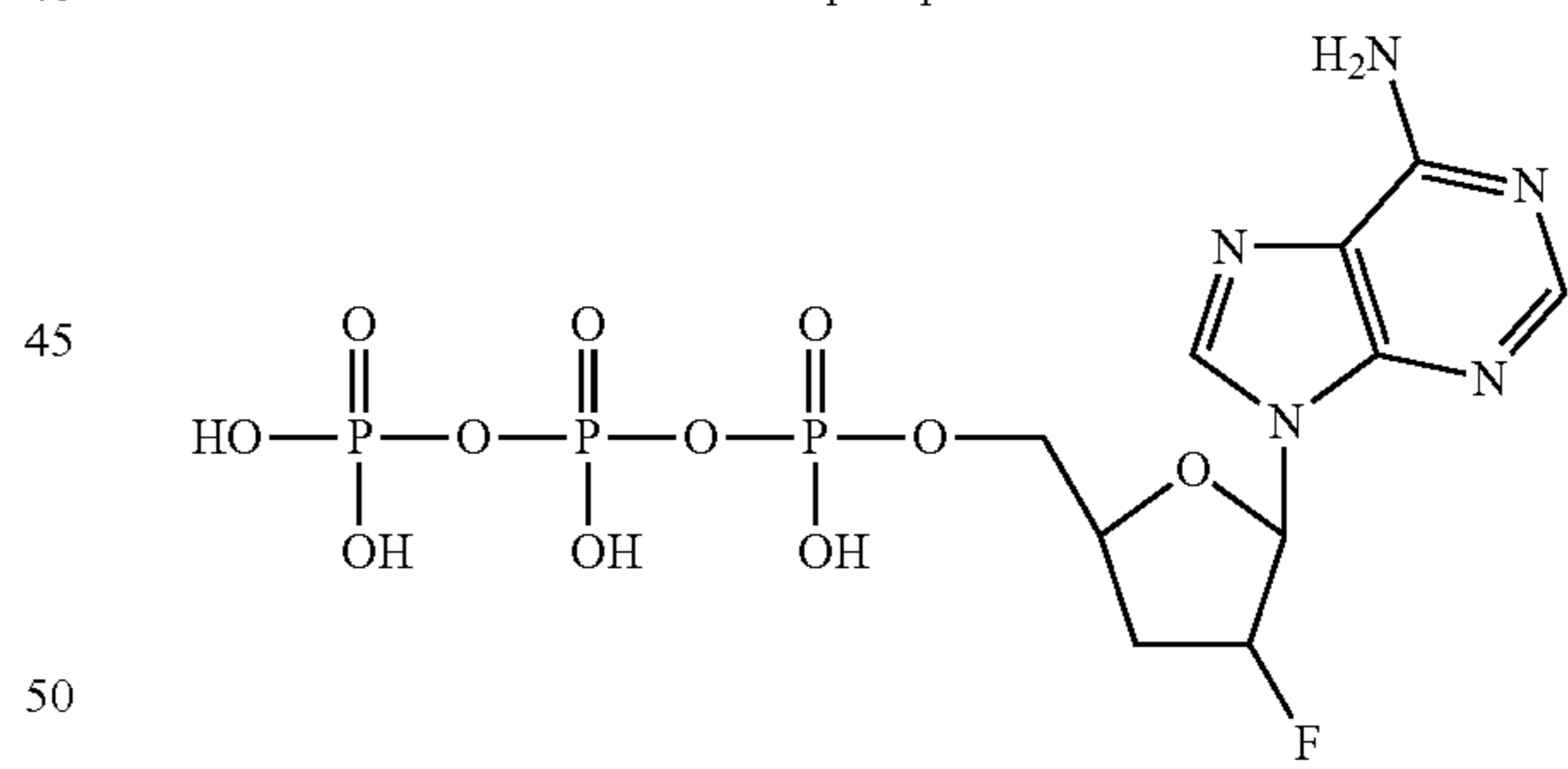
2'-fluoro-2',3'-dideoxy-adenosine-5'-triphosphate
