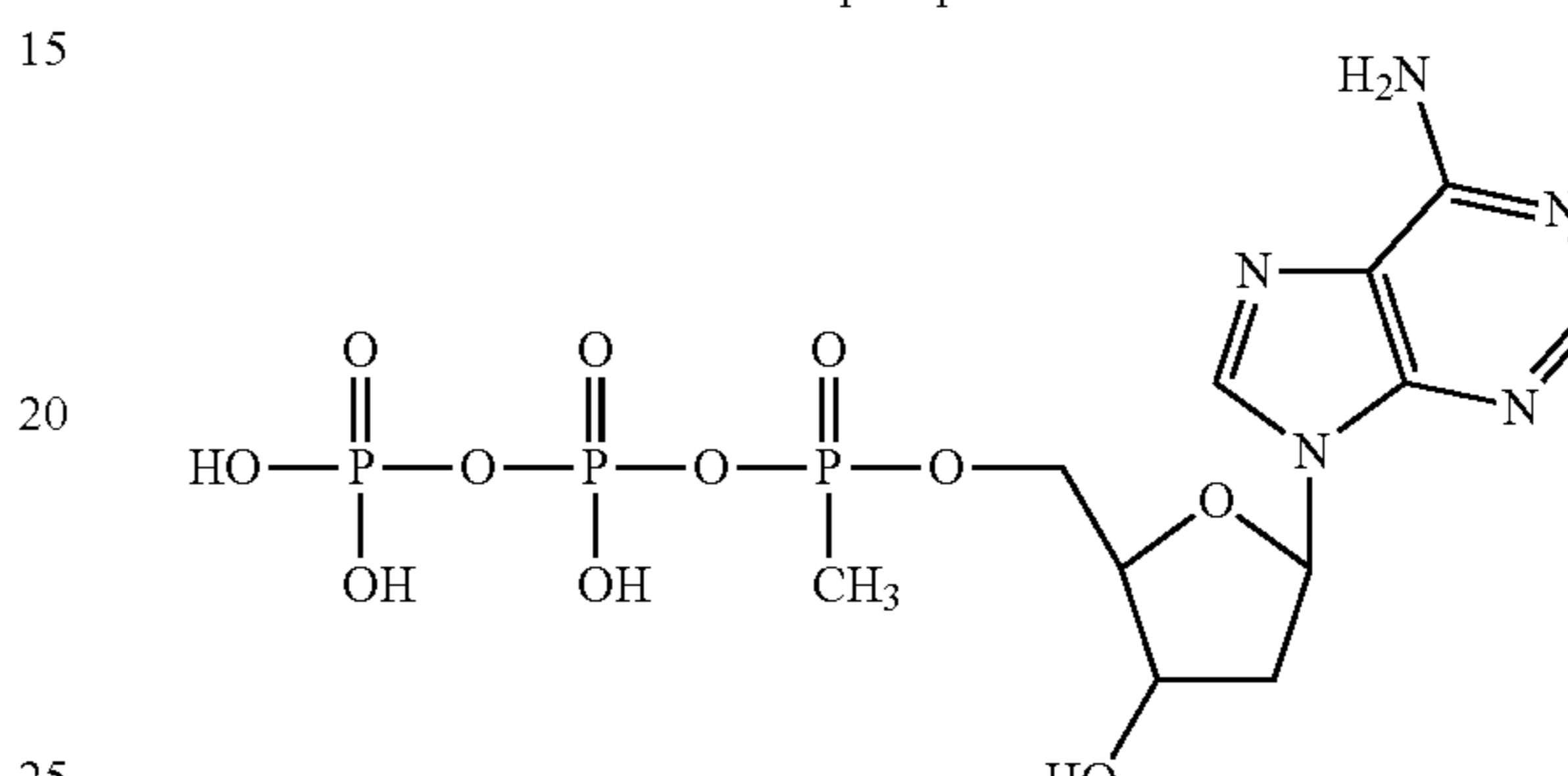
5'-alpha-methylphosphonate-2'-deoxyadenosine-5'-triphosphate
