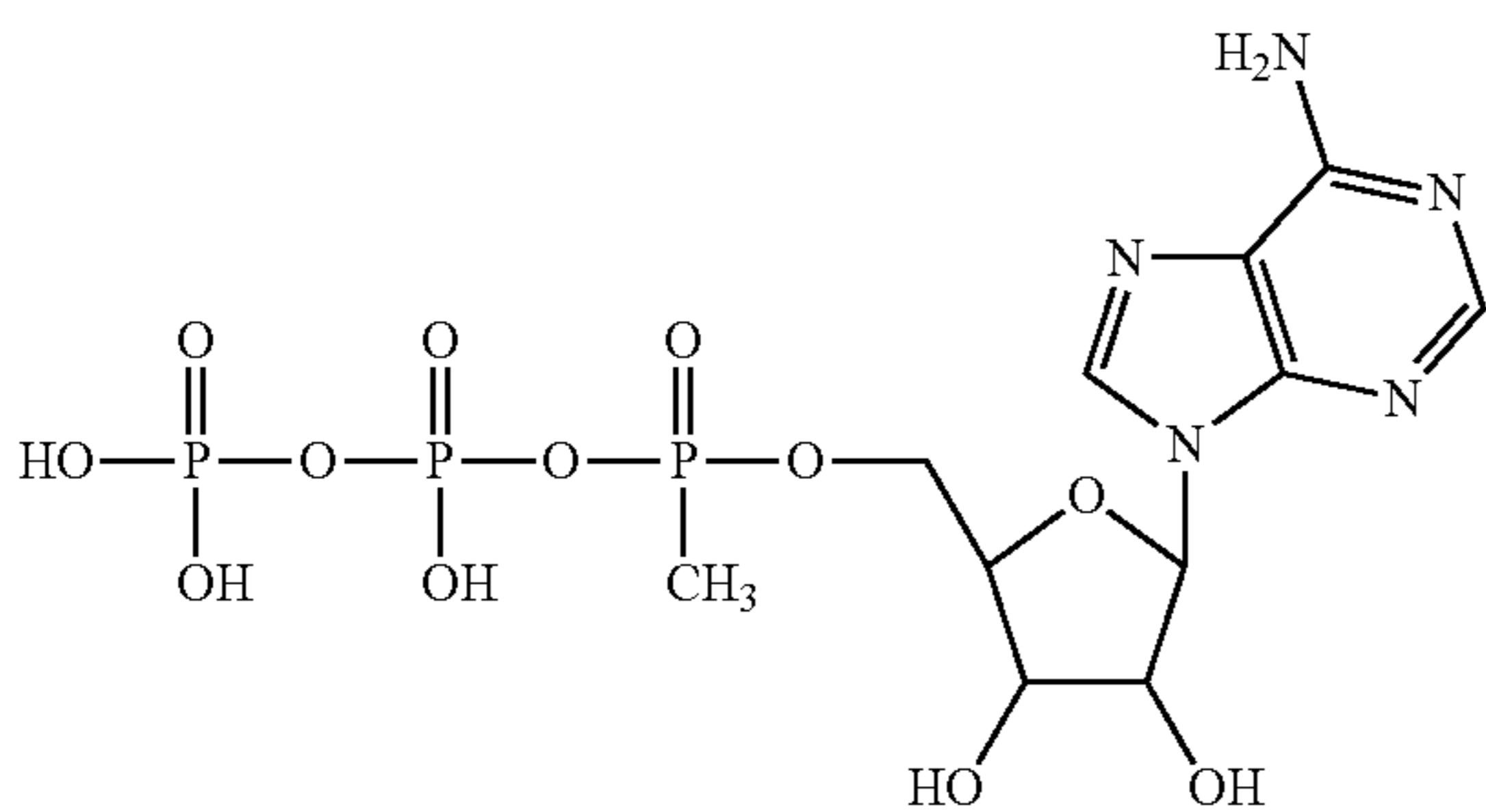
5'-alpha-methylphosphonate-adenosine-5'-triphosphate
