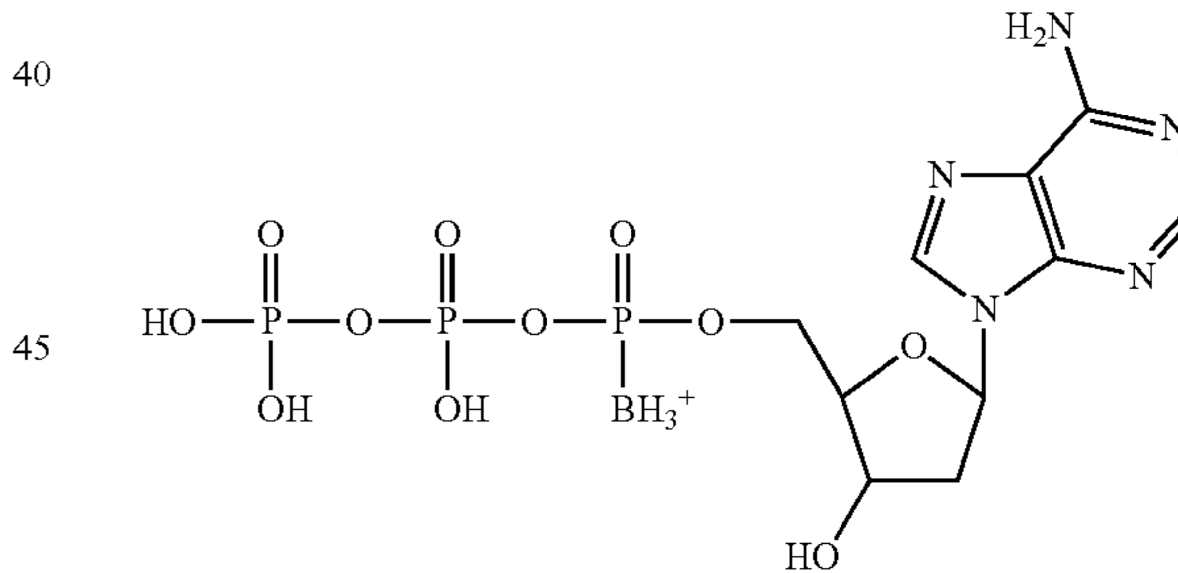
5'-alpha-[P-borano]-2'-deoxyadenosine-5'-triphosphate
