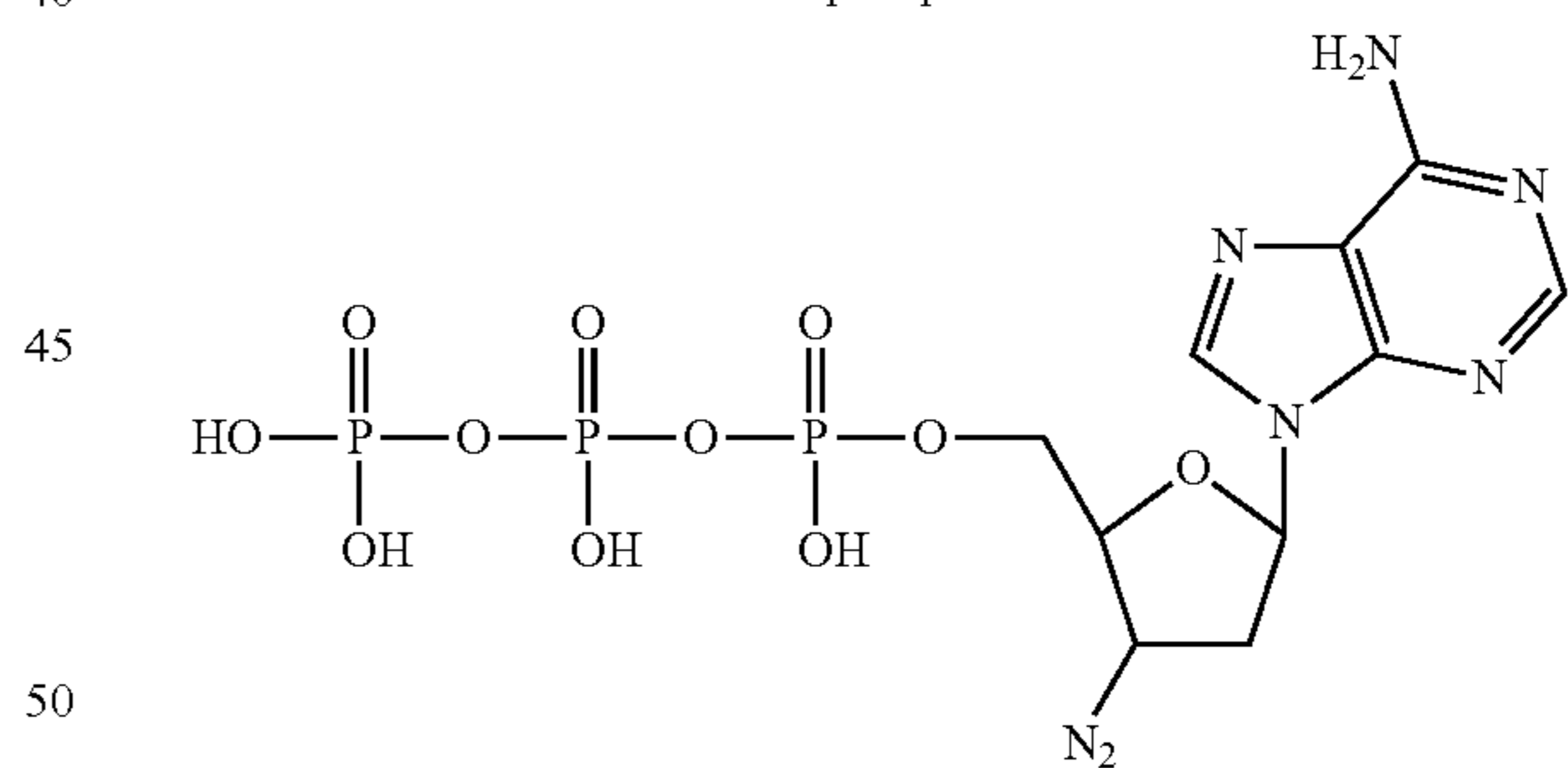
3'-azido-2',3'-dideoxy-adenosine-5'-triphosphate
