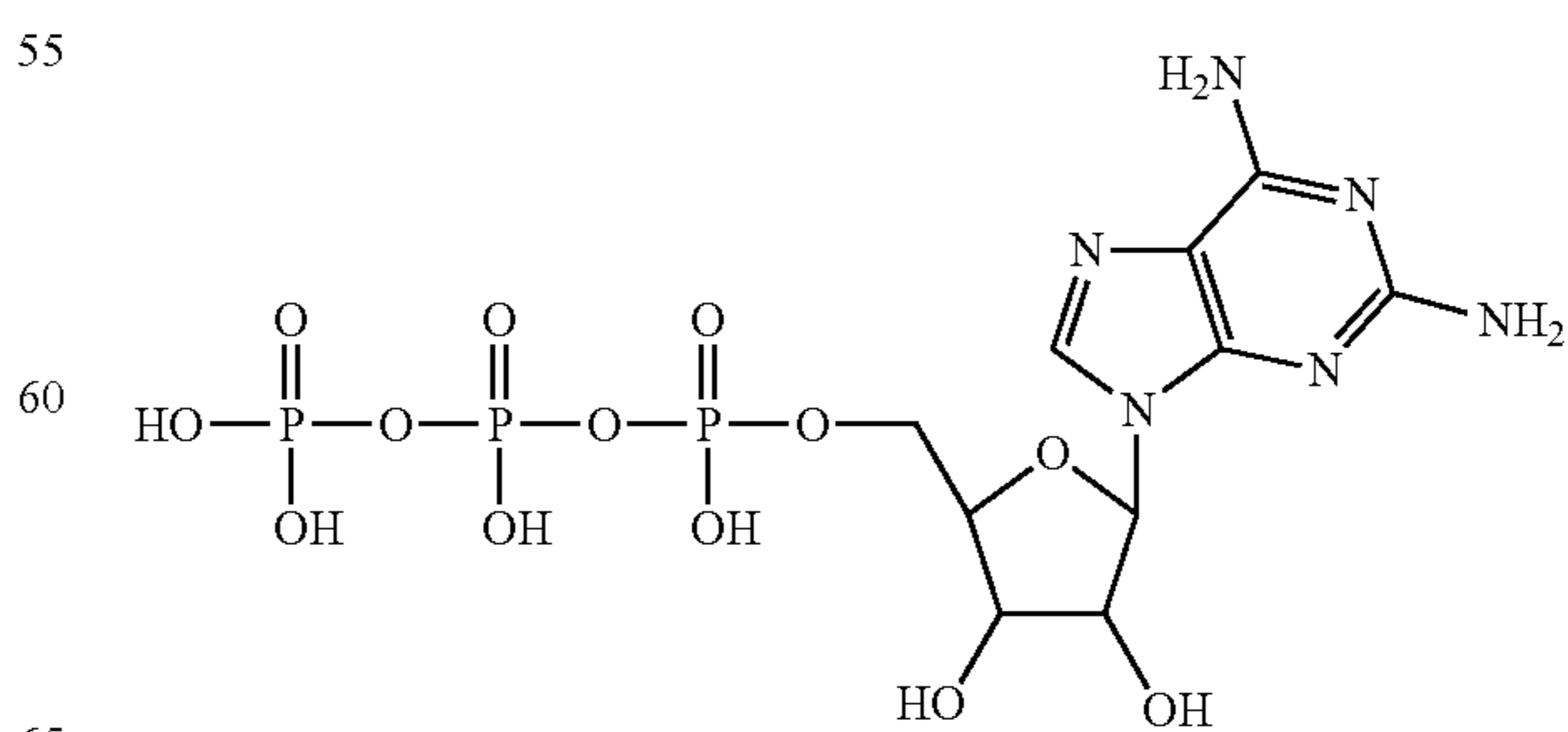
2-amino-adenosine-5'-triphosphate
