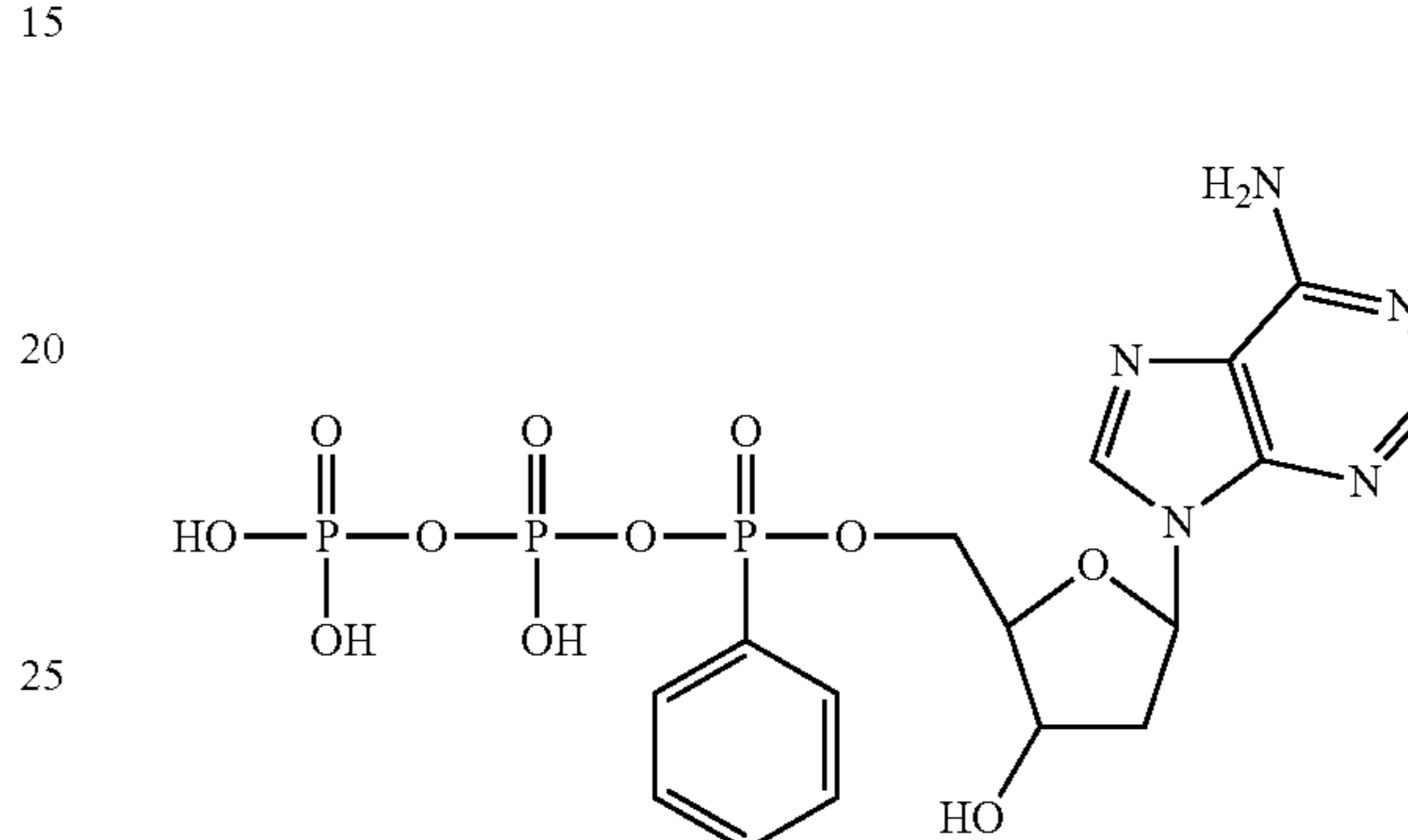
5'-alpha-phenylphosphonate-2'-deoxyadenosine-5'-triphosphate
