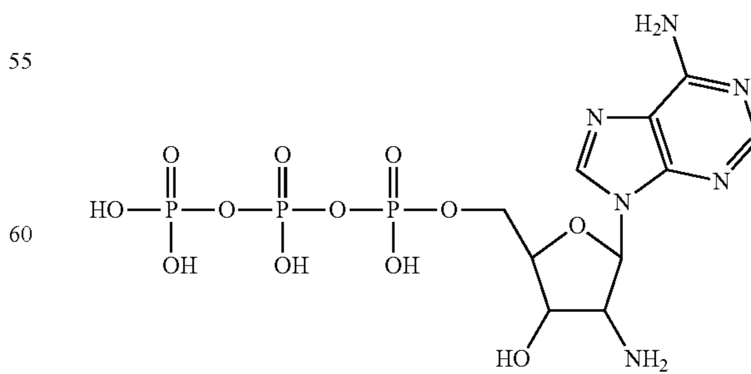
2'-amino-2'-deoxy-adenosine-5'-triphosphate
