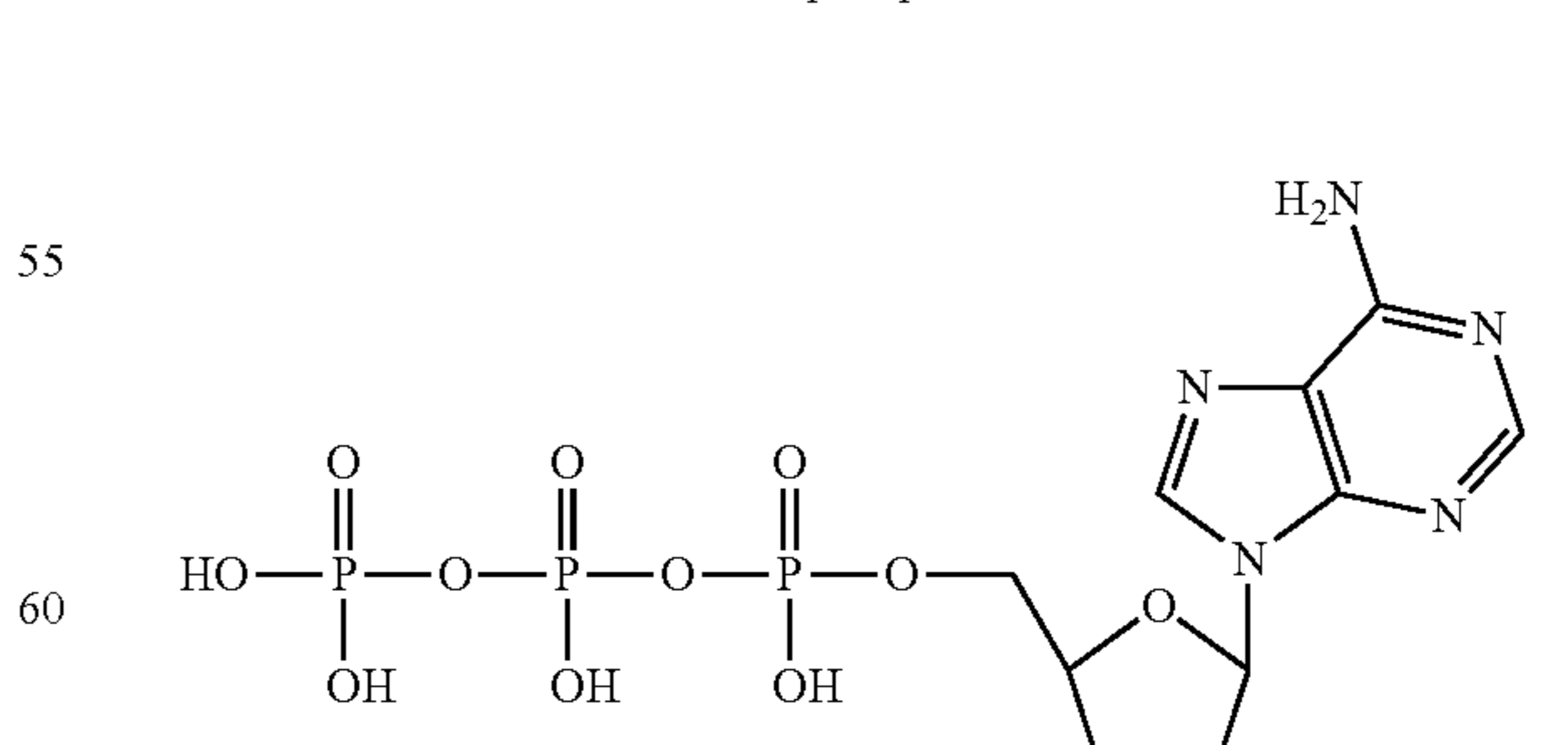
2'-methoxy-2',3'-dideoxyadenosine-5'-triphosphate
