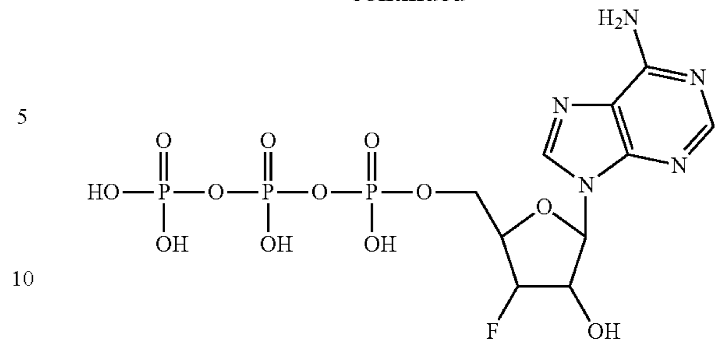
3'-fluoro-3'-deoxy-adenosine-5'-triphosphate
