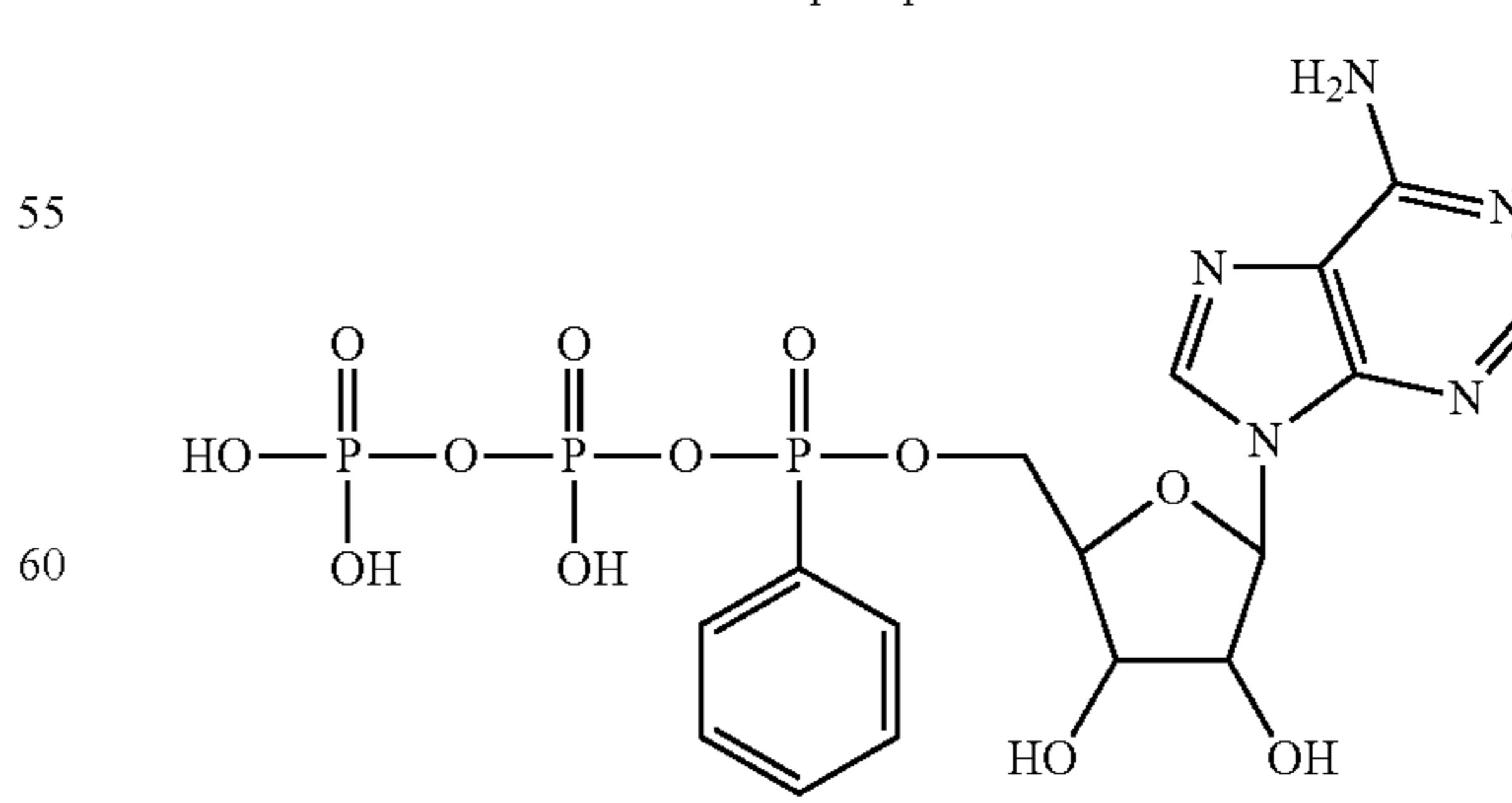
5'-alpha-phenylphosphonate-adenosine-5'-triphosphate
