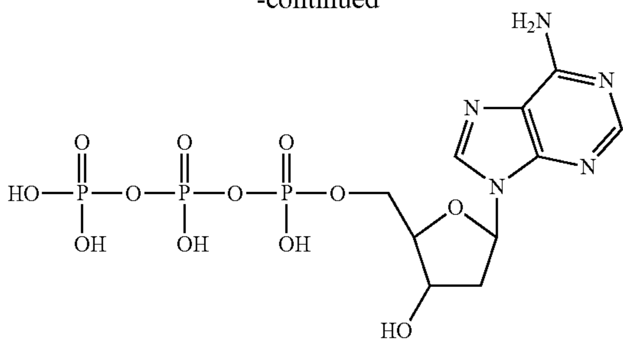
2'-deoxy-adenosine- 5'-triphosphate
