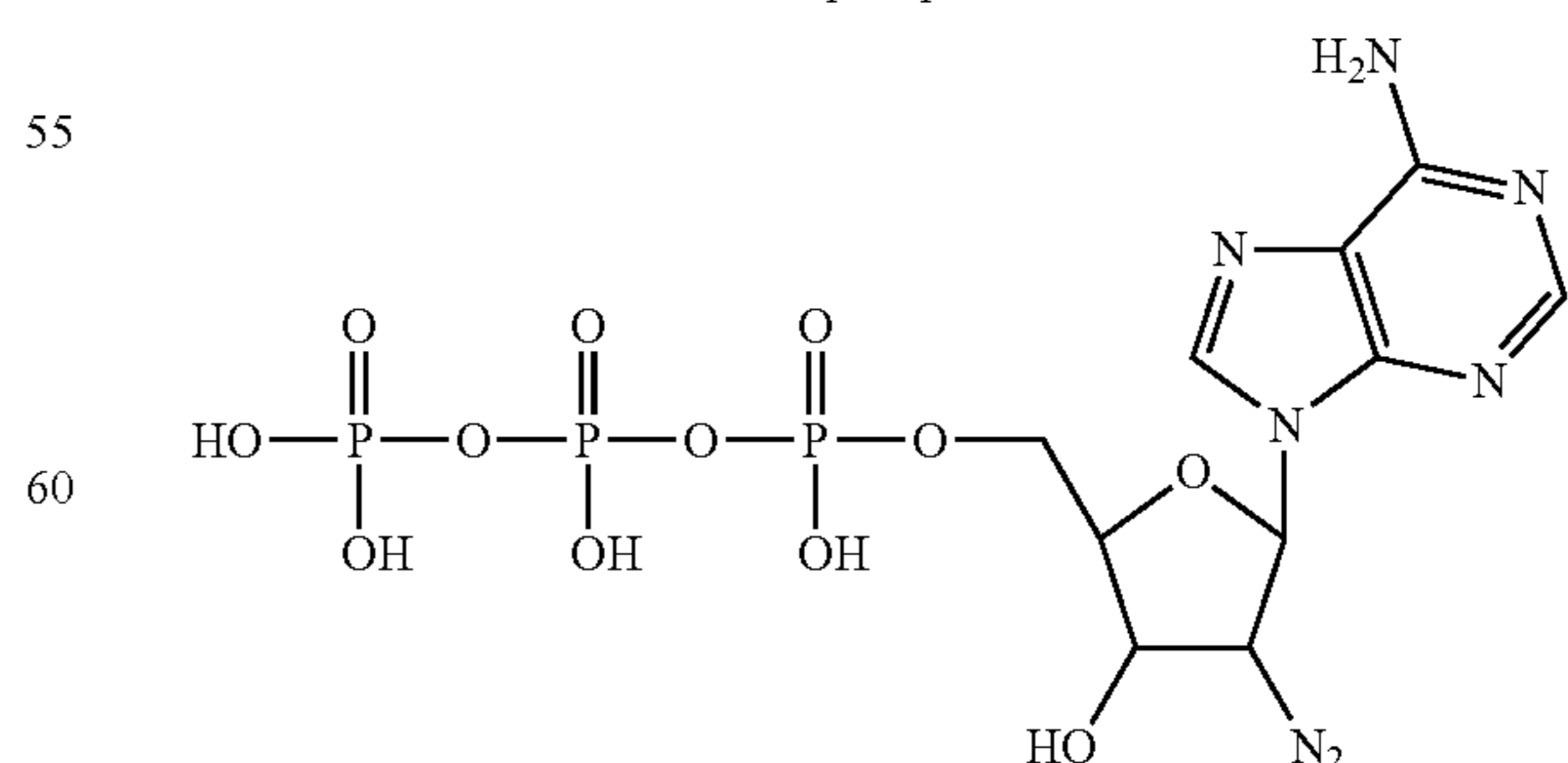
2'-azido-2'-deoxy-adenosine-5'-triphosphate
