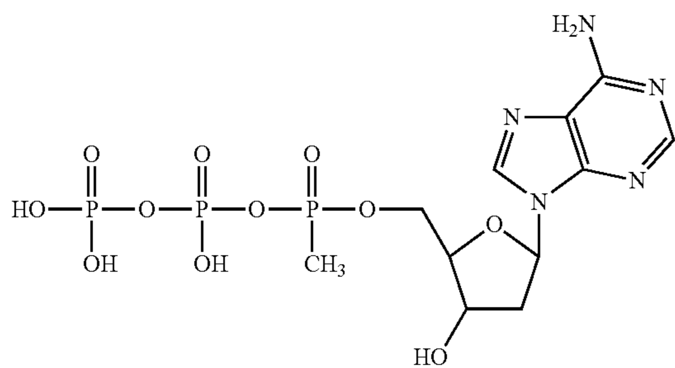
5'-alpha-methylphosphonate-2'-deoxyadenosine-5'-triphosphate
