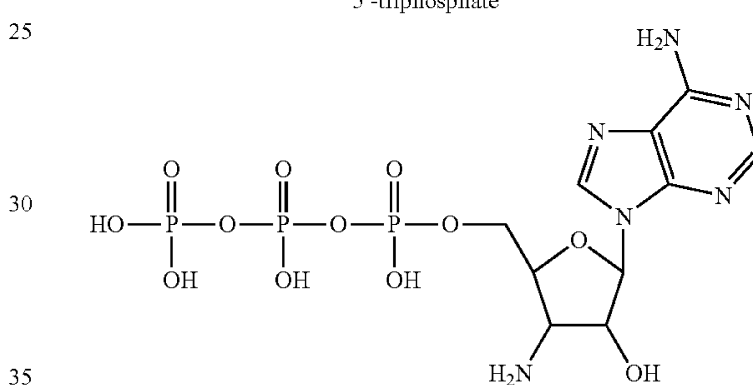
3'-amino-3'-deoxy-adenosine-5'-triphosphate
