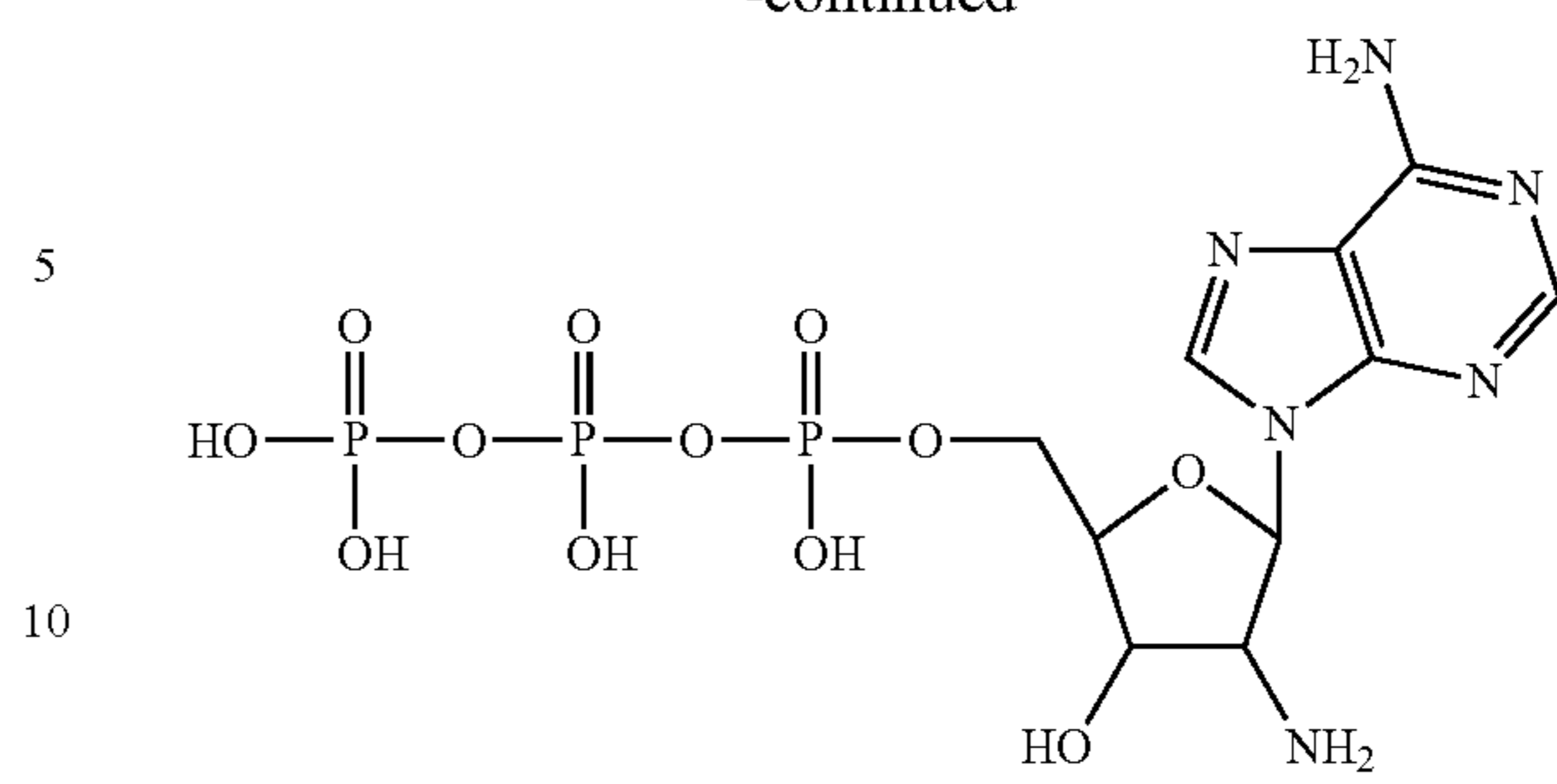
2'-amino-2'-deoxy-adenosine-5'-triphosphate
