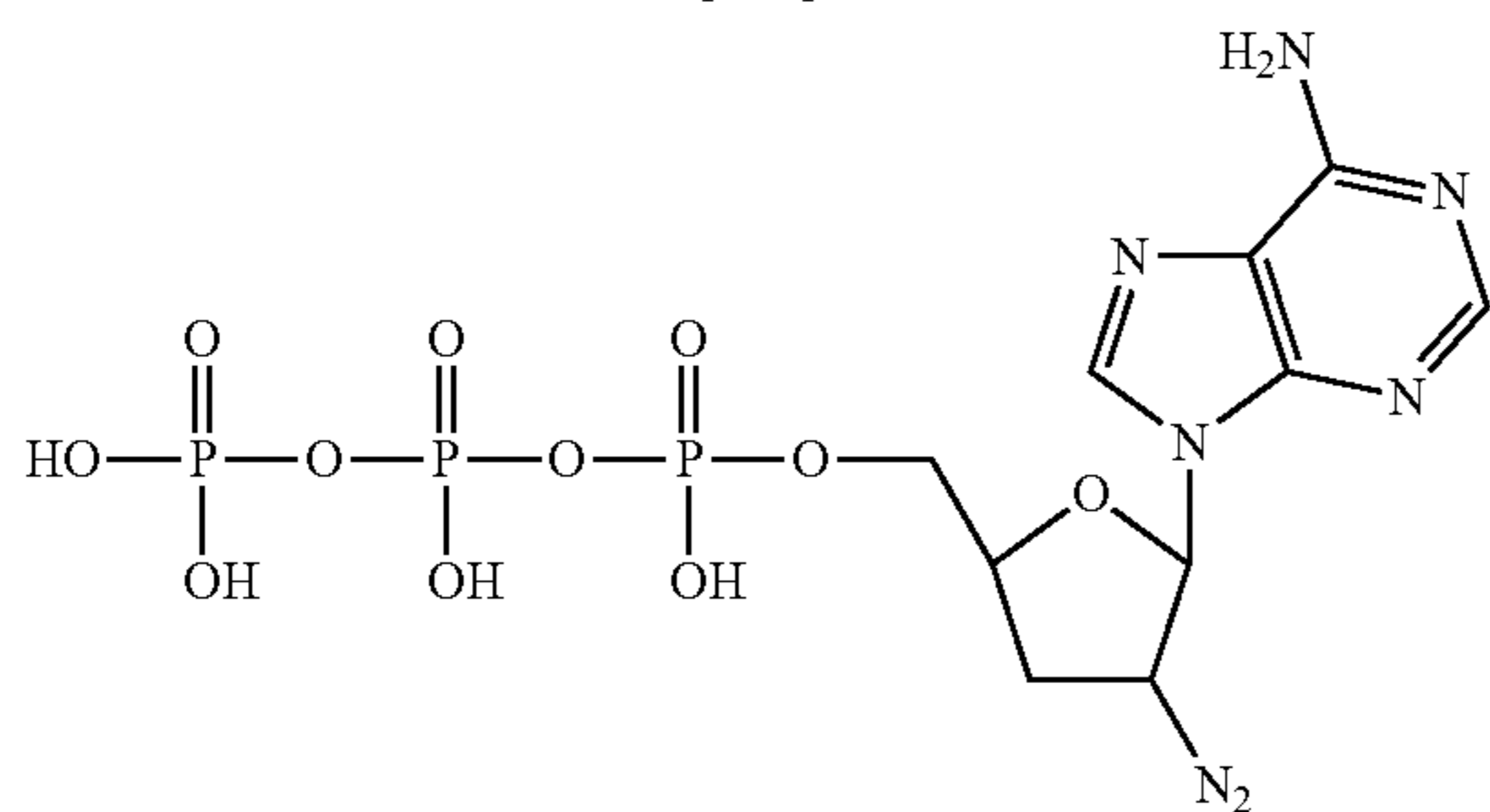
2'-azido-2',3'-dideoxy-adenosine-5'-triphosphate
