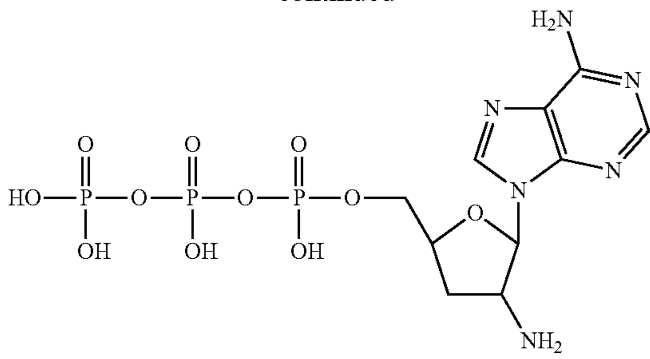
2'-amino-2',3'-dideoxy-adenosine-5'-triphosphate
