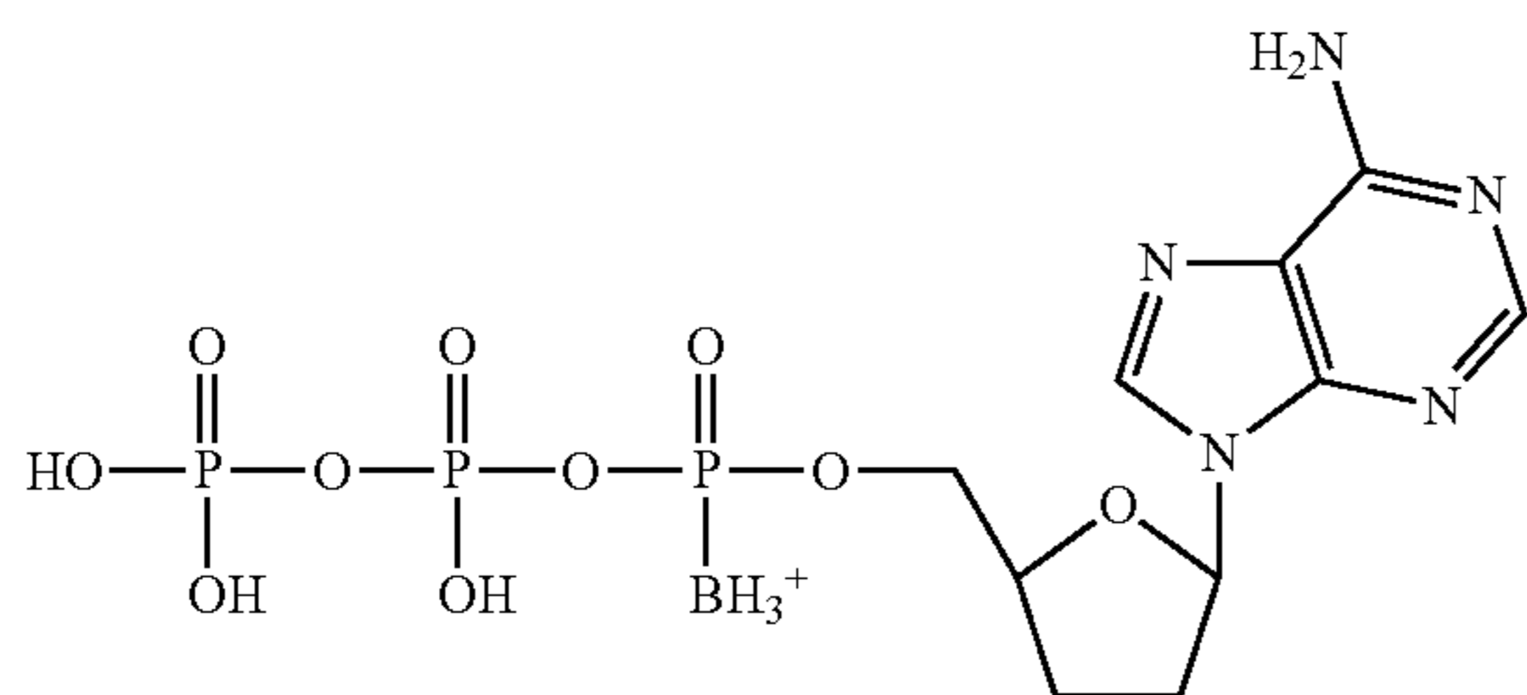
5'-alpha-[P-borano]-3'-deoxyadenosine-5'-triphosphate
