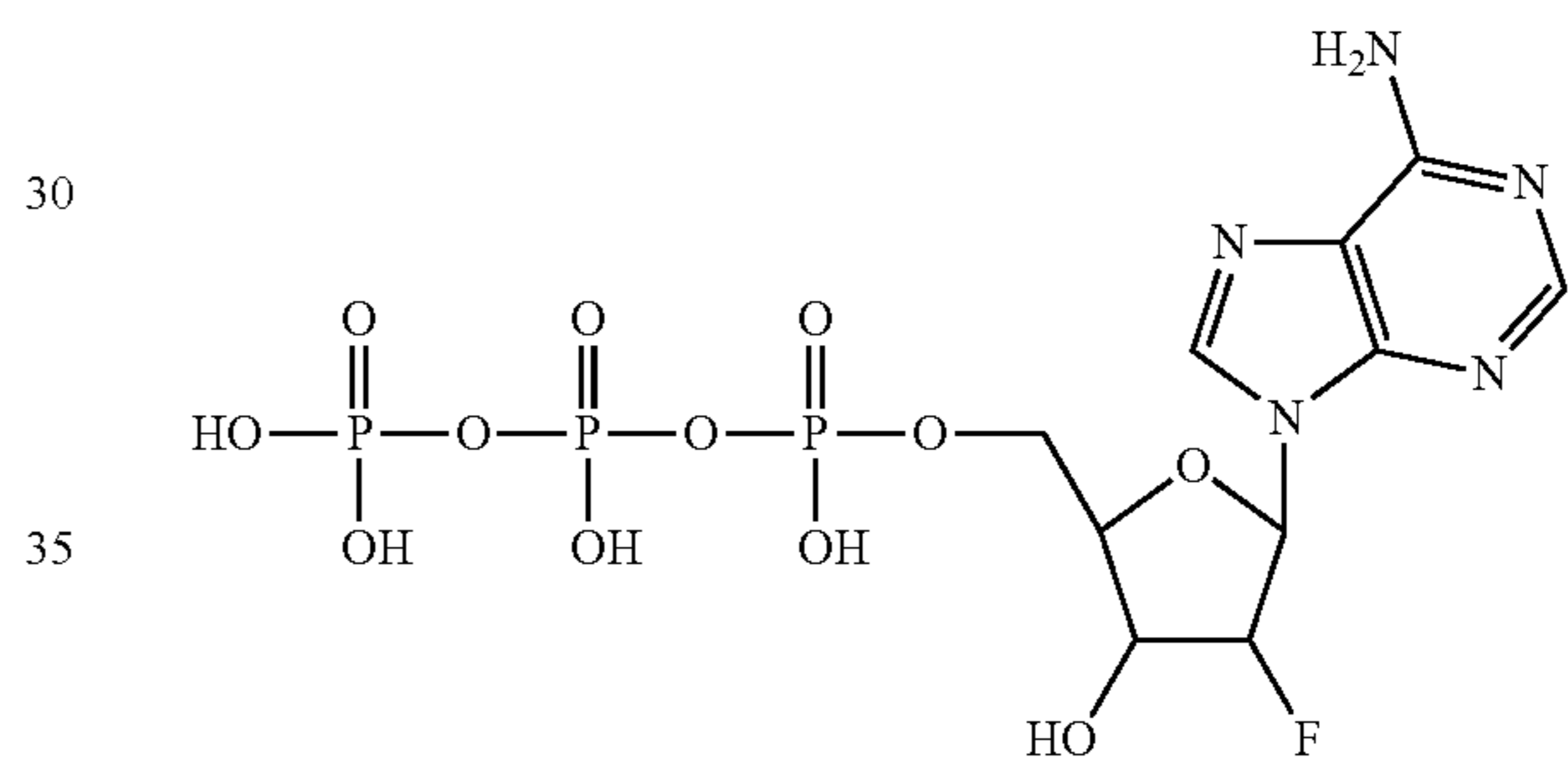
2'-fluoro-2'-deoxy-adenosine-5'-triphosphate
