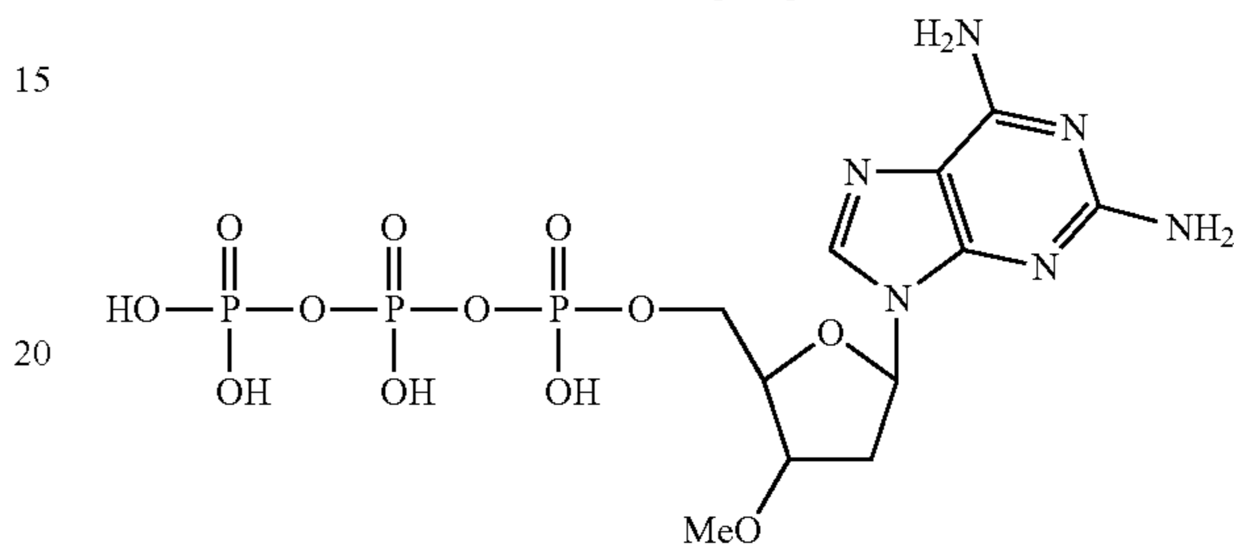
3'-methoxy-2',3'-dideoxy-2-aminoadenosine-5'-triphosphate
