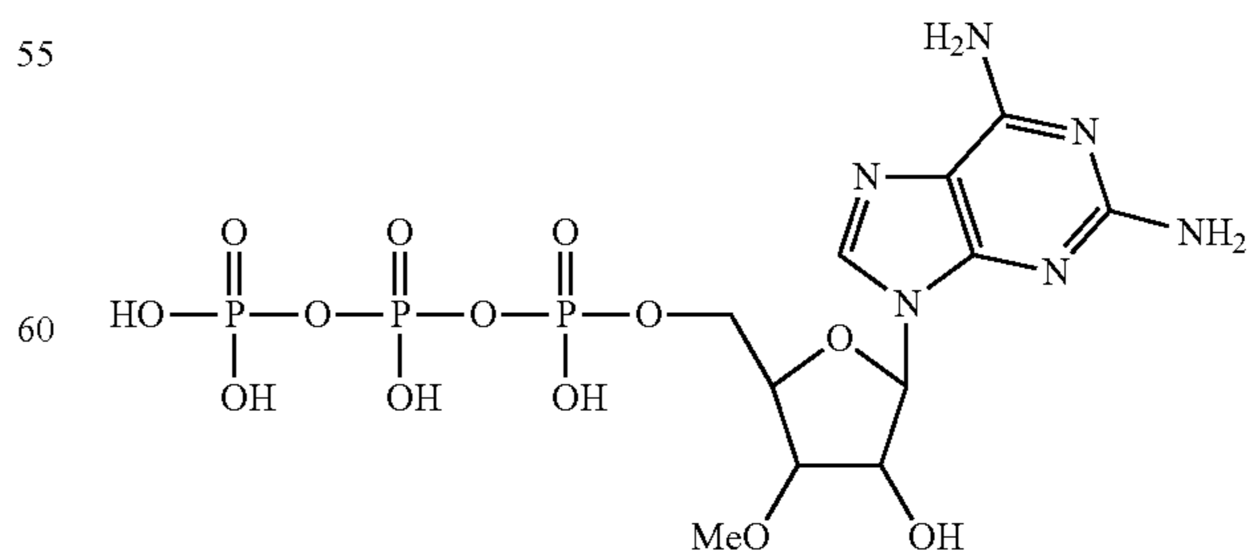
3'-methoxy-3'-deoxy-2-aminoadenosine-5'-triphosphate
