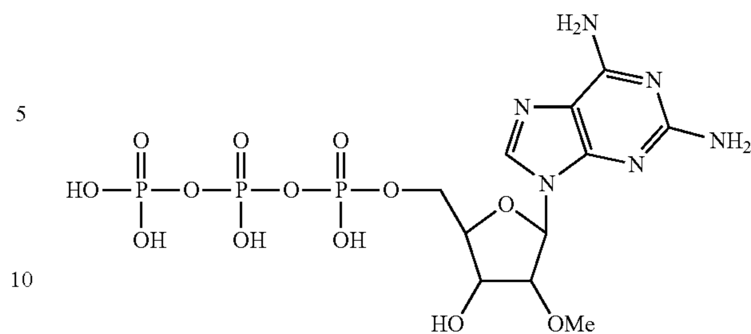
2'-methoxy-2'-deoxy-2-amino-adenosine-5'-triphosphate
