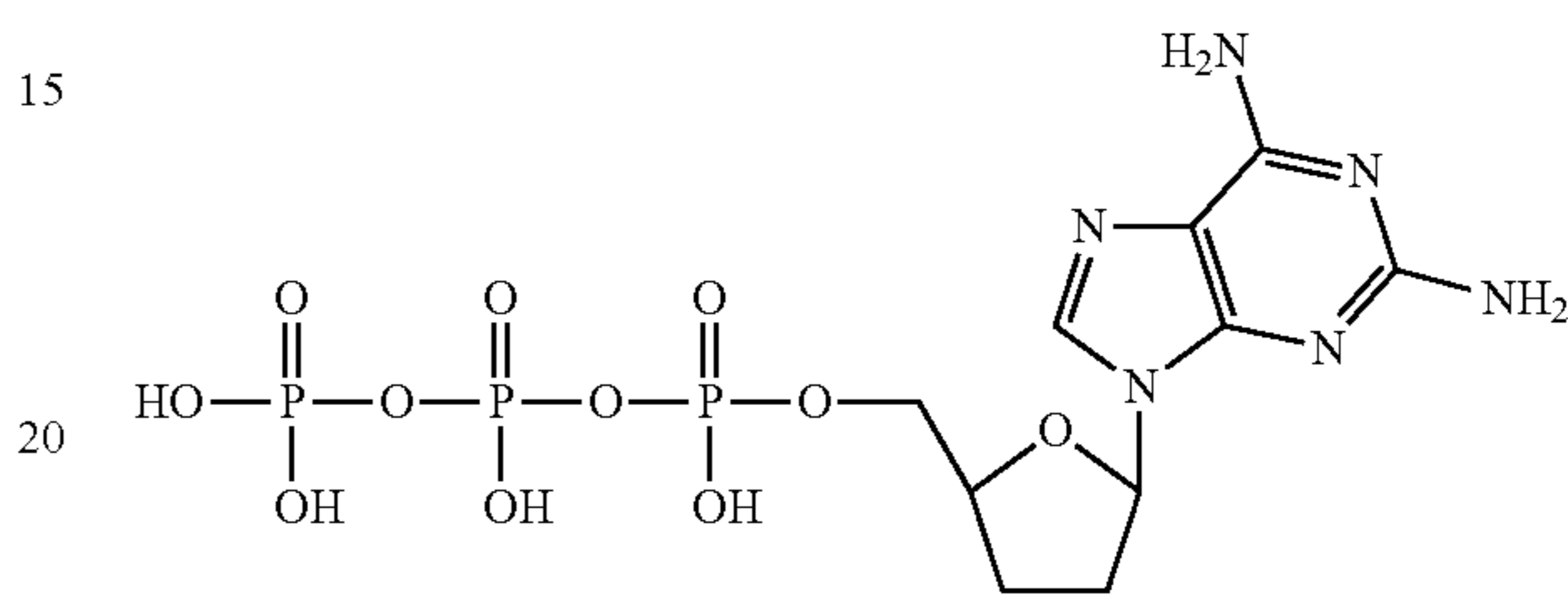
2-amino-2',3'-dideoxyadenosine-5'-triphosphate
