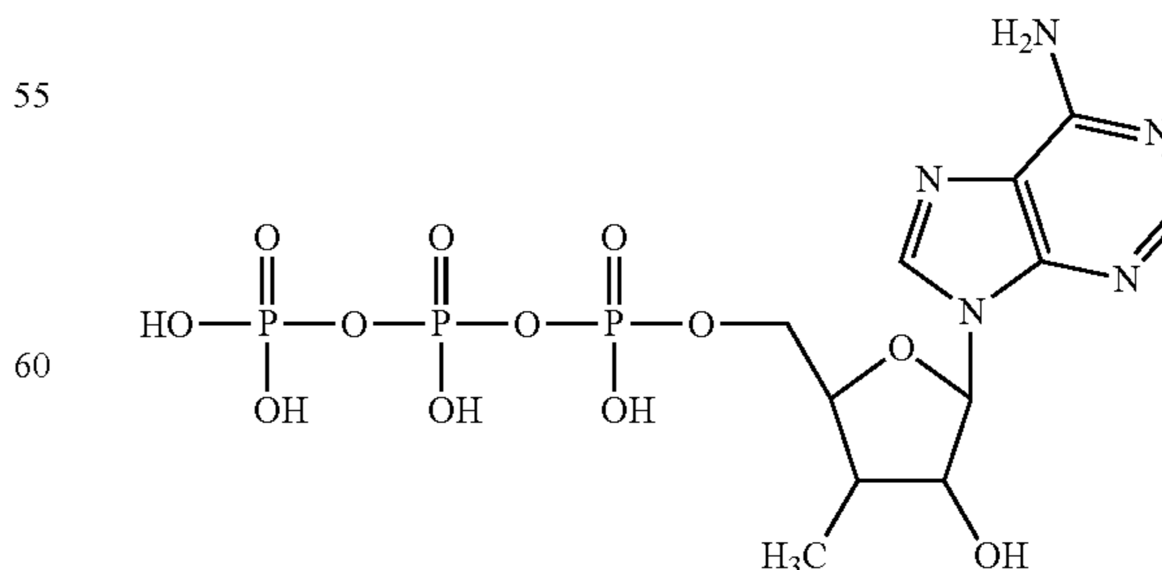
3'-methyl-3'-deoxyadenosine-5'-triphosphate
