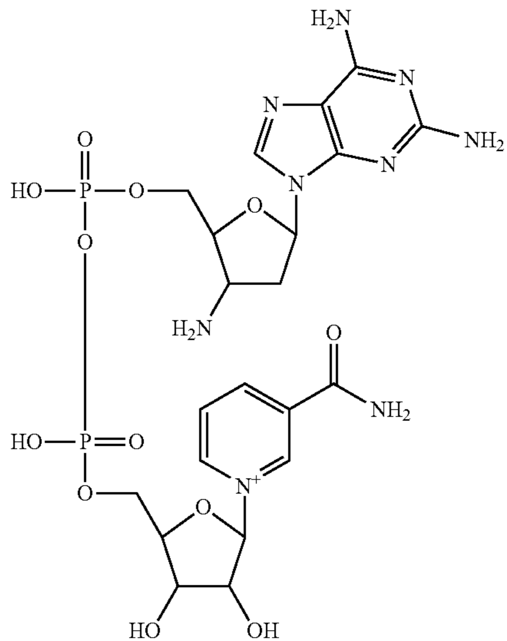
2'-deoxy-3'-amino-2-amino-NAD +
