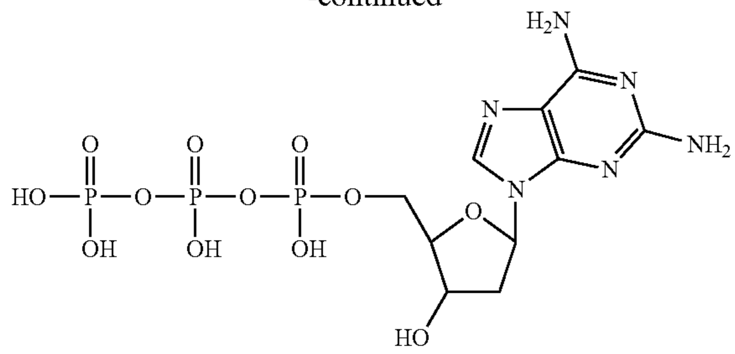
2-amino-2'-deoxyadenosine-5'-triphosphate
