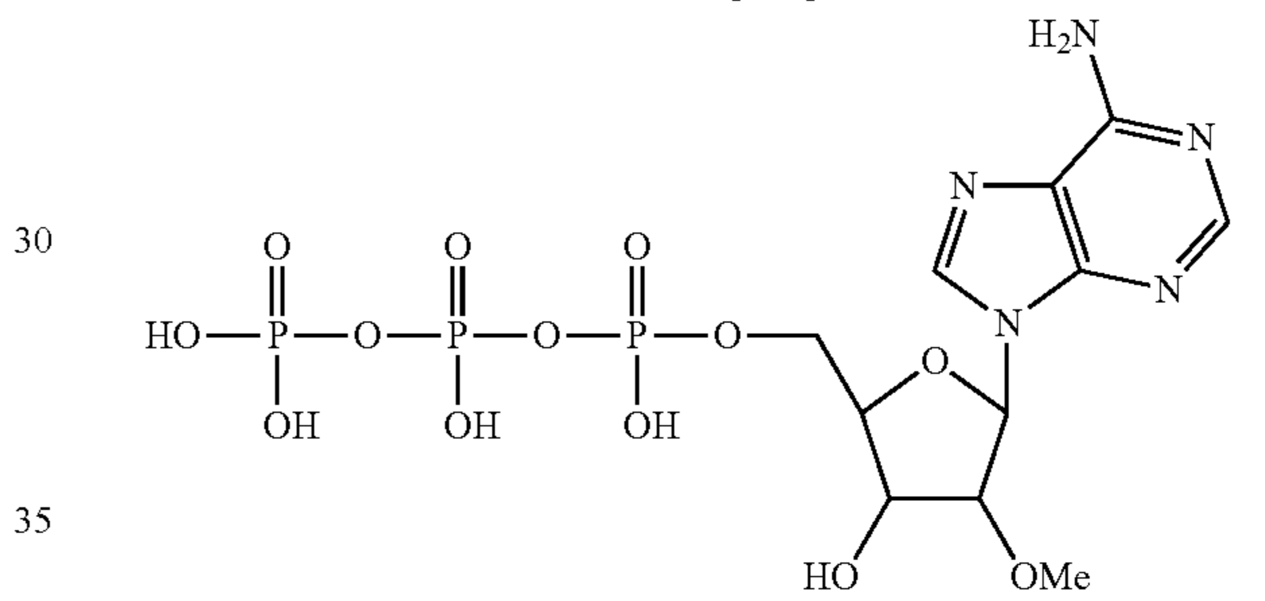
2'-methoxy-2'-deoxyadenosine-5'-triphosphate
