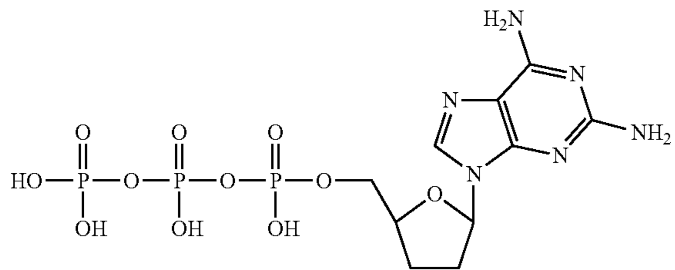
2-amino-2',3'-dideoxyadenosine-5'-triphosphate
