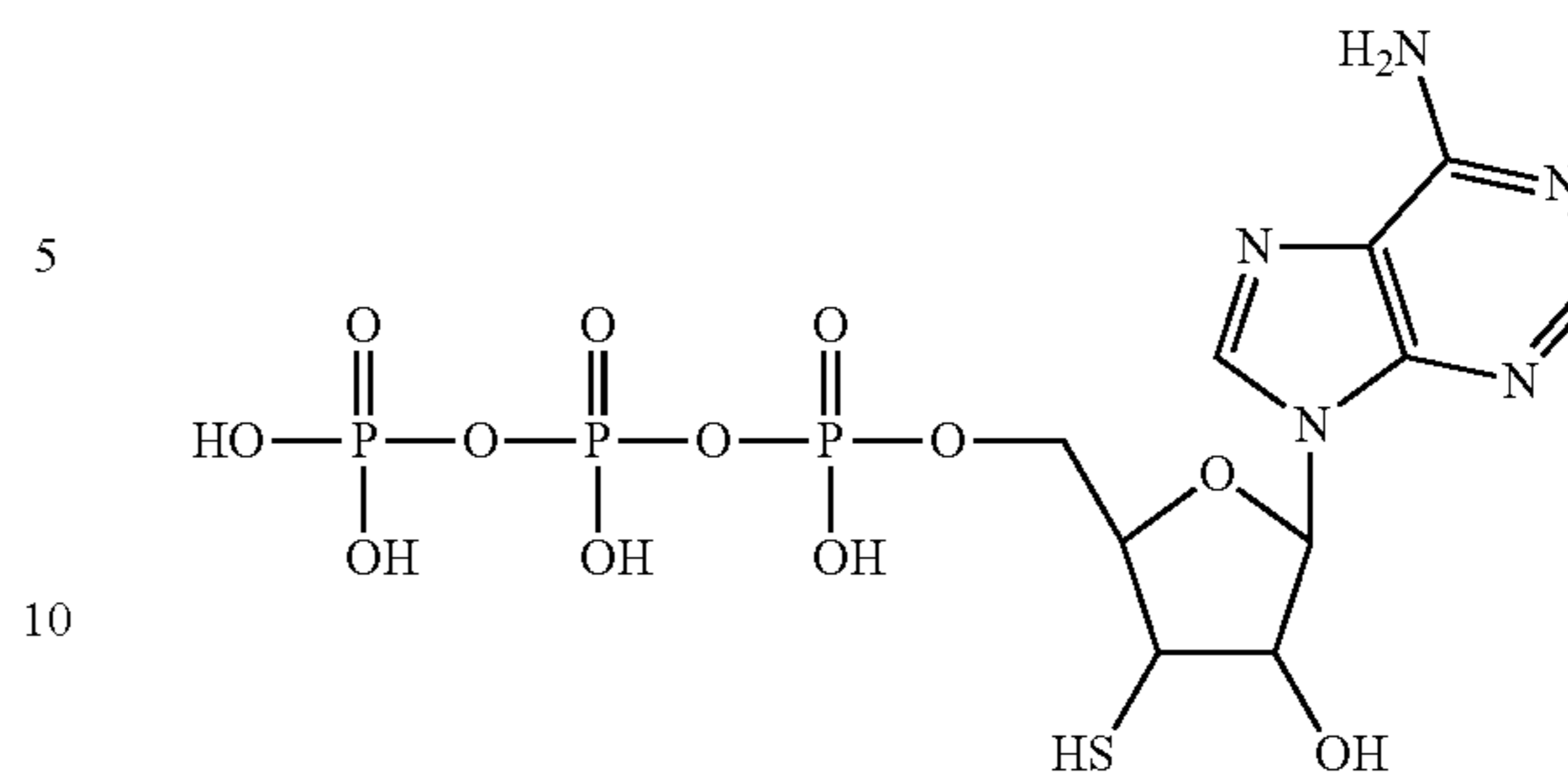
3'-thio-3'-deoxyadenosine-5'-triphosphate
