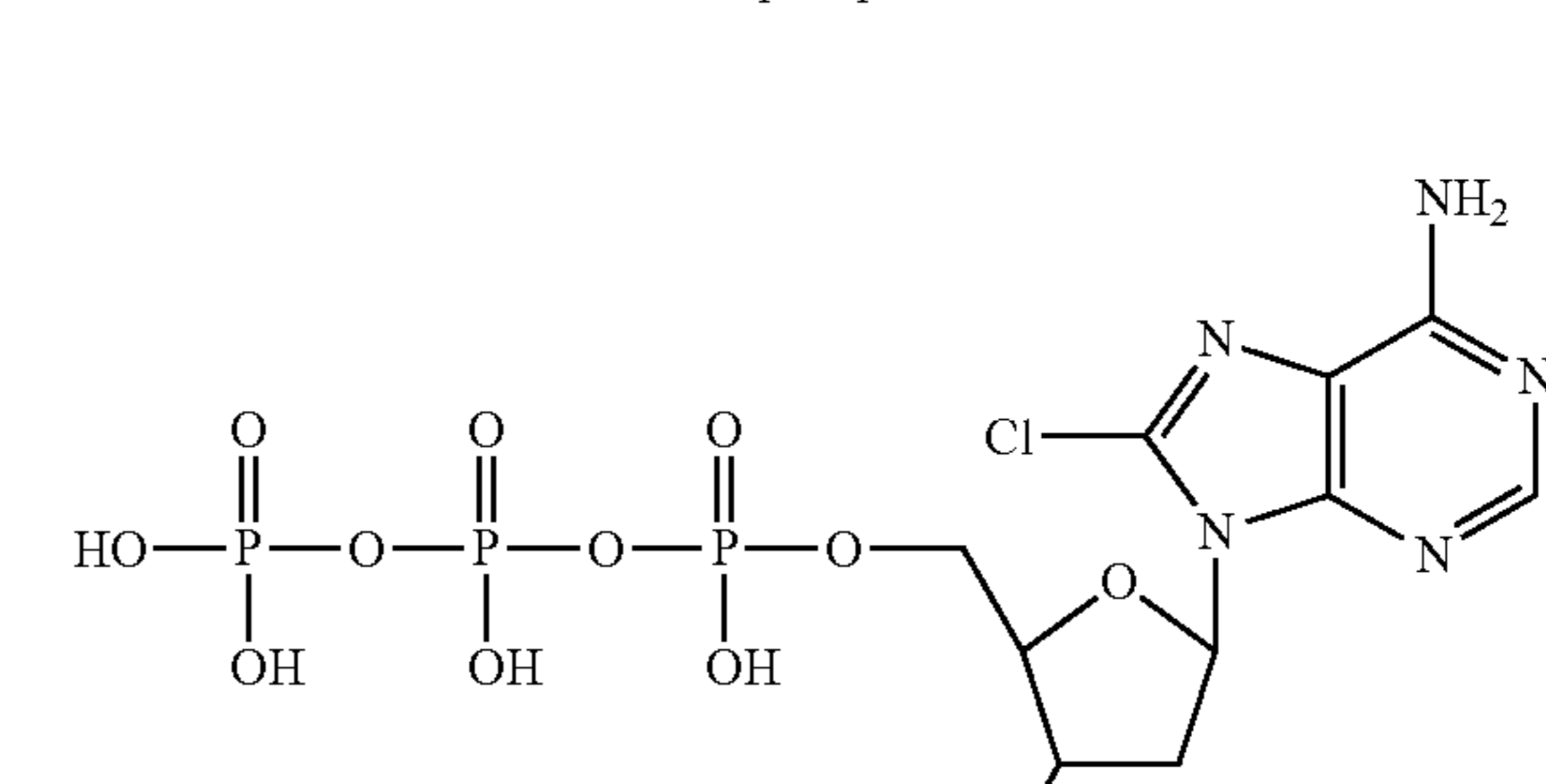
8-chloro-adenosine-5'-triphosphate
