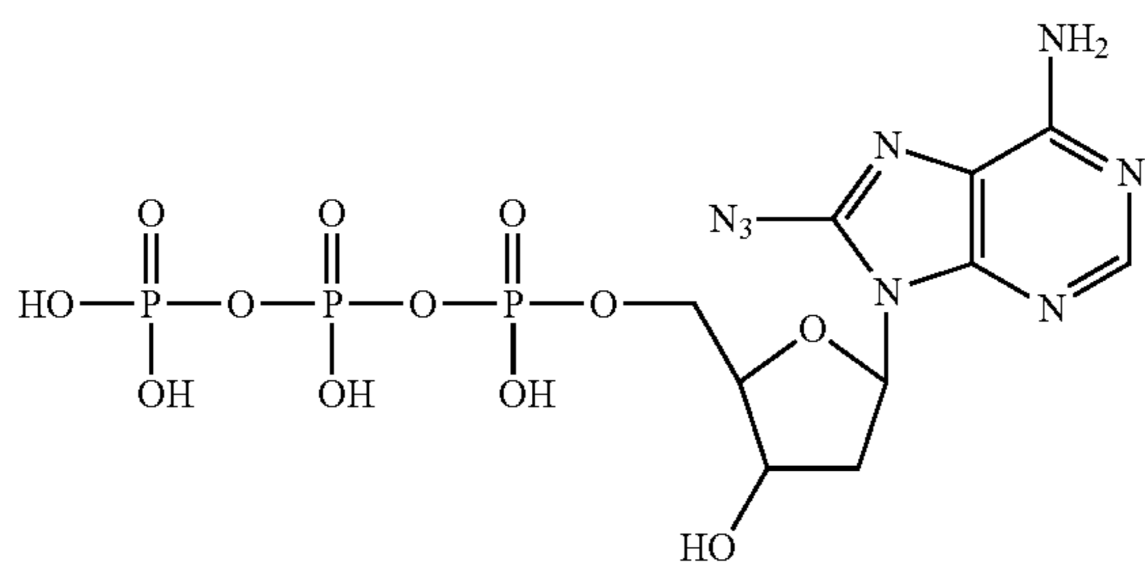
8-azido-2'-deoxy-adenosine-5'-triphosphate
