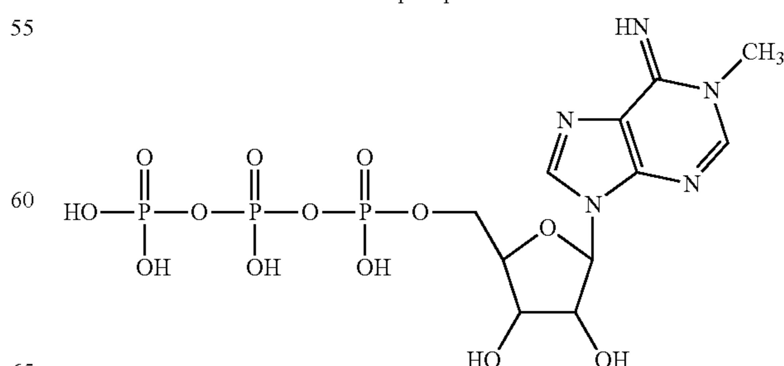
N1-methyl-adenosine-5'-triphosphate
