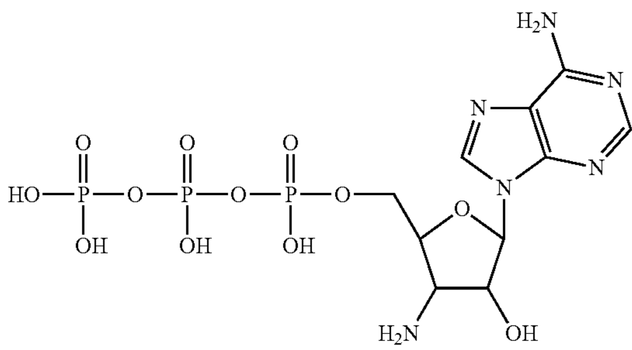
3'-amino-3'-deoxy-adenosine-5'-triphosphate
