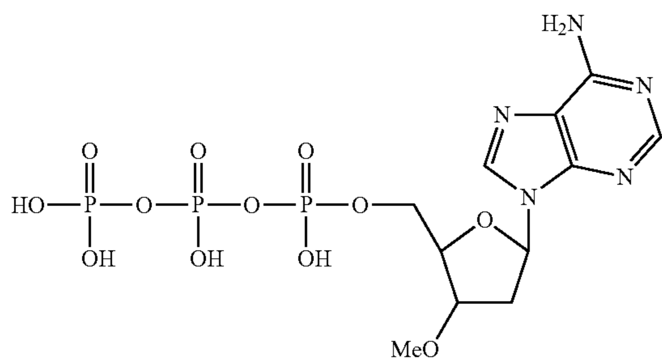
3'-methoxy-2',3'-dideoxy-adenosine-5'-triphosphate
