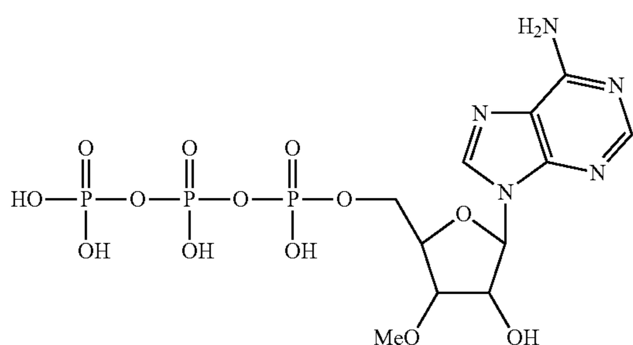
3'-methoxy-3'-deoxy-adenosine-5'-triphosphate
