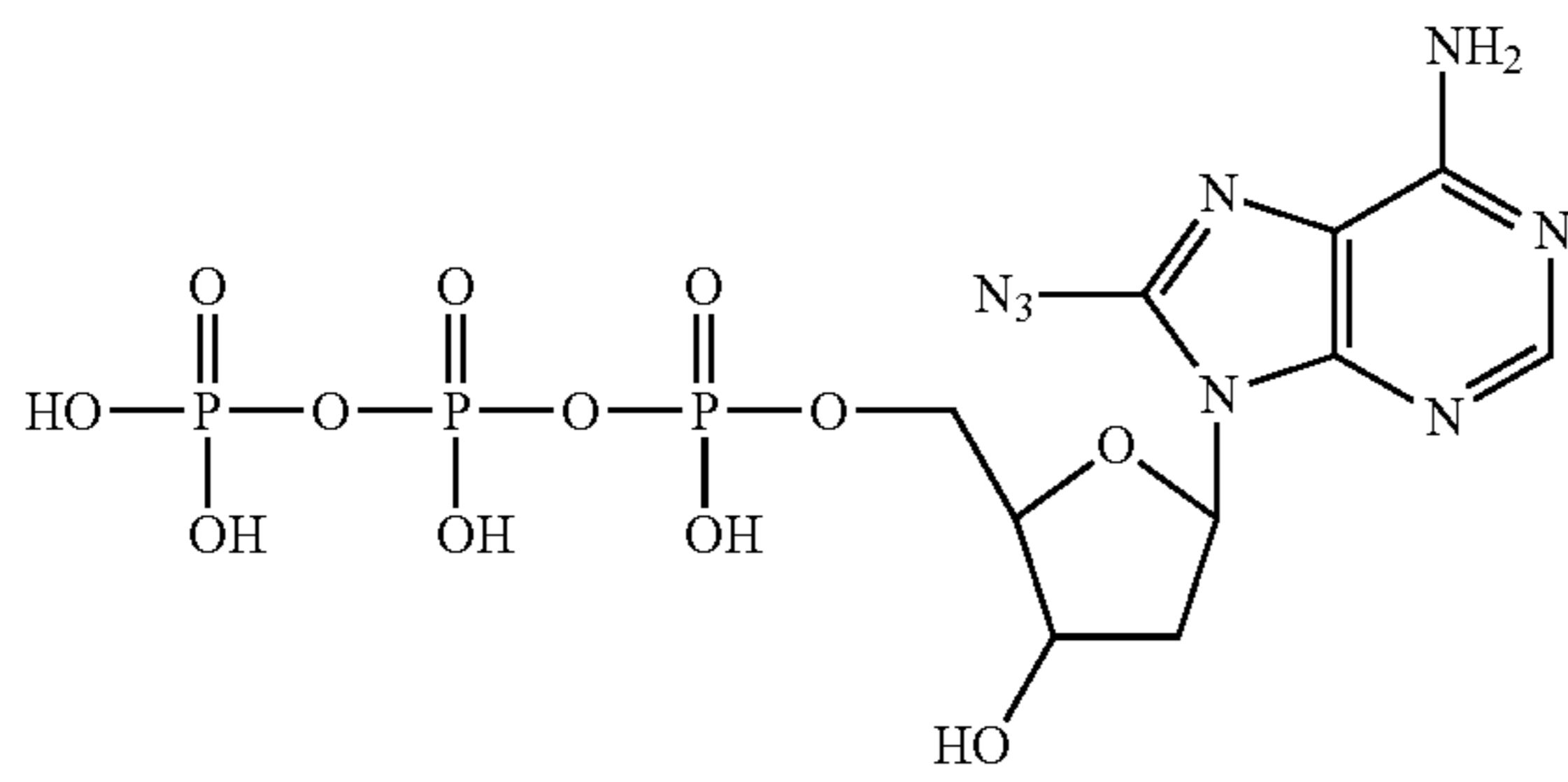
8-azido-2'-deoxy-adenosine-5'-triphosphate
