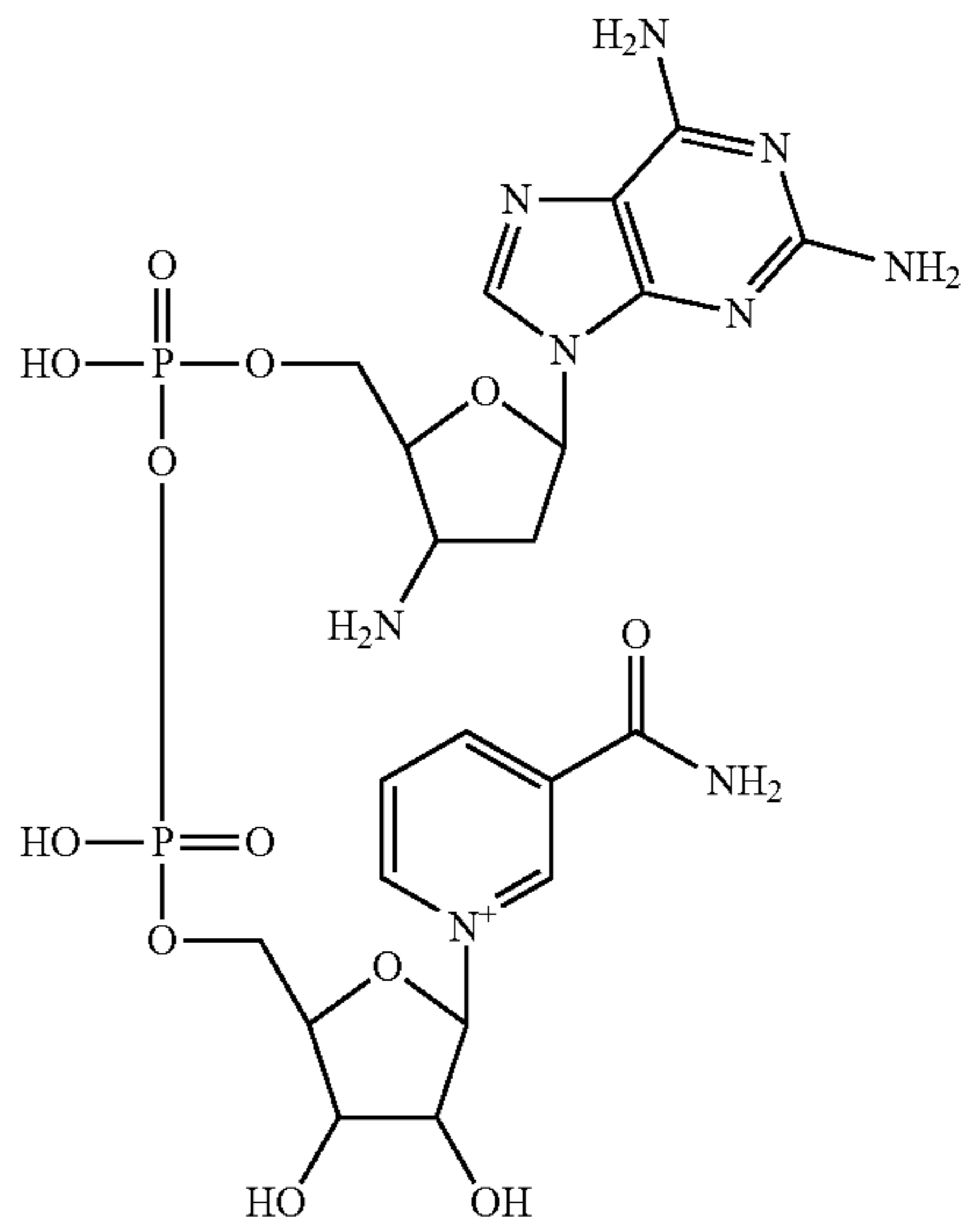
2'-deoxy-3'-amino-2-amino-NAD +
