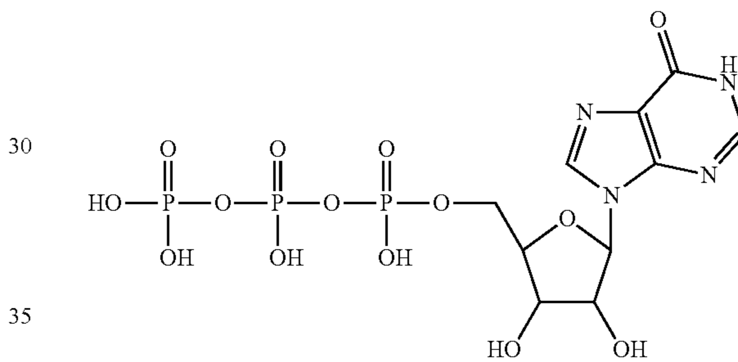
inosine-5'-triphosphate
