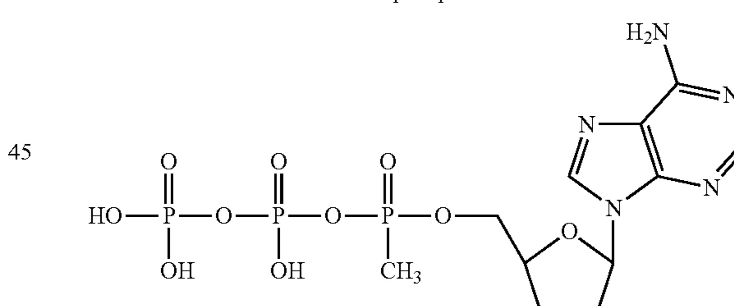
5'-alpha-methylphosphonate-2',3'-dideoxyadenosine-5'-triphosphate
