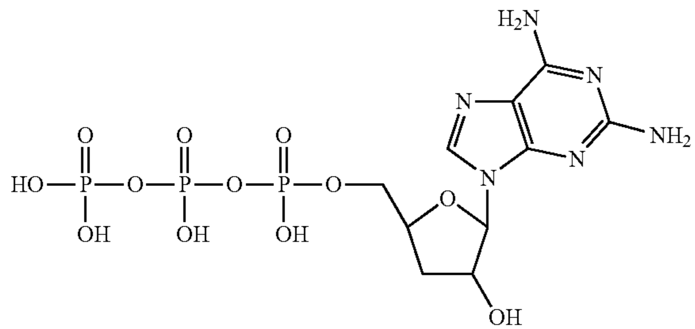
2-amino-3'-deoxyadenosine-5'-triphosphate
