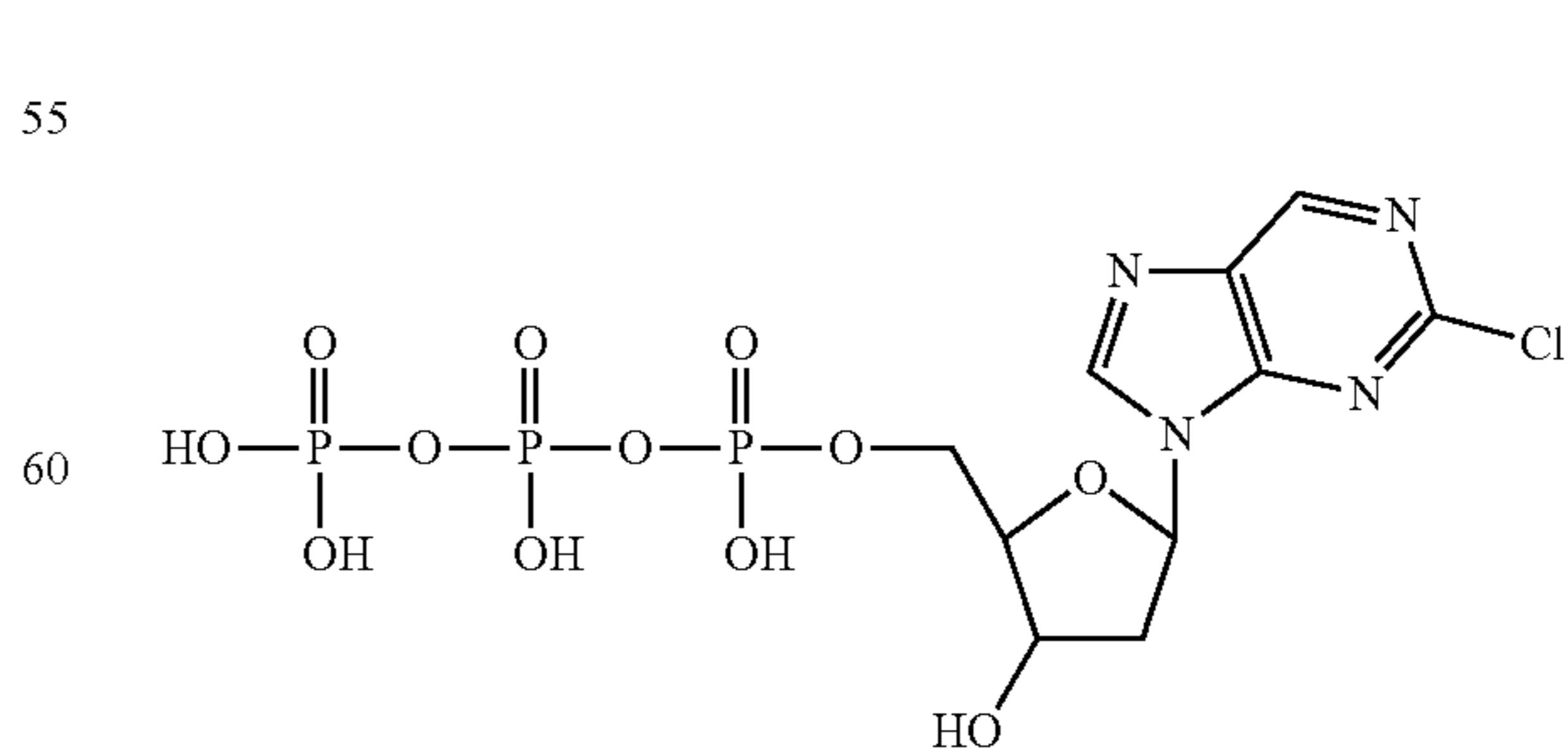
2-Chloropurine-2'-deoxyriboside-5'-triphosphate
