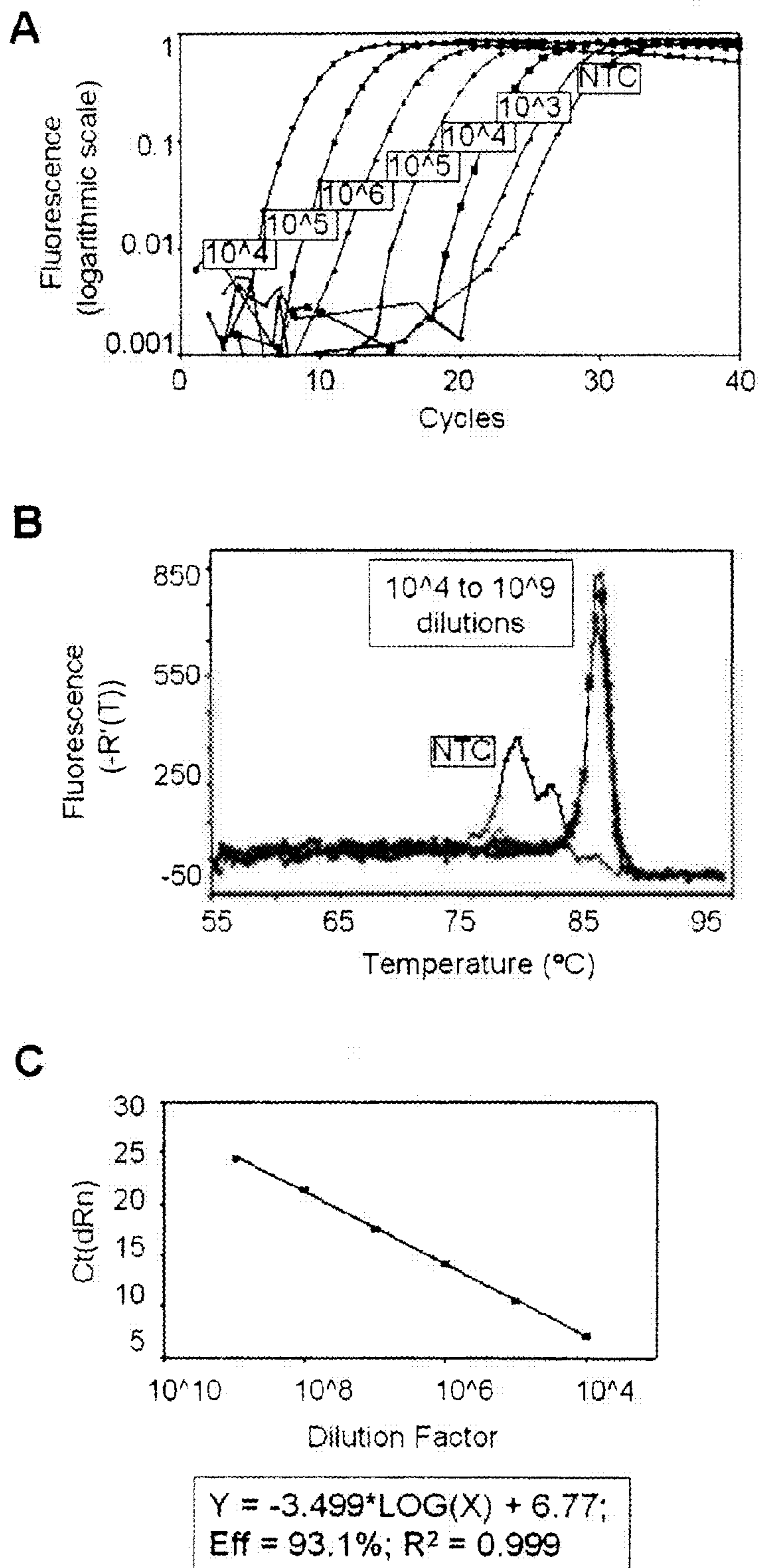
Figure 3
