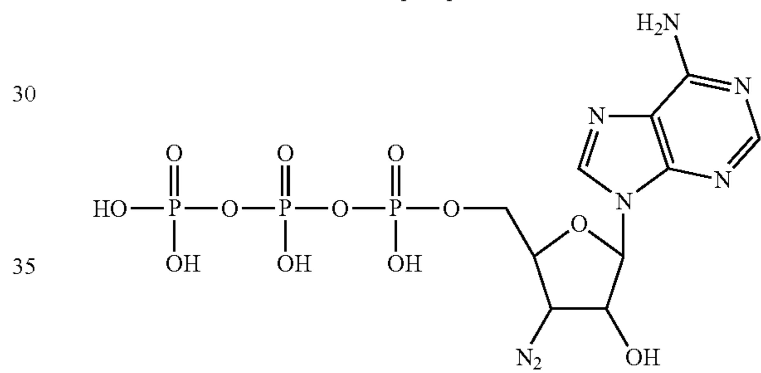
3'-azido-3'-deoxy-adenosine-5'-triphosphate
