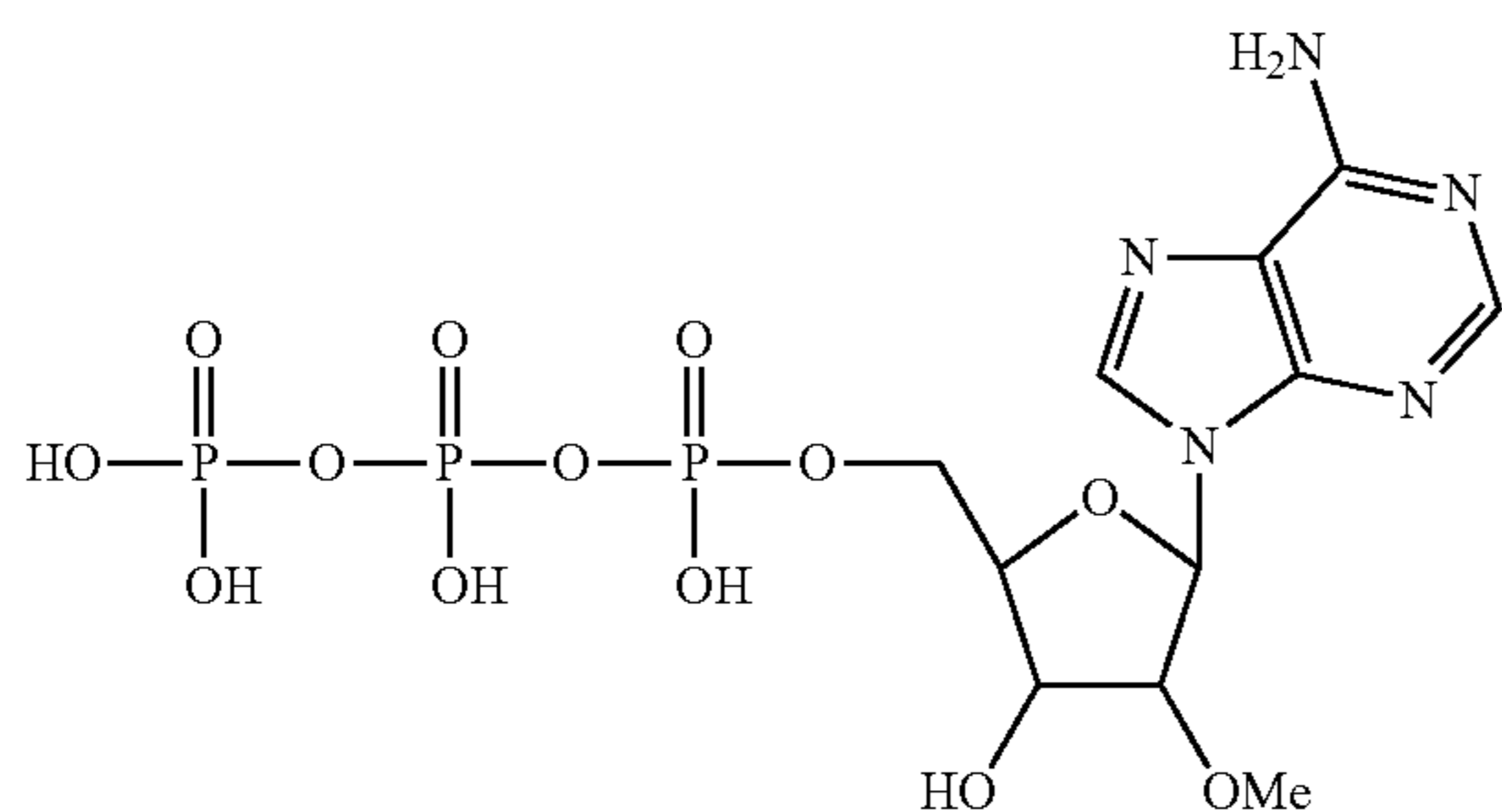
2'-methoxy-2'-deoxy-adenosine-5'-triphosphate
