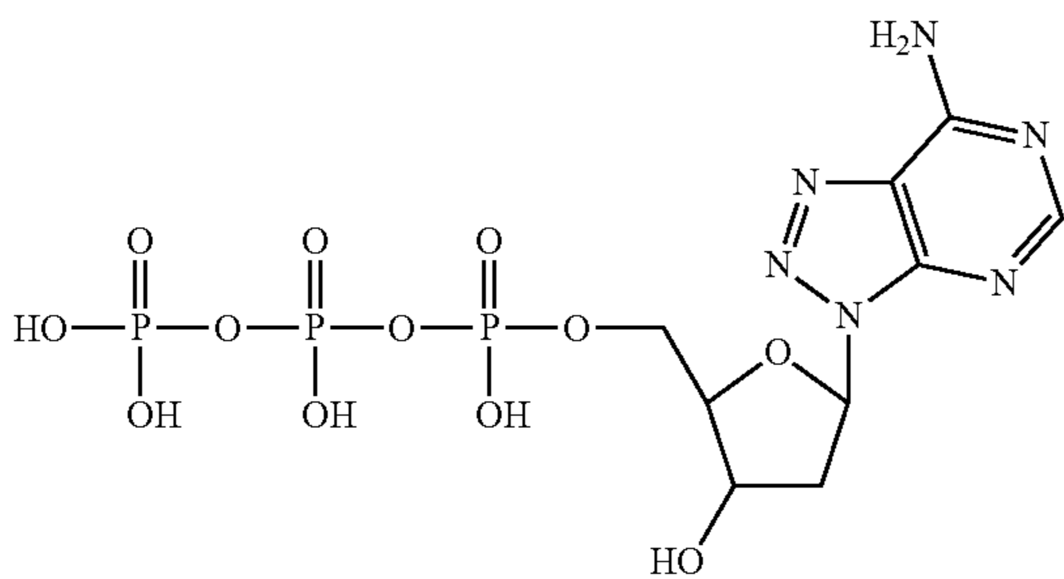
8-aza-2'-deoxy-adenosine-5'-triphosphate
