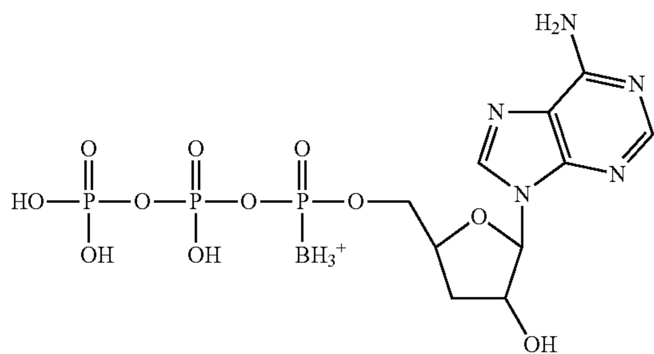
5'-alpha-[P-borano]-3'-deoxyadenosine-5'-triphosphate
