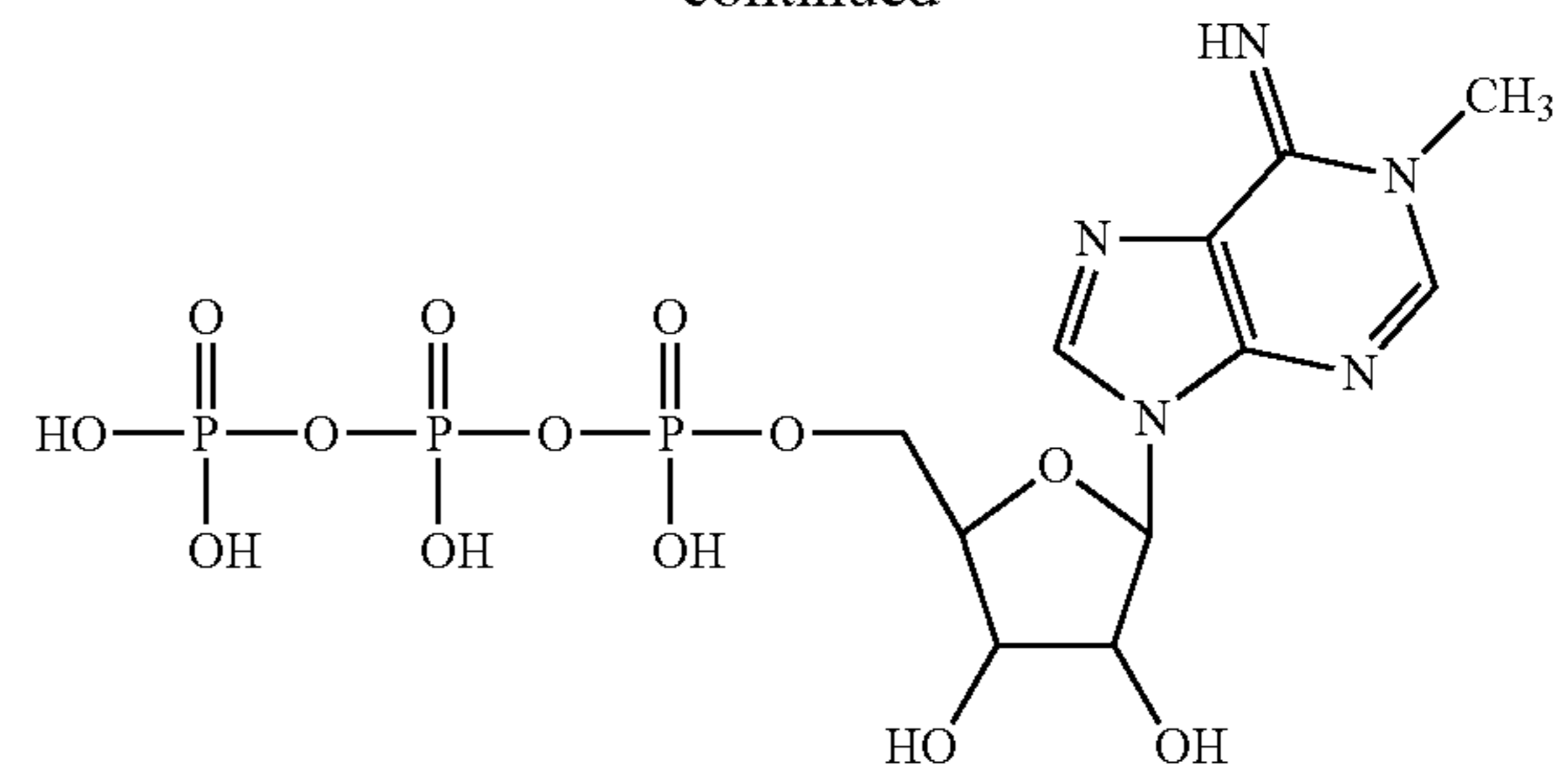
N1-methyl-adenosine-5'-triphosphate
