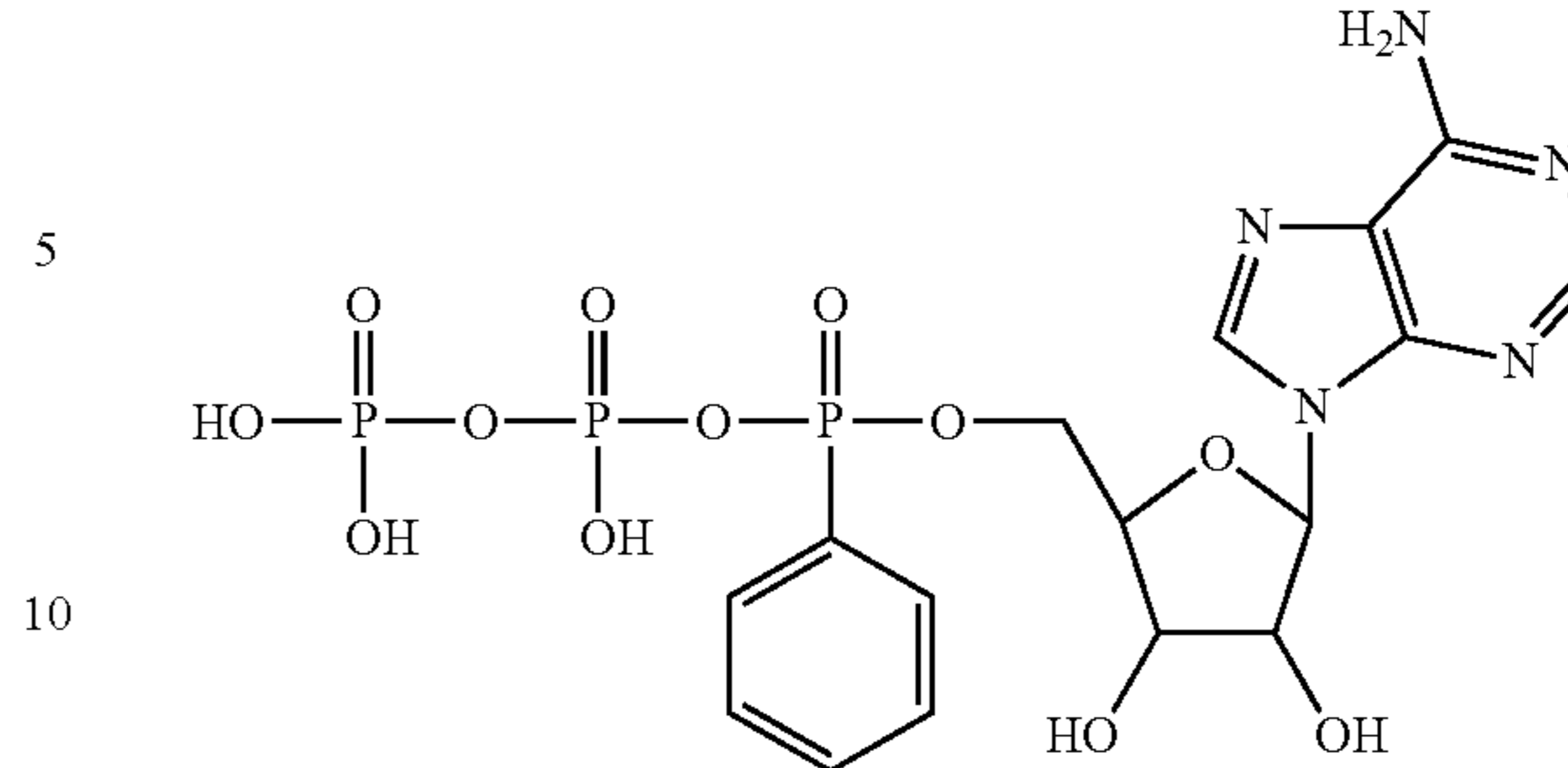
5'-alpha-phenylphosphonate-adenosine-5'-triphosphate
