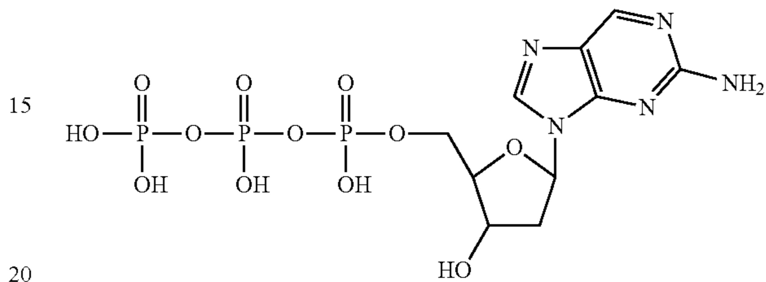
2-aminopurine-2'-deoxyriboside-5'-triphosphate
