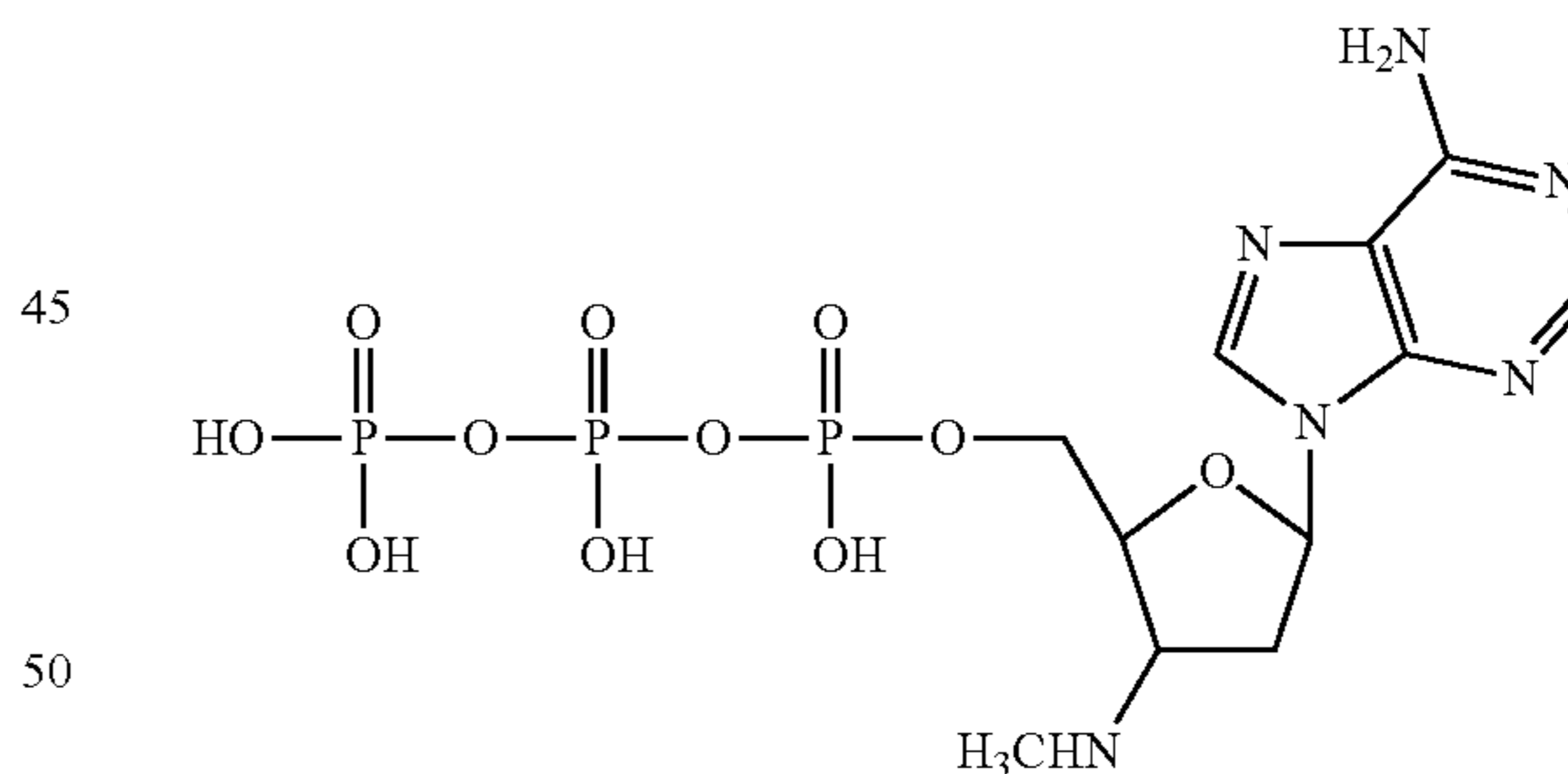
3'-methylamino-2',3'-dideoxyadenosine-5'-triphosphate
