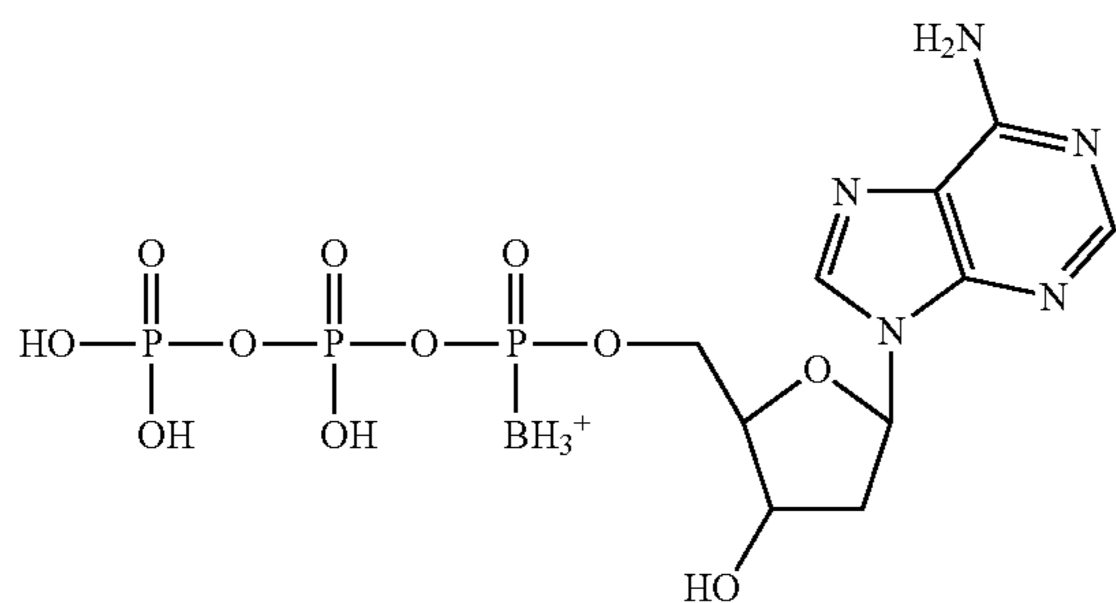
5'-alpha-[P-borano]-2'-deoxyadenosine-5'-triphosphate
