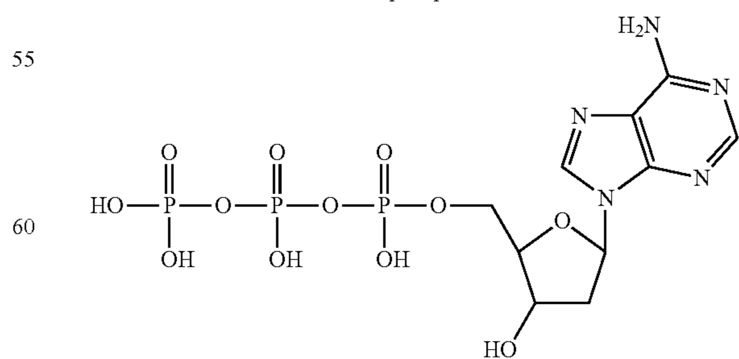
2'-deoxy-adenosine-5'-triphosphate
