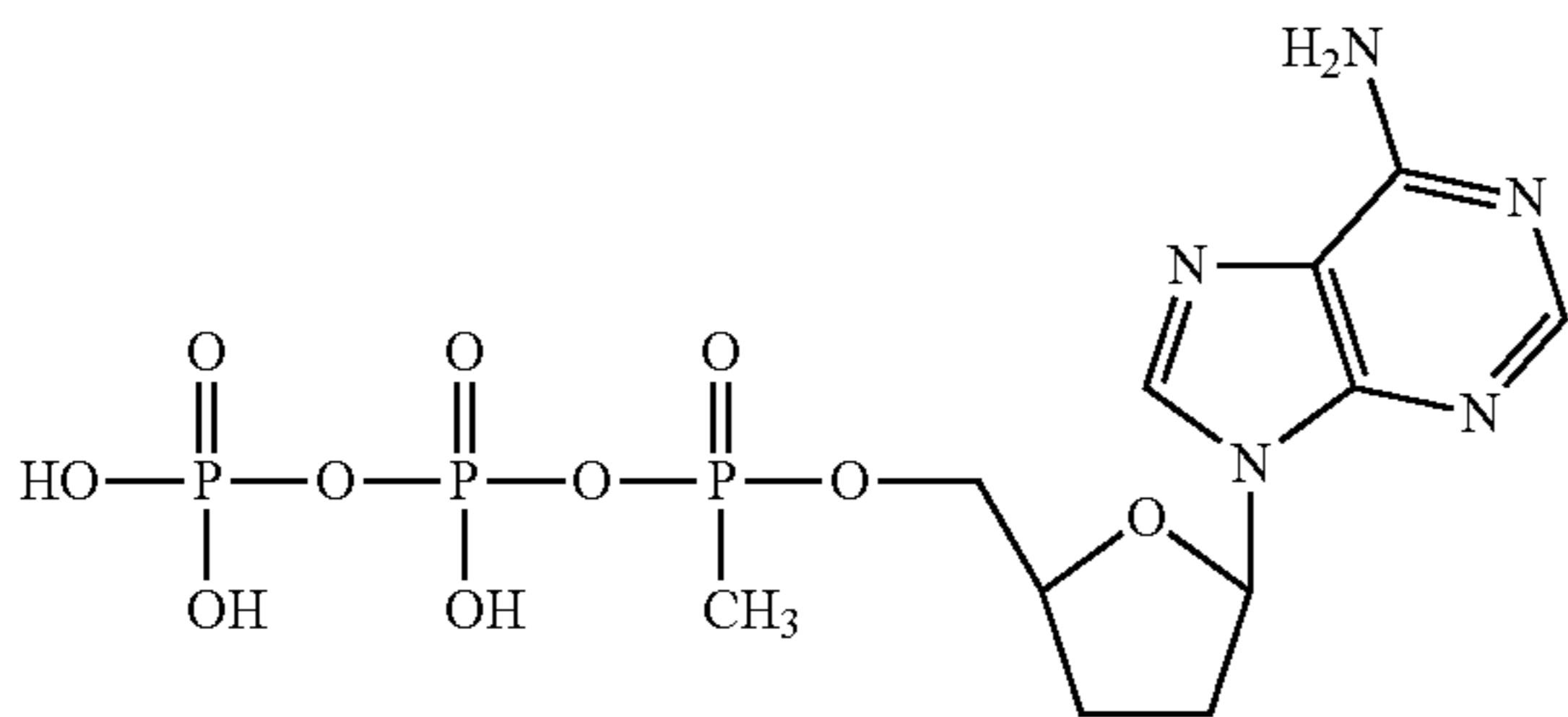
5'-alpha-methylphosphonate-2',3'-dideoxyadenosine-5'-triphosphate
