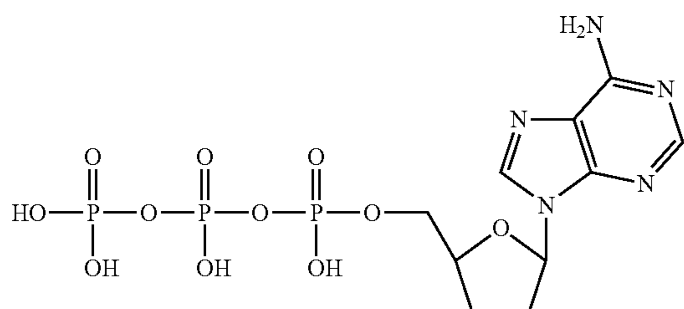
2',3'-dideoxy-adenosine-5'-triphosphate
