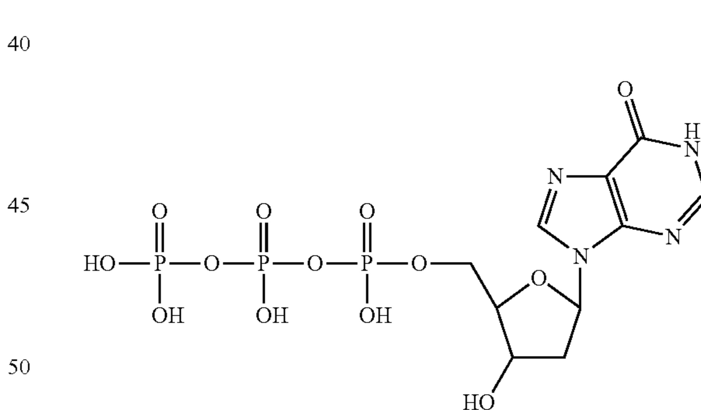
2'-deoxy-inosine-5'-triphosphate
