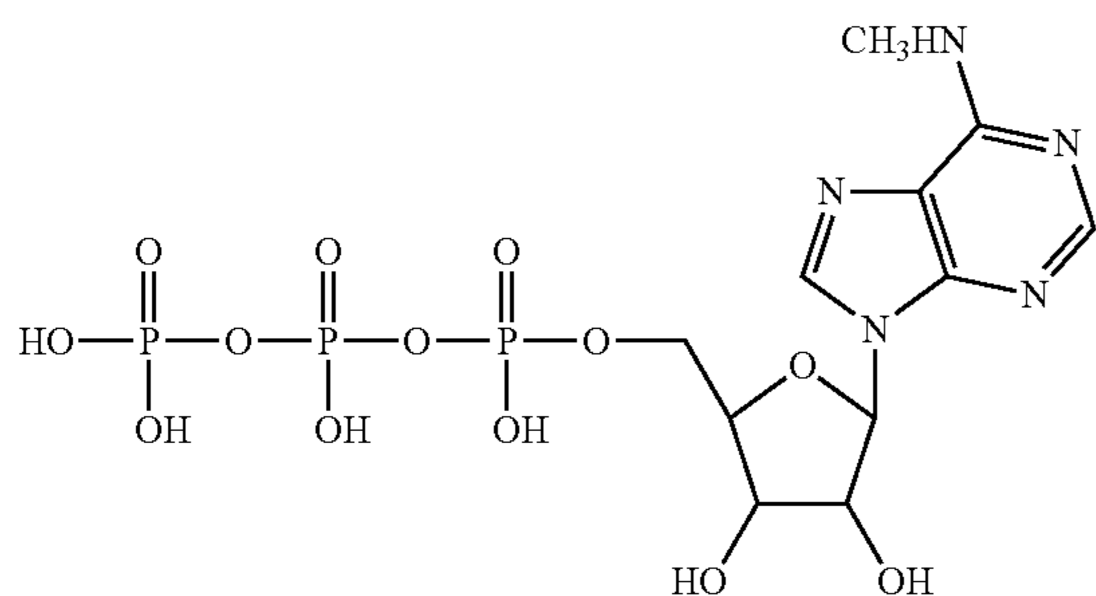
N6-methyl-adenosine-5'-triphosphate
