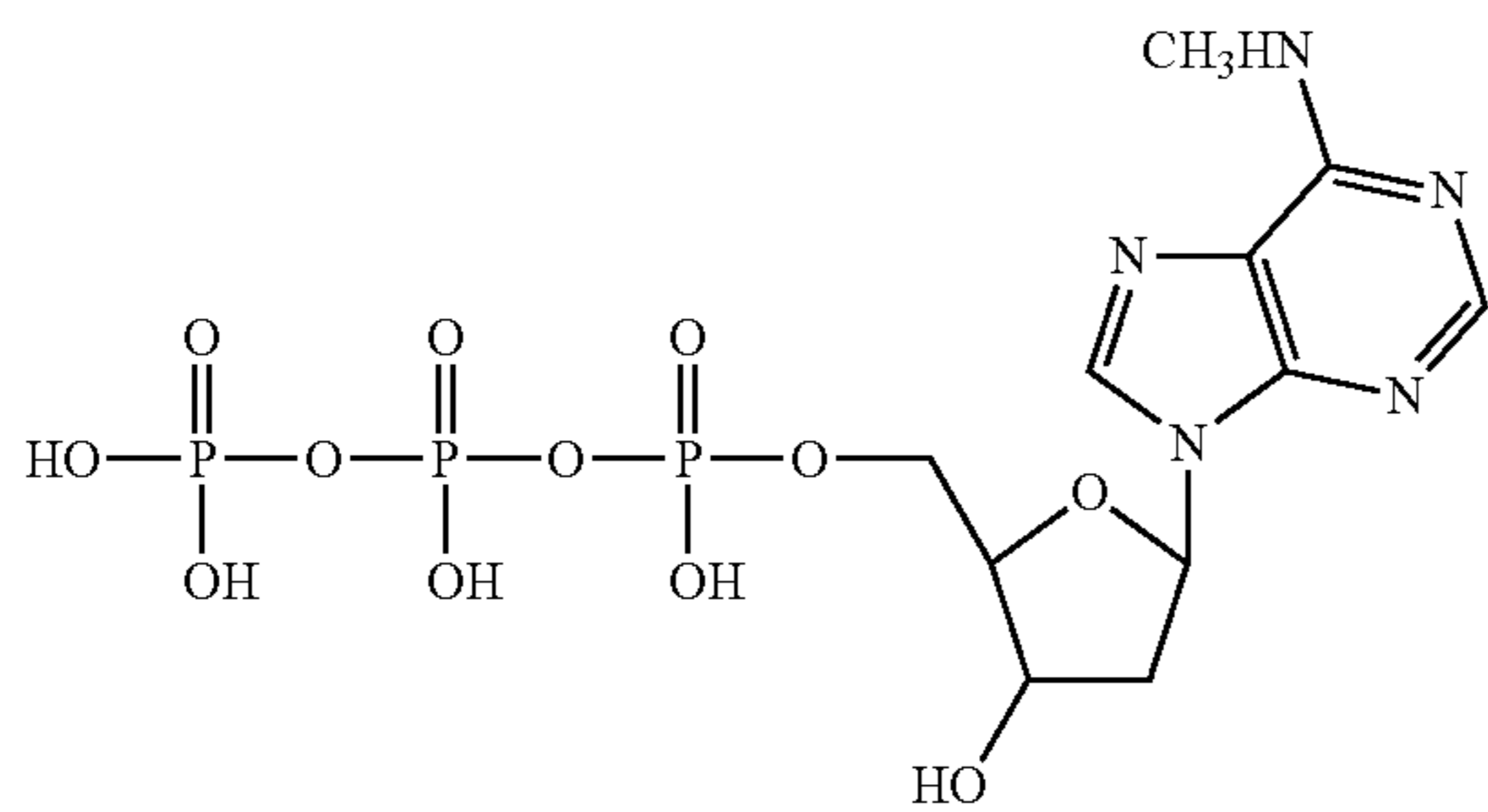
N6-methyl-2'-deoxy-adenosine-5'-triphosphate
