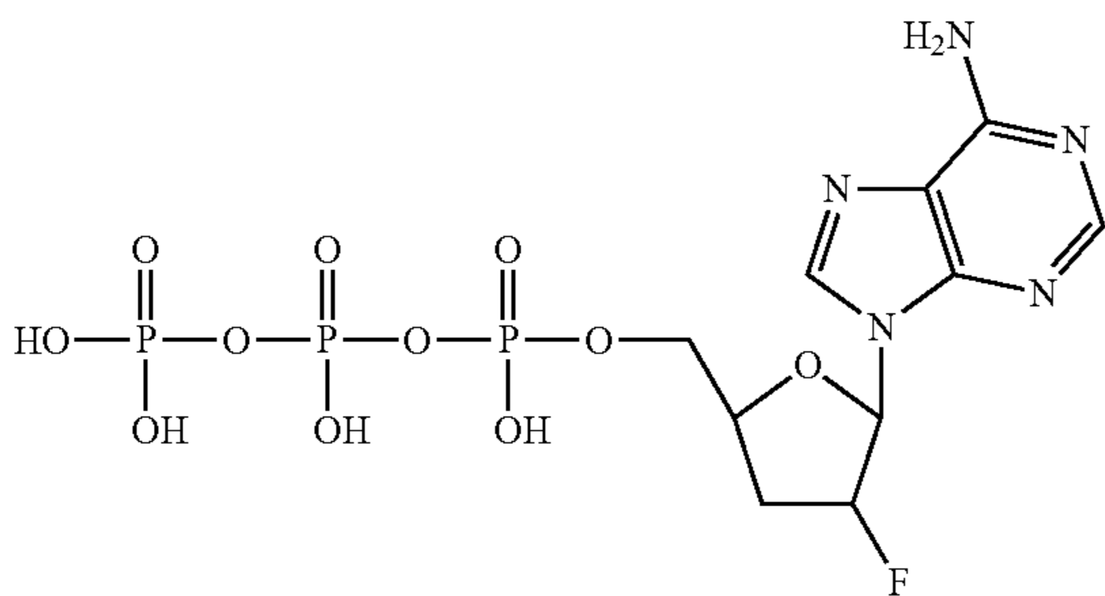
2'-fluoro-2',3'-dideoxy-adenosine-5'-triphosphate
