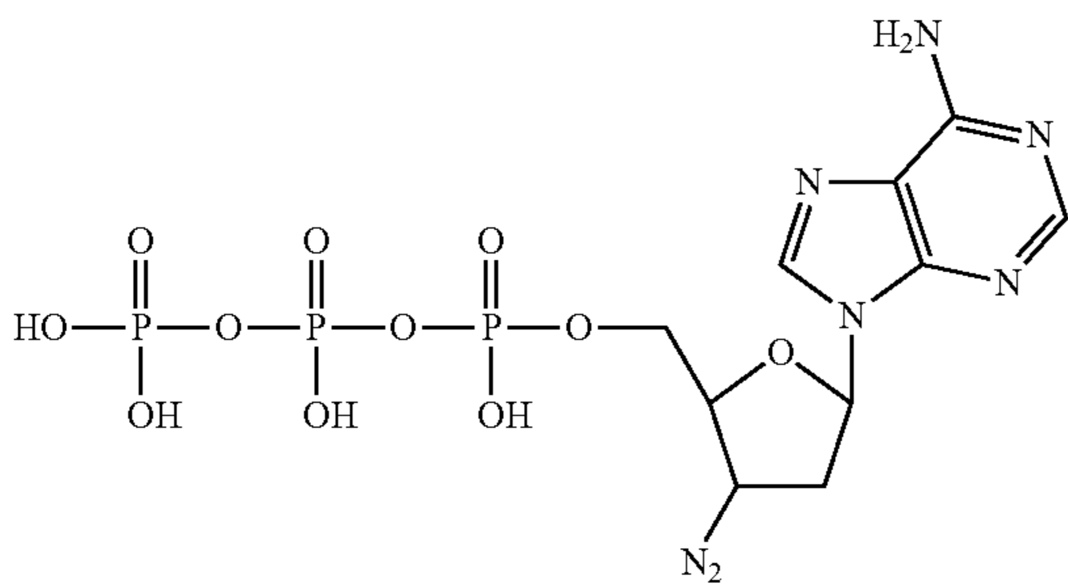
3'-azido-2',3'-dideoxy-adenosine-5'-triphosphate
