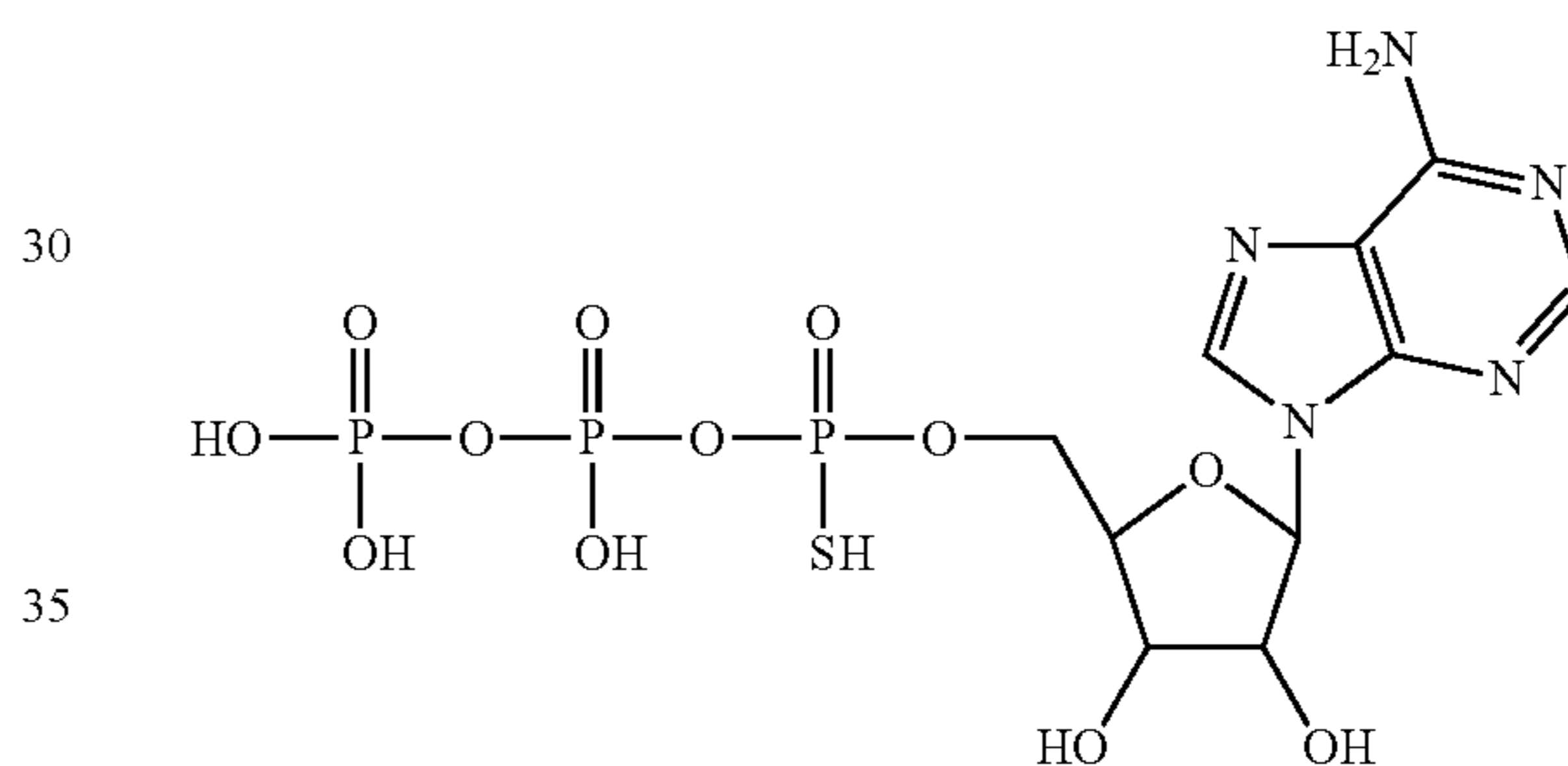
5'-alpha-thio-adenosine-5'-triphosphate
