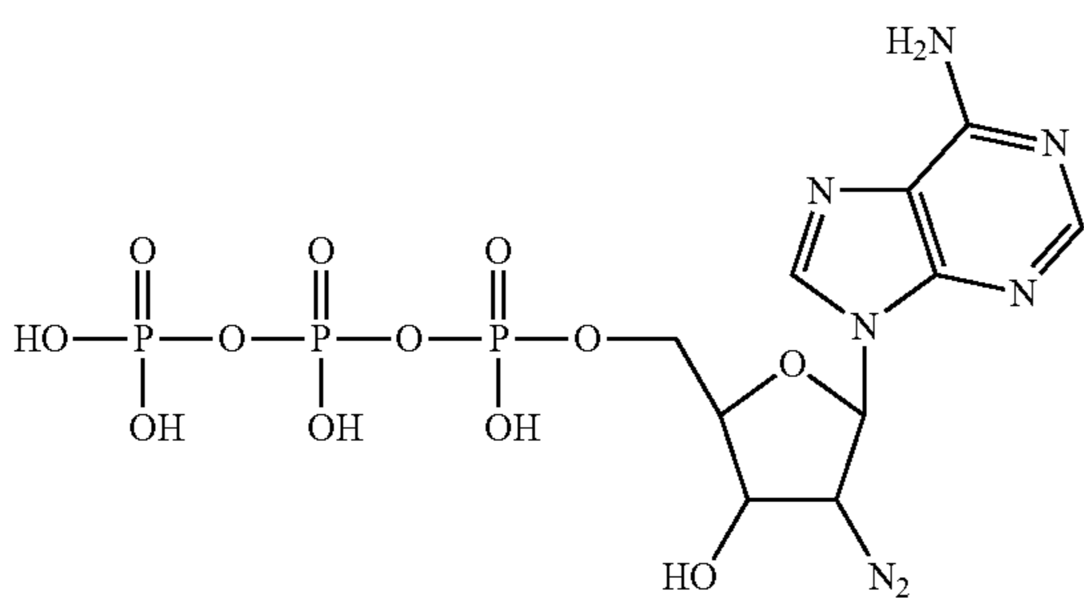
2'-azido-2'-deoxy-adenosine-5'-triphosphate
