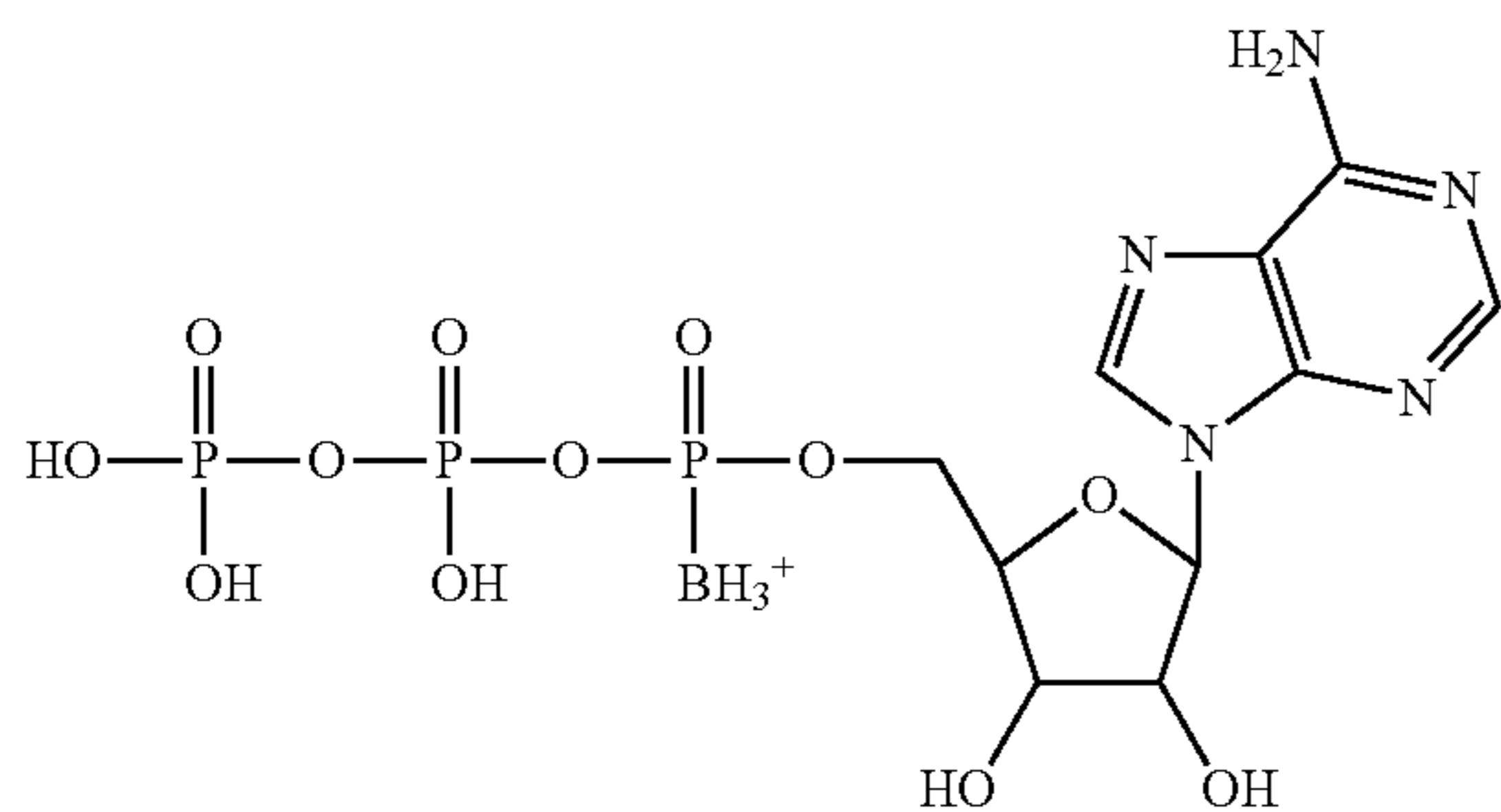
5'-alpha-[P-borano]-adenosine-5'-triphosphate
