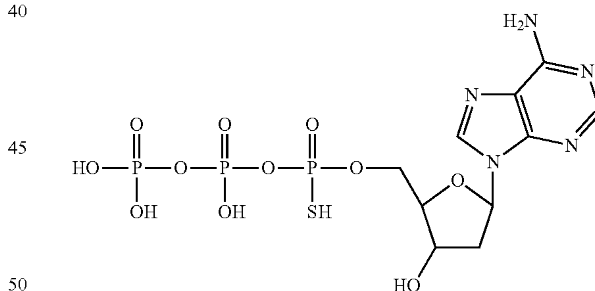
5'-alpha-thio-2'-deoxyadenosine-5'-triphosphate
