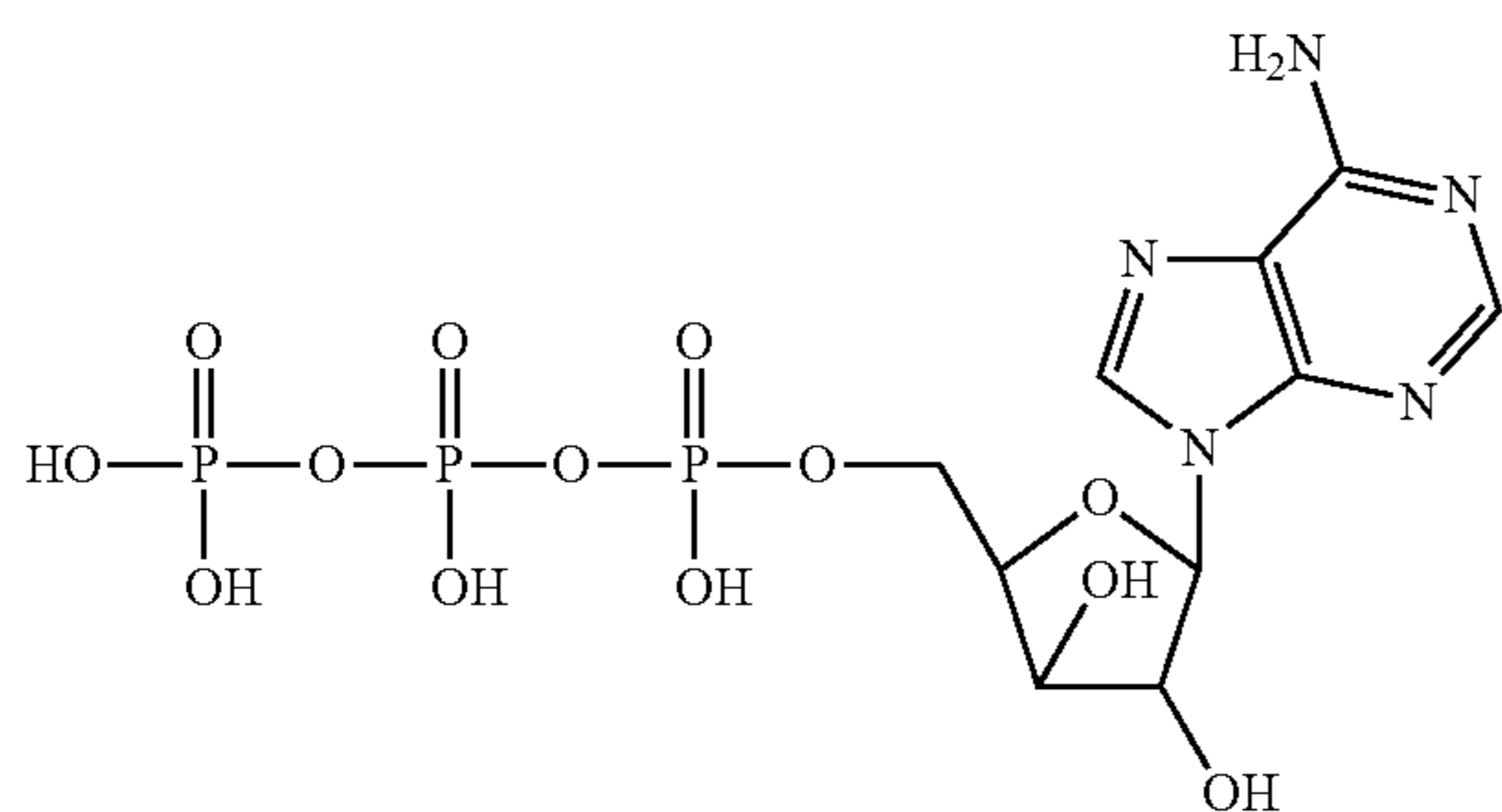
2'-ara-adenosine-5'-triphosphate
