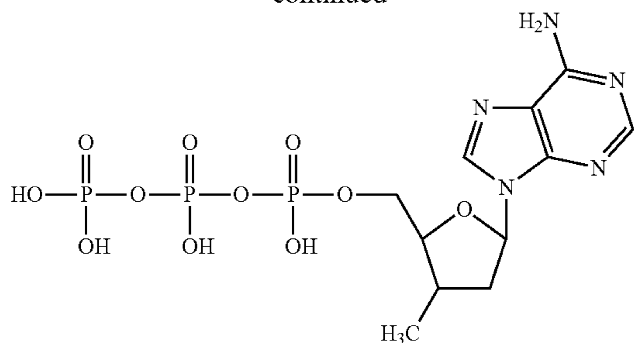
3'-methyl-2',3'-dideoxyadenosine-5'-triphosphate
