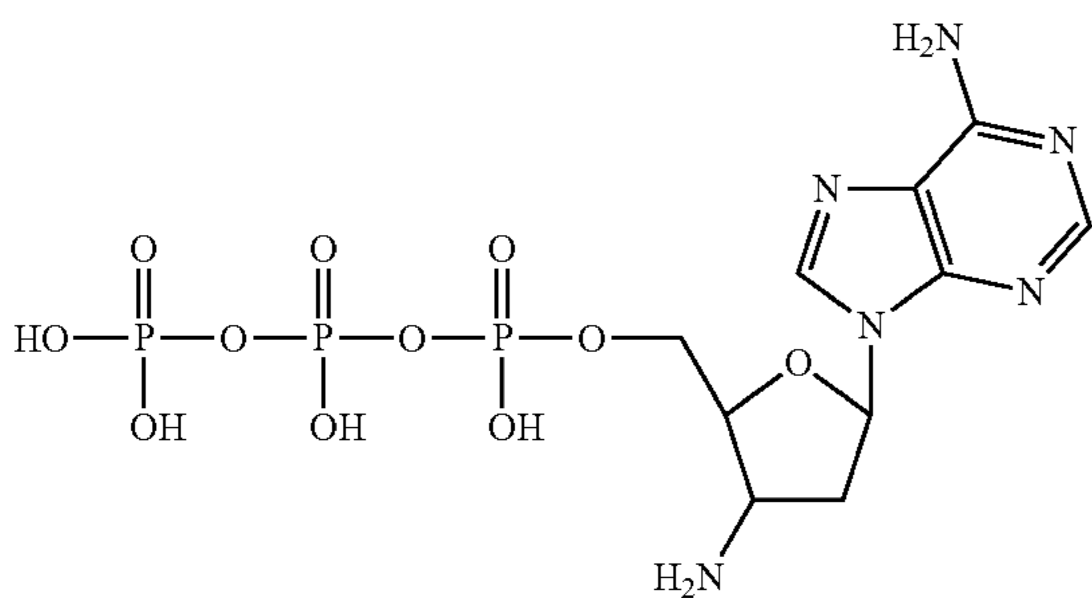
3'-amino-2',3'-dideoxy-adenosine-5'-triphosphate
