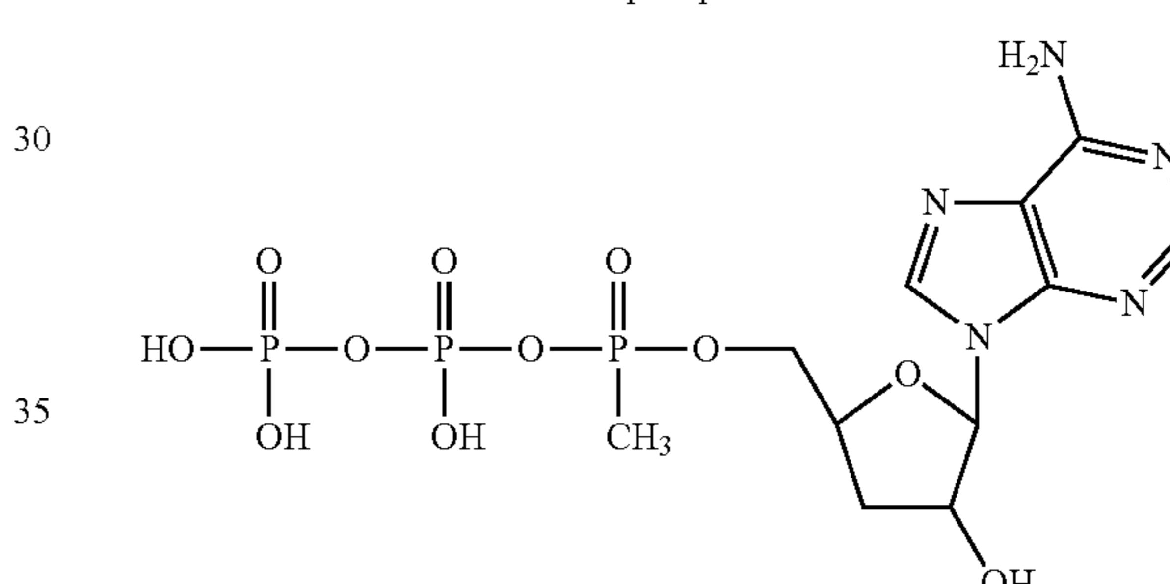
5'-alpha-methylphosphonate-3'-deoxyadenosine-5'-triphosphate
