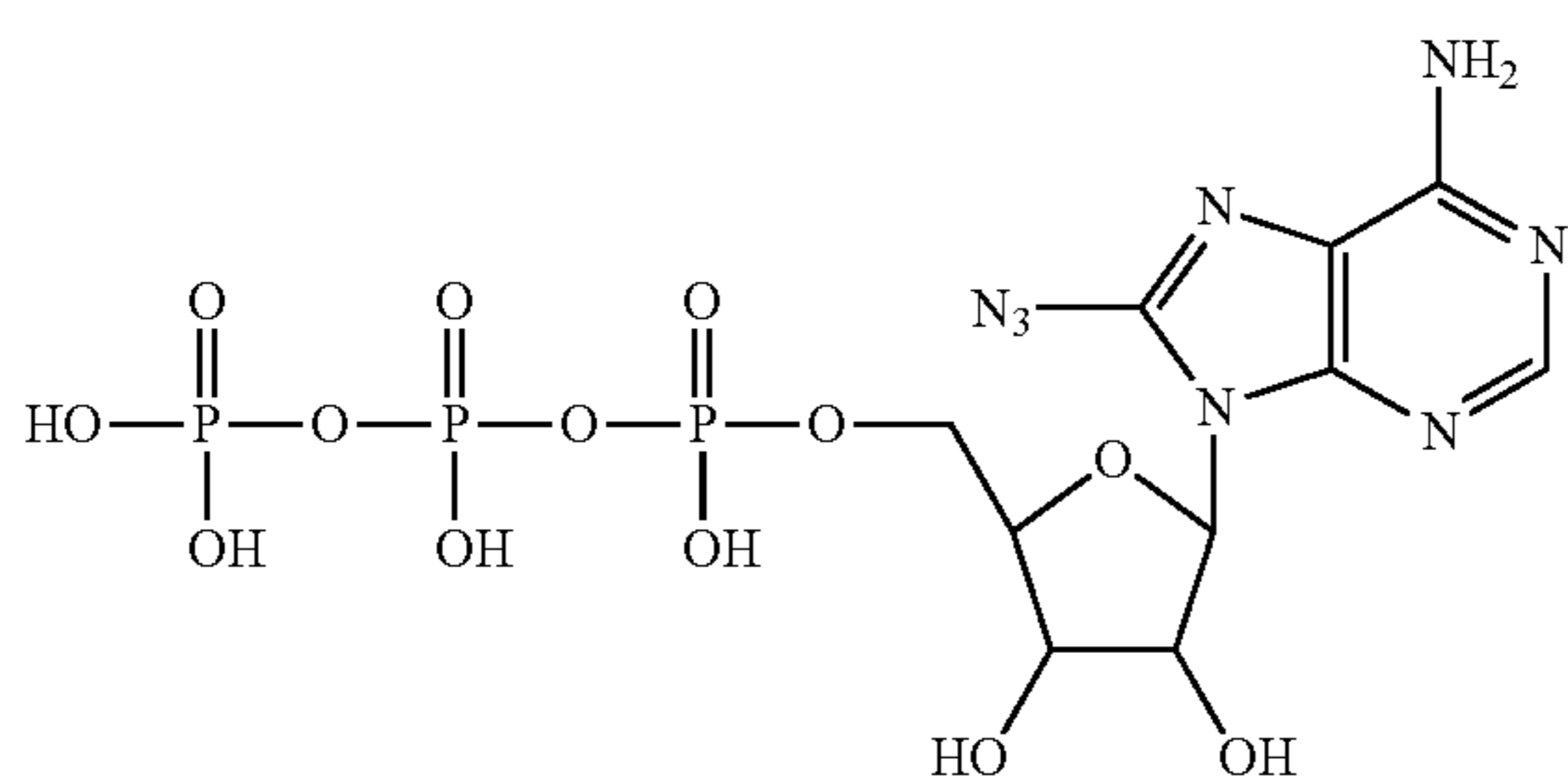
8-azido-adenosine-5'-triphosphate
