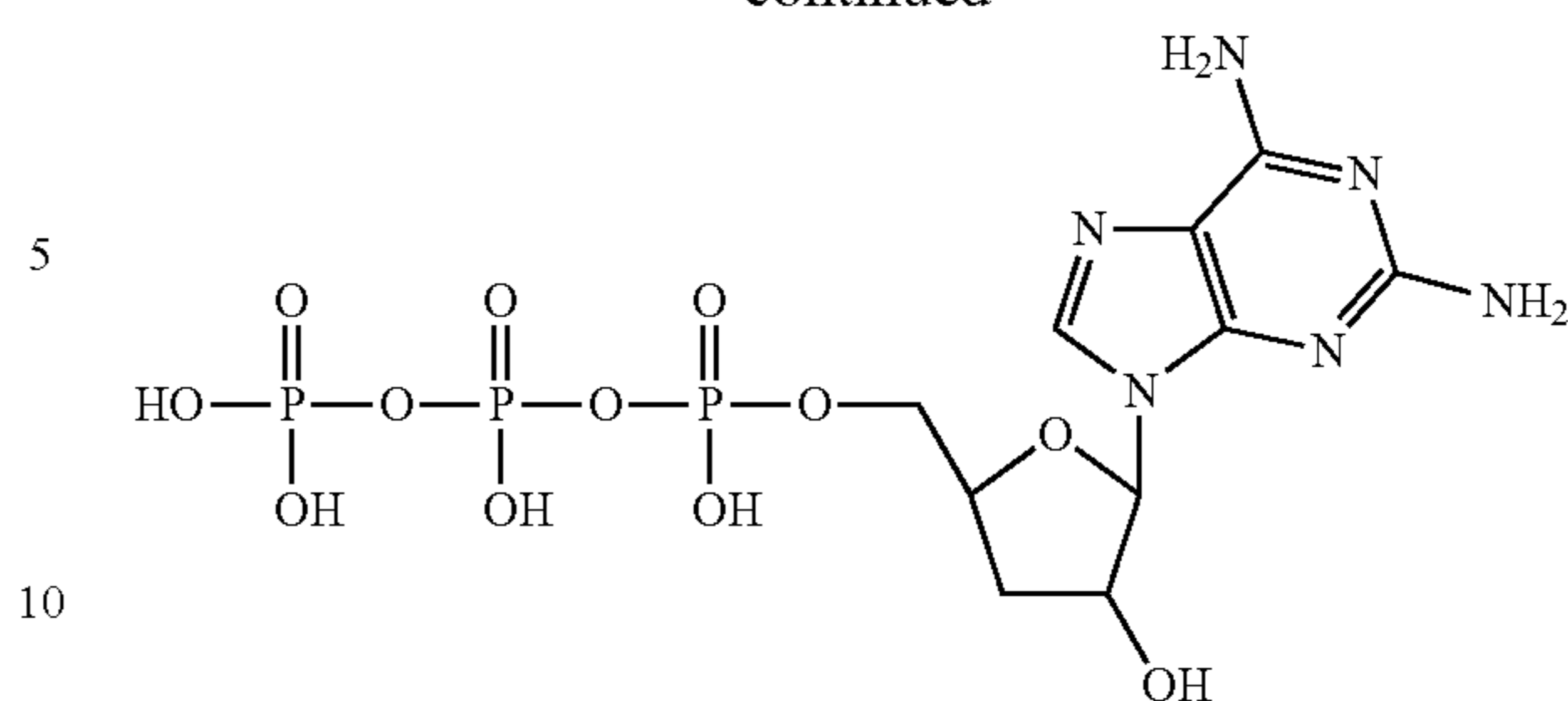
2-amino-3'-deoxyadenosine-5'-triphosphate
