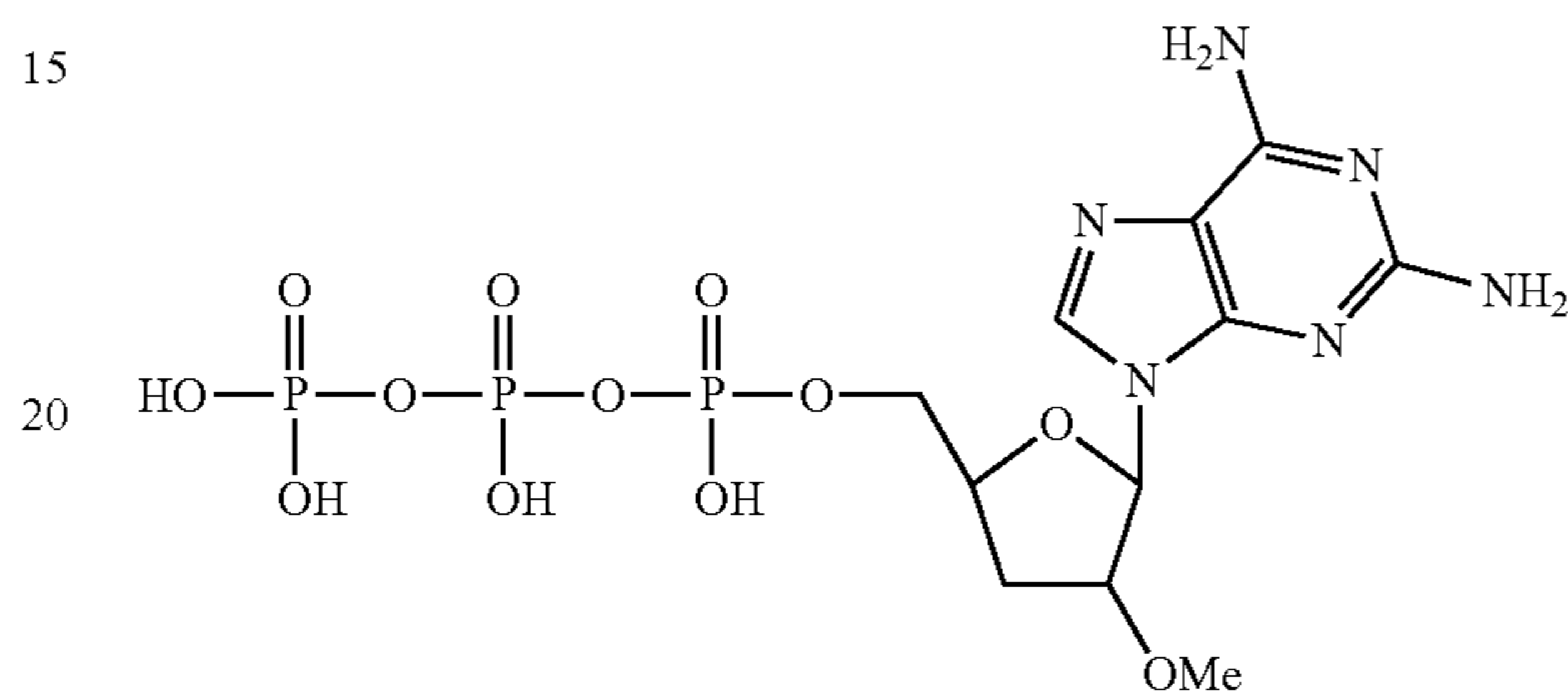
2'-methoxy-2',3'-dideoxy-2-amino-adenosine-5'-triphosphate
