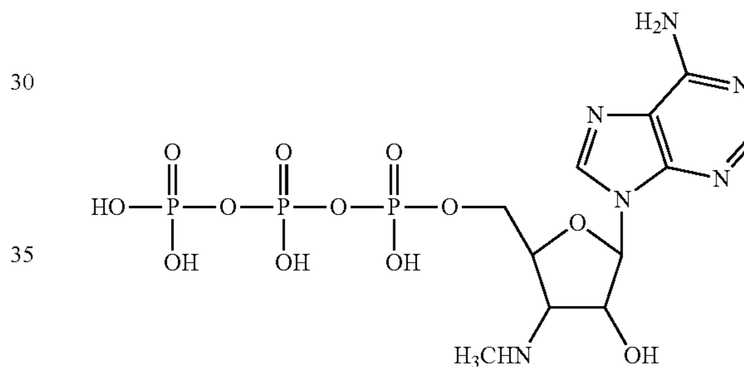
3'-methylamino-3'-deoxyadenosine-5'-triphosphate
