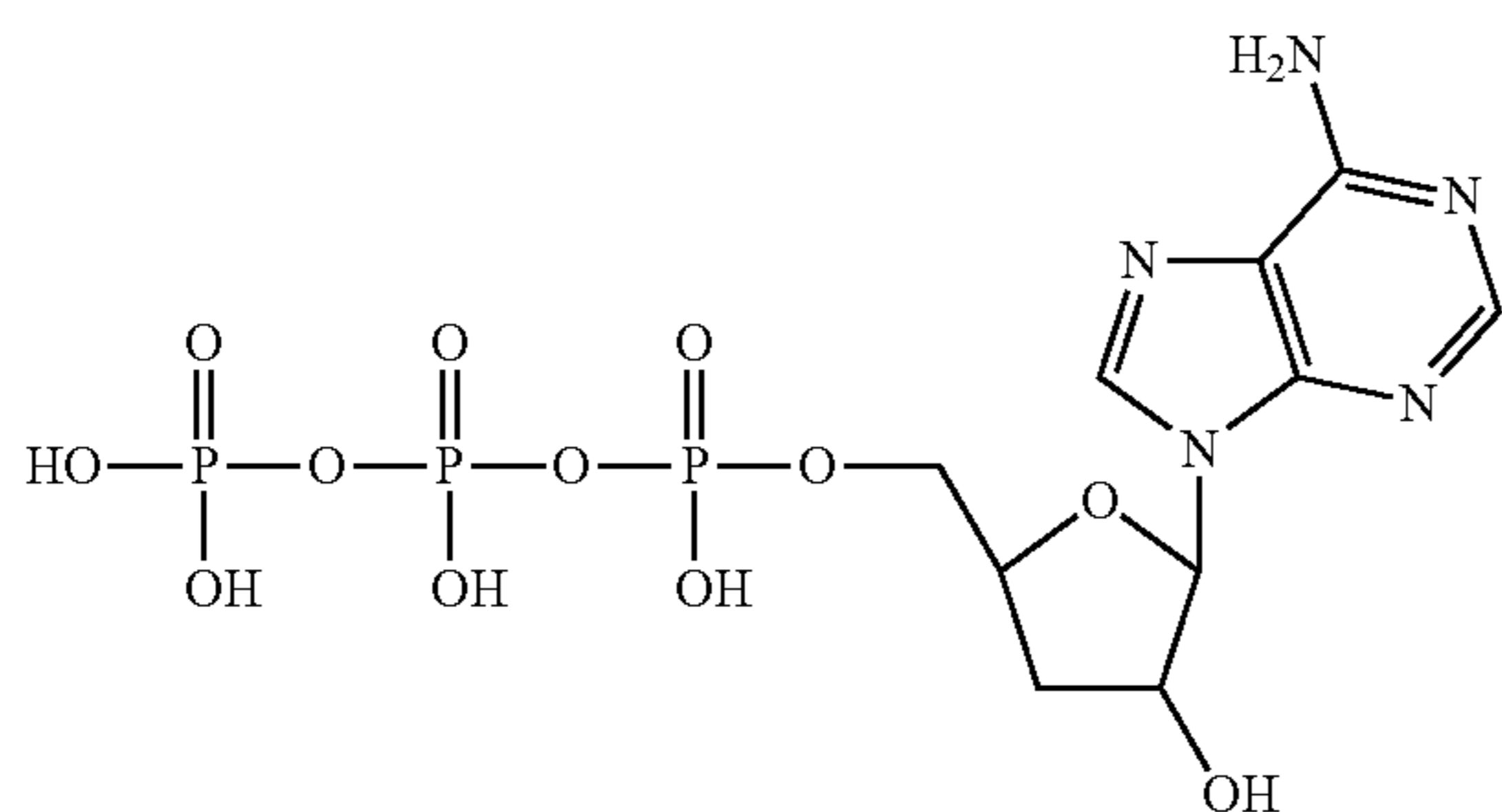
3'-deoxy-adenosine-5'-triphosphate
