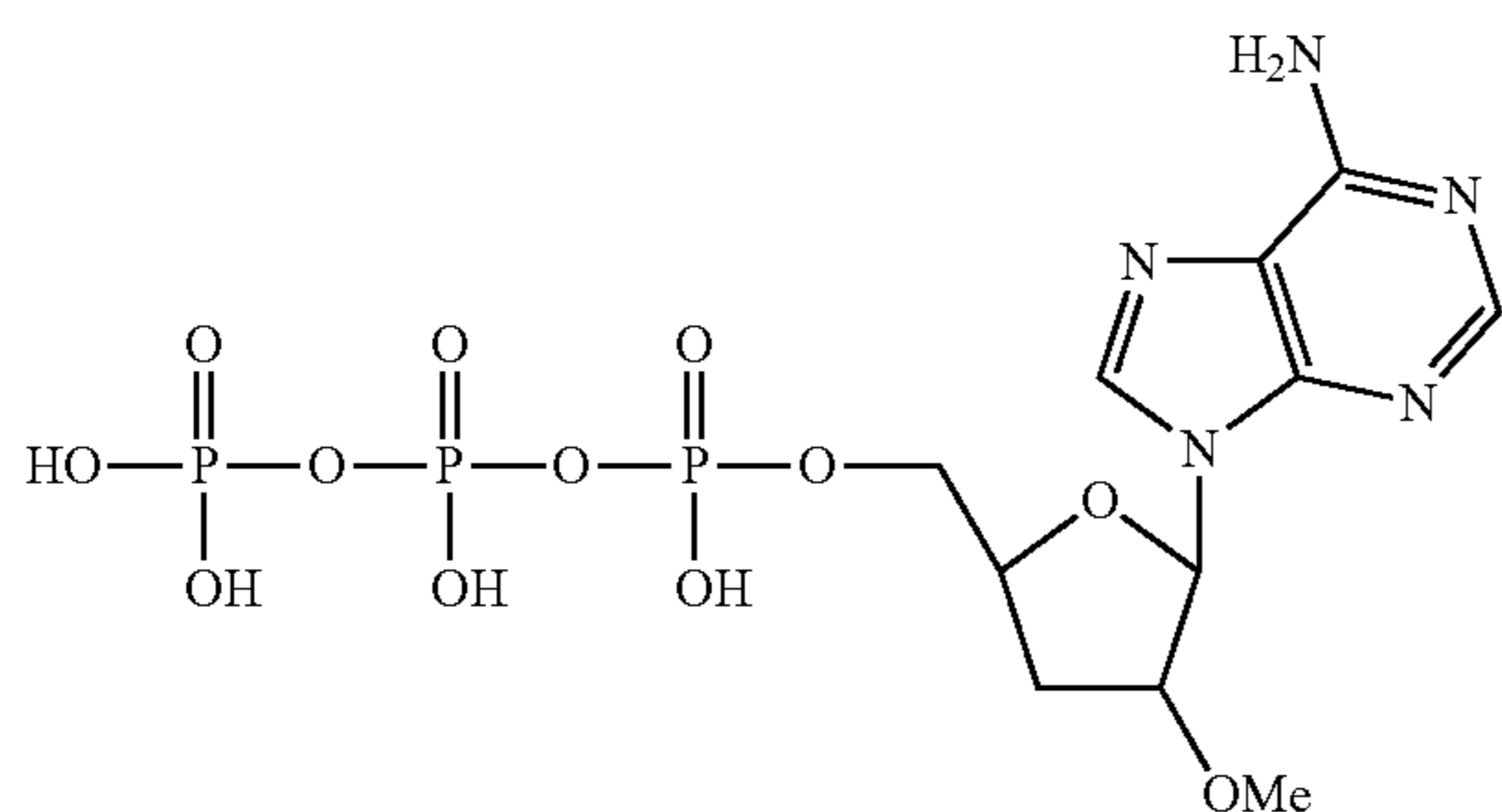
2'-methoxy-2',3'-dideoxy-adenosine-5'-triphosphate
