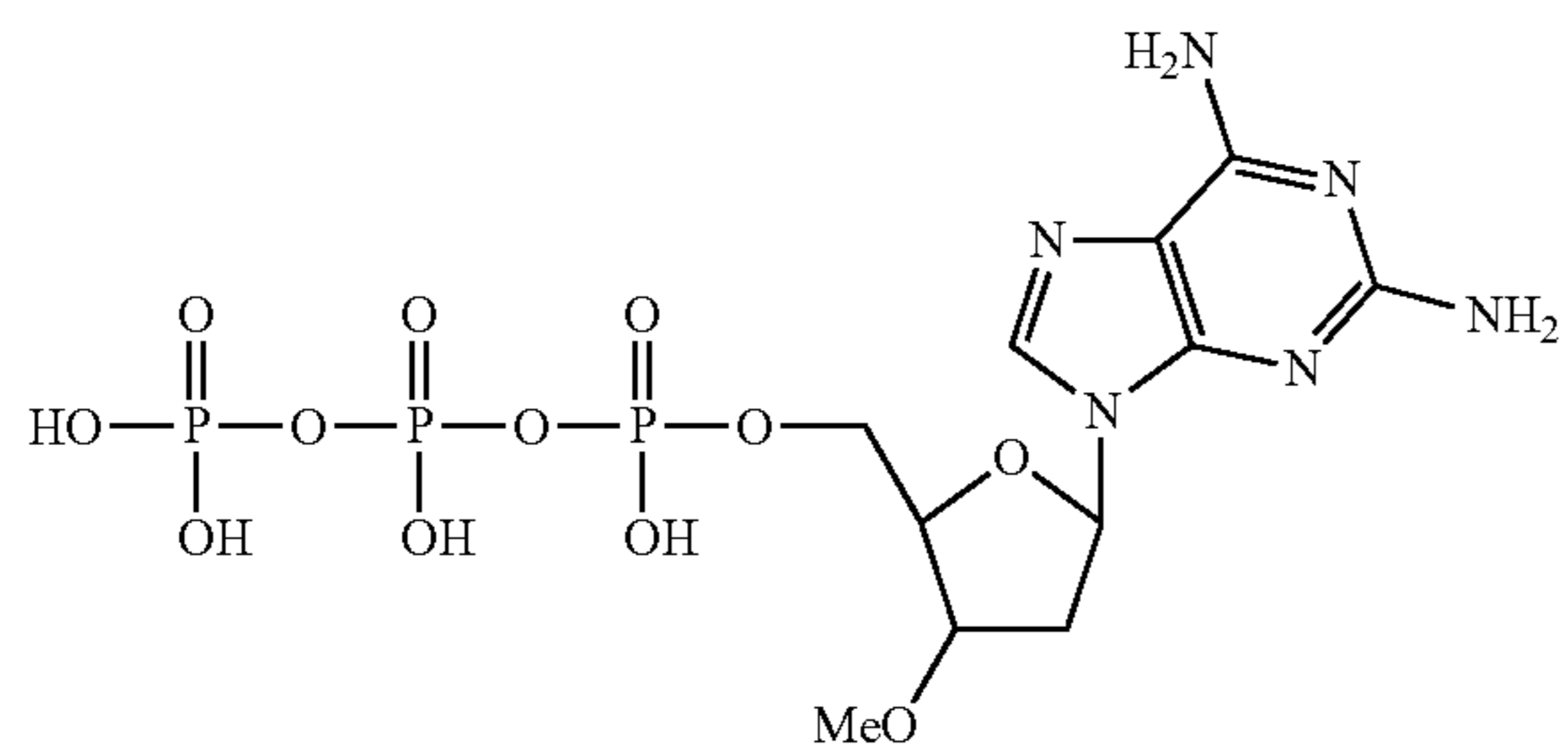
3'-methoxy-2',3'-dideoxy-2-amino-adenosine-5'-triphosphate
