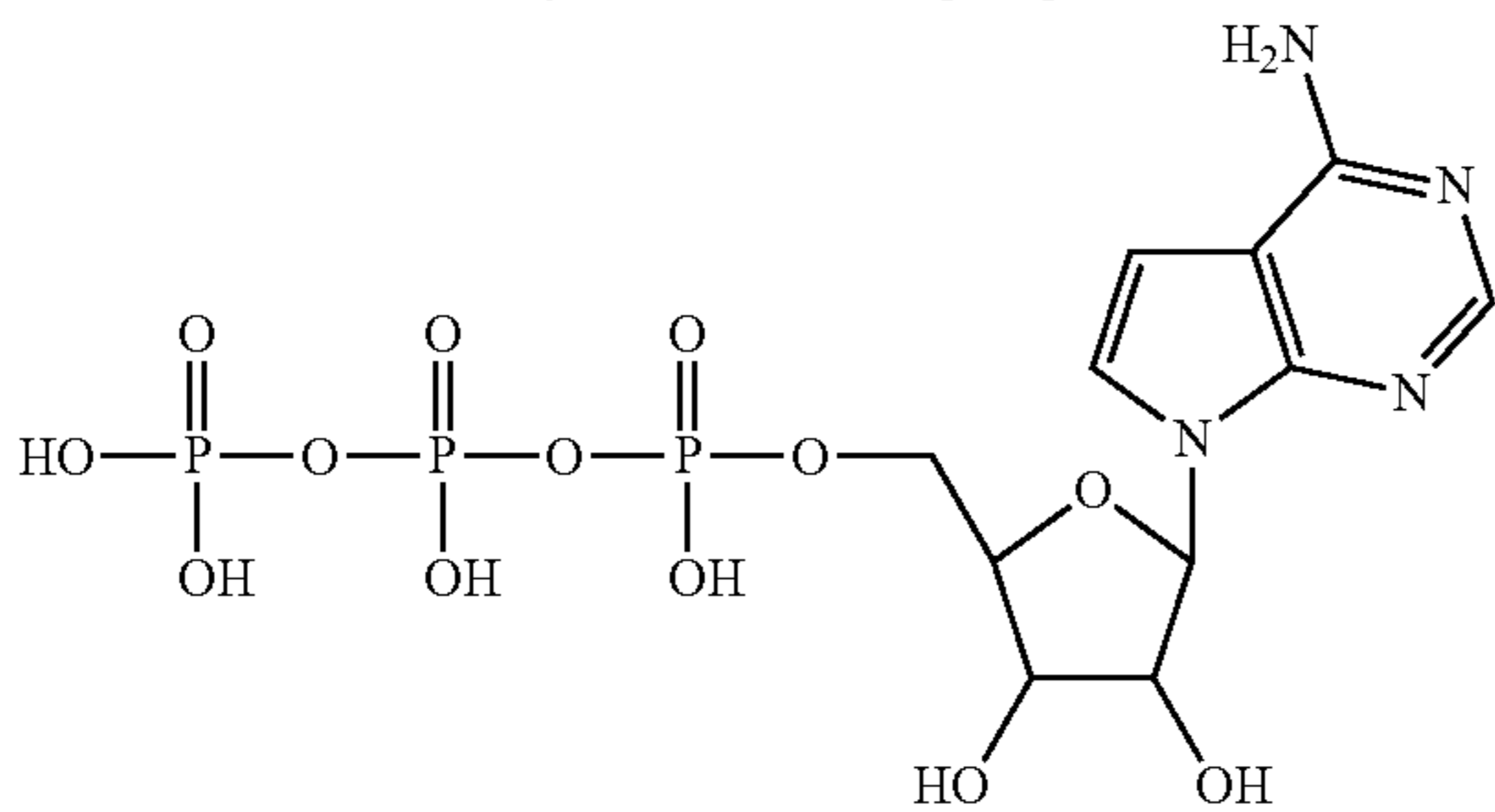
7-deaza-adenosine-5'-triphosphate
