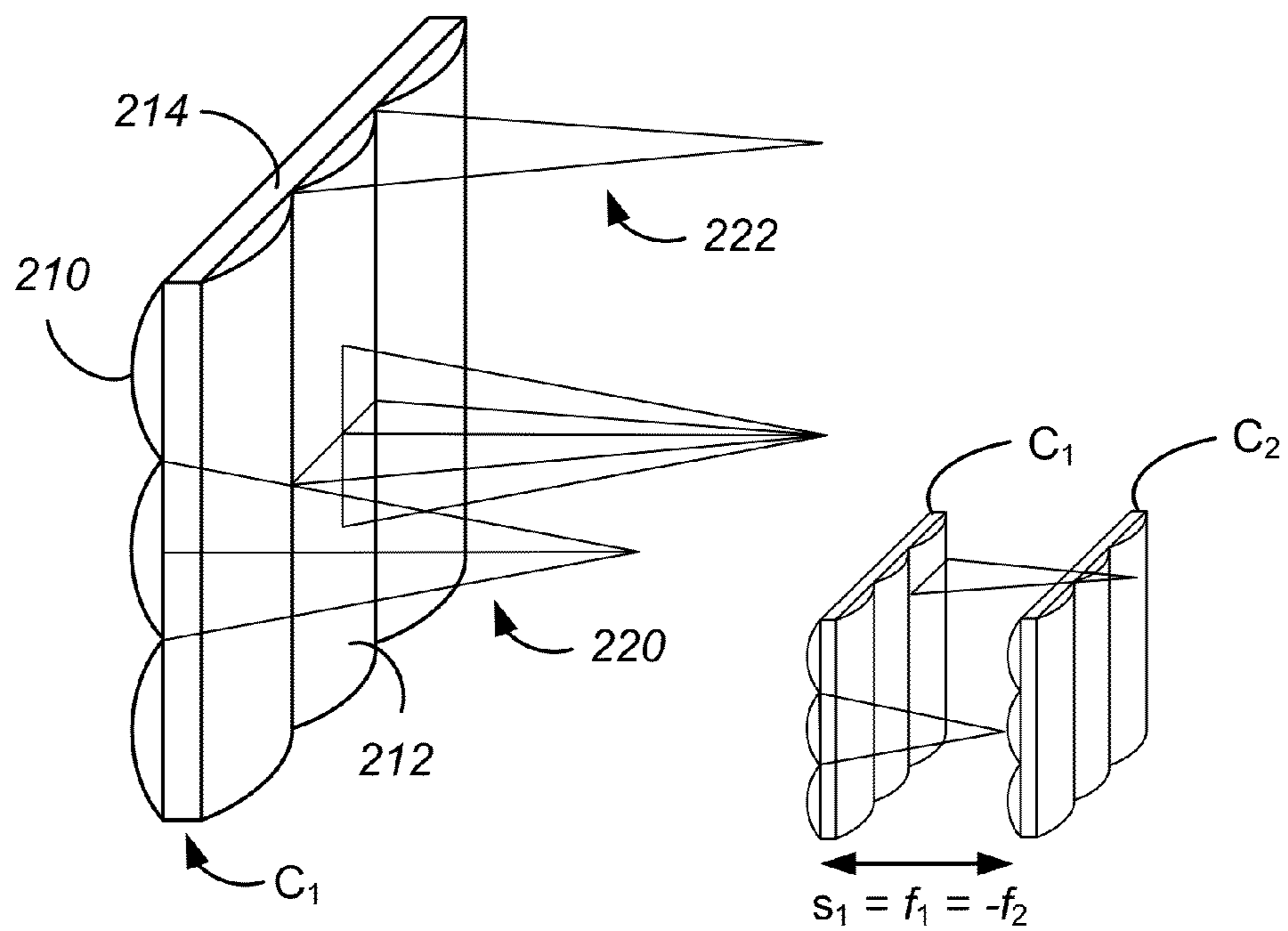
FIG. 2 (Prior Art)
