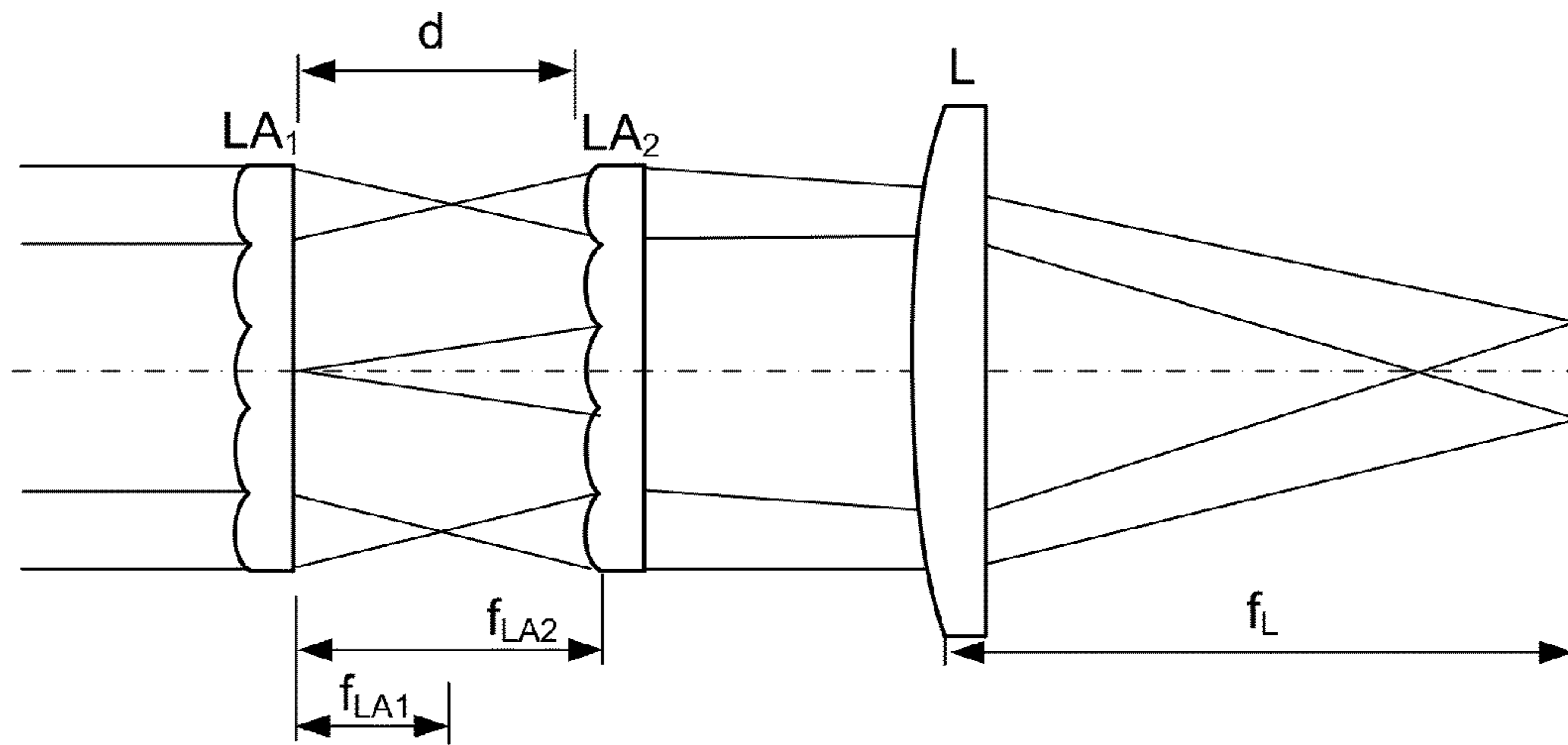
FIG. 1 (Prior Art)
