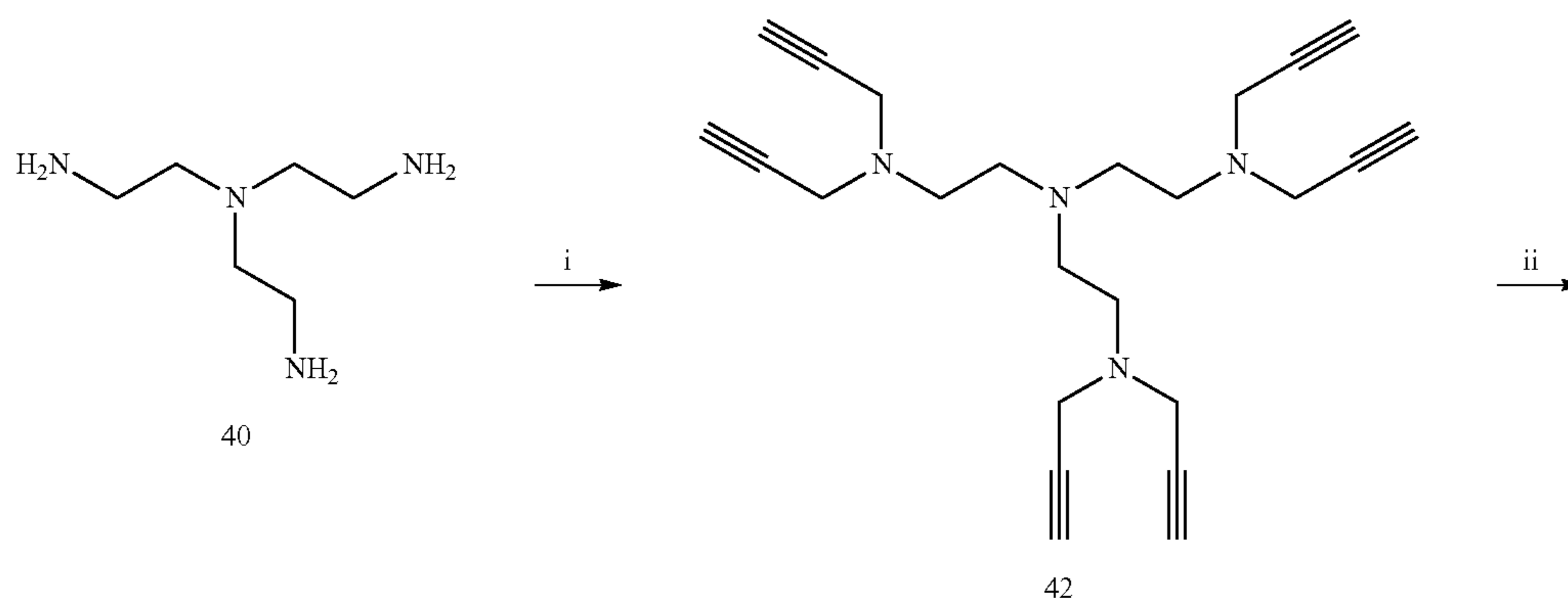
Scheme 14. Synthesis of a 'Click Reaction'-derived hexameric dendrimer.
