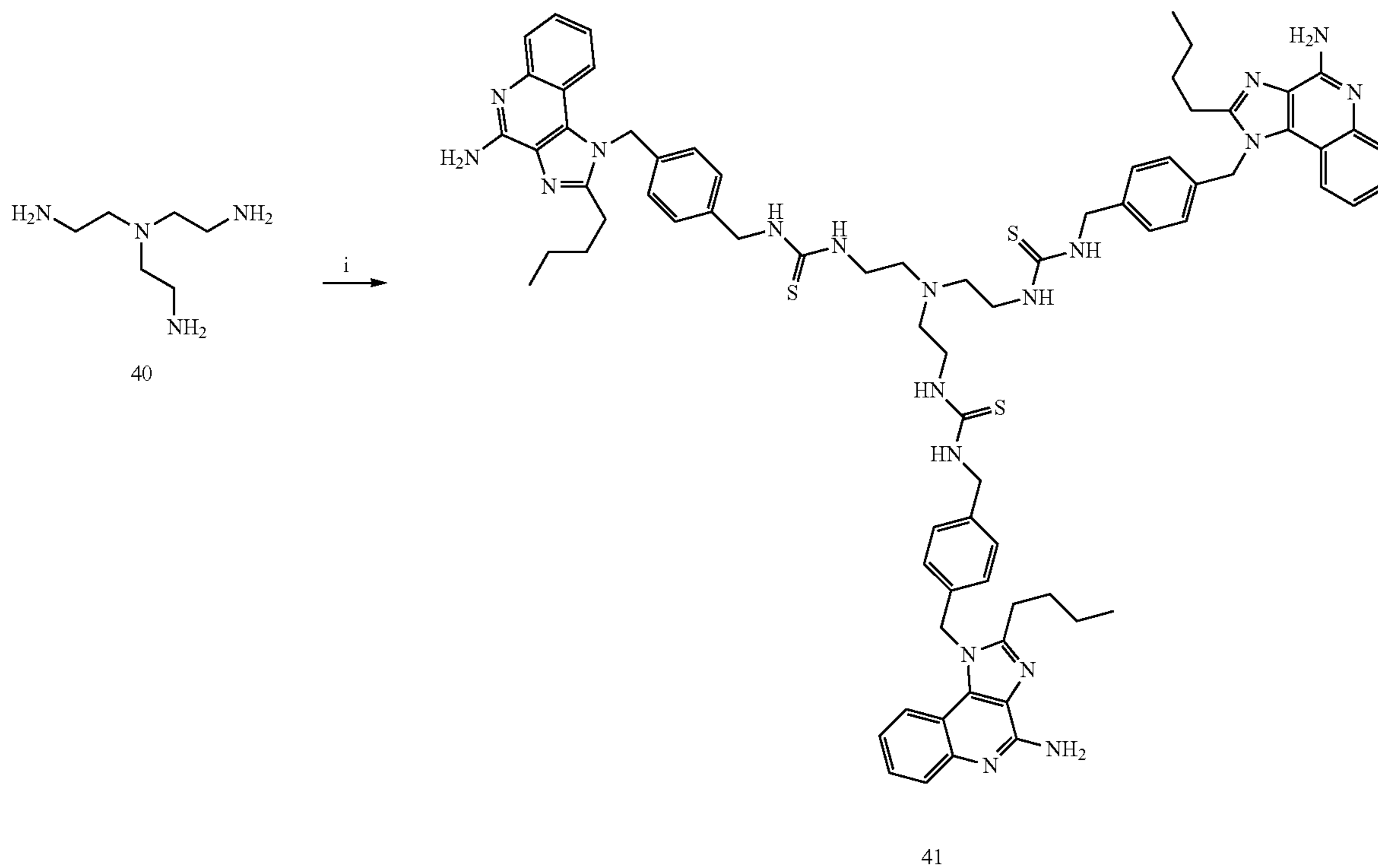
Scheme 13. Syntheses of the trimeric imidazoquinoline dendrimer.
