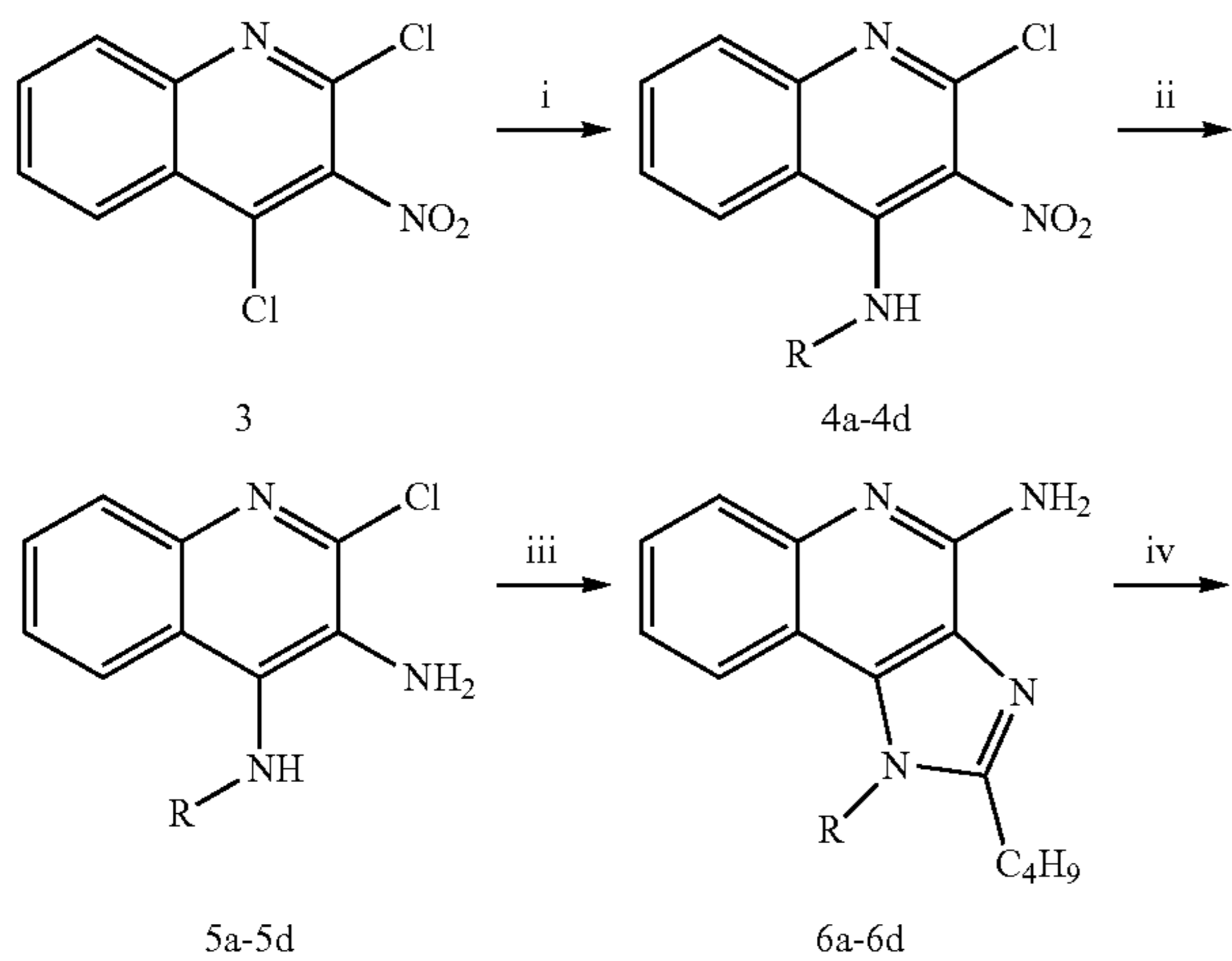
Scheme 1. Syntheses of N 1 -substituted imidazoquinolines.
