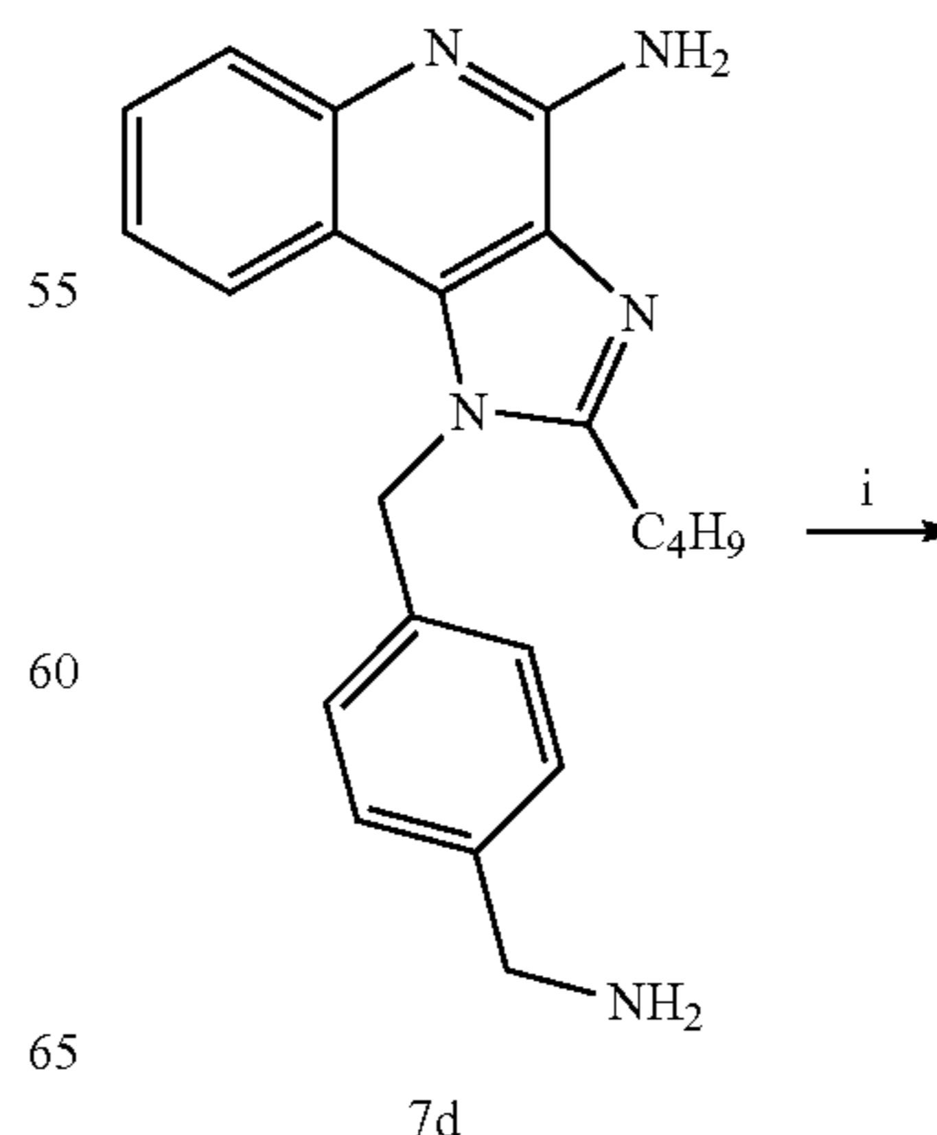
Scheme 18. Syntheses of imidazoquinoline dimers linked at C8-NH 2
