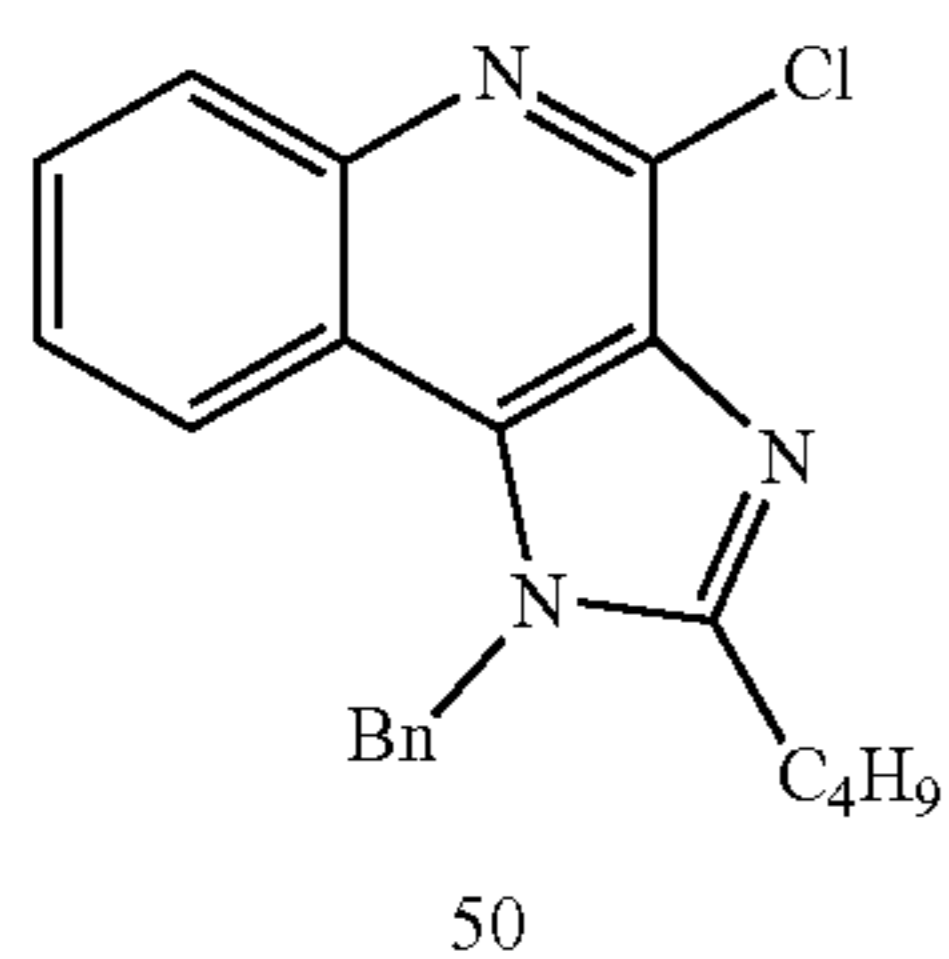
Scheme 16. Syntheses of imidazoquinoline dimers linked at C4-NH 2 .
