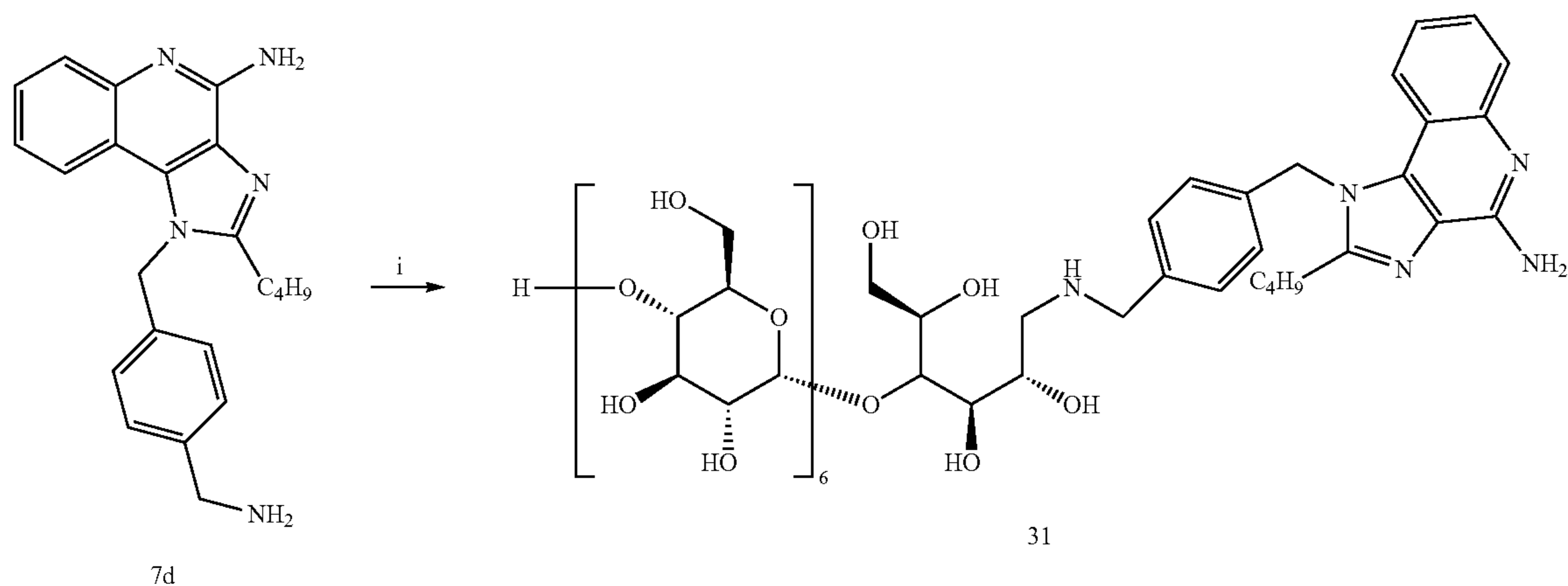
Scheme 8. Syntheses of maltoheptaose conjugate.
