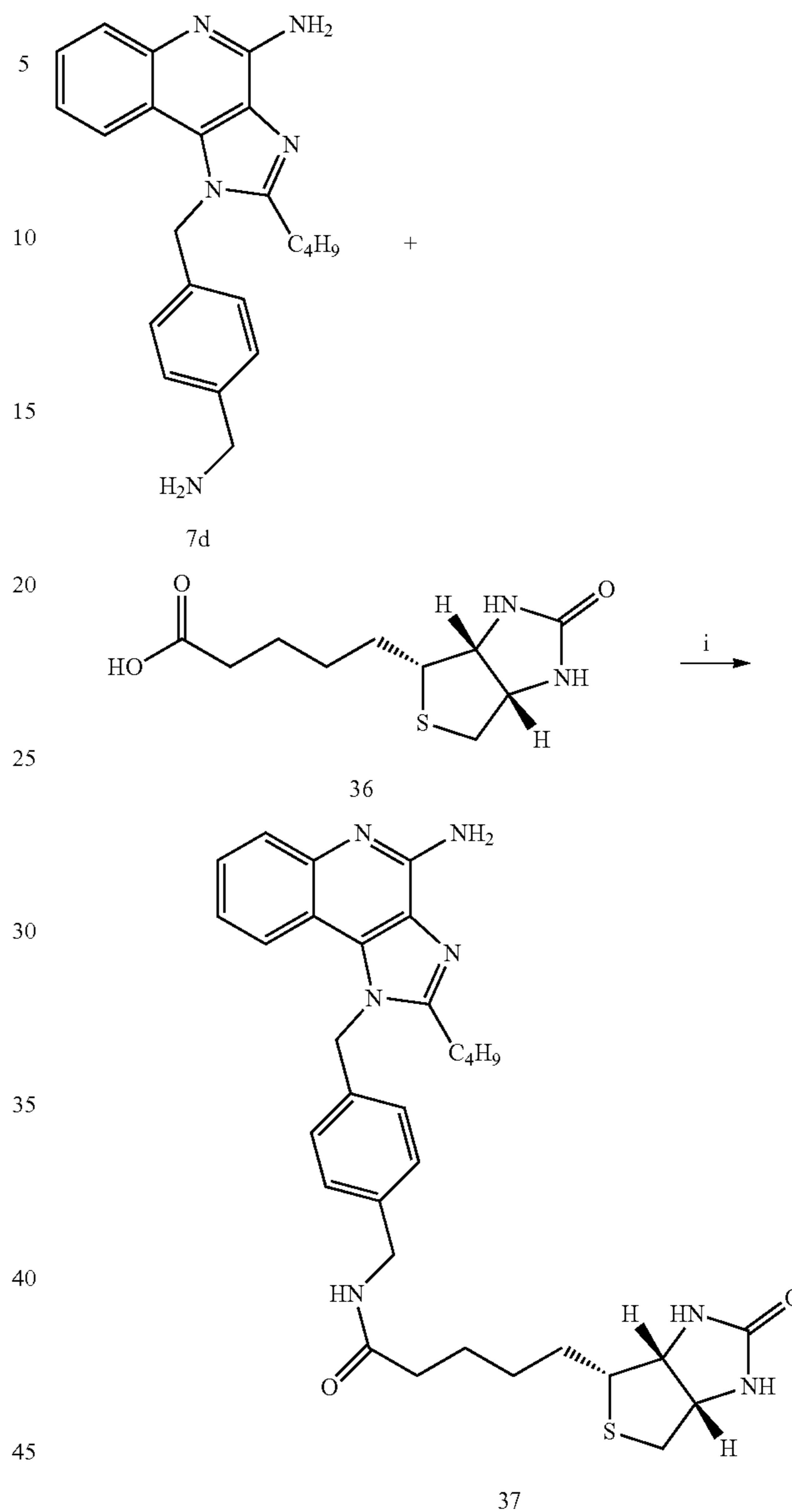
Scheme 11. Synthesis of a biotin derivative 37.
