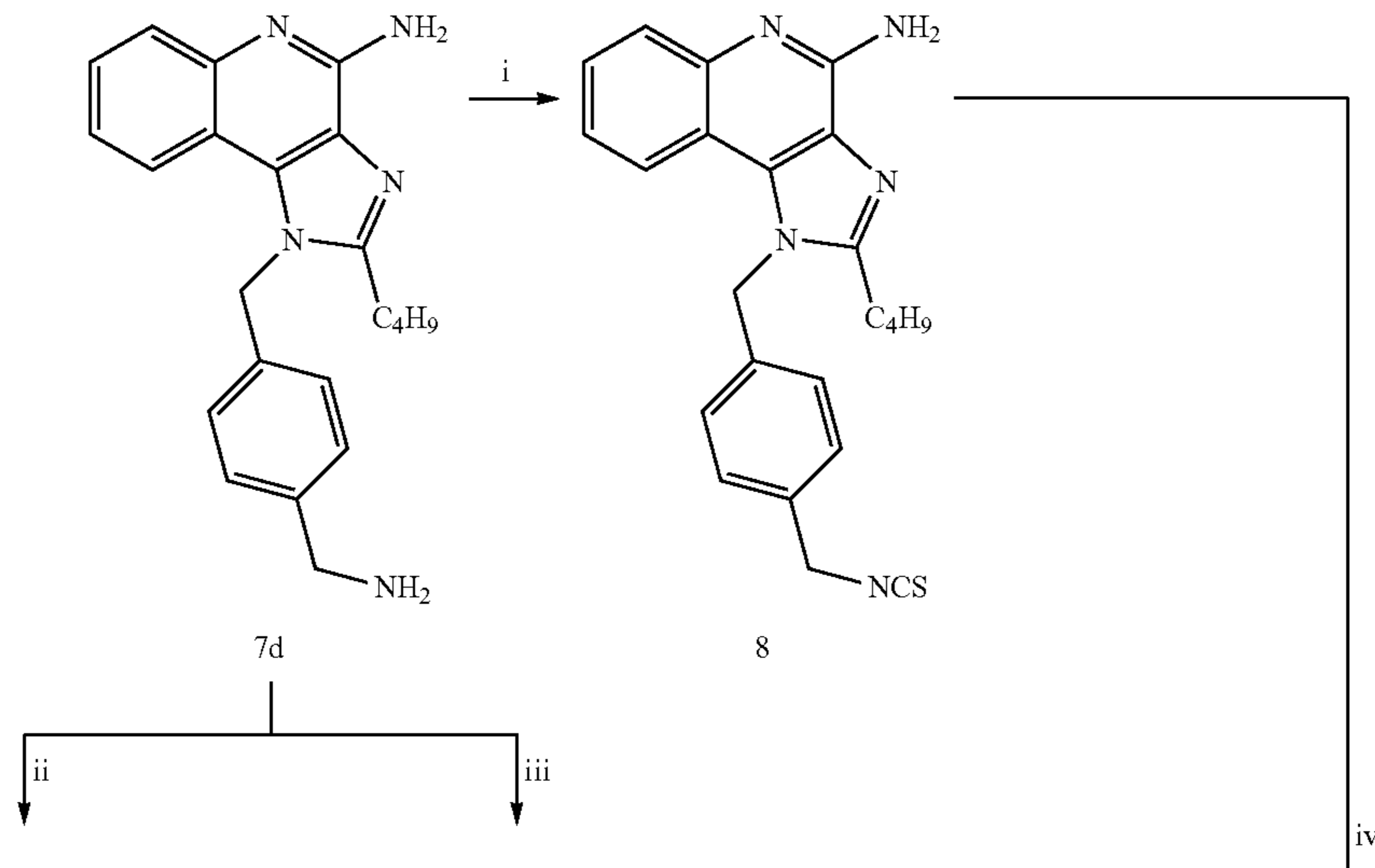
Scheme 6. Syntheses of fluorescent analogues of 7d.
