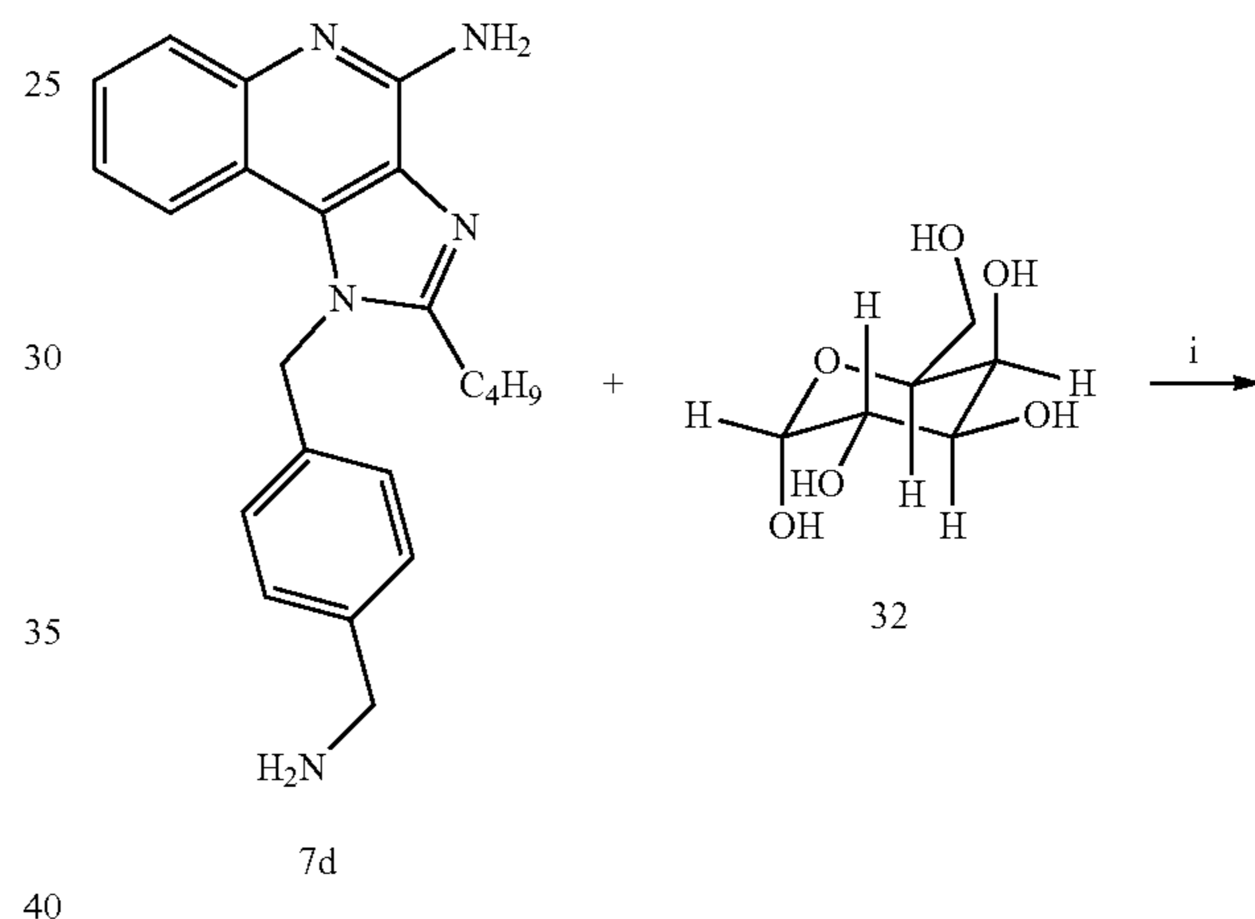
Scheme 9. Synthesis of a galactose derivative 33.
