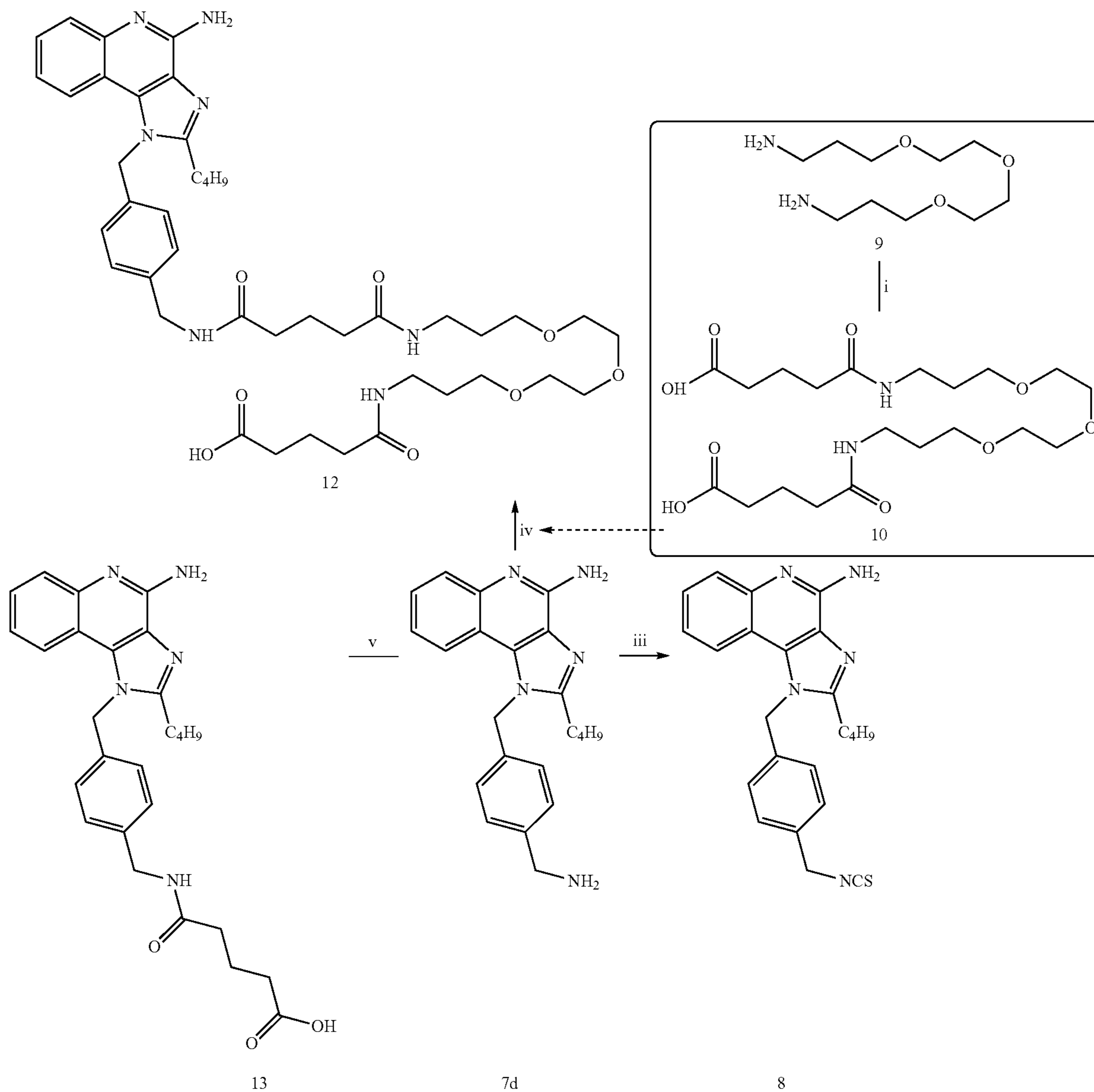
Scheme 2. Syntheses of derivatives of 7d.
