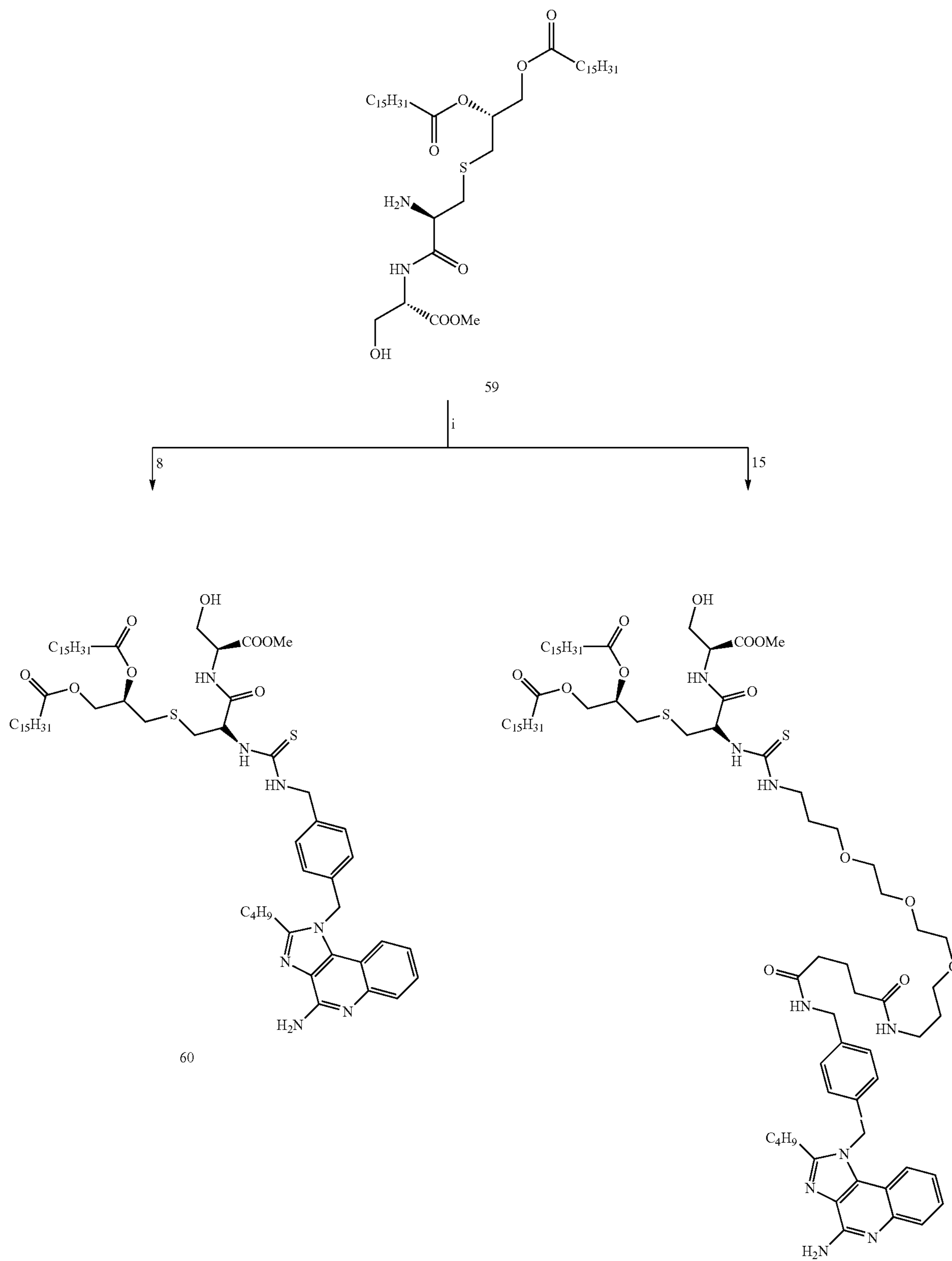
Scheme 20. Synthesis of thiourea-linked TLR-2/7 hybrid compounds 60 and 61.
