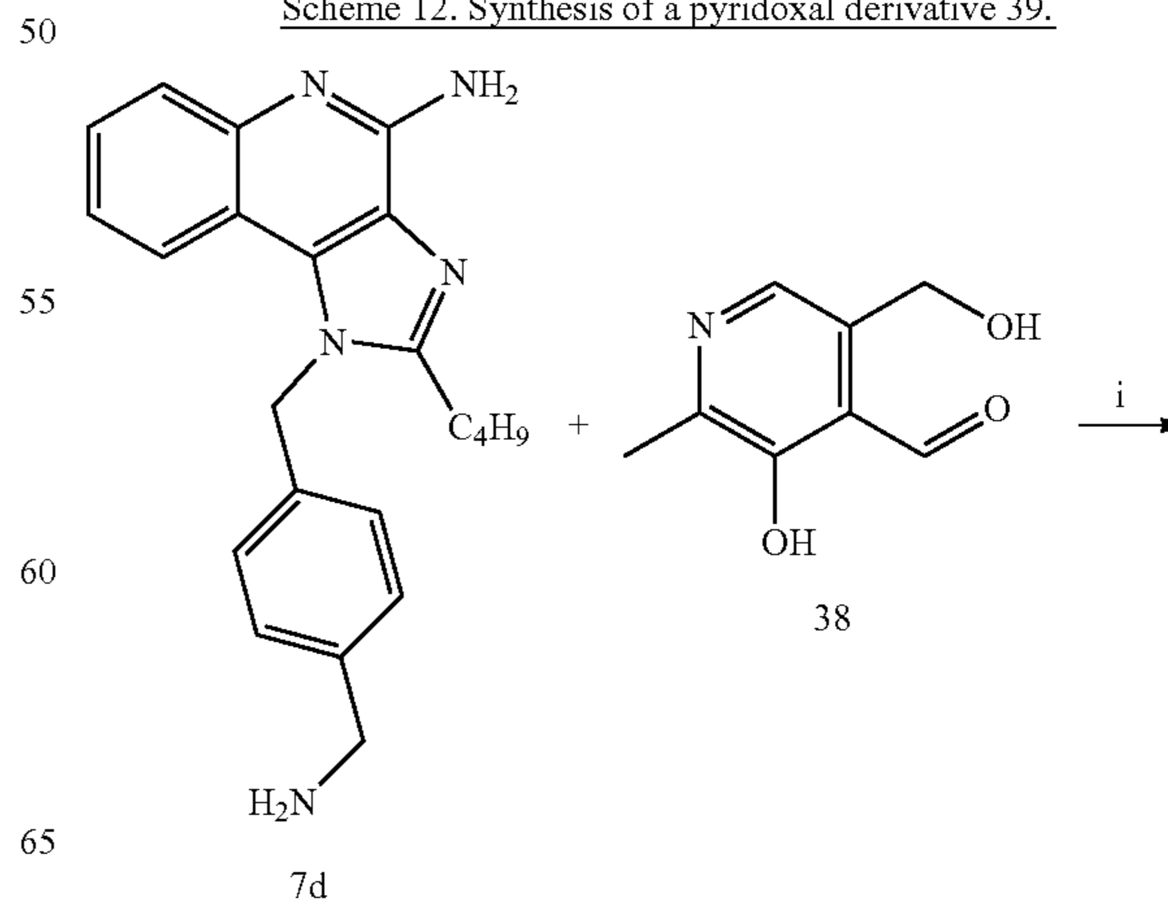
Scheme 12. Synthesis of a pyridoxal derivative 39.
