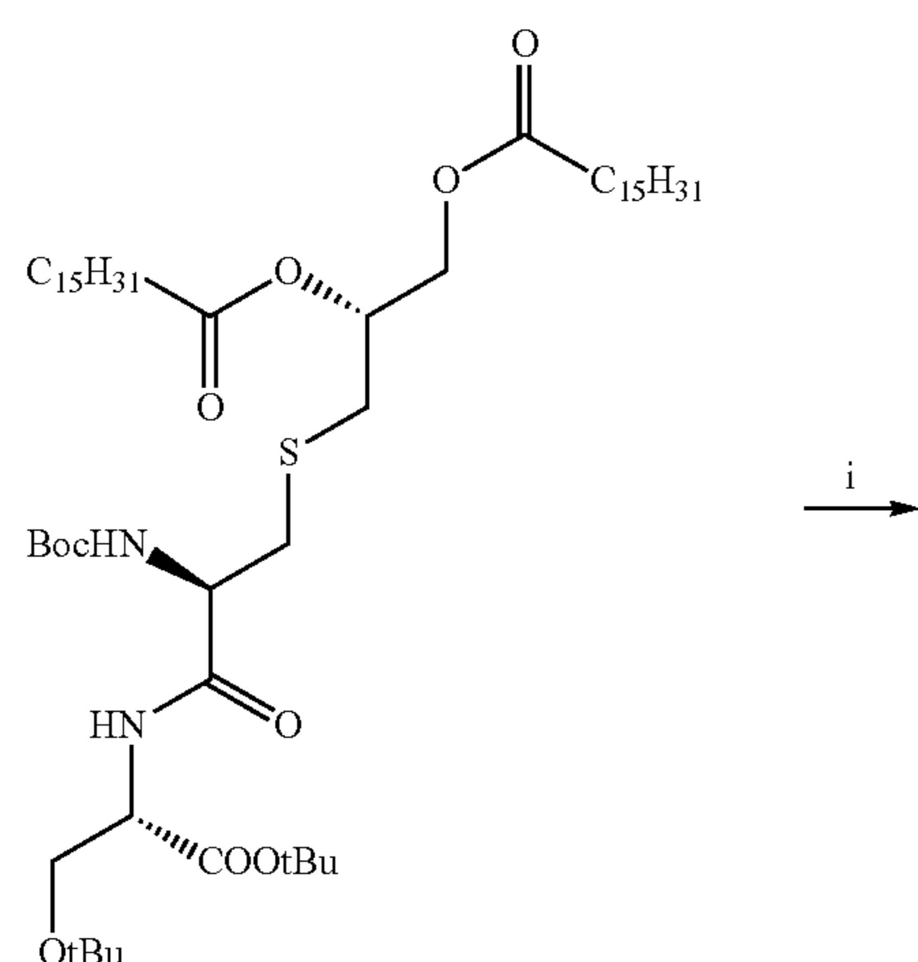
Scheme 19. Syntheses of derivatives of PAM 2 CS.
