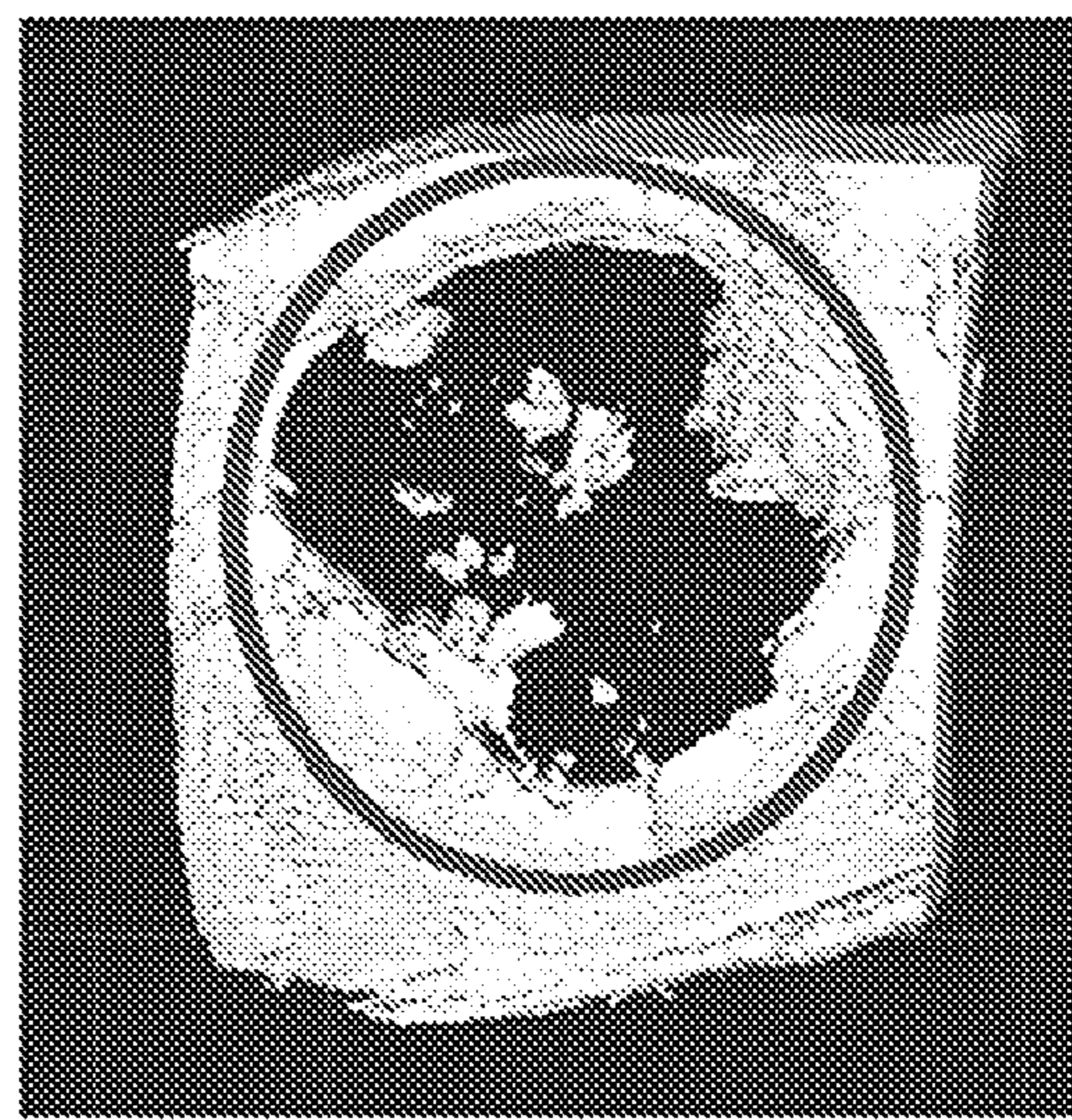
Condensed DNA
