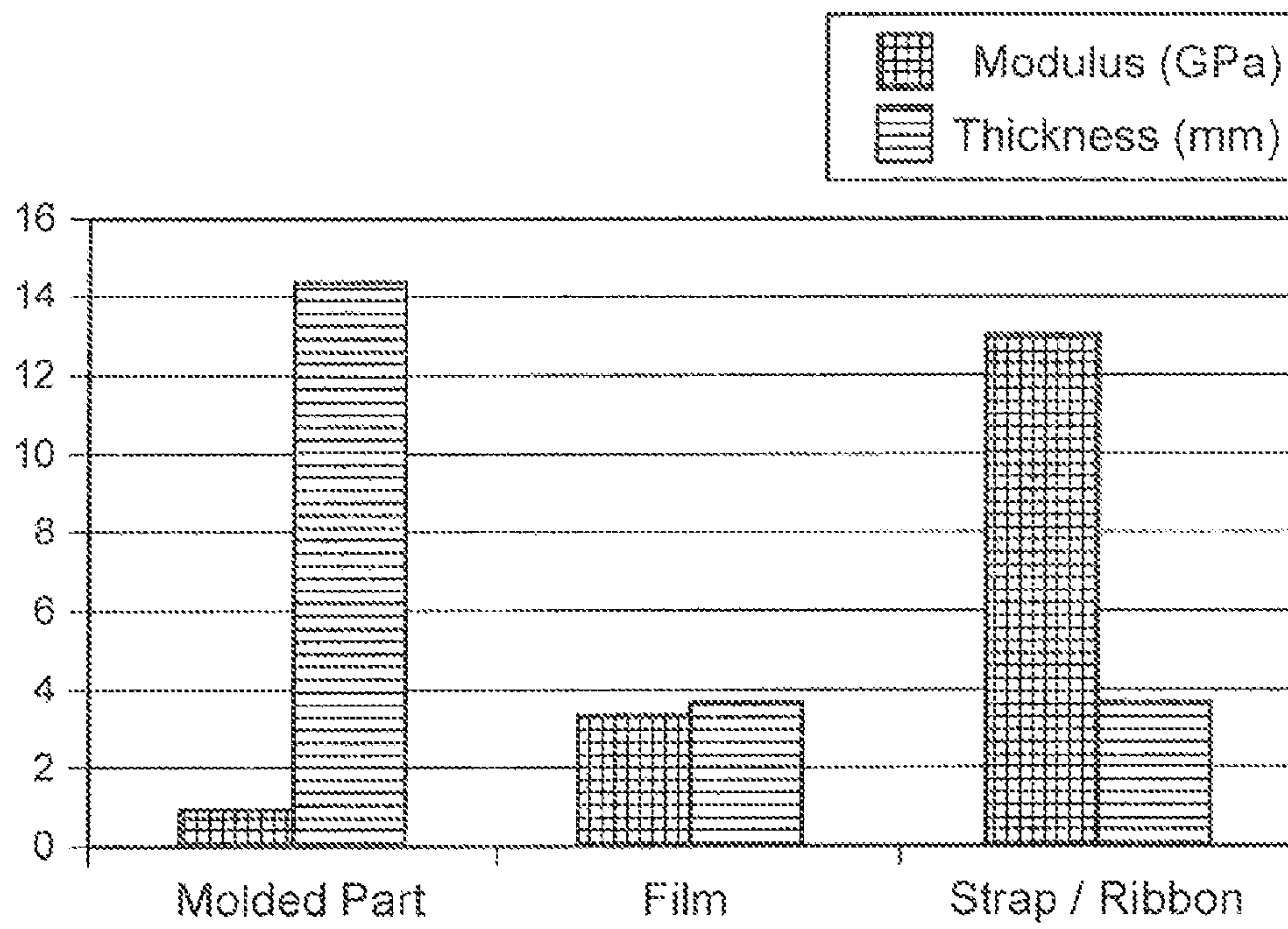
Thickness and Modulus for Equal Load & Width
