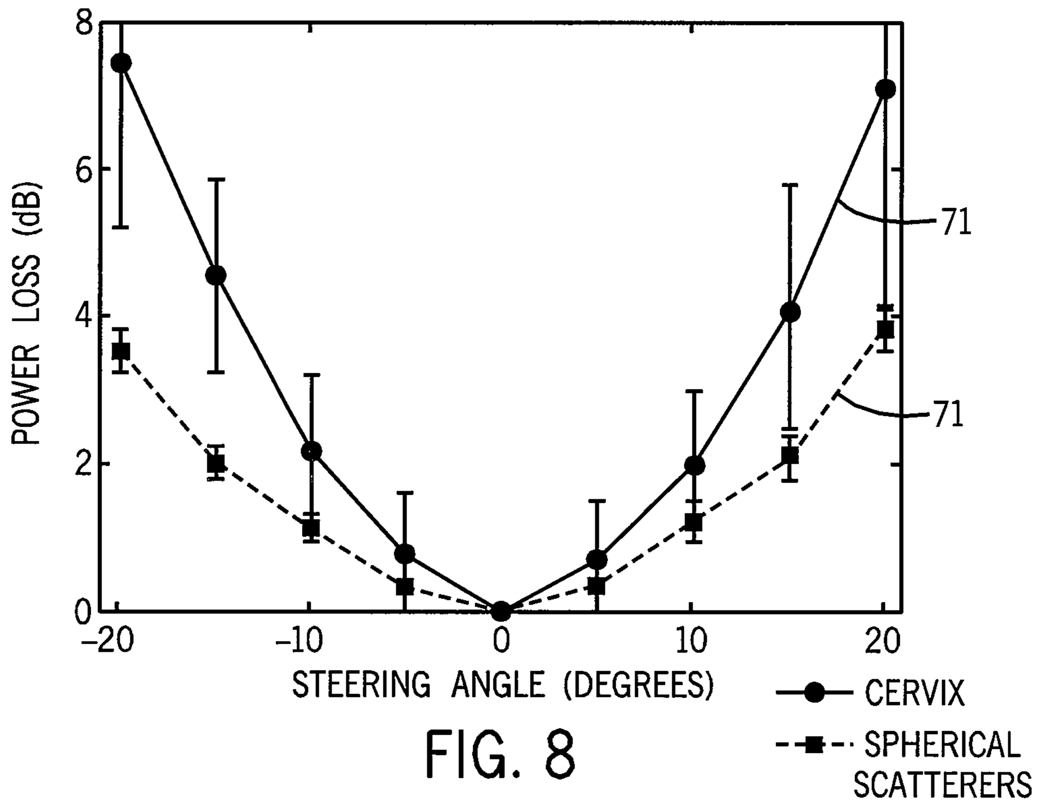
BACKSCATTERED POWER AT 9MHz CENTER FREQUENCY
