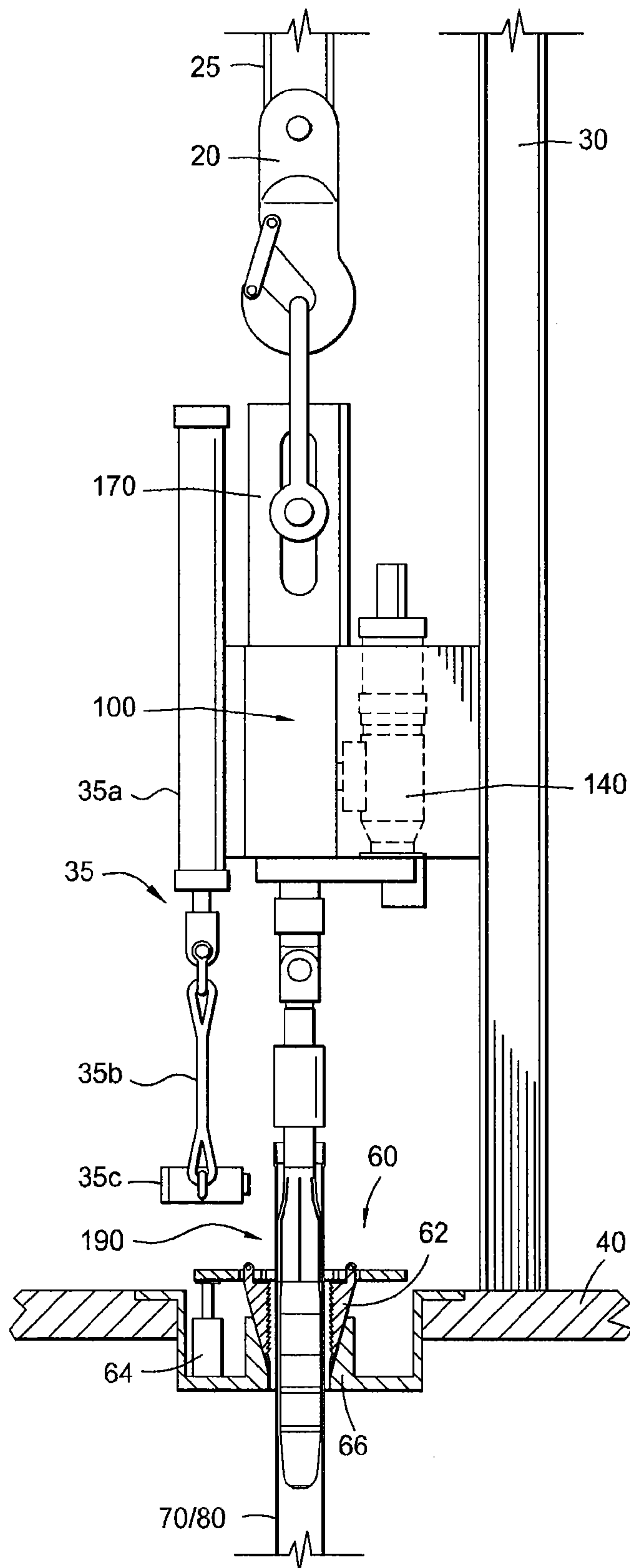
FIG. 1C (PRIOR ART)
