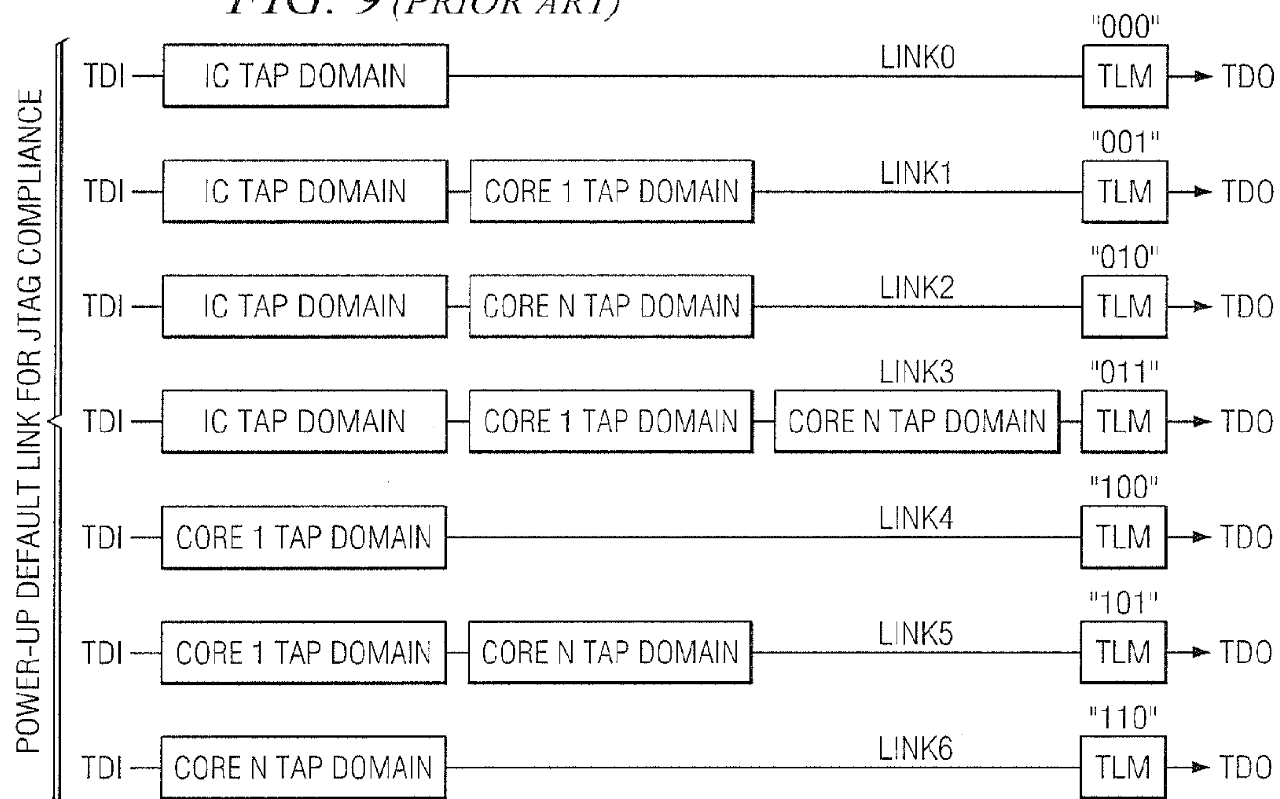
FIG. 9 (PRIOR ART)
