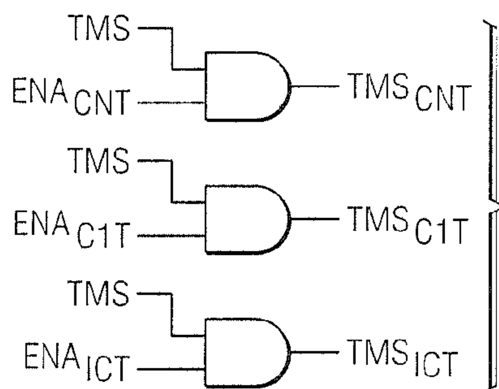
FIG. 5 (PRIOR ART)
