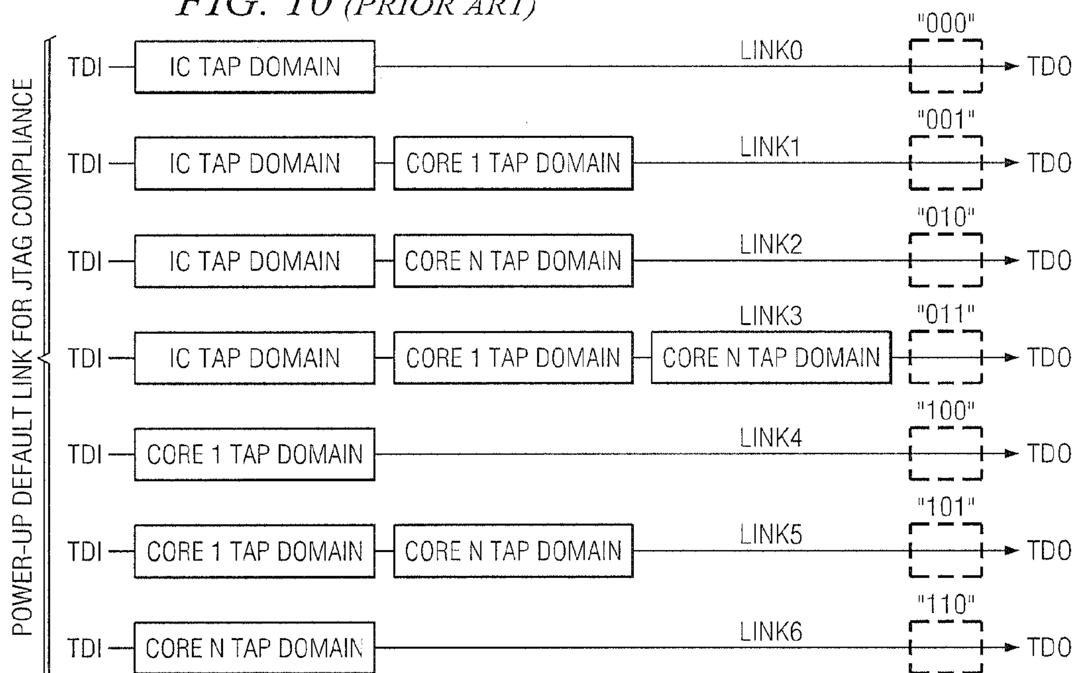
FIG. 10 (PRIOR ART)
