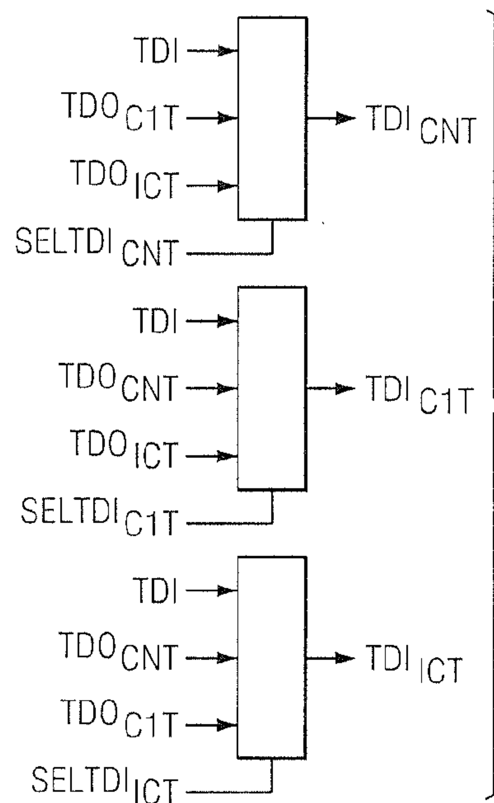
FIG. 6 (PRIOR ART)
