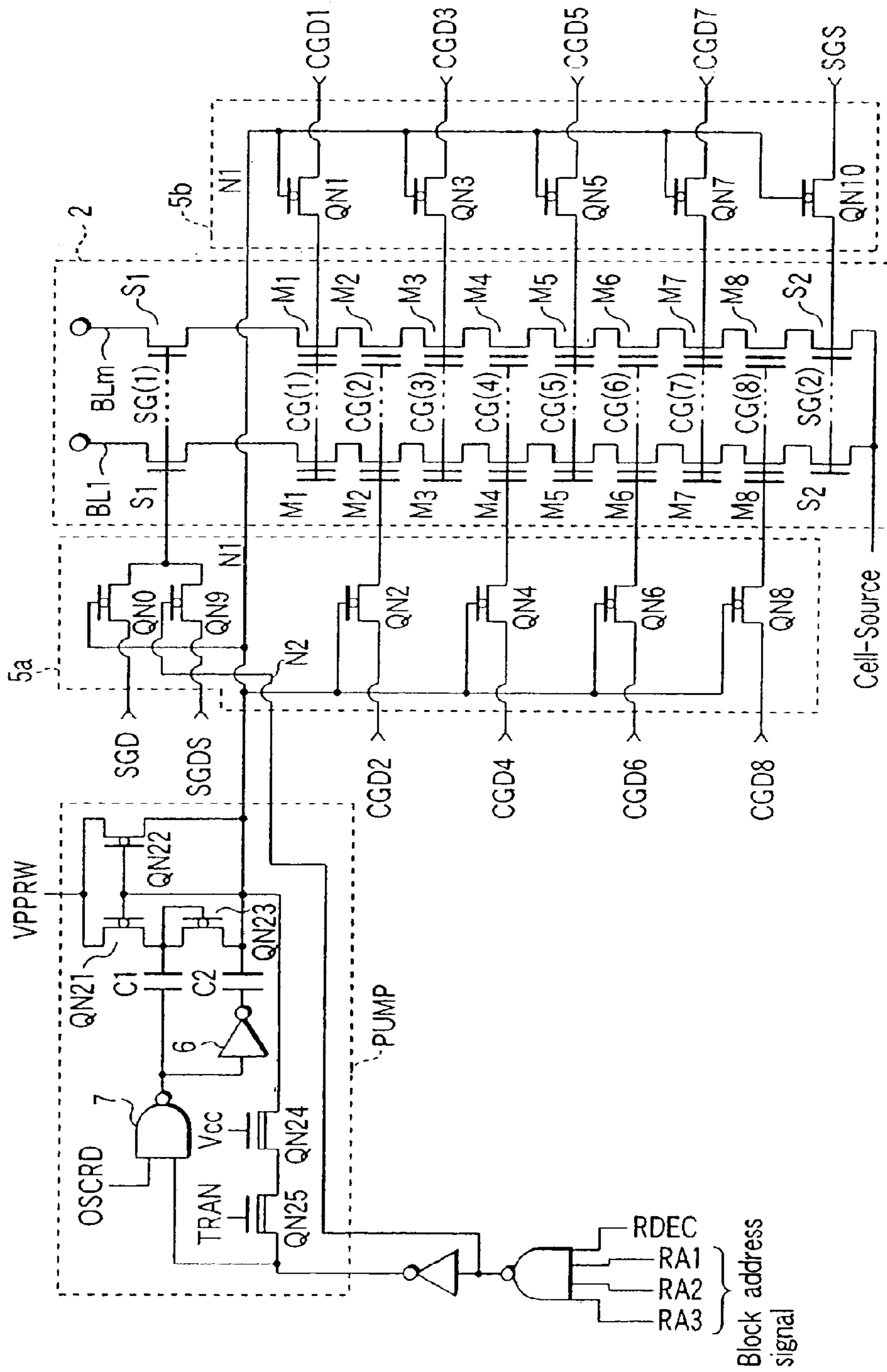
FIG. 2 PRIOR ART
