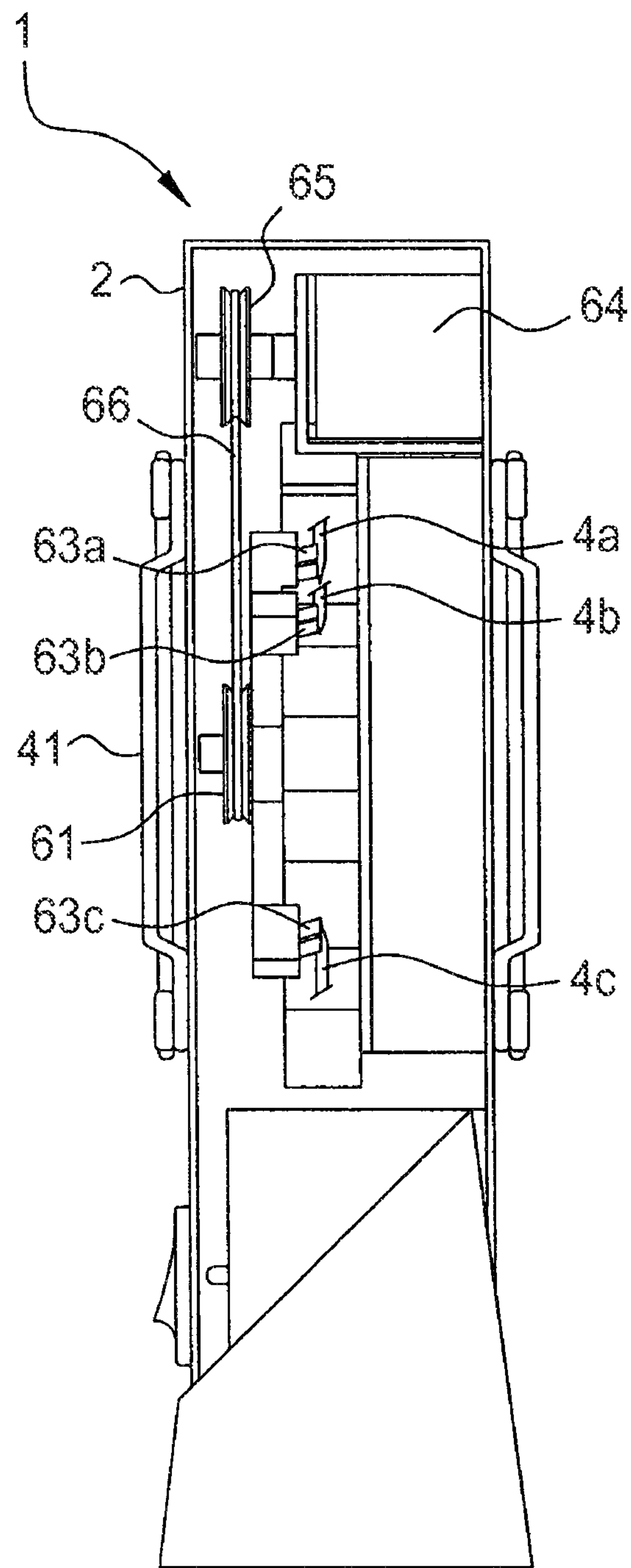
II - II SECTION
