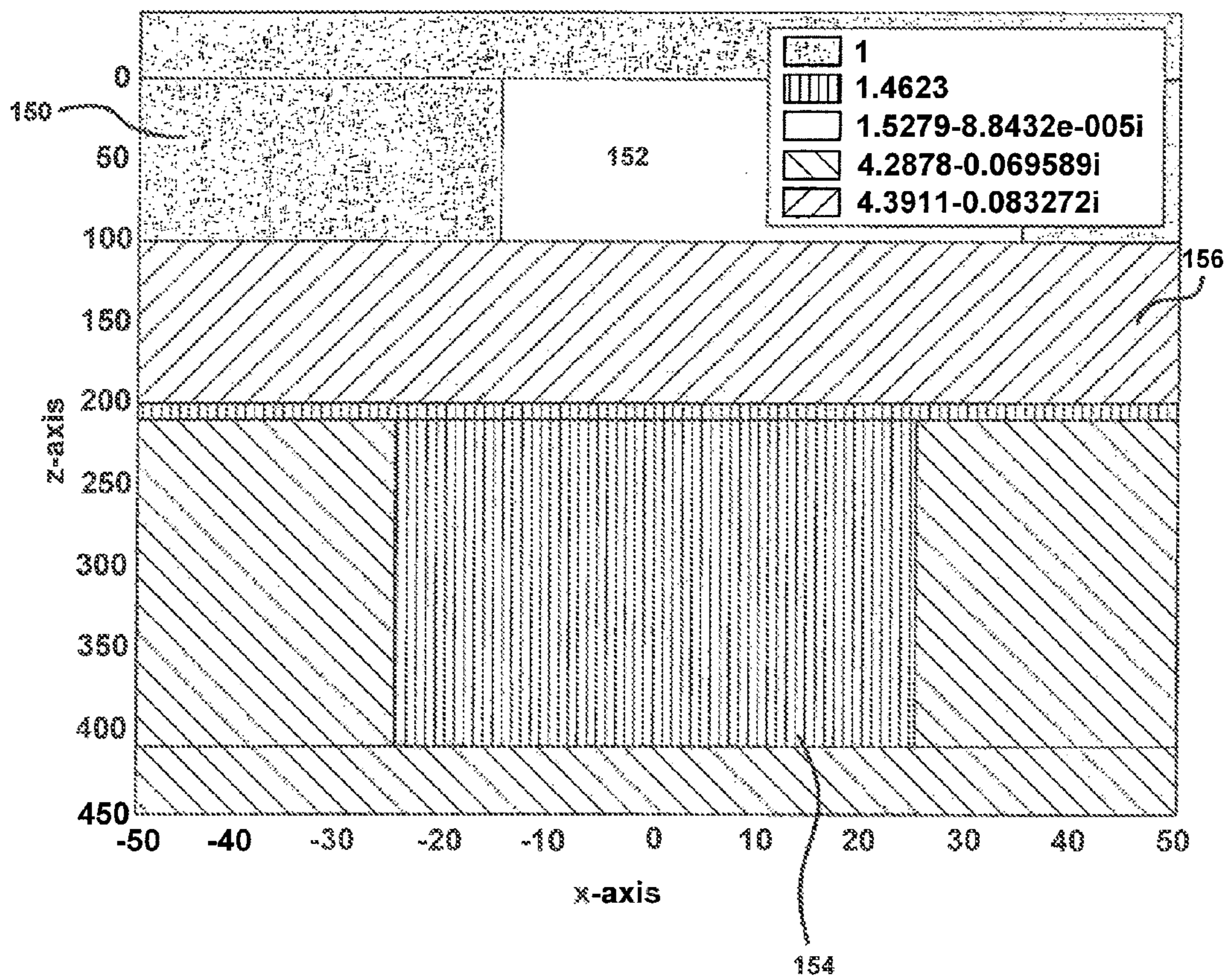
Grating structure with colour-coded refraction indices
