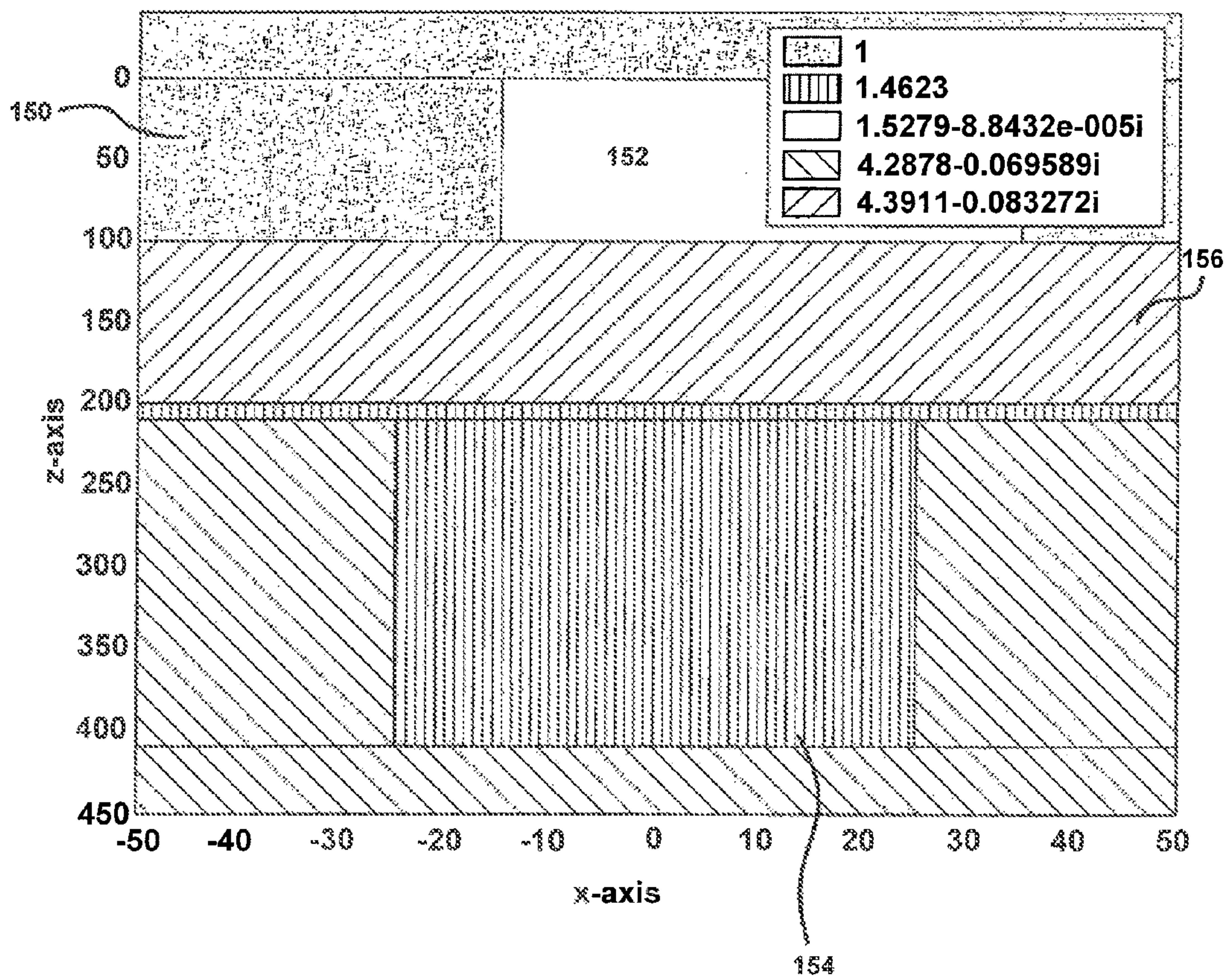
Grating structure with colour-coded refractive indices
