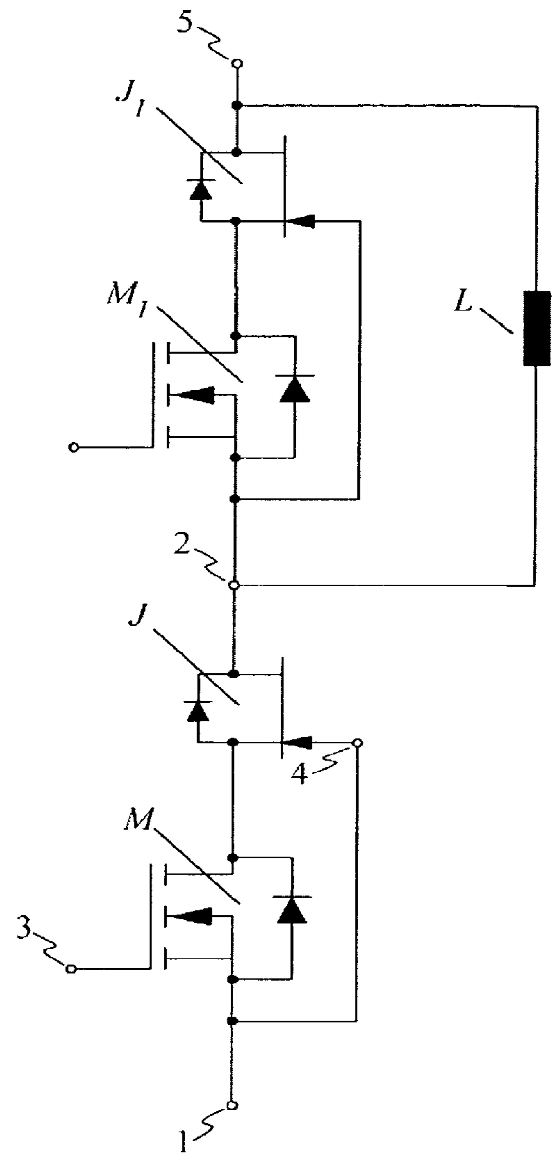
Fig. 2 PRIOR ART
