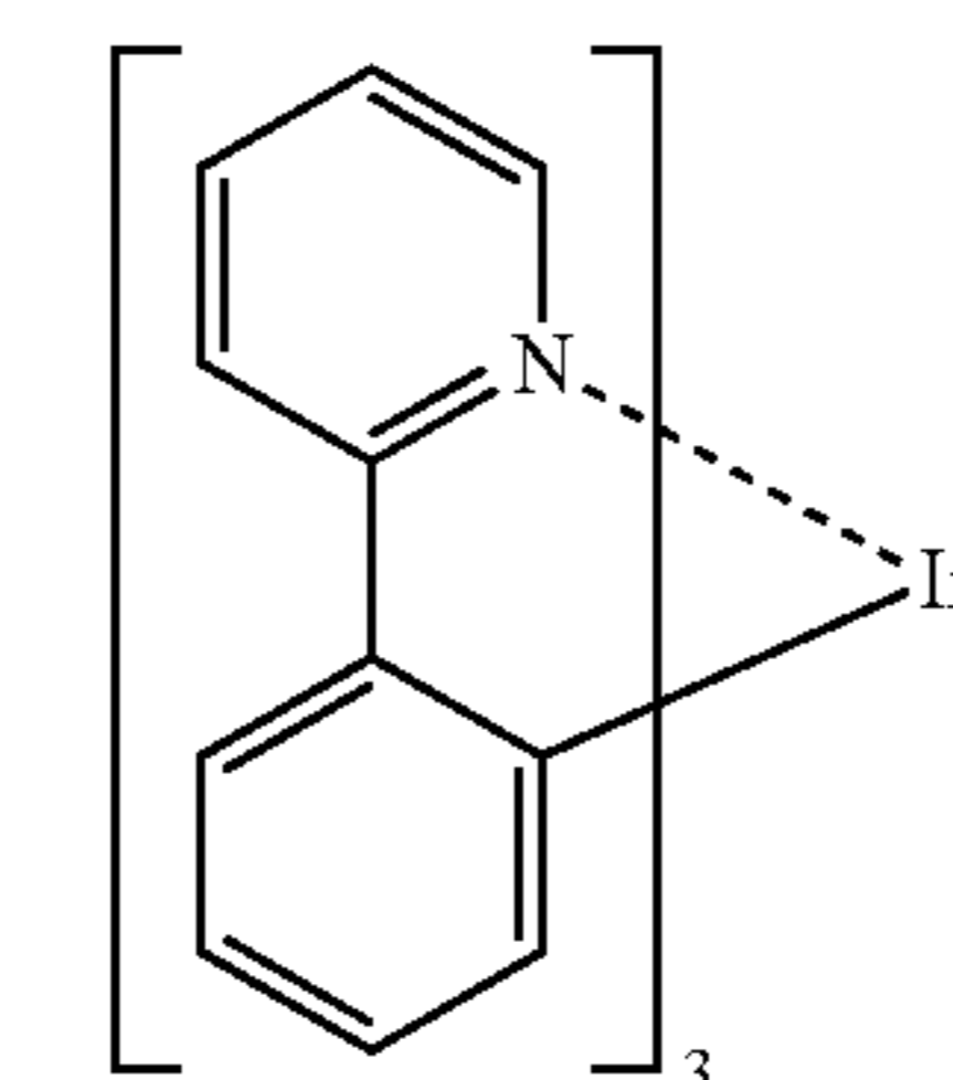
Ir(ppy)3 E^T = 2.45 eV Ionization potential = 5.2 eV
