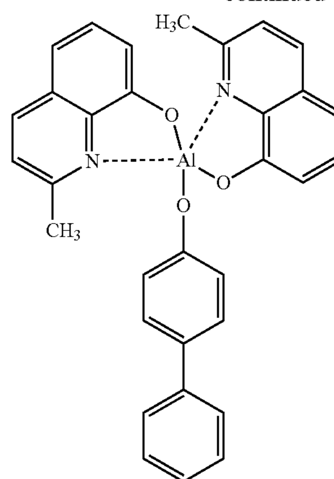
BAlq E^T = 2.4 eV Affinity = 3.0 eV
