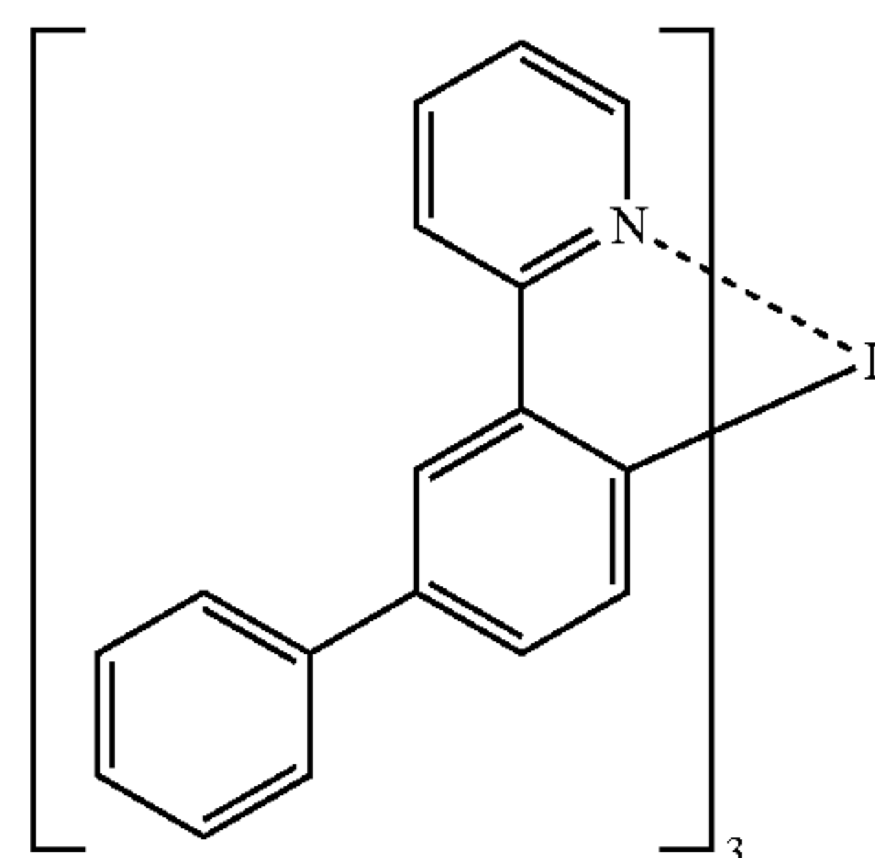
Ir(Ph-ppy)3 E^T = 2.4 eV Ionization potential = 5.3 eV
