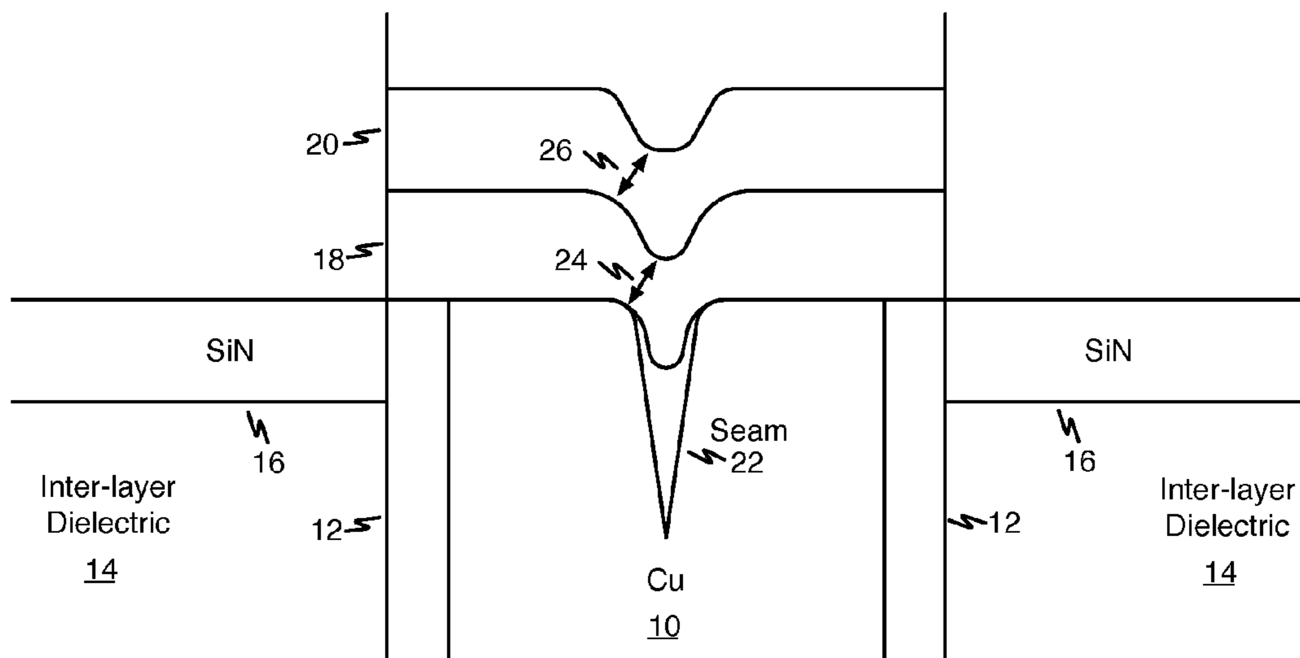
FIGURE 5 (PRIOR ART)
