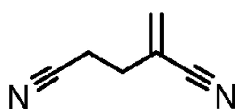
19 D 2-methyleneglutaronitrile
