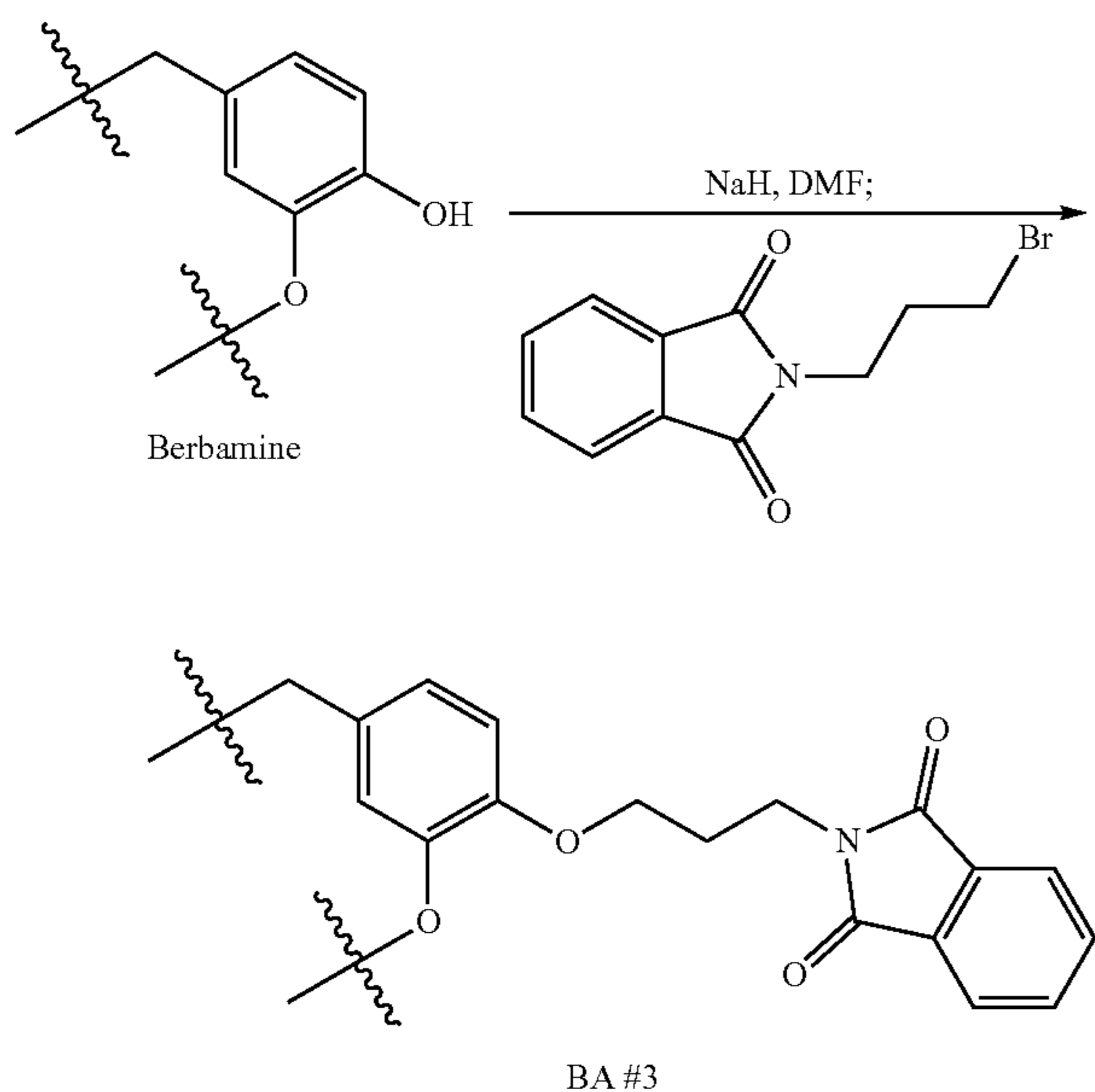
Scheme 1. Synthesis of BA #3.
