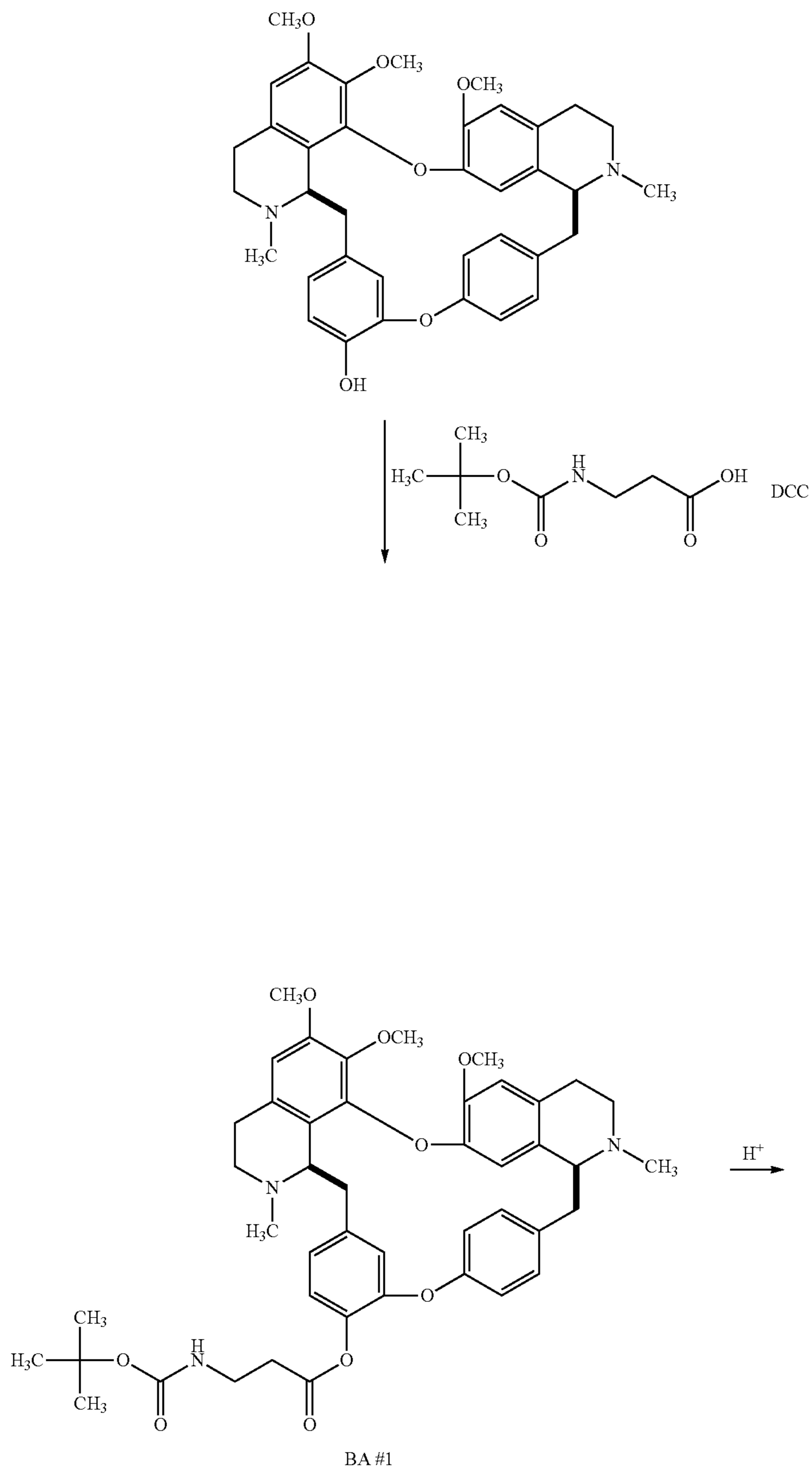
Scheme 4. Synthesis of BA #1 and BA #2
