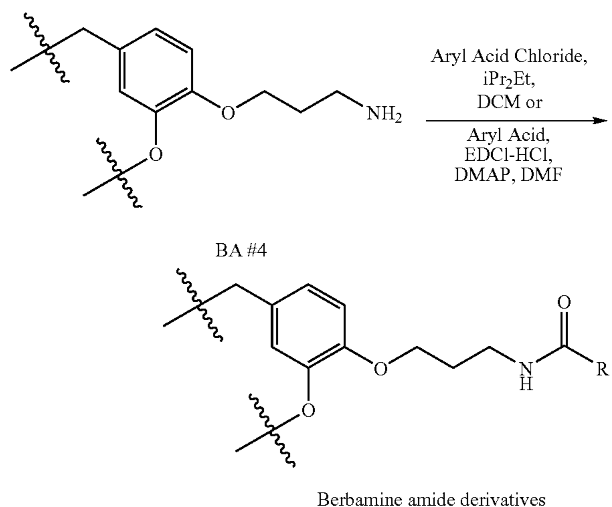
Scheme 3. Synthesis of berbamine amide derivatives.
