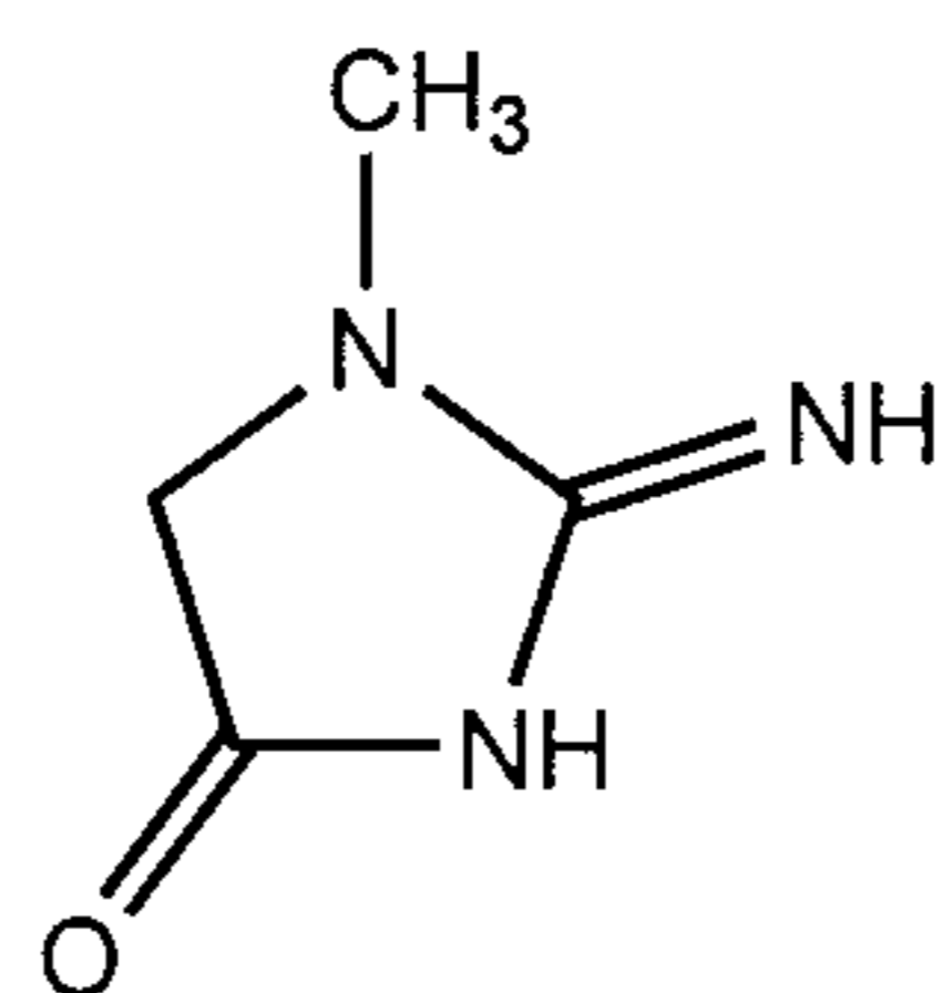
Creatinine (1)
